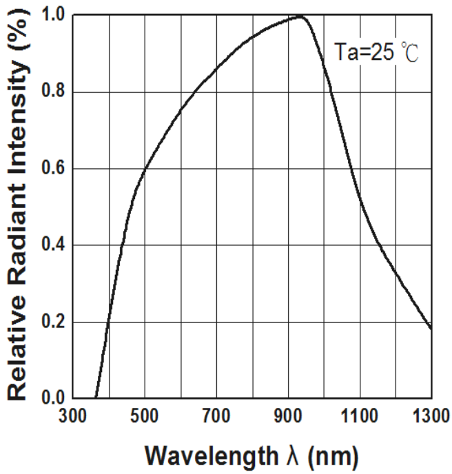
Fig. Spectral Sensitivity
