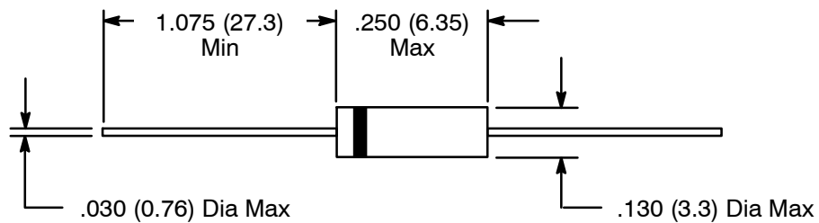
DO-15 (1N5060, 1N5061)
