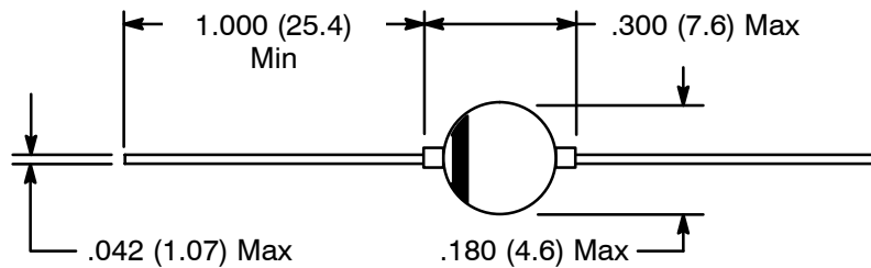
SOD-64 (1N5059, 1N5062)
