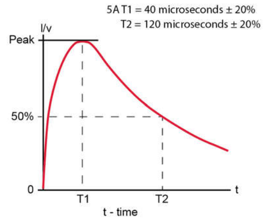
FIGURE 9 – Waveform 5A
