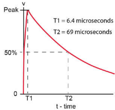
FIGURES 8 – Waveform 4
