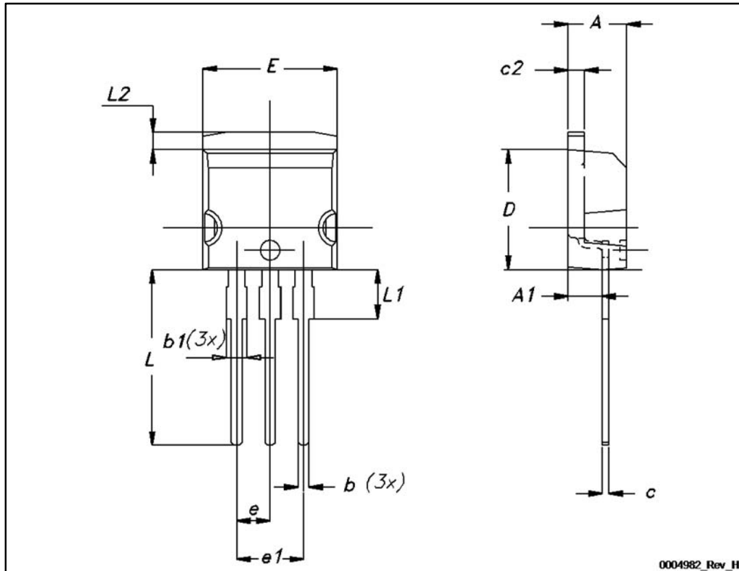
Figure 20: I 2 PAK package outline
