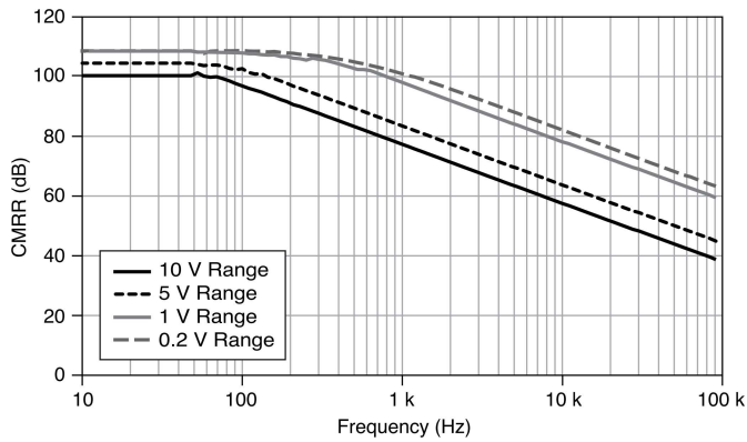
Figure 3. AI CMRR
