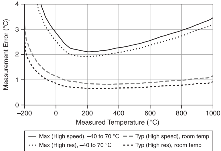
Figure 5. Thermocouple Type B Errors
