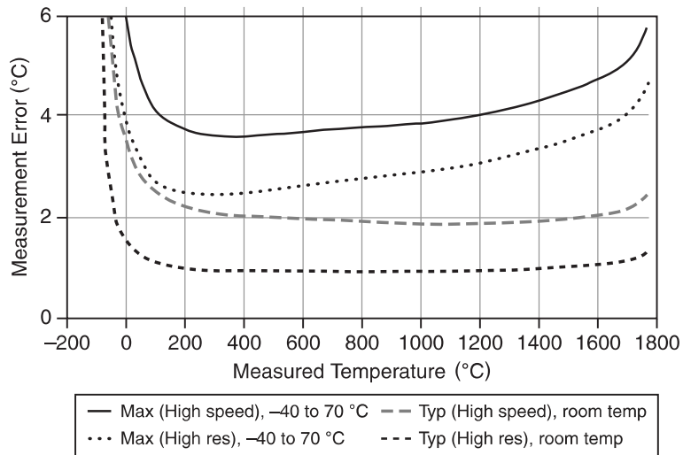
Figure 6. Thermocouple Types R and S Errors
