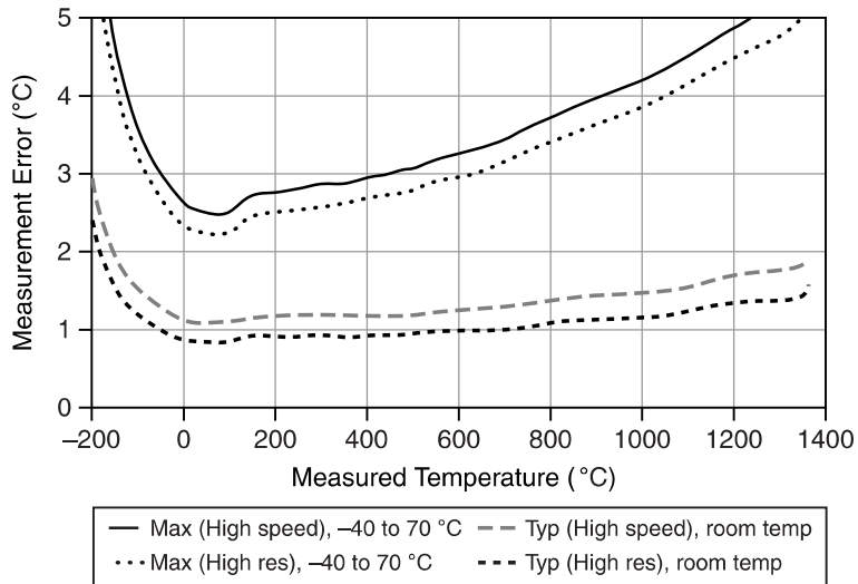
Figure 3. Thermocouple Type K Errors
