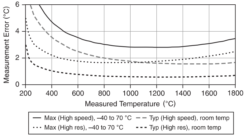
Figure 6. Thermocouple Types R and S Errors
