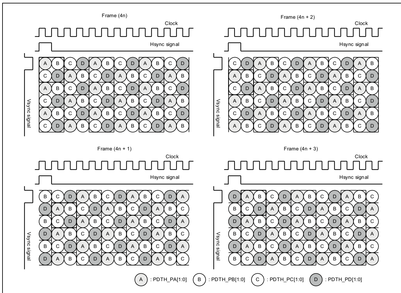
Figure 38.63 Operation Specification of 2 \times 2 Pattern Dither
