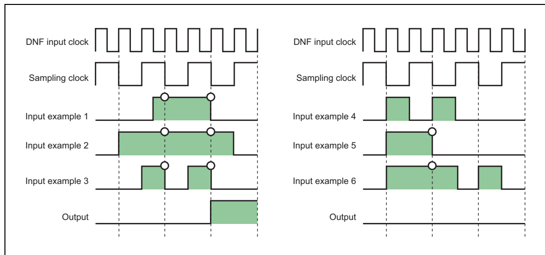
Figure 2.15 Timing Chart of Digital Noise Elimination
