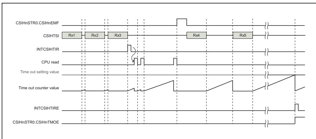
Figure 19.38 Time-Out Check Functional Timing Diagram
