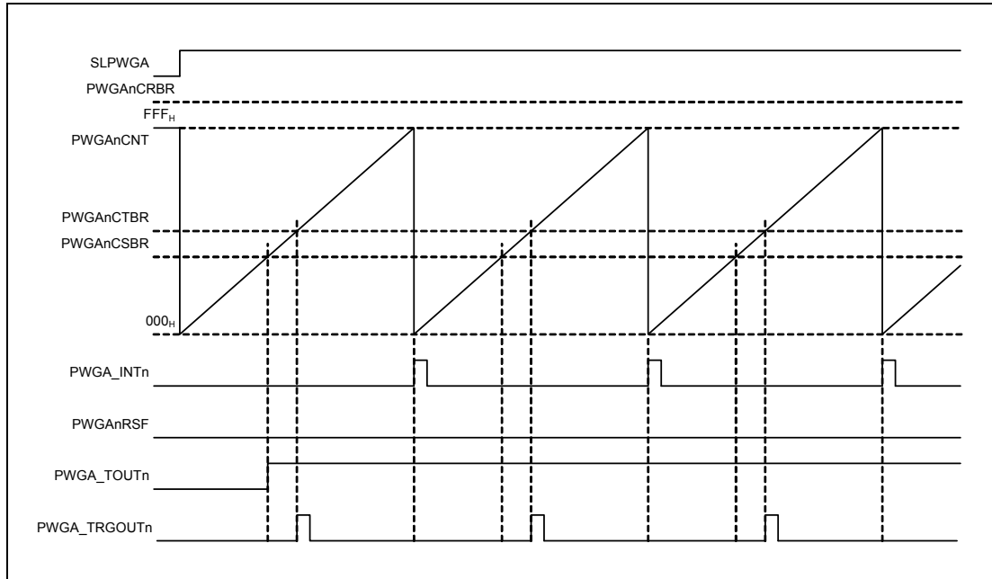
Figure 32.9 PWGA_TOUTn = 100% Output Waveform
