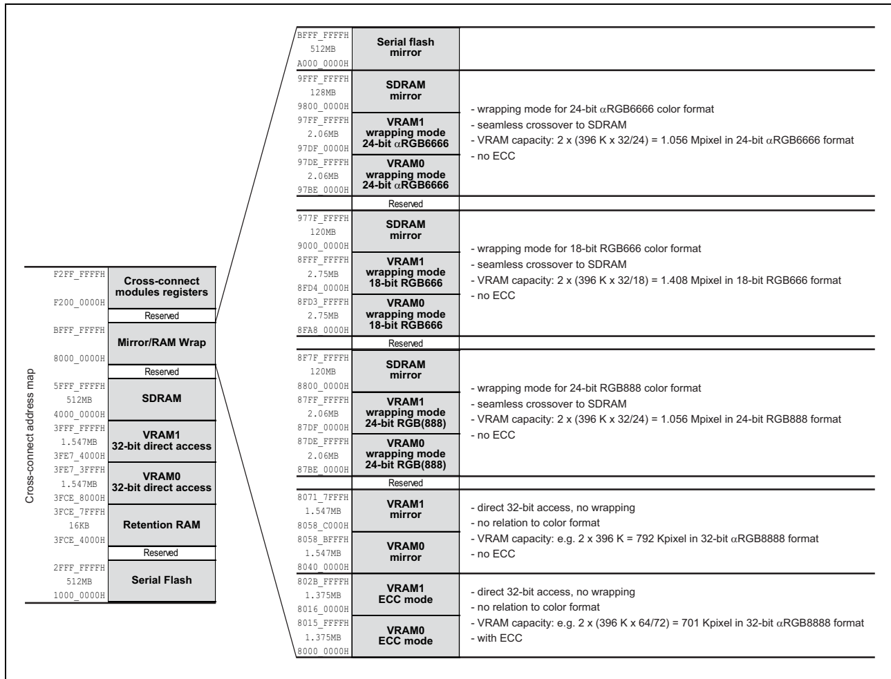
Figure 54.12 D1M2(H) Mirror/RAM Wrap mapping
