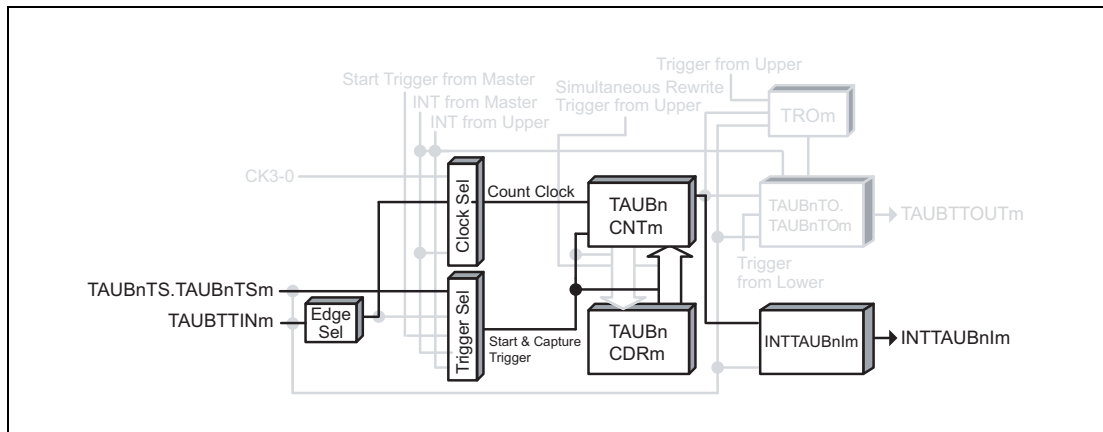
Figure 29.40 Block Diagram for External Event Count Function
