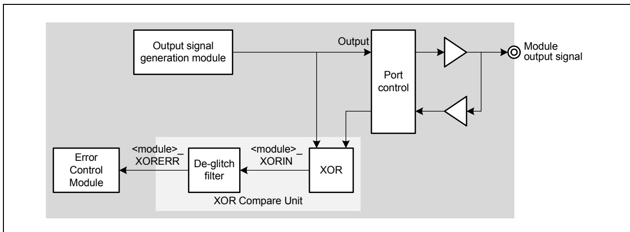
Figure 2.14 Port output check by XOR Compare Units
