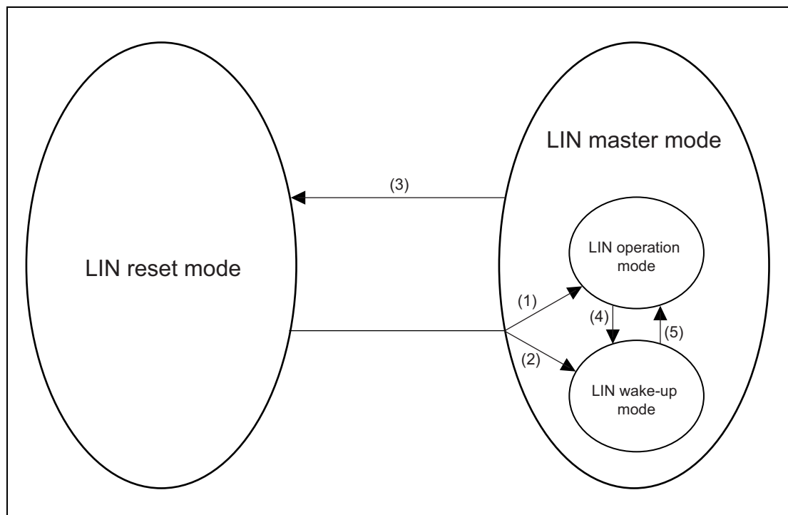
Figure 20.3 Transition of Operation Modes
