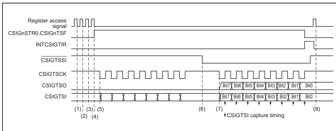
Figure 18.15 Rx/Tx Communication Timing in Slave Mode
