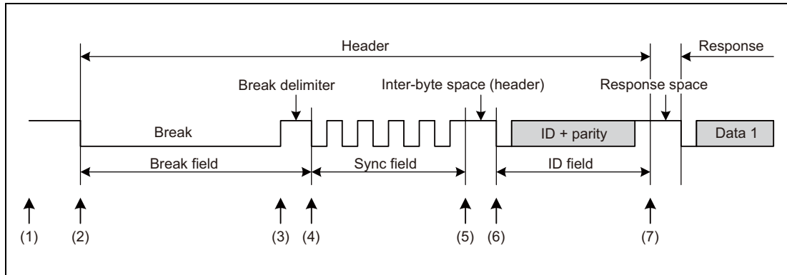
Figure 20.4 Operation in Header Transmission
