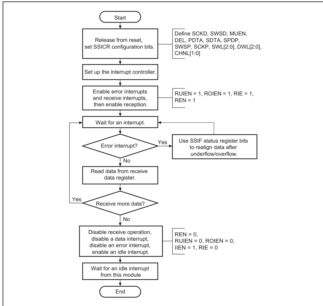
Figure 35.26 Reception Using Interrupt-Driven Data Flow Control
