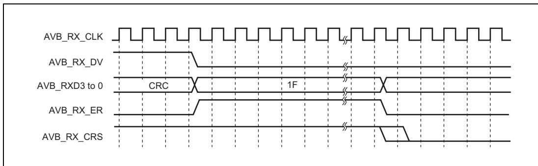
Figure 24.73 MII Frame Receive Timing (Error with Carrier Extension)
