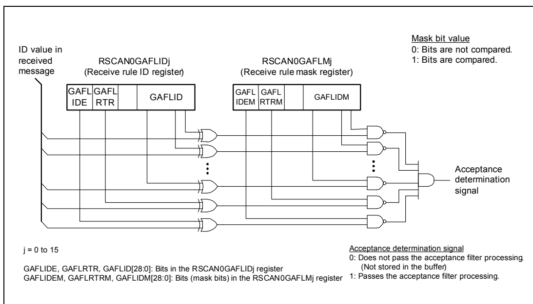
Figure 22.7 Acceptance Filter Function
