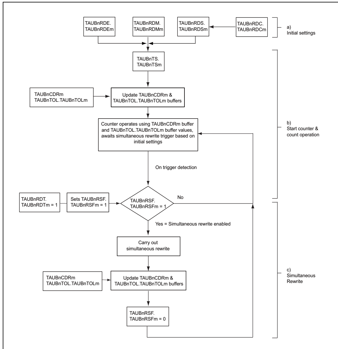
Figure 29.4 General Procedure for Simultaneous Rewrite
