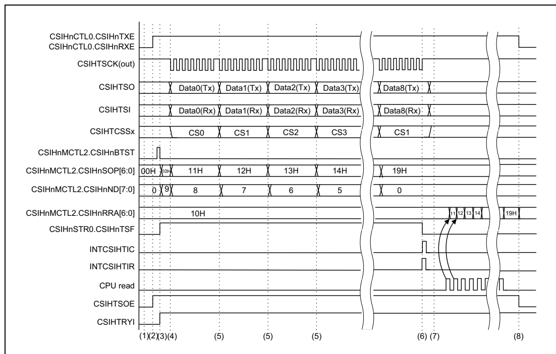
Figure 19.54 Master in Dual Buffer Mode, CSIHnCTL1.CSIHnJE = 0
