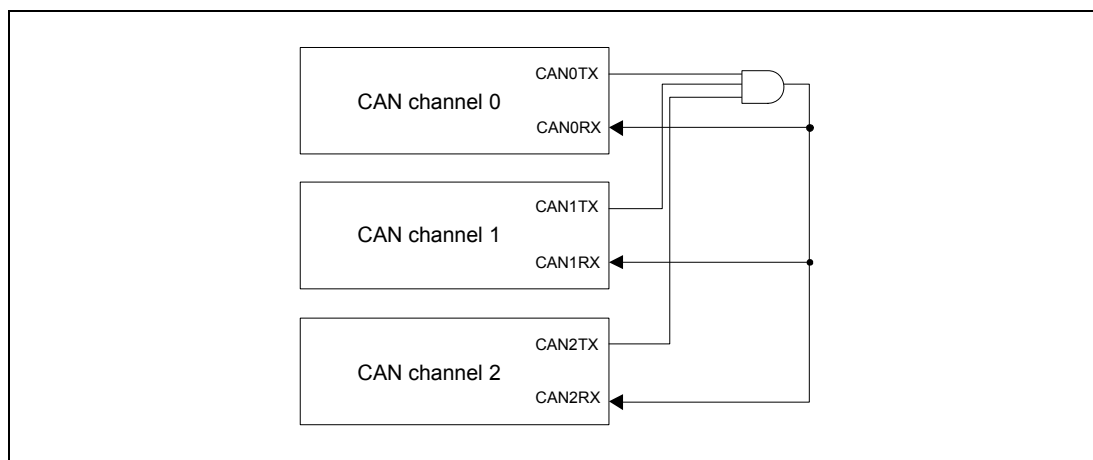
Figure 23.15 Connection for Inter-Channel Communication Test
