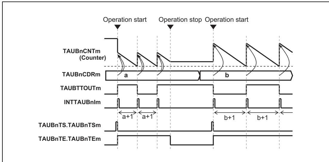
Figure 29.28 Operation Stop and Restart, TAUBnCMORm.TAUBnMD0 = 1
