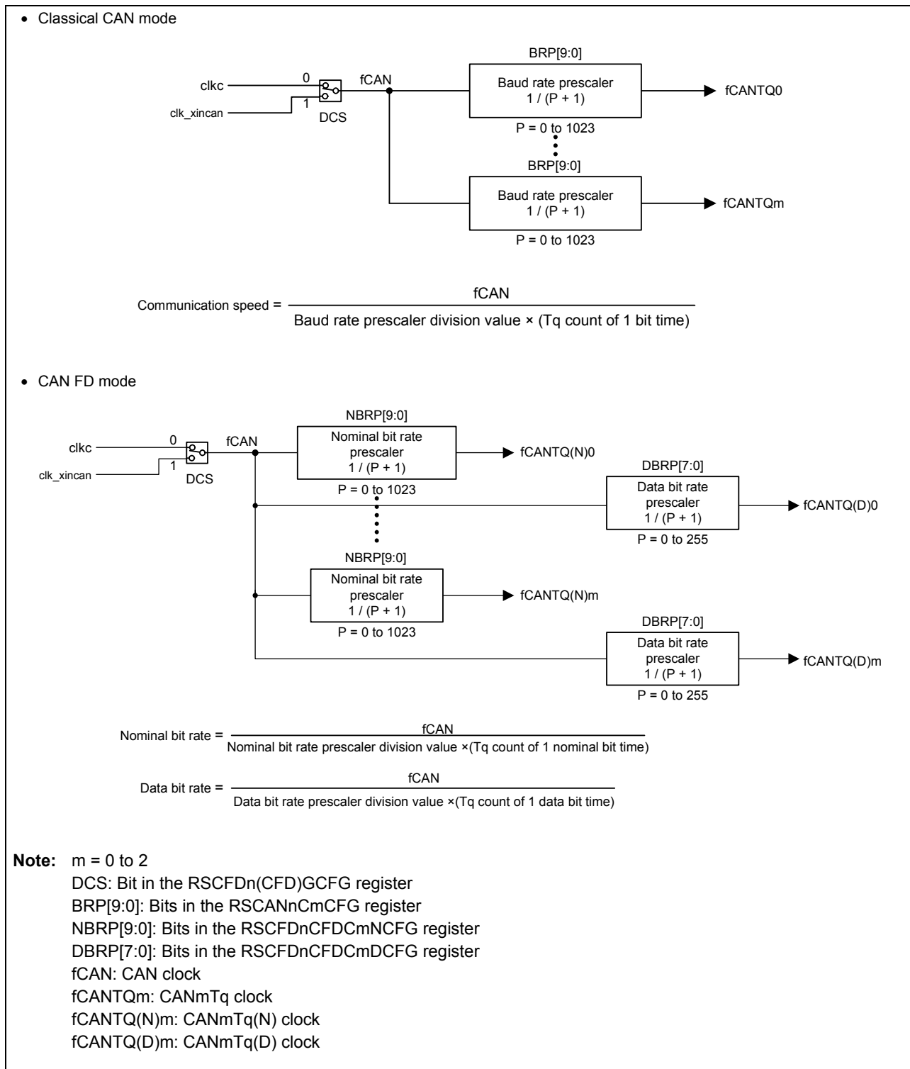
Figure 23.18 CAN Clock Control Block Diagram
