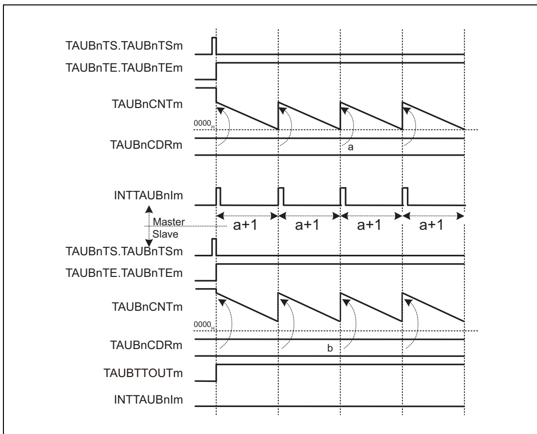
Figure 29.81 TAUBnCDRm (slave) ≥ TAUBnCDRm (master) + 1, Positive Logic (TAUBnTOL.TAUBnTOLm (slave) = 0)
