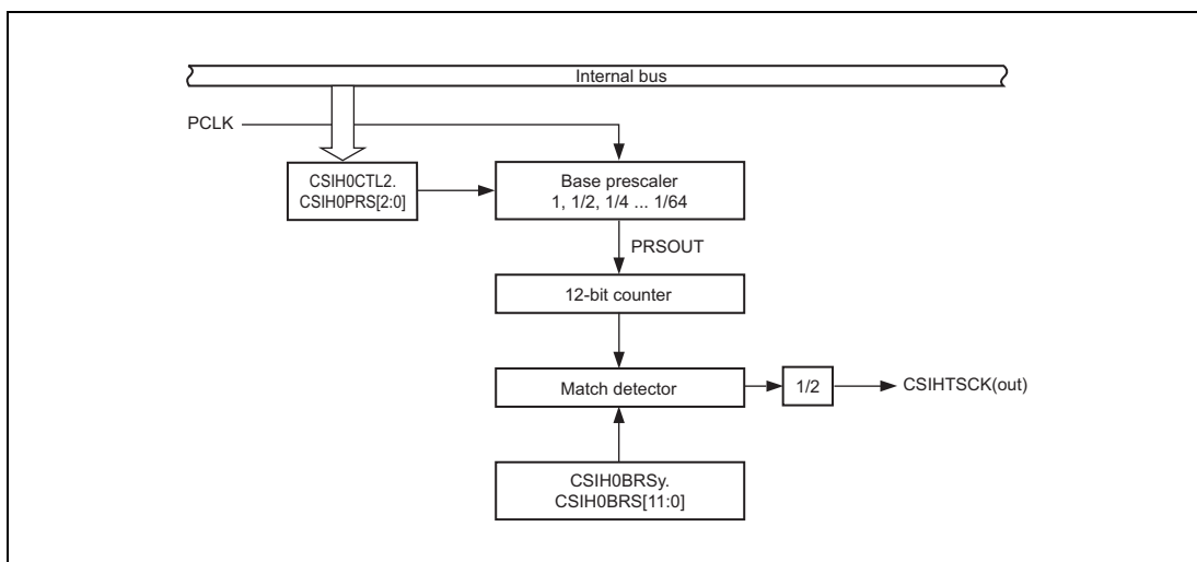
Figure 19.21 CSIH0 Baud Rate Generator Block Diagram
