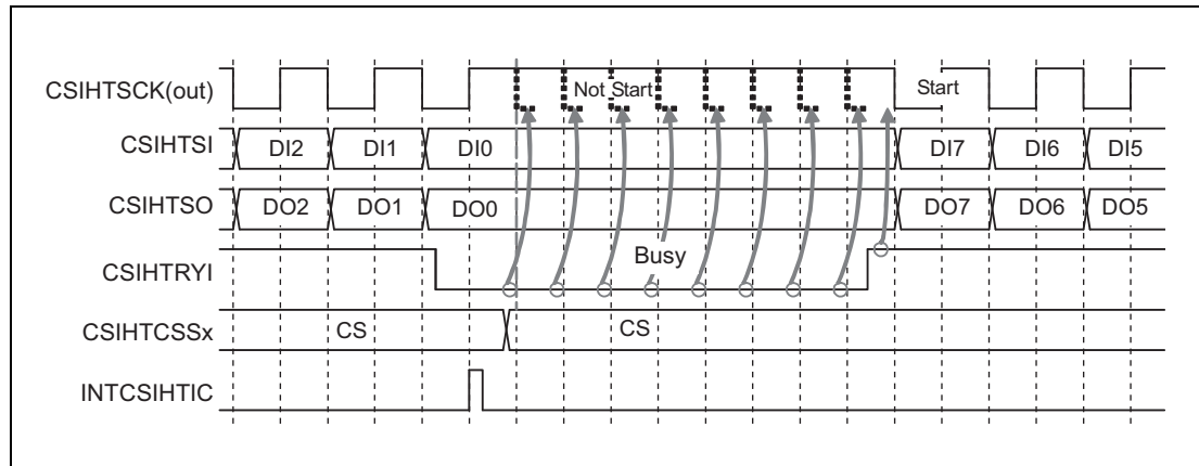
Figure 19.34 Master's Reaction on CSIHTRYI ( CSIHnCFGx.CSIHnDAPx = 0 )
