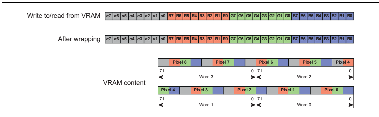
Figure 54.3 Direct 32-bit mode without ECC
