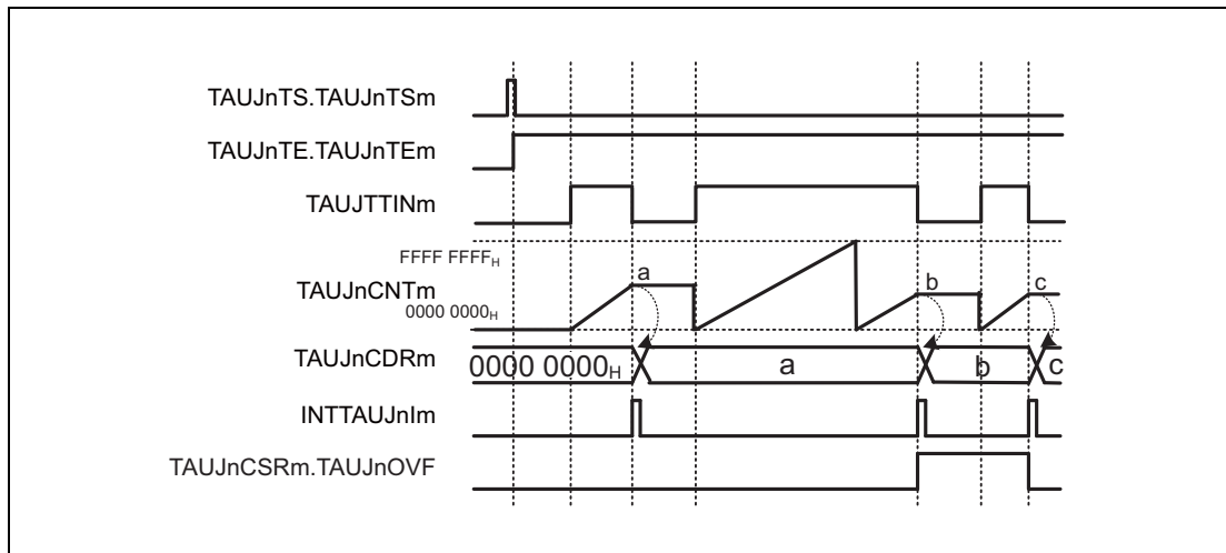
Figure 30.29 \text{TAUJnCMORm.TAUJnCOS}[1:0] = 00_{\text{B}} , \text{TAUJnCMORm.TAUJnMD0} = 0 , \text{TAUJnCMURm.TAUJnTIS}[1:0] = 11_{\text{B}}
