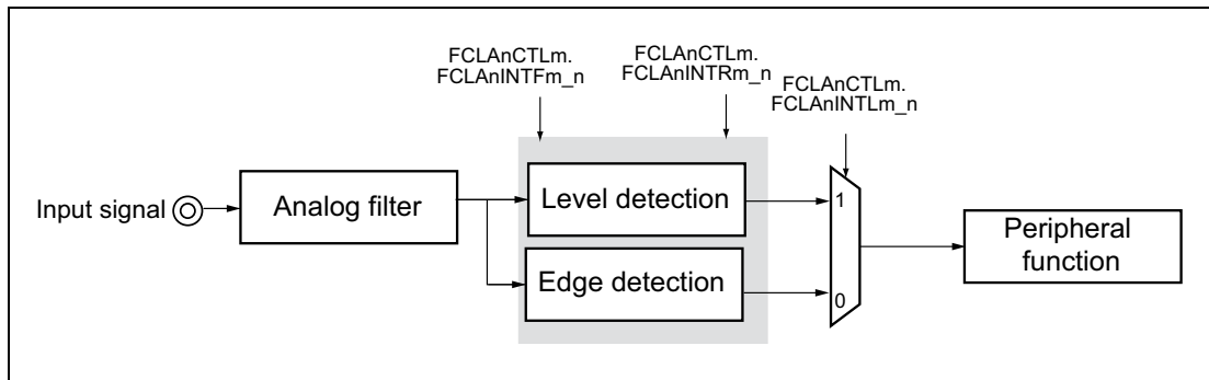
Figure 2.17 Block Diagram of Analog Filter Type B
