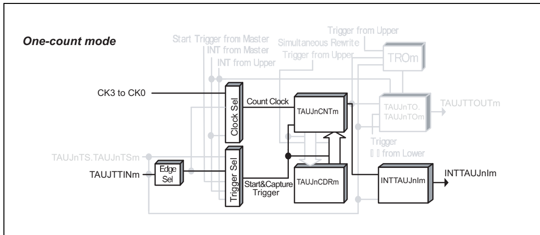
Figure 30.39 Block Diagram for Overflow Interrupt Output Function (during TAUJTTINm Width Measurement)
