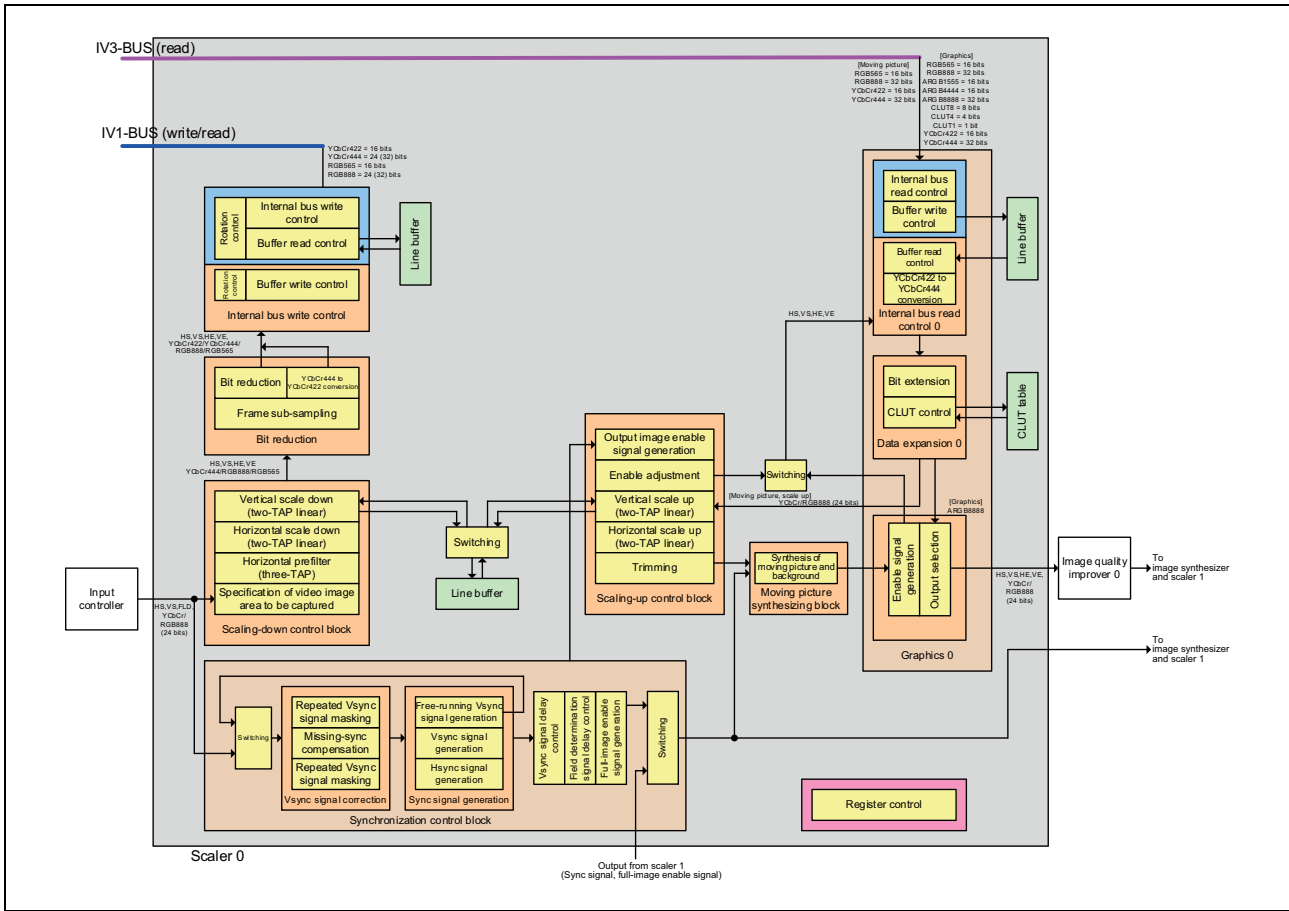
Figure 38.24 Functional Block Diagram of Scaler 0
