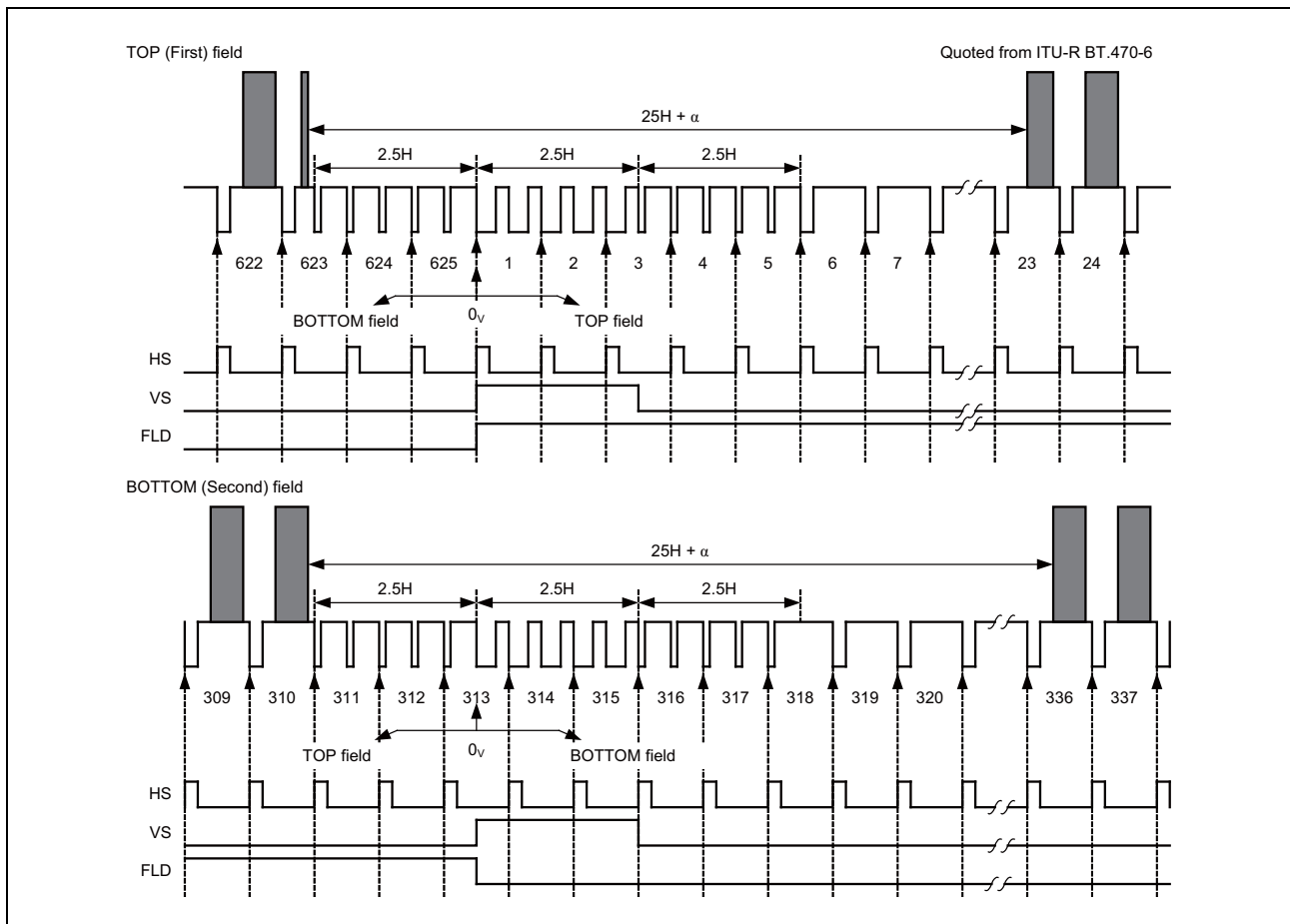
Figure 38.11 BT601 Vertical Timing (625 Lines/50.00 Hz)
