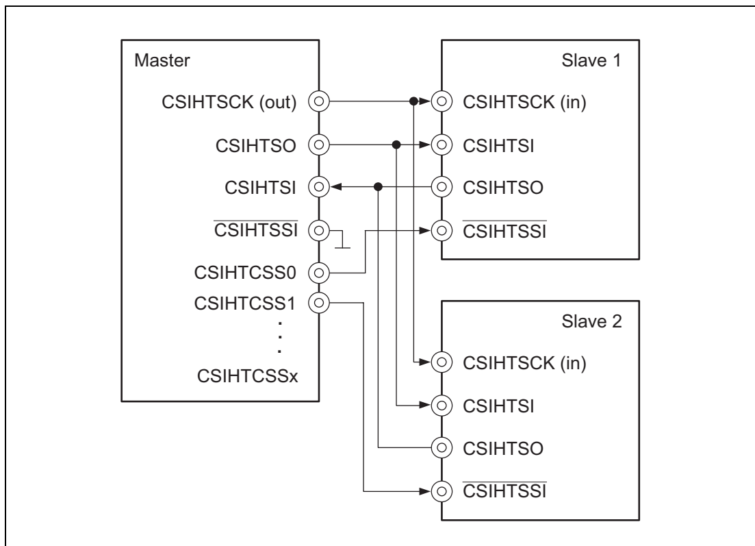
Figure 19.12 Connections between One Master and Multiple Slaves
