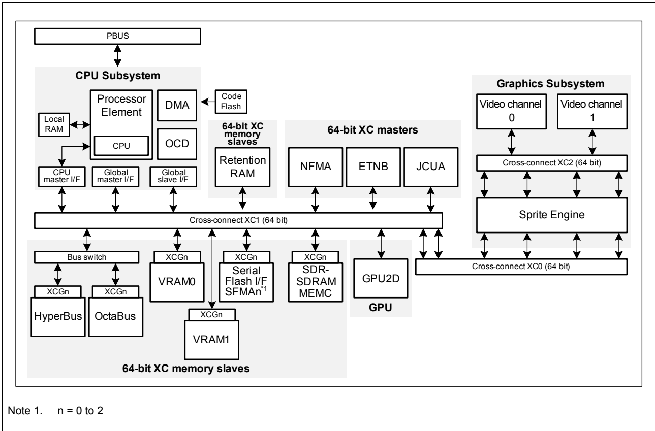
Figure 14.15 D1M1A bus architecture overview
