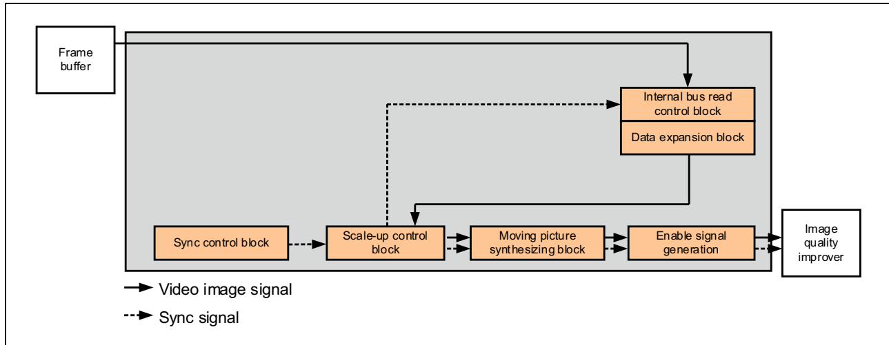
Figure 38.41 Signal Paths for Scaled-up Graphics Display
