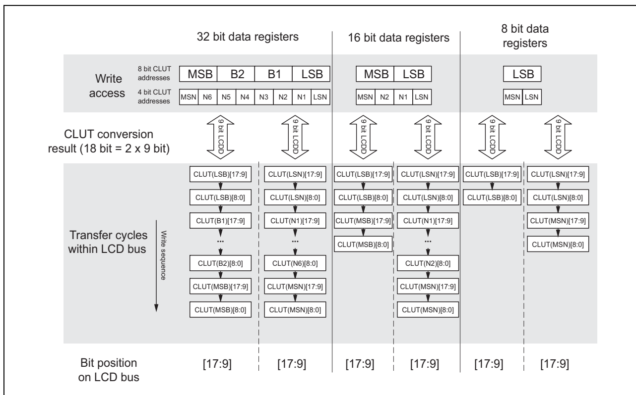
Figure 36.10 Data transfer types with CLUT usage on 9-bit LCD bus
