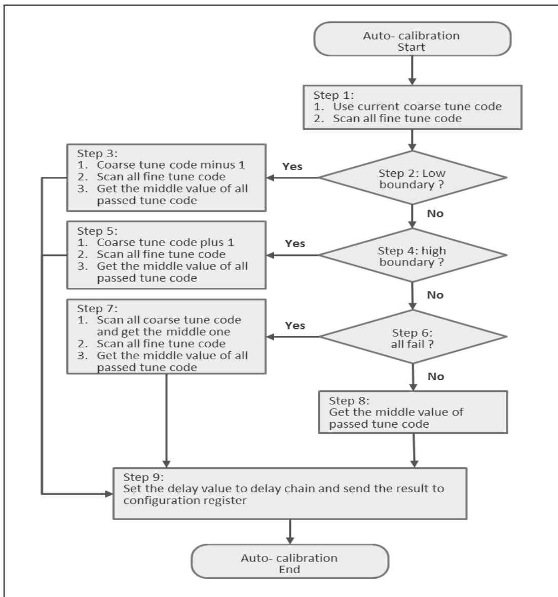
Figure 57.7 Auto-calibration flow chart
