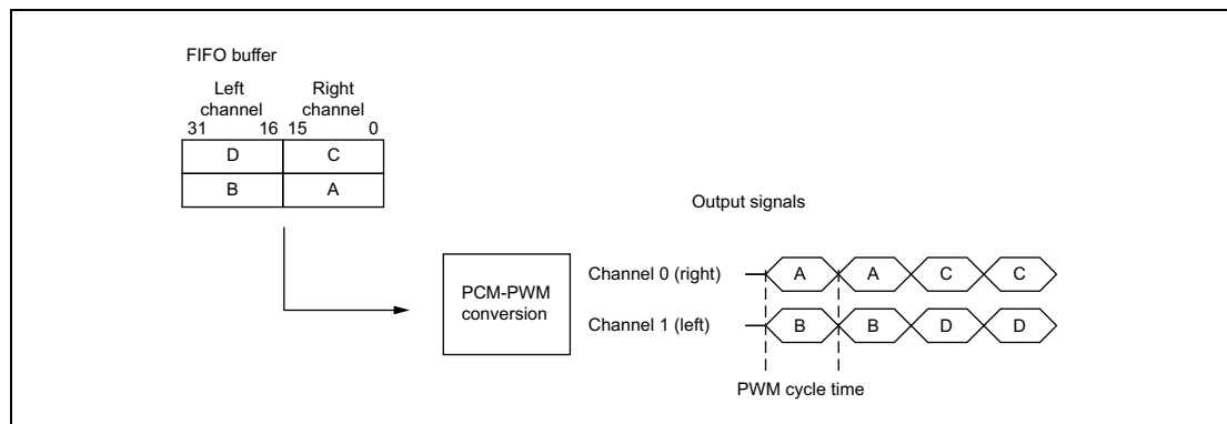
Figure 34.7 Double output mode (in stereo mode)
