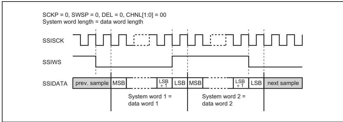
Figure 35.2 I 2 S Compatible Format (without Padding)
