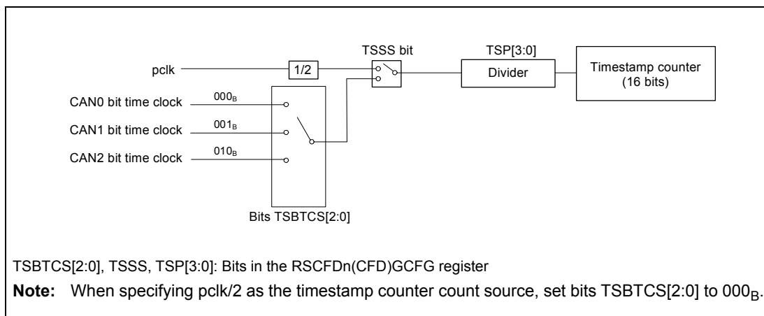
Figure 23.8 Timestamp Function Block Diagram
