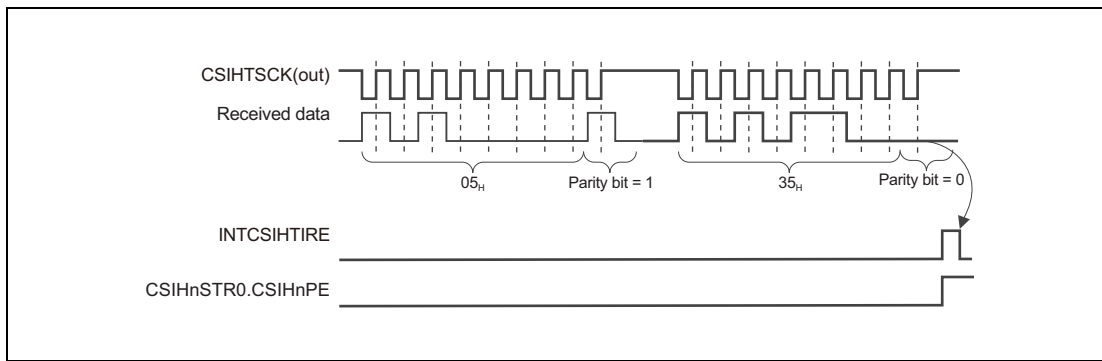
Figure 19.37 Parity Check Example
