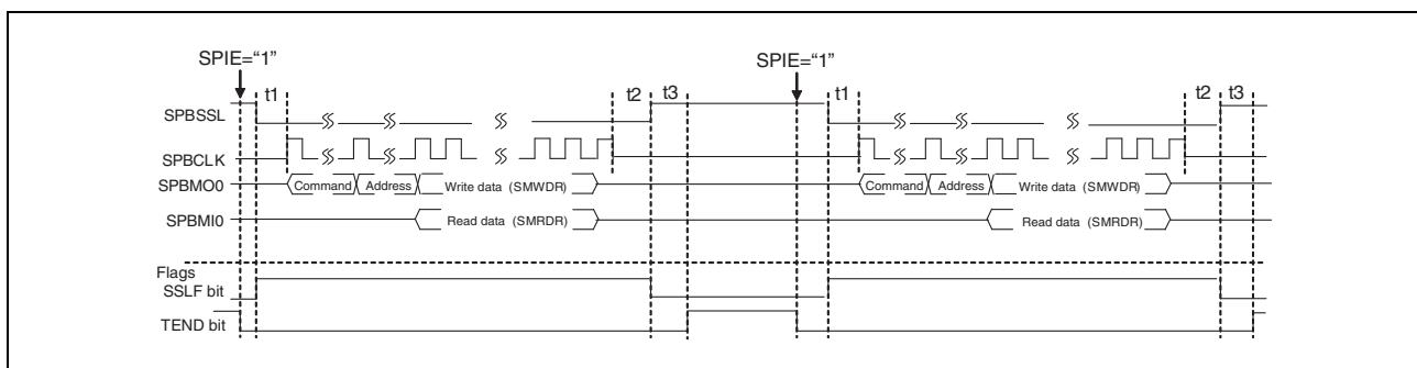
Figure 17.14 SPI Operation Timing
