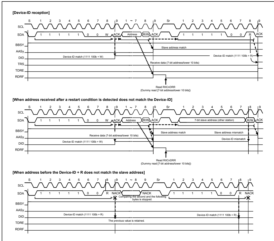
Figure 21.28 AASy/DID Flag Set/Clear Timing during Reception of Device-ID
