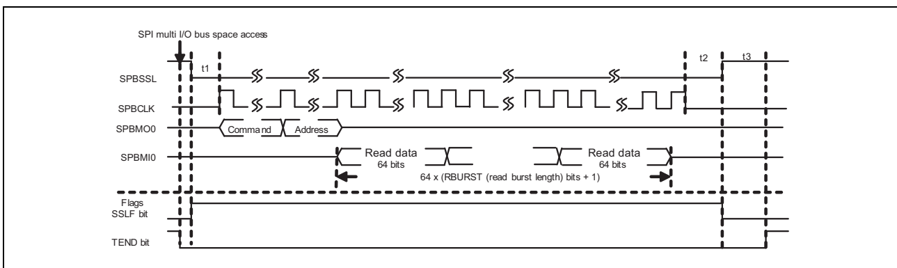
Figure 17.9 Burst Read Operation Timing (SSLE Bit = 0)
