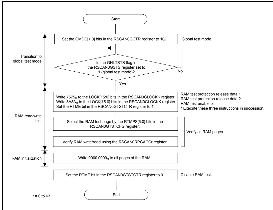
Figure 22.36 RAM Test Setting Procedure
