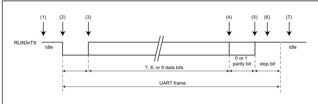
Figure 20.20 LIN/UART Interface (in UART Mode) Reception Operation
