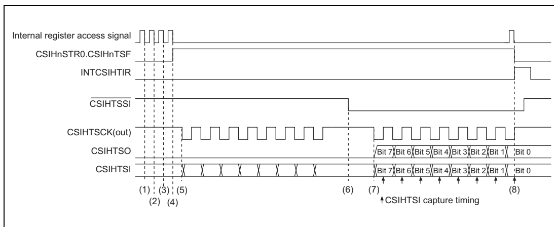
Figure 19.28 Tx/Rx Timing of Communication Using SS Function
