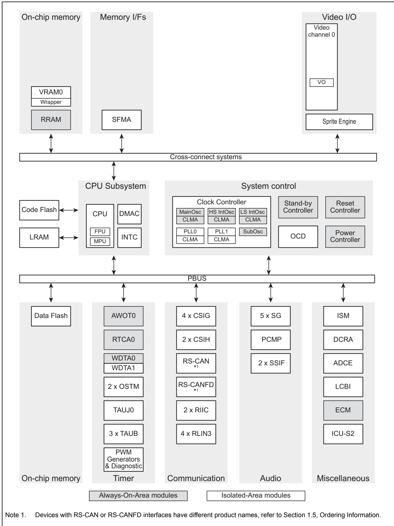
Figure 1.2 D1L2(H) block diagram
