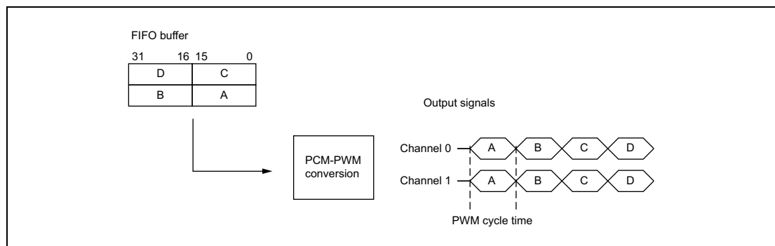
Figure 34.5 PCM-PWM in mono mode
