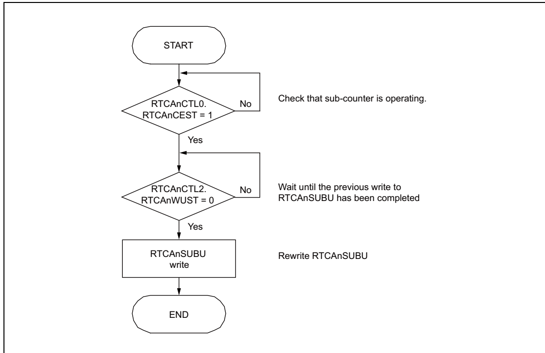
Figure 31.10 Writing to the RTCAnSUBU Register
