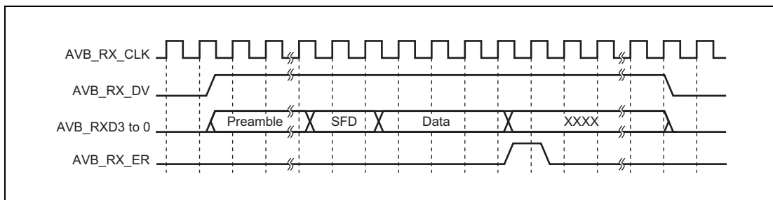
Figure 24.67 MII Frame Receive Timing (Reception Error (1))
