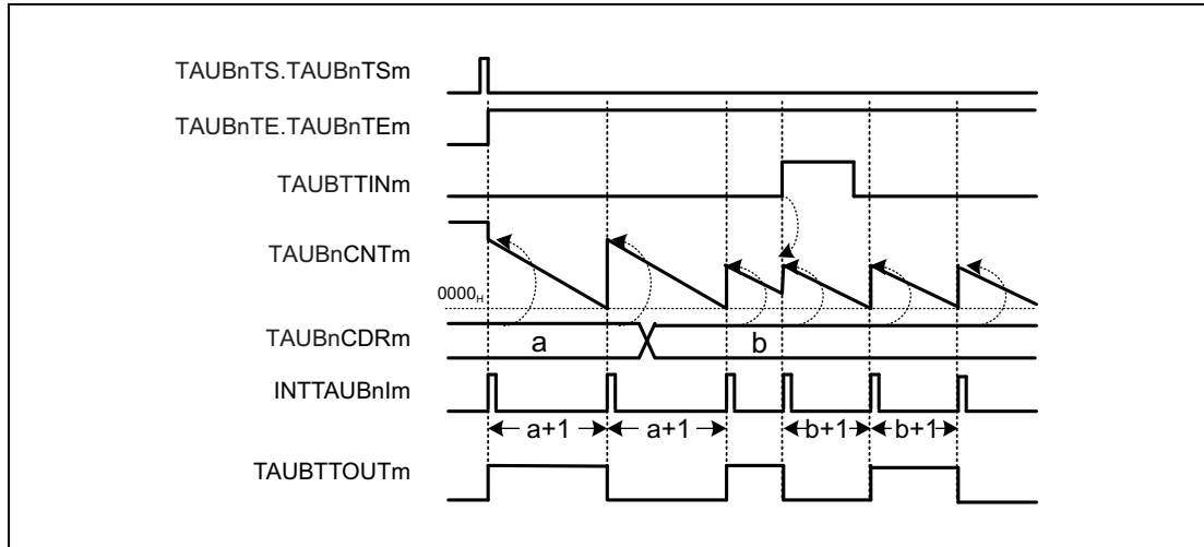
Figure 29.34 Counter Triggered by Rising TAUBTTINm Input Edge (TAUBnCMURm.TAUBnTIS[1:0] = 01 B ), TAUBnCMORM.TAUBnMD0 = 1
