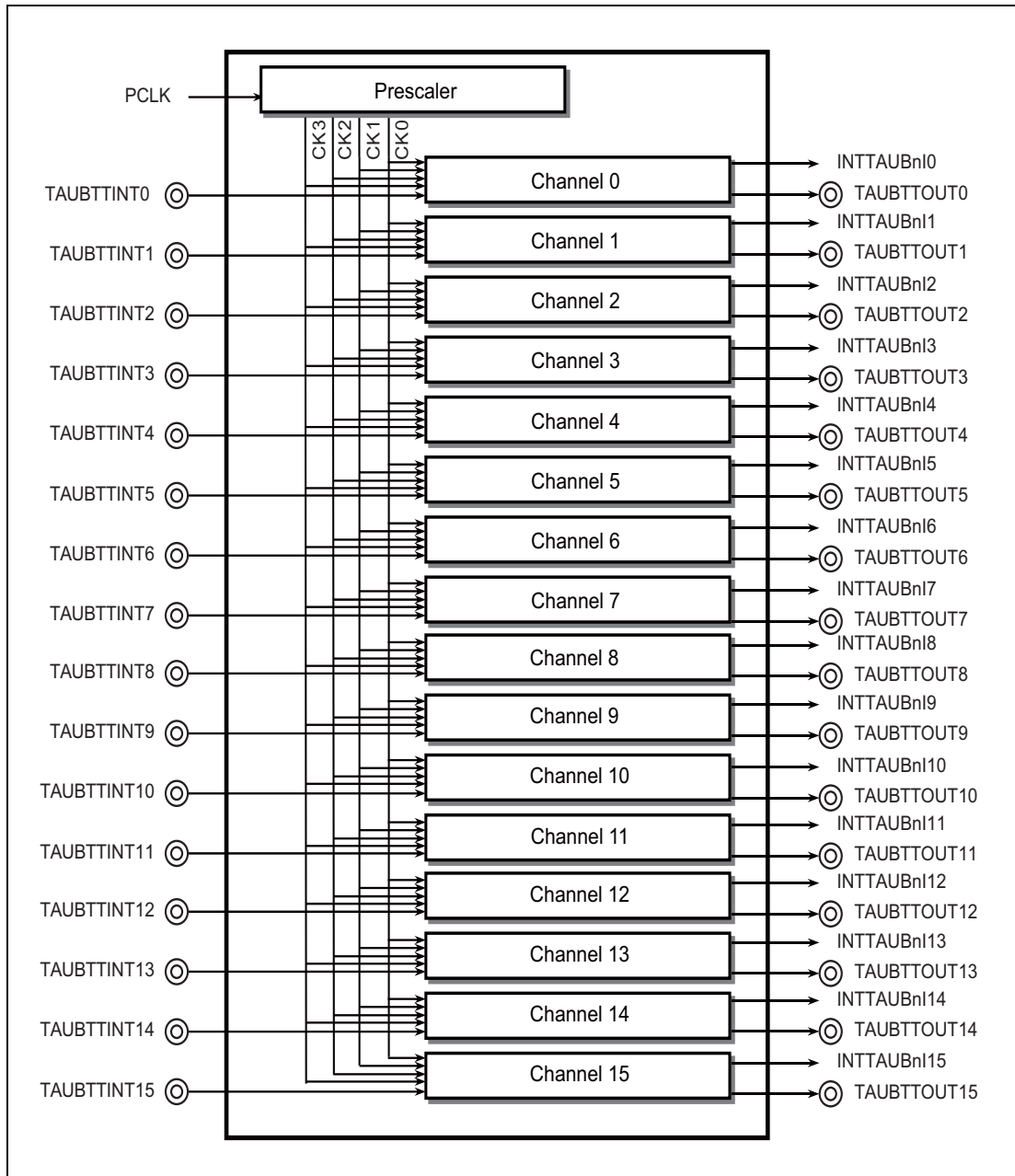
Figure 29.1 TAUB Input/Output and Interrupt Request Signals
