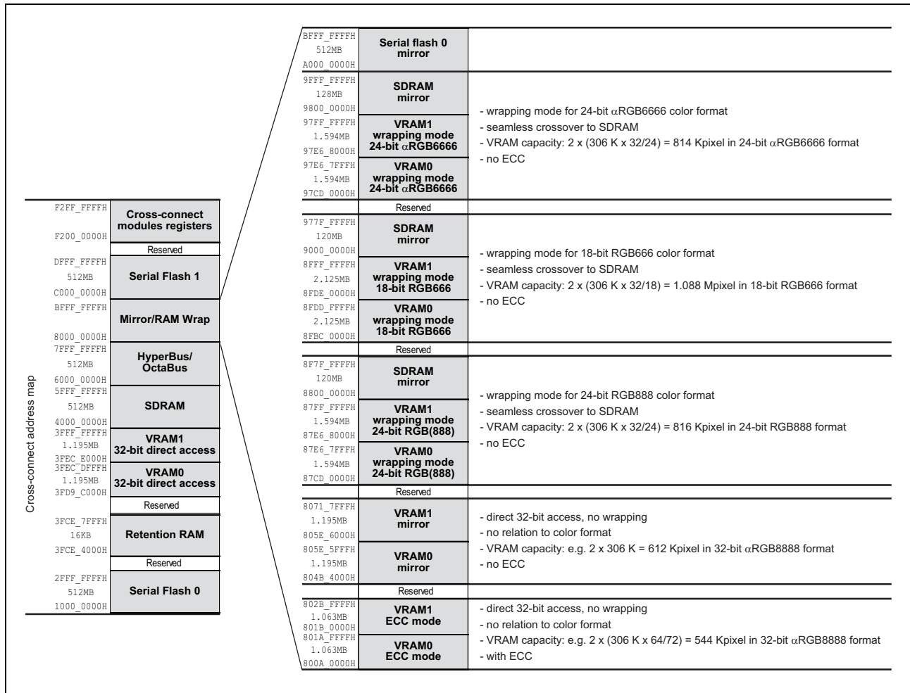
Figure 54.11 D1M1A Mirror/RAM Wrap mapping
