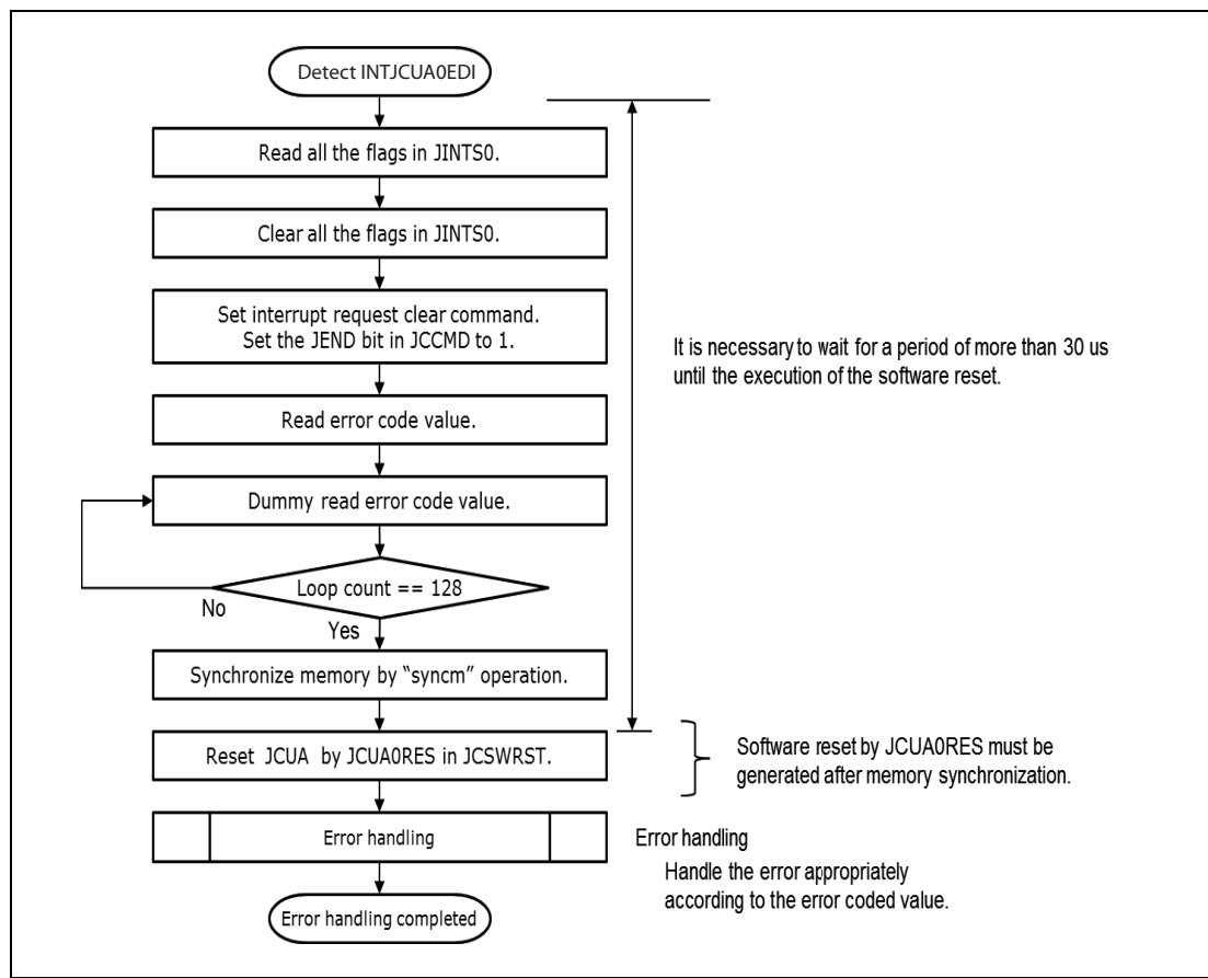
Figure 44.8 Error Handling Flow
