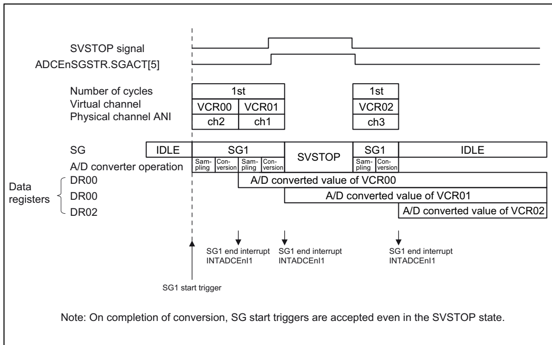
Figure 45.16 Example of SVSTOP Operation (ADCEnADCR.SUSMTD[1:0] = 00 and ADCEnEMU.SVSDIS = 0)
