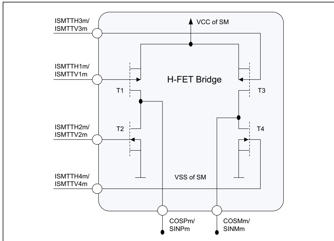
Figure 46.8 Structure of an H-FET full-bridge
