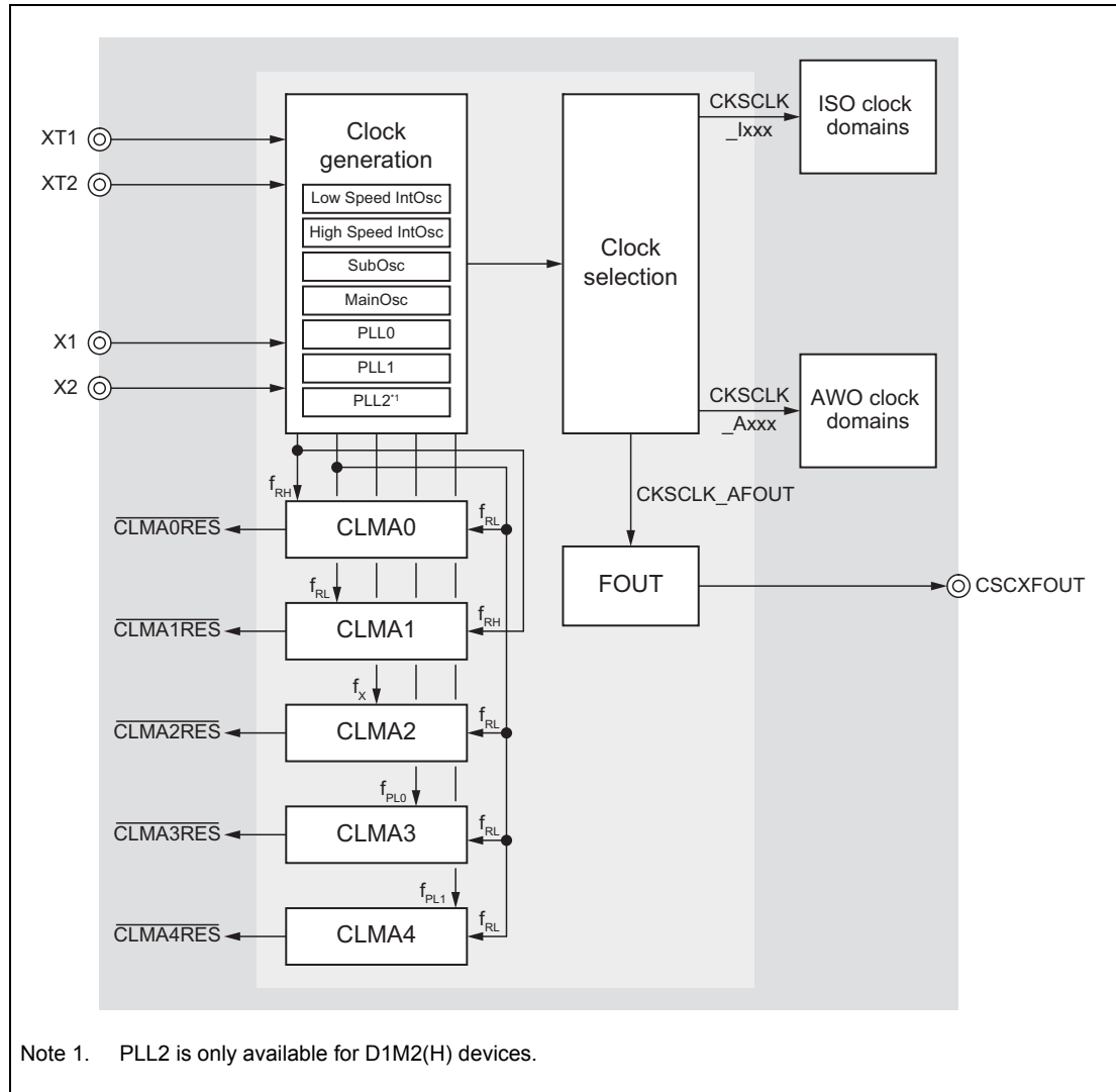
Figure 12.1 Clock Controller overview
