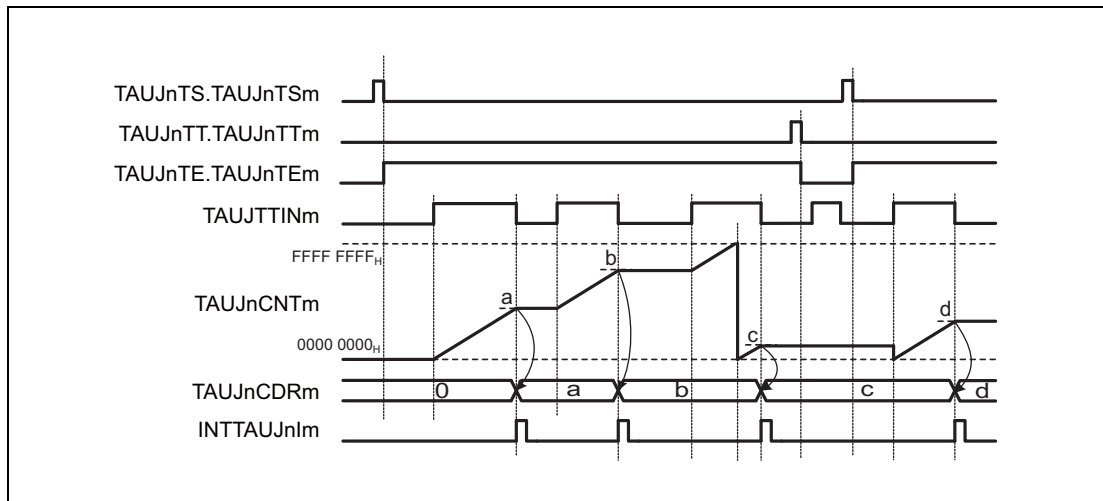
Figure 30.38 Operation Stop and Restart (TAUJnCMURm.TAUJnTIS[1:0] = 11 B )
