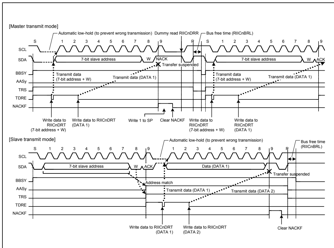
Figure 21.30 Suspension of Data Transfer when NACK is Received (NACKE = 1)
