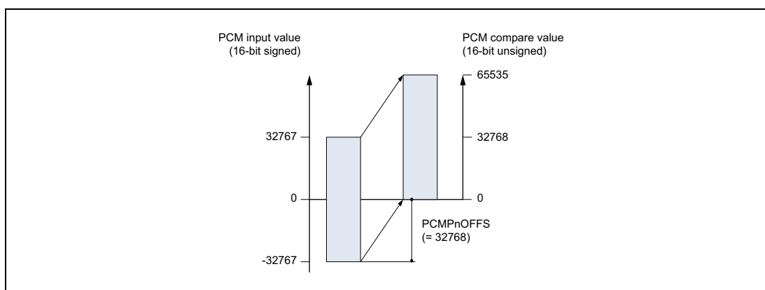
Figure 34.12 Converting the audio input in half H-bridge mode (PCMPnCTL.MODE = 0)
