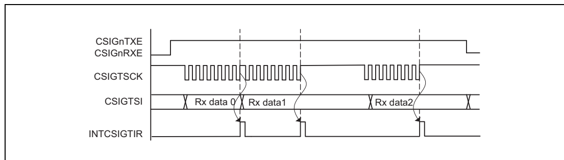
Figure 18.5 Generation of INTCSIGTIR
