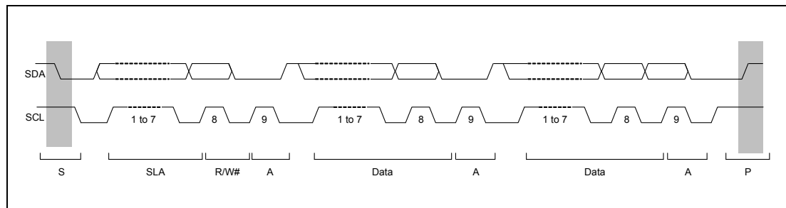
Figure 21.4 I 2 C Bus Timing (SLA = 7 Bits)
