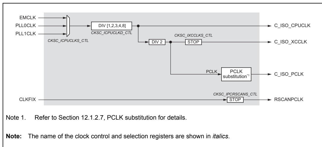
Figure 12.7 D1L1, D1L2(H) CPU and bus subsystems clock domains
