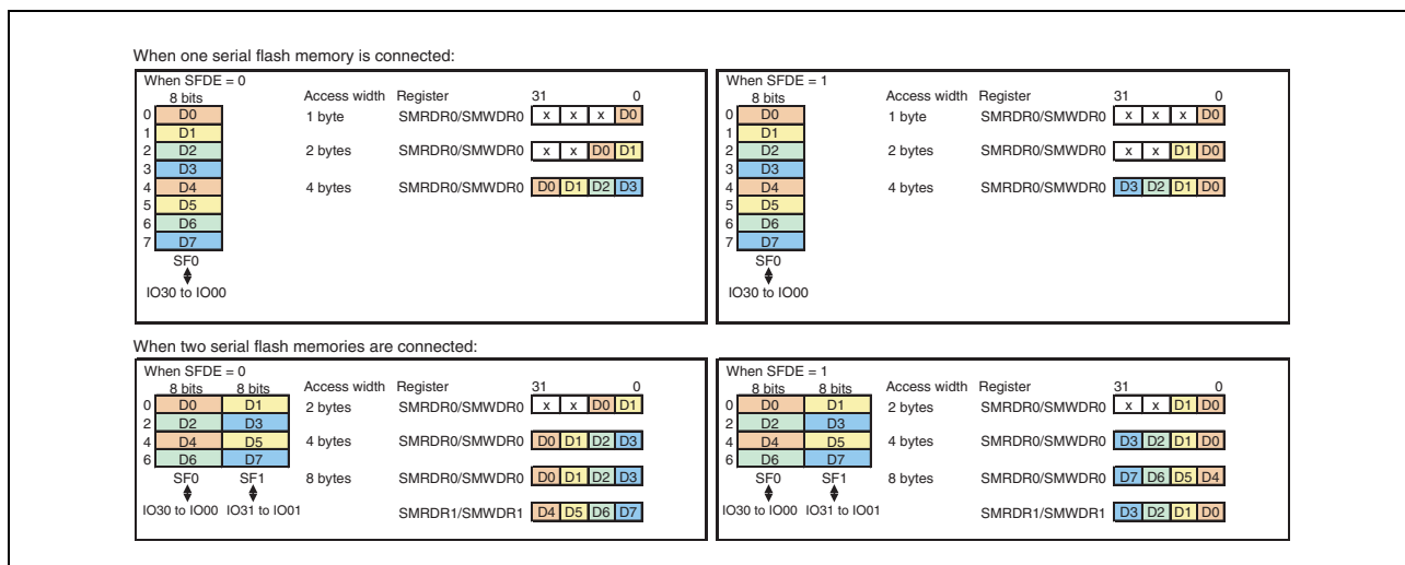
Figure 17.6 Data Alignment in SPI Mode
