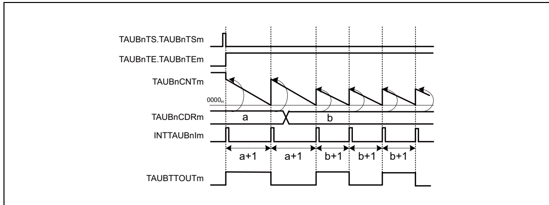
Figure 29.25 General Timing Diagram for Interval Timer Function
