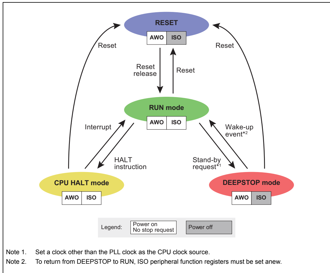
Figure 13.1 State transition diagram of stand-by mode
