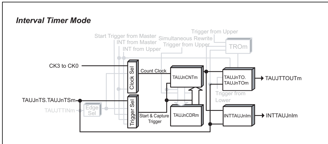
Figure 30.12 Block Diagram for Interval Timer Function
