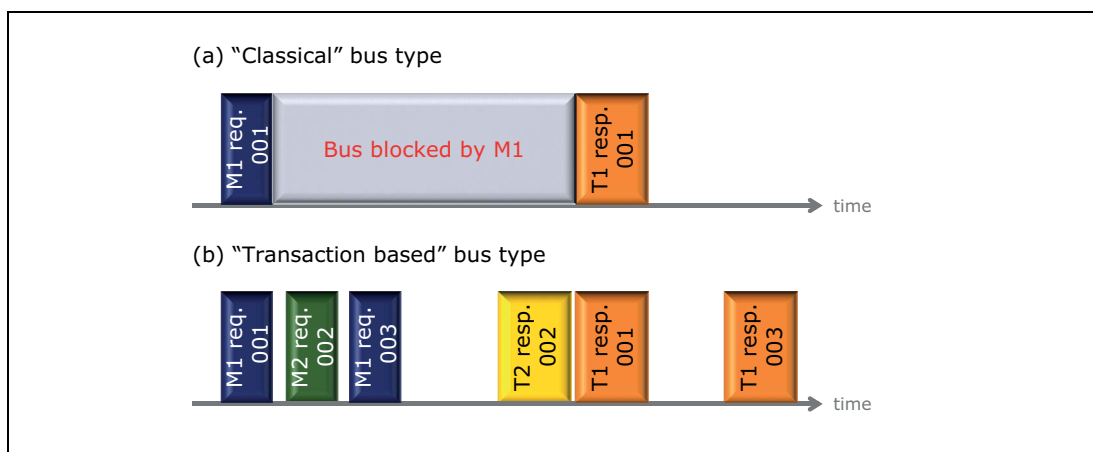
Figure 14.23 “Classical” vs. “transaction based” bus types
