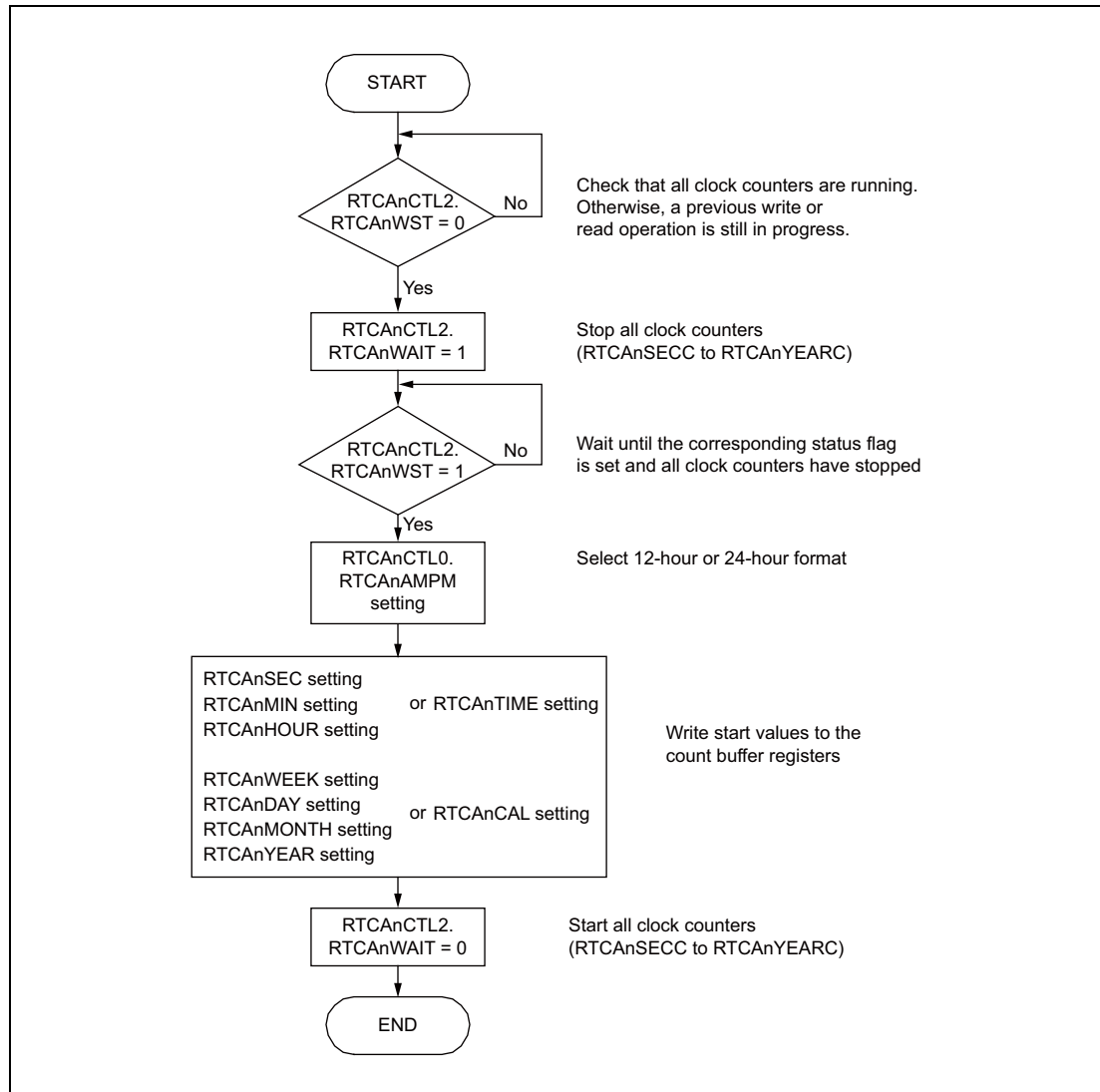
Figure 31.6 Updating Clock Counter Values
