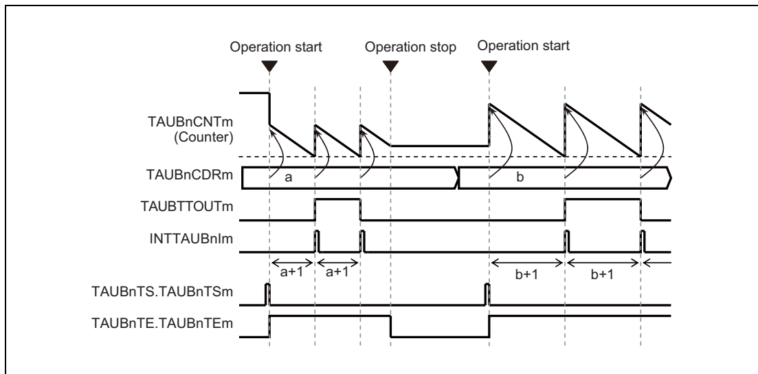
Figure 29.29 Operation Stop and Restart, TAUBnCMORm.TAUBnMD0 = 0
