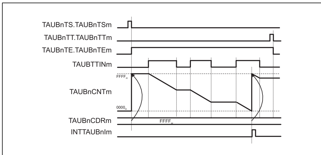
Figure 29.75 General Timing Diagram for Overflow Interrupt Output Function (during TAUBTTINm Input Period Count Detection)
