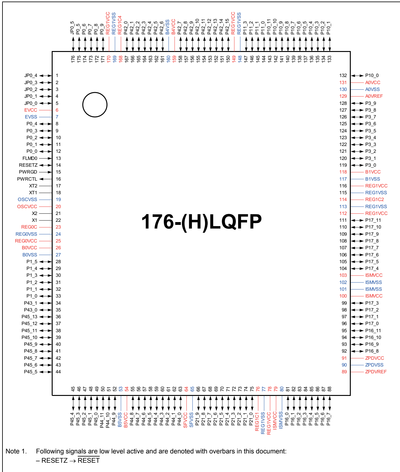
Figure 2.2 D1L2H and D1M1 pin connection diagram (176 pins (H)LQFP package)
