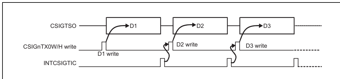
Figure 18.3 Generation of INTCSIGTIC after Communication (CSIGNCTL1.CSIGNSLIT = 0)
