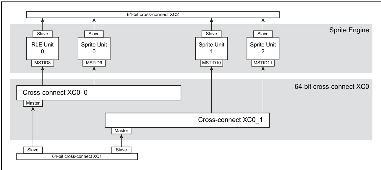
Figure 14.4 D1L2(H) cross-connect XC0
