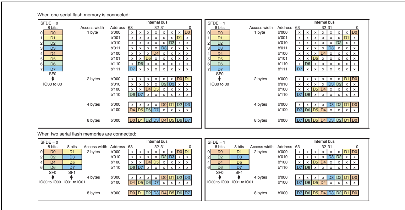
Figure 17.5 Data Alignment in Data Read Mode
