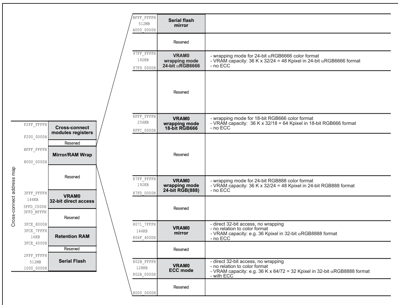
Figure 54.8 D1L2(H) Mirror/RAM Wrap mapping
