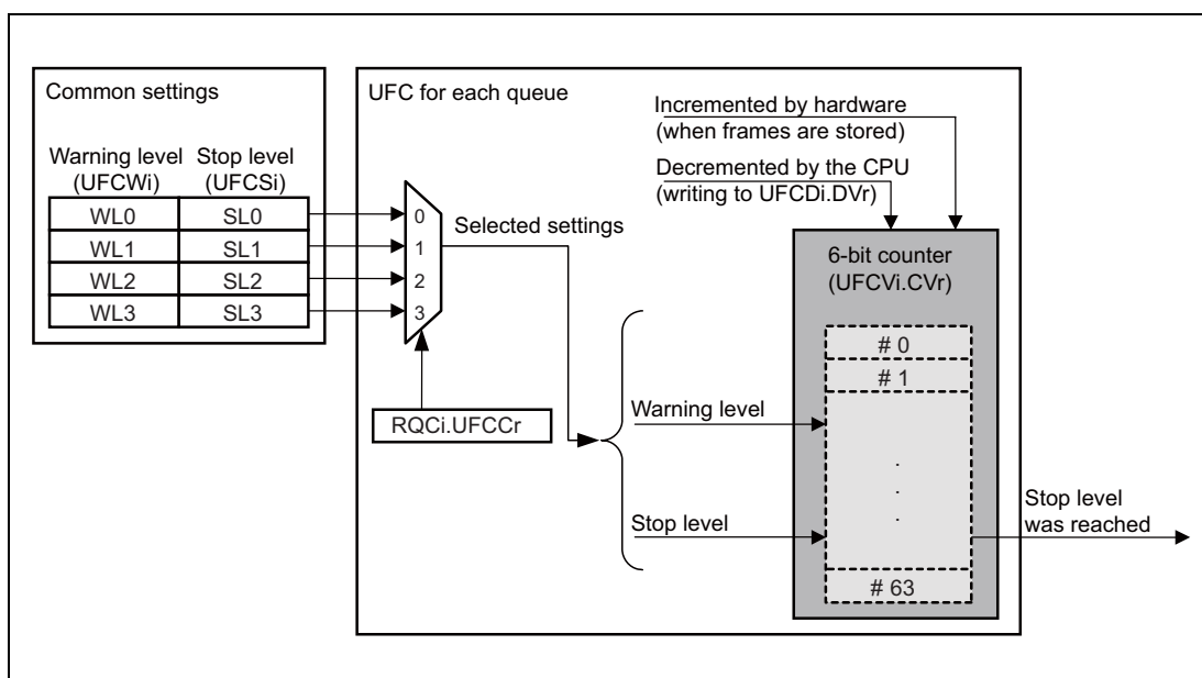
Figure 24.29 Overview of an Unread Frame Counter
