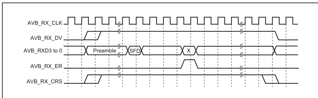
Figure 24.72 MII Fame Receive Timing (Reception Error)
