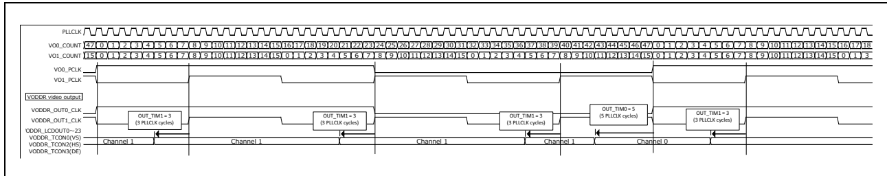
Figure 37.37 VODDR WVGA + WQVGA (60Hz) Video Output
