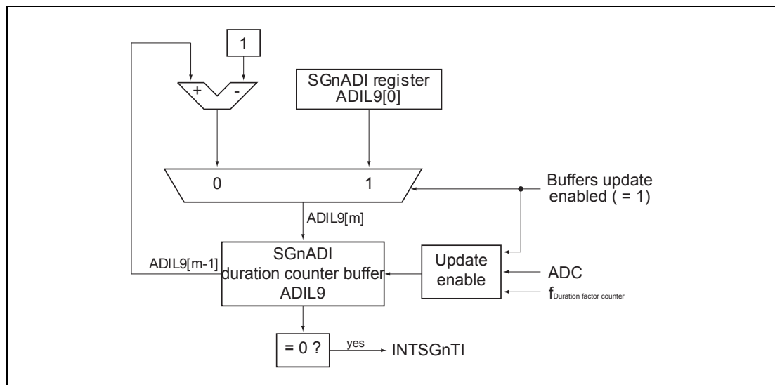
Figure 33.11 Time calculation in ADC mode
