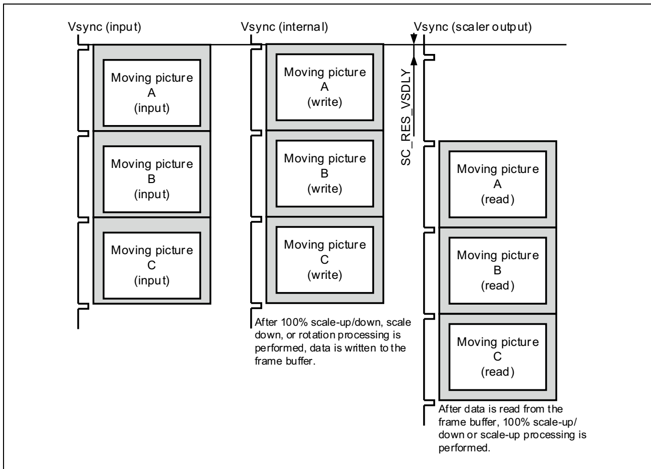
Figure 38.30 Vsync Signal Phases (Two Frame-Buffer Planes Used)
