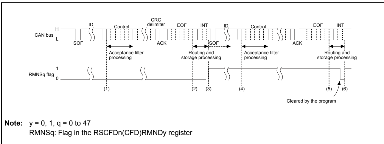
Figure 23.24 Receive Buffer Reception Timing Chart
