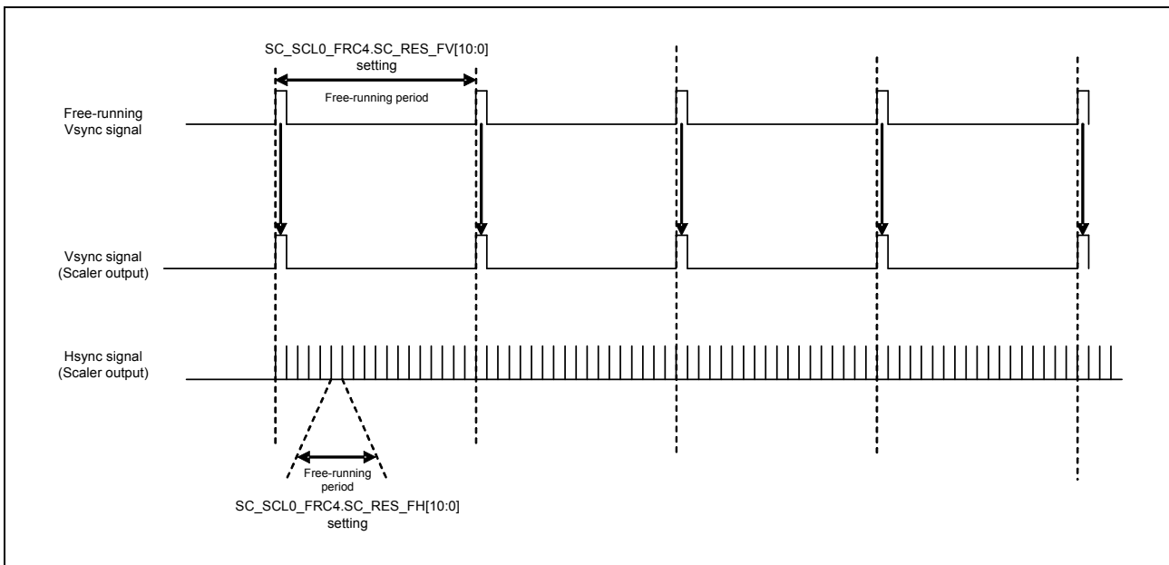
Figure 38.6 Free Running Vsync Timing
