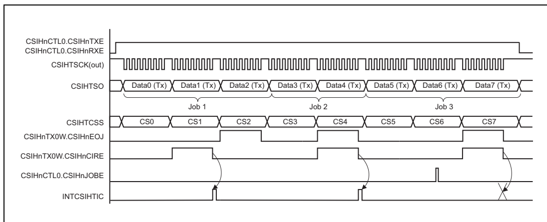
Figure 19.6 Generation of INTCSIHTIC in Job Mode
