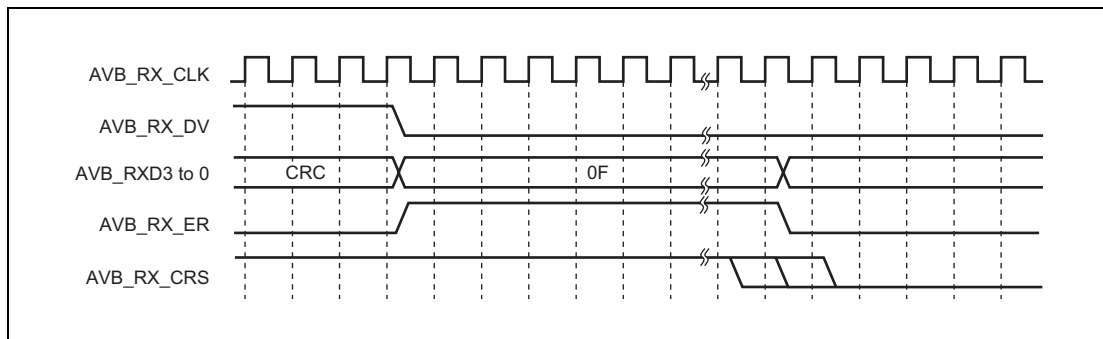
Figure 24.70 MII Fame Receive Timing (with Carrier Extension)
