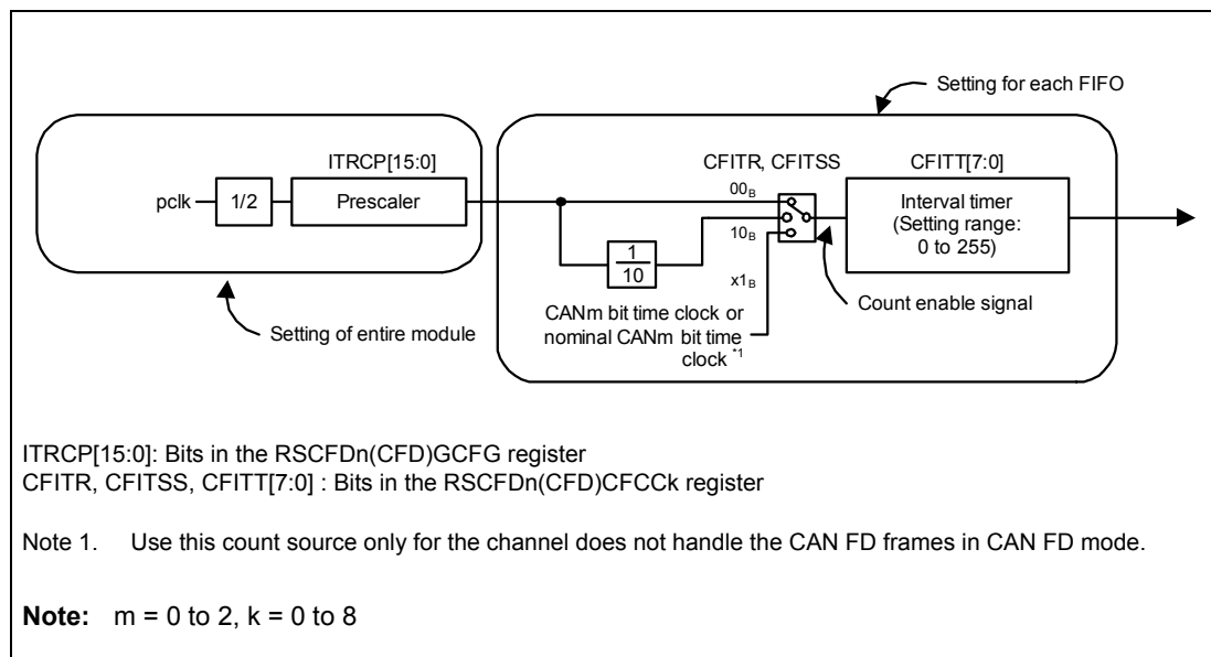
Figure 23.10 Interval Timer Block Diagram
