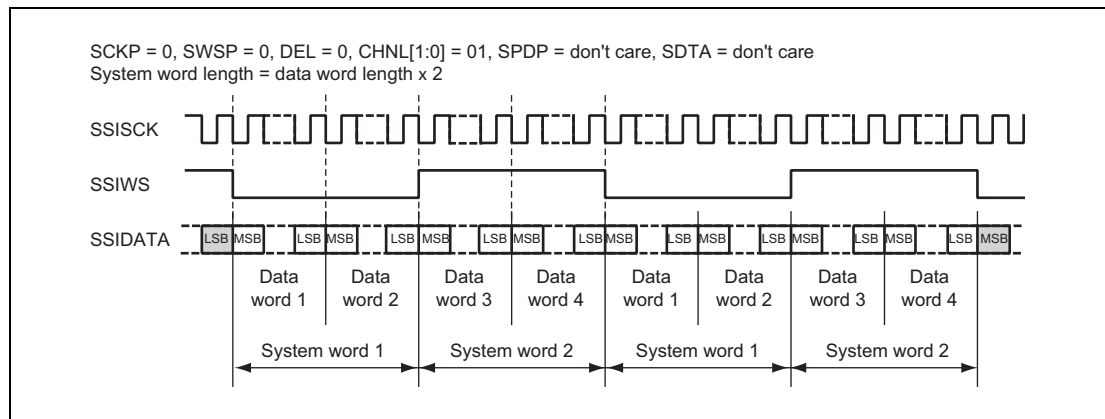
Figure 35.6 Multi-Channel Format (4 Channels Without Padding)
