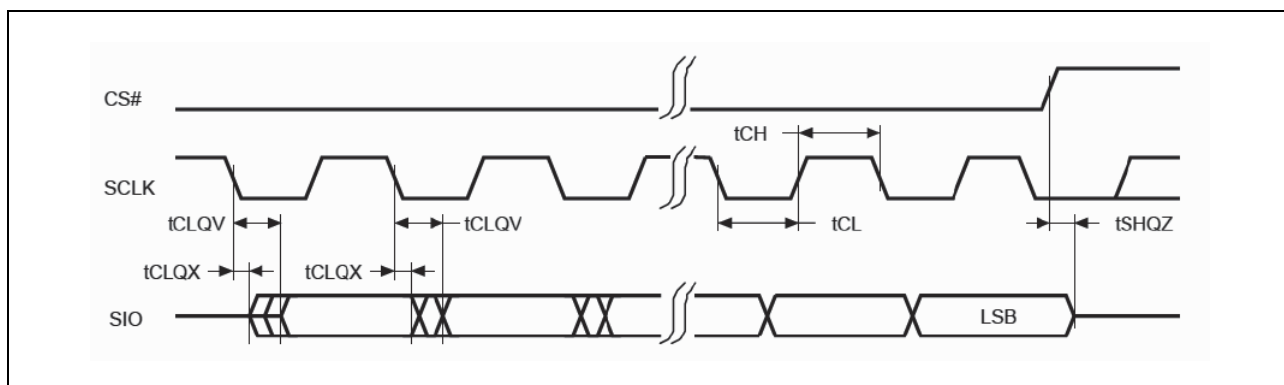
Figure 57.1 STR Read Sequence (Flash Only)
