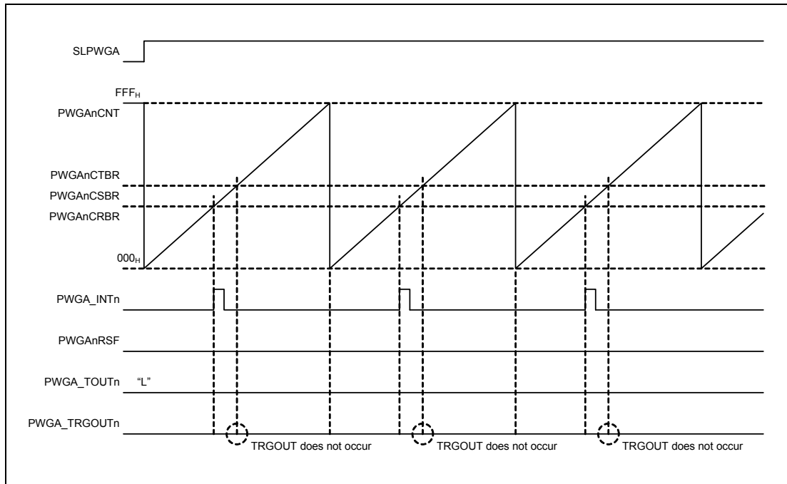
Figure 32.8 PWGA_TOUTn = 0% Output Waveform
