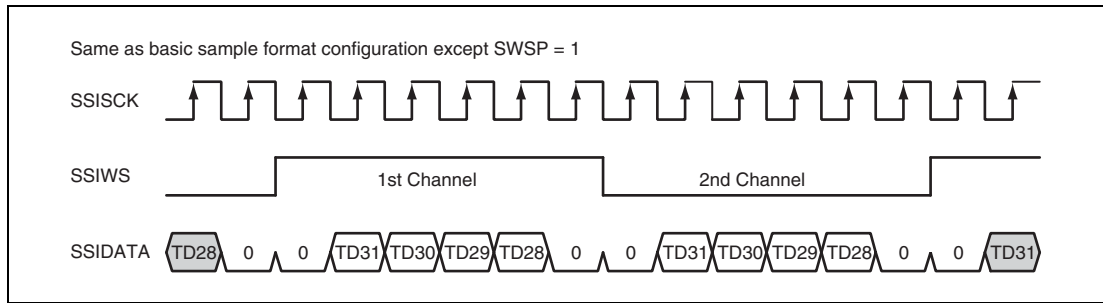
Figure 35.11 Inverted Word Select
