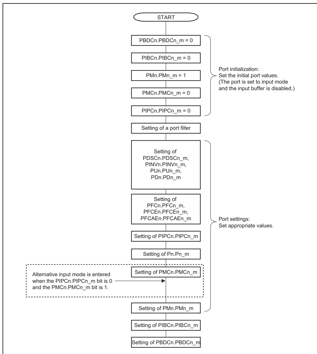
Figure 2.9 Example of Port Configuration Flow (batch setting)
