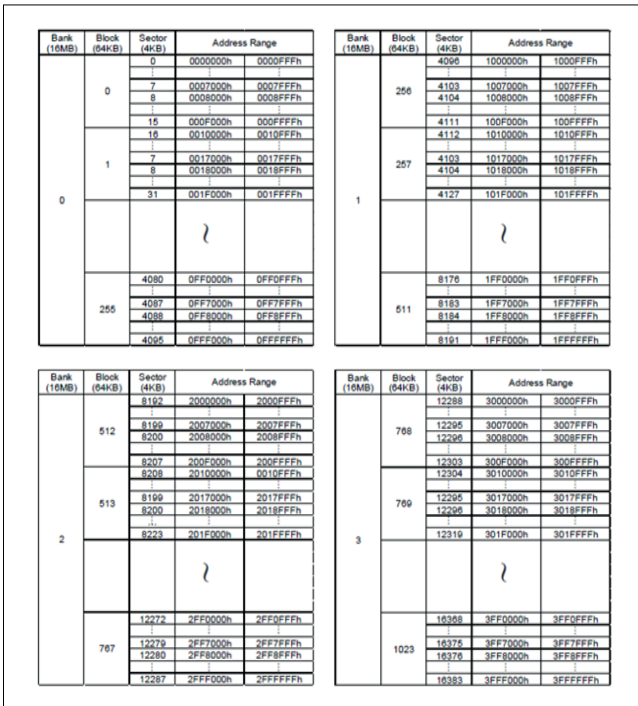
Figure 57.4 MX25LW51245G-Automotive memory organization
