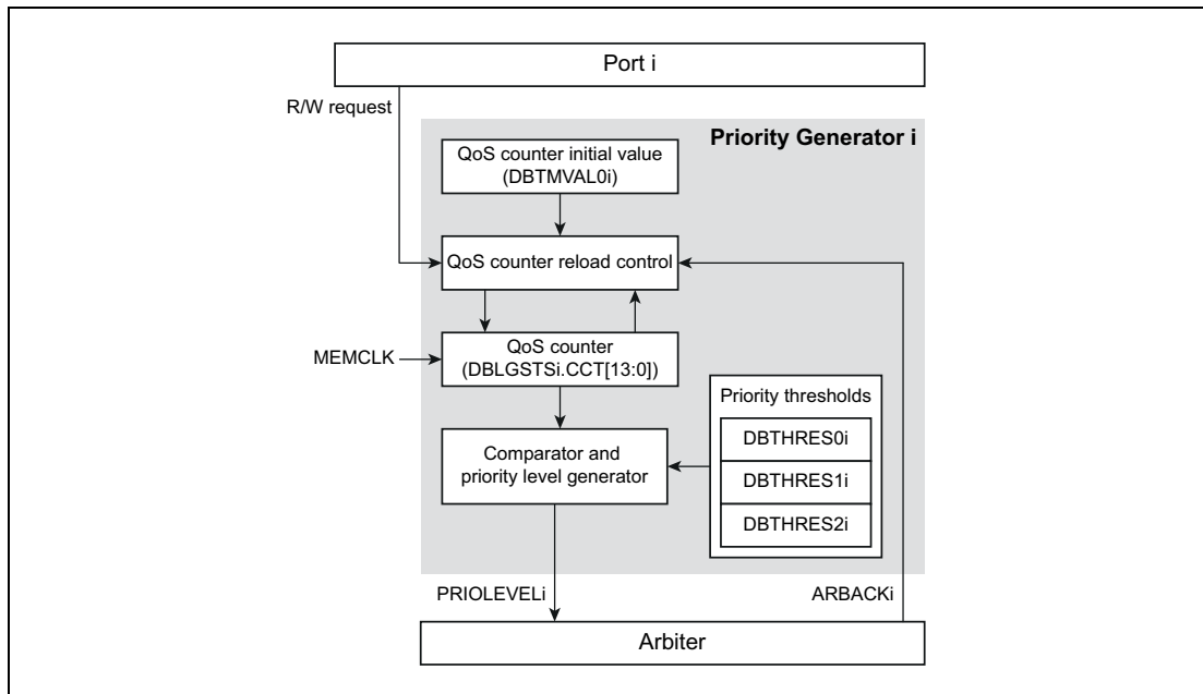
Figure 16.2 Dynamic Priority Generator block diagram
