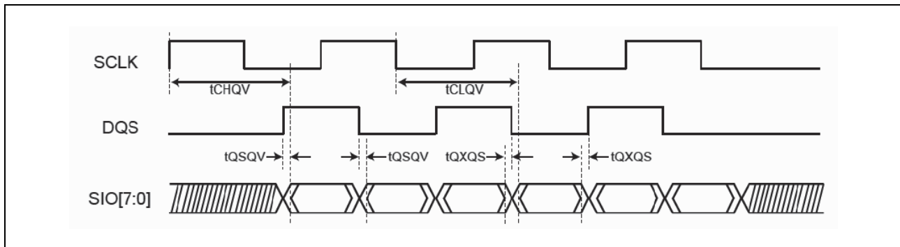
Figure 57.2 DTR Read Sequence (Flash/RAM)
