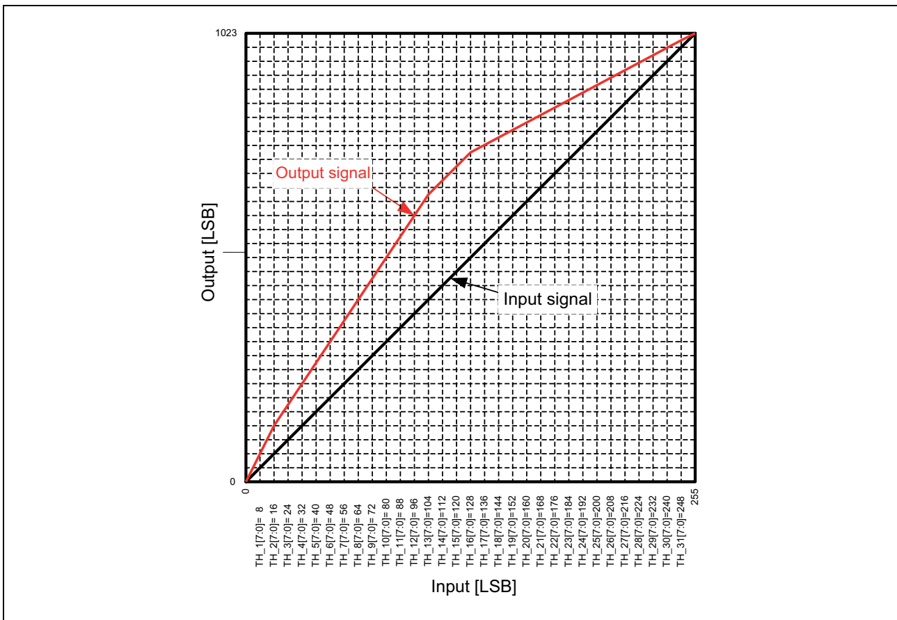
Figure 38.62 Example of Input-Output Characteristics of Gamma Correction
