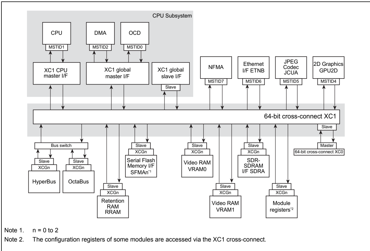
Figure 14.17 D1M1A cross-connect XC1
