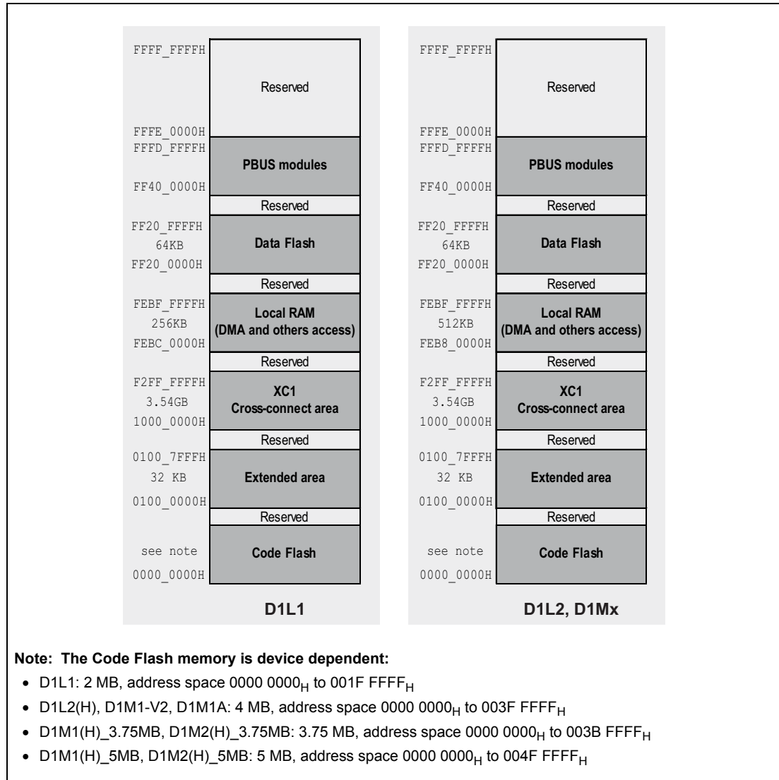
Figure 5.2 DMA address map
