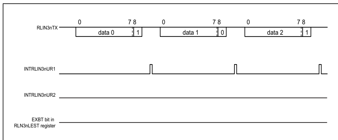
Figure 20.23 Expansion Bit Reception Example (LSB First)
