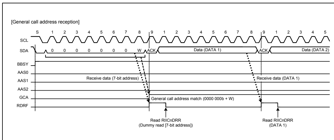
Figure 21.27 Timing of GCA Flag Setting during Reception of General Call Address
