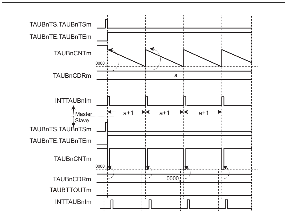
Figure 29.80 TAUBnCDRm (slave) = 0000 H , Positive Logic (TAUBnTOL.TAUBnTOLm (slave) = 0)
