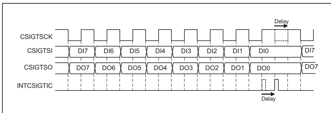
Figure 18.2 Interrupt Delay Function (CSIGNCTL1.CSIGNSIT = 1)
