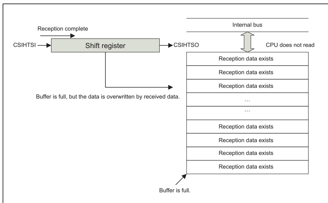
Figure 19.42 Overrun Error Detection in FIFO Mode (FIFO Full)
