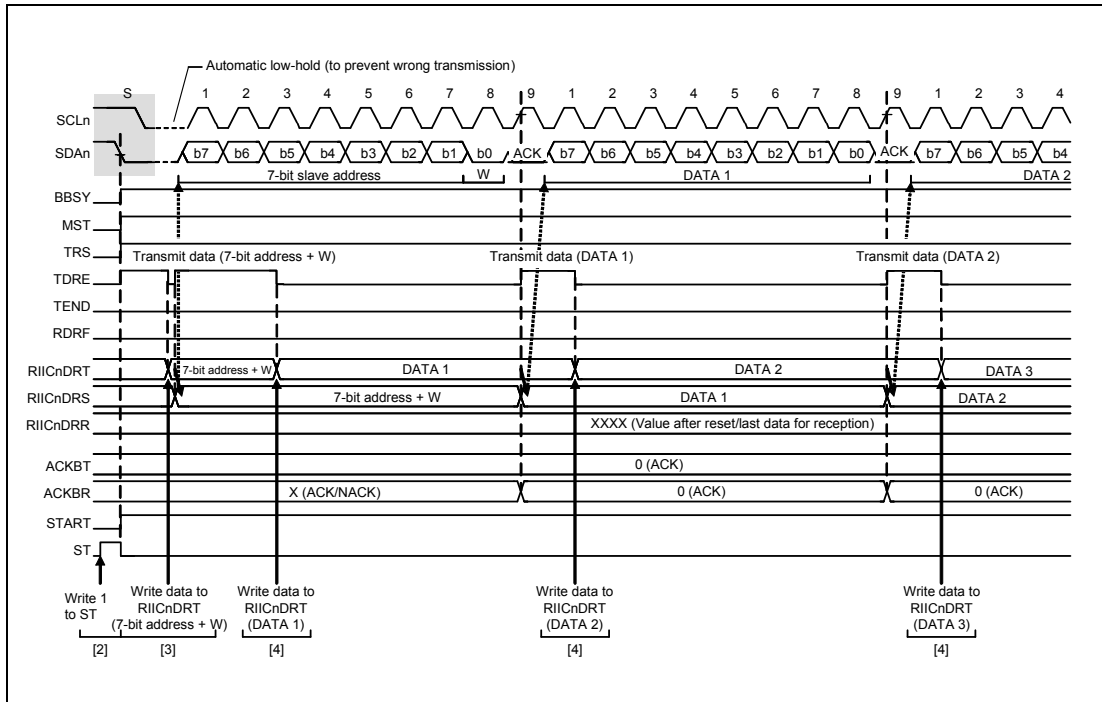
Figure 21.7 Master Transmit Operation Timing (1) (7-Bit Address Format)
