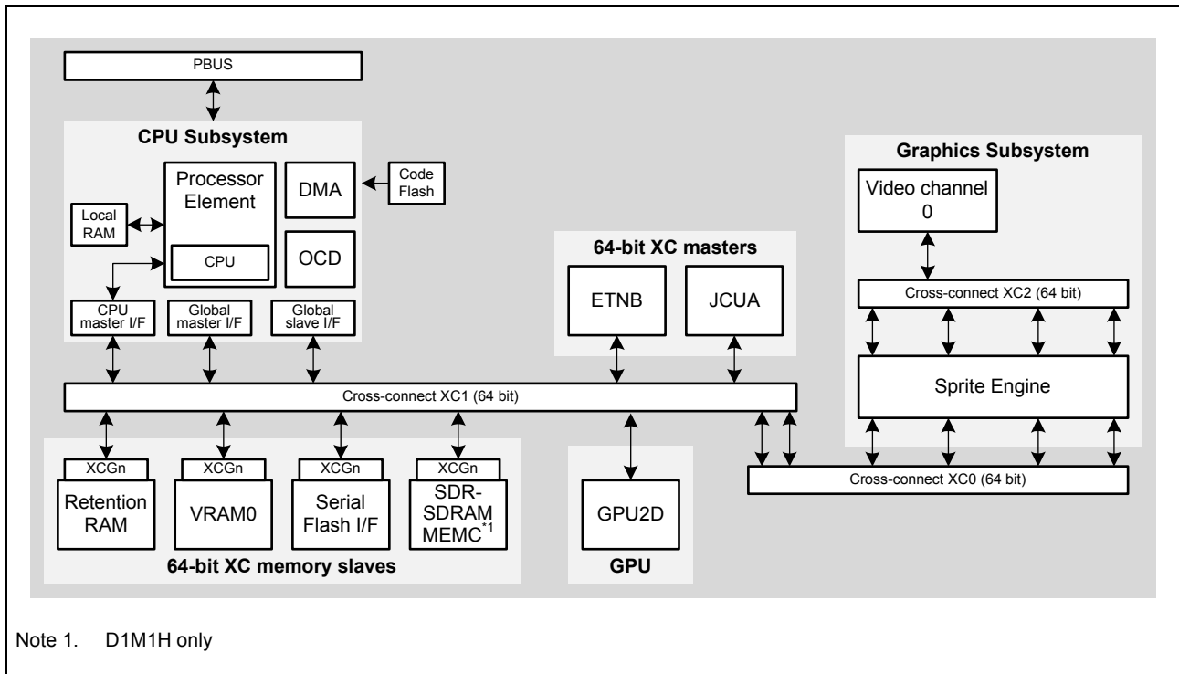
Figure 14.7 D1M1(H) bus architecture overview
