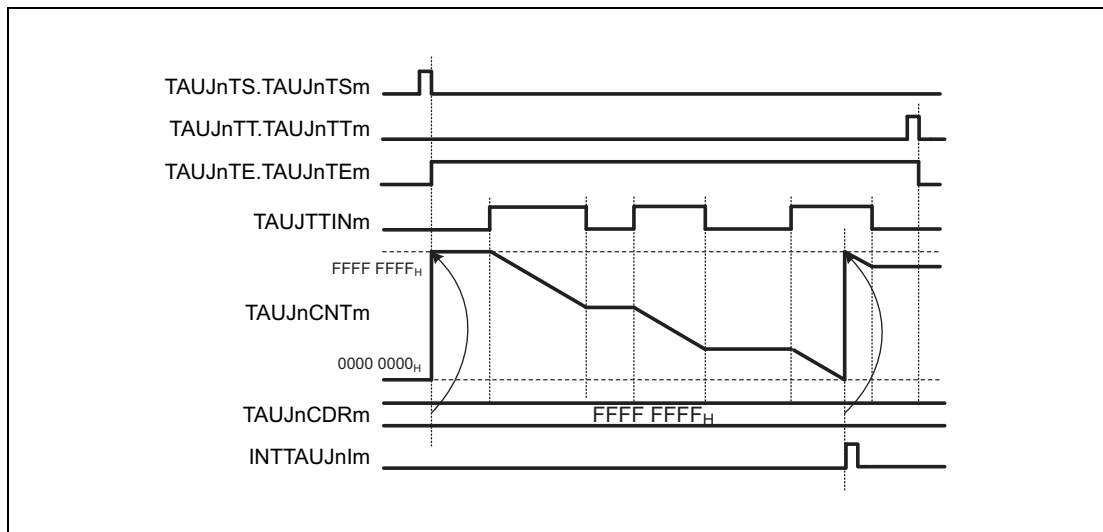
Figure 30.42 General Timing Diagram For Overflow Interrupt Output Function (during TAUJTTINm Input Period Count Detection)
