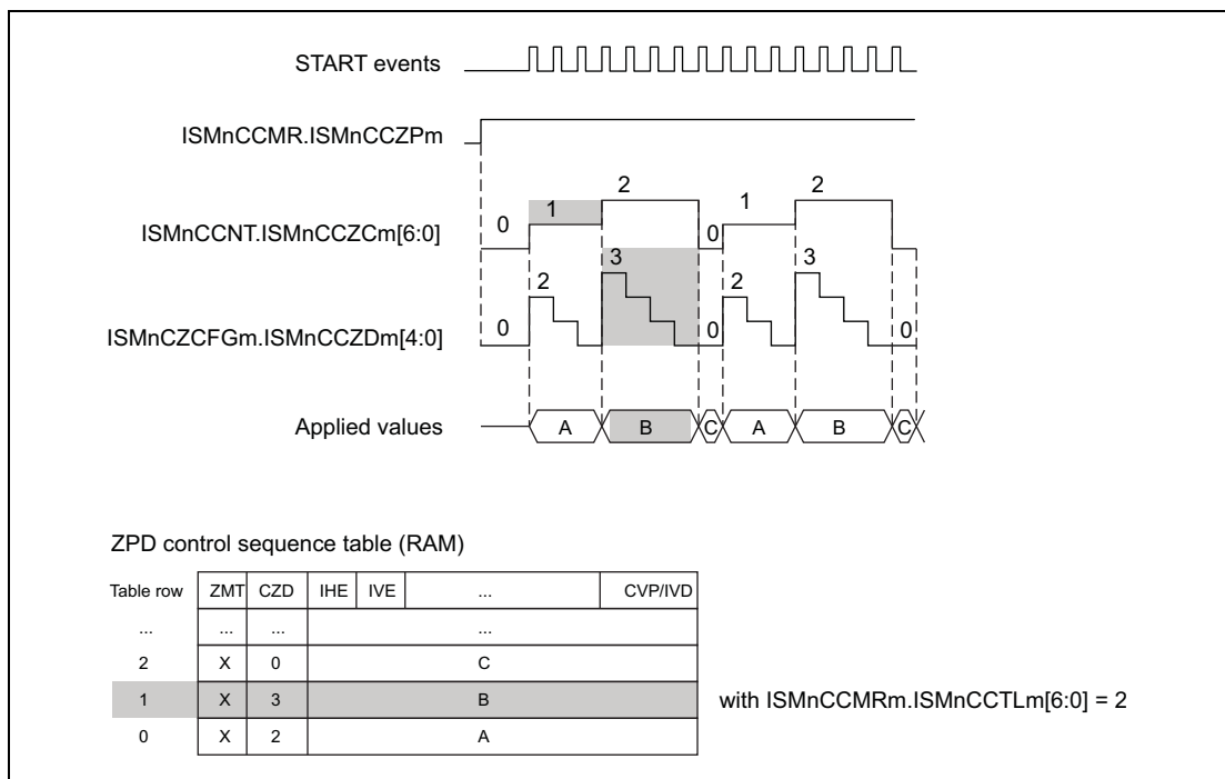
Figure 46.14 Processing of ZPD table
