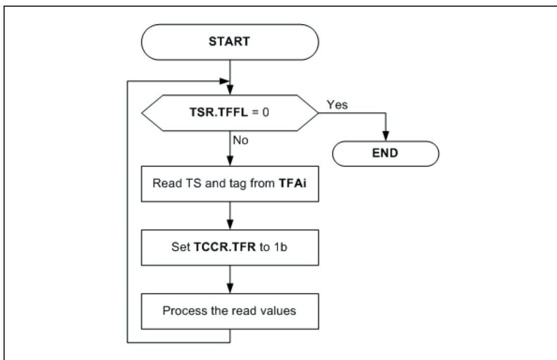
Figure 24.42 Flow of Transmission Time Stamping
