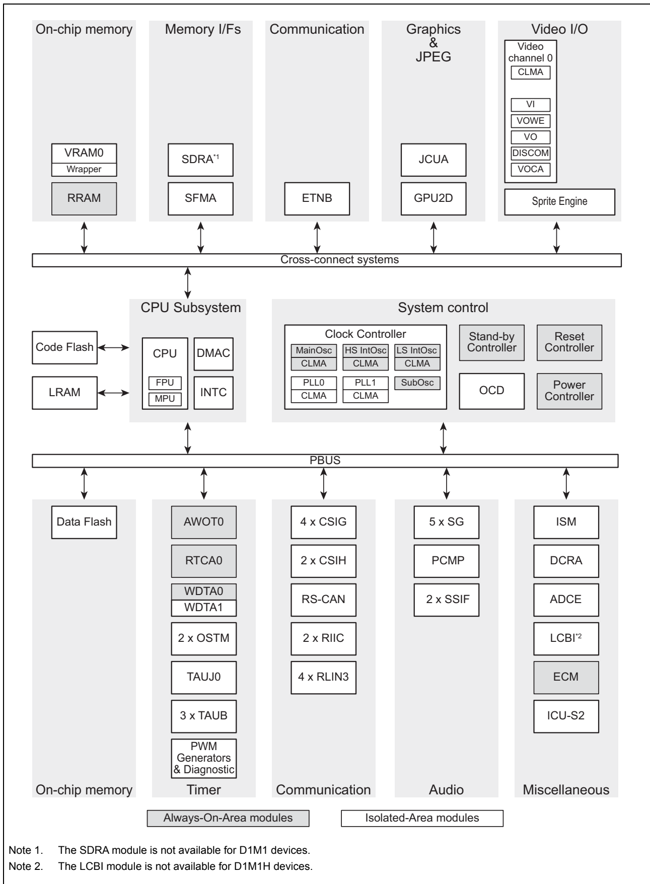
Figure 1.3 D1M1(H) block diagram
