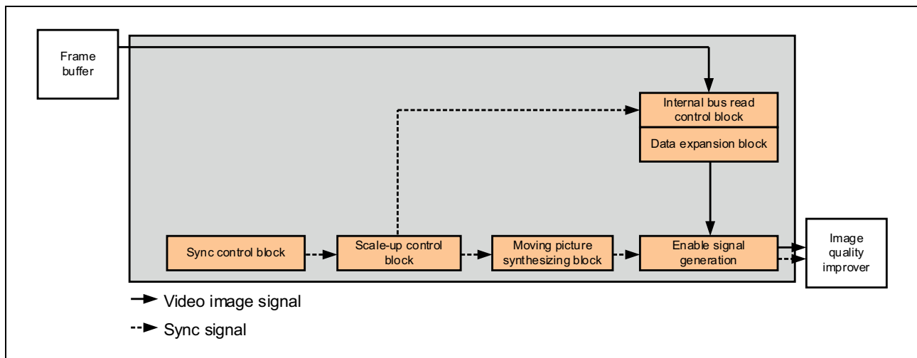
Figure 38.40 Signal Paths for Graphics Display
