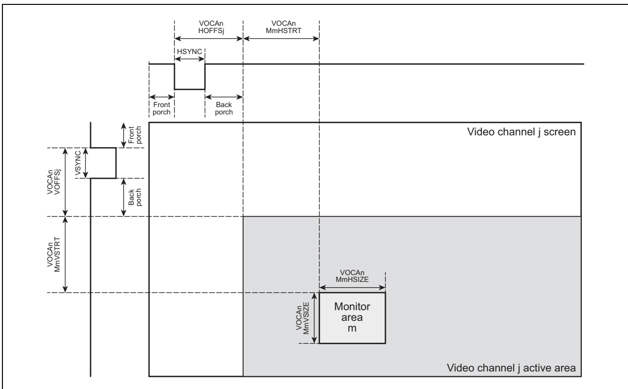
Figure 40.4 Monitor area definition with active low HSYNC and VSYNC
