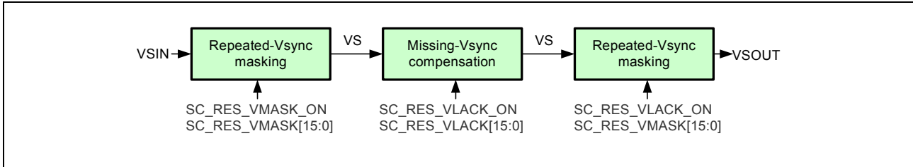
Figure 38.28 Repeated-Vsync Masking and Missing-Vsync Compensation
