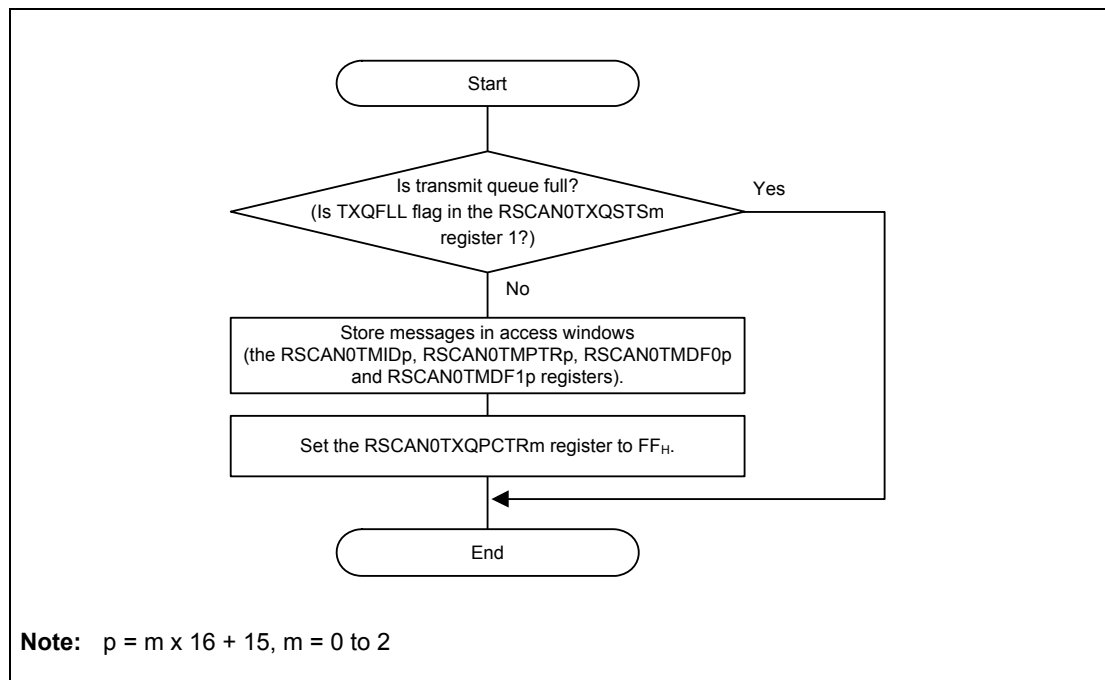
Figure 22.32 Procedure for Transmission from the Transmit Queue
