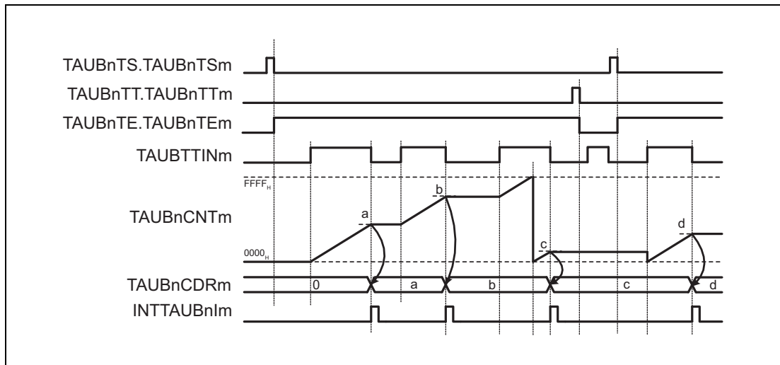
Figure 29.67 Operation Stop and Restart, (TAUBnCMURm.TAUBnTIS[1:0] = 11 B )
