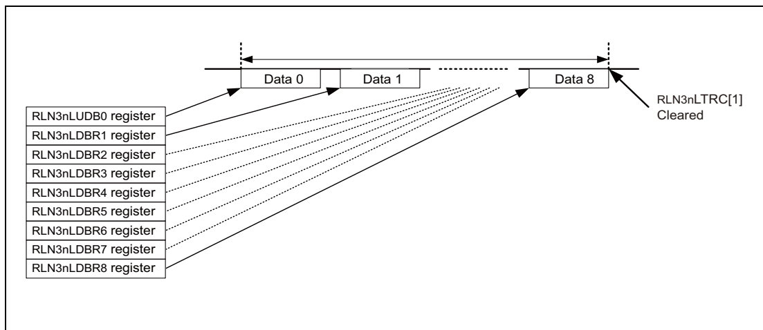
Figure 20.17 UART Buffer and Transmission Processing (for 9-Byte Transmission)
