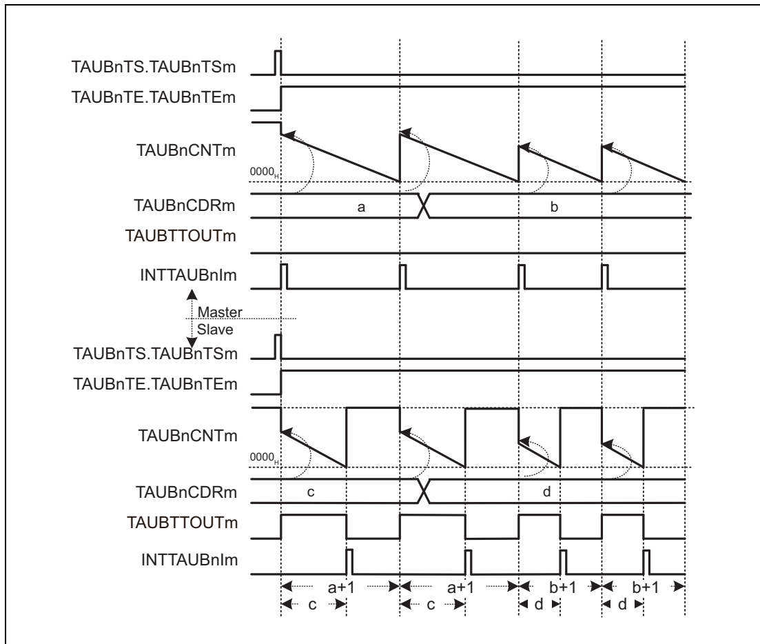
Figure 29.79 General Timing Diagram for PWM Output Function
