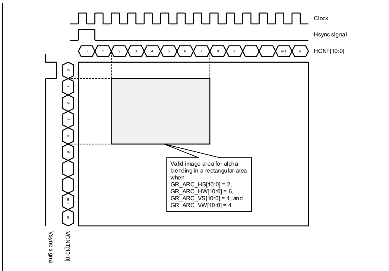
Figure 38.52 Rectangular Area Setting for Alpha Blending
