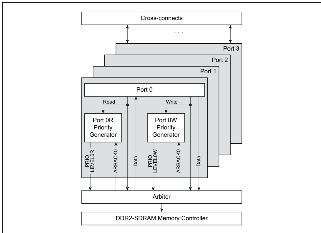
Figure 16.1 Priority Generators connection
