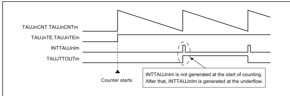
Figure 30.9 INTTAUJnIm Generation Timing (when TAUJnCMORm.TAUJnMD0 = 0)
