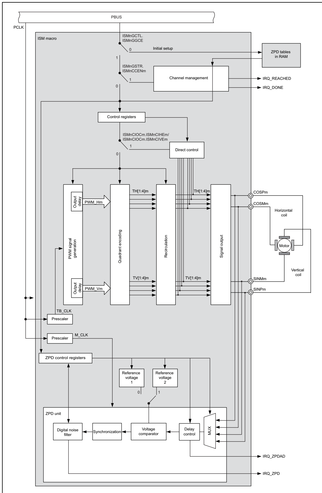
Figure 46.2 Block diagram of zero point detection of channel m
