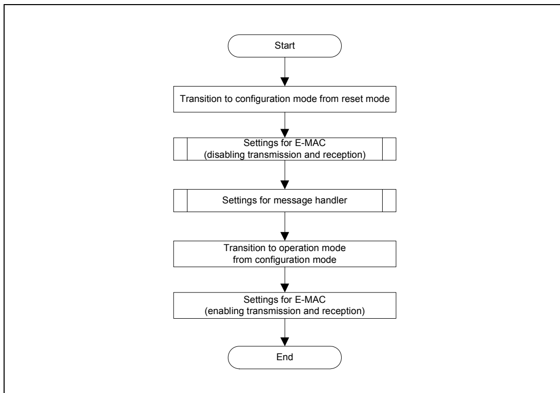
Figure 24.8 Outline of the Initialization Procedure
