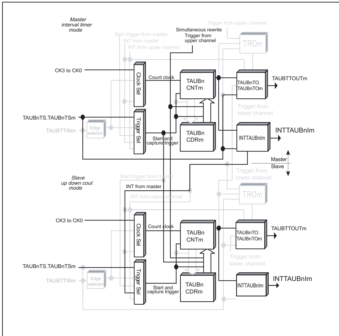
Figure 29.98 Block Diagram for Triangle PWM Output Function
