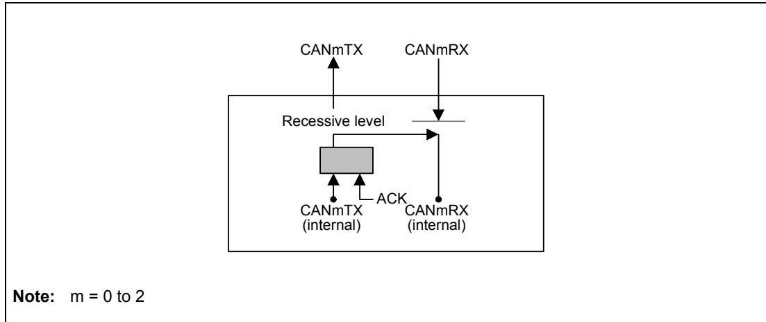
Figure 23.14 Connection when Self-Test Mode 1 is Selected
