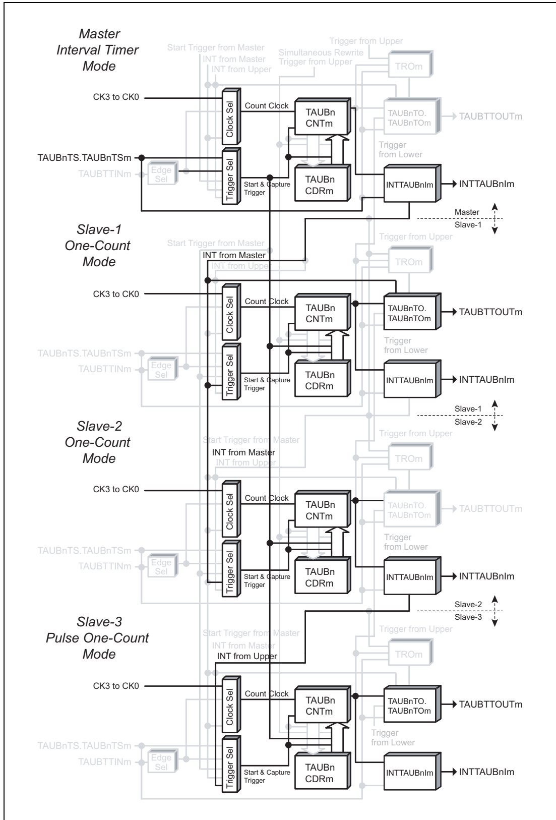
Figure 29.92 Block Diagram for Delay Pulse Output Function
