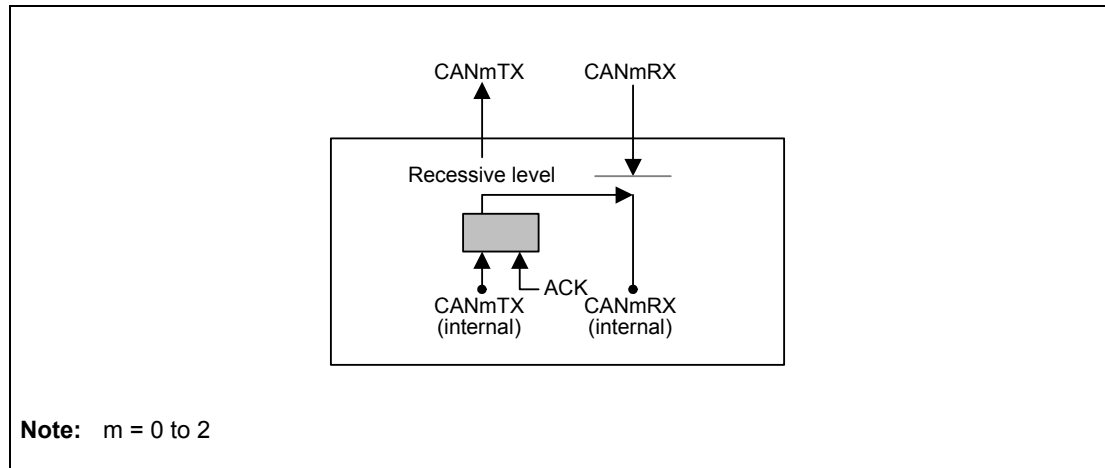
Figure 22.14 Connection when Self-Test Mode 1 is Selected
