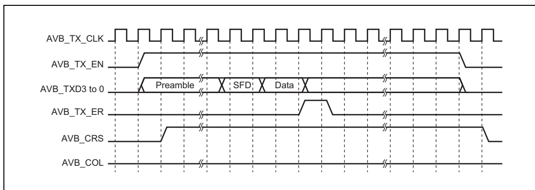
Figure 24.65 MII Frame Transmit Timing (Transmit Error)
