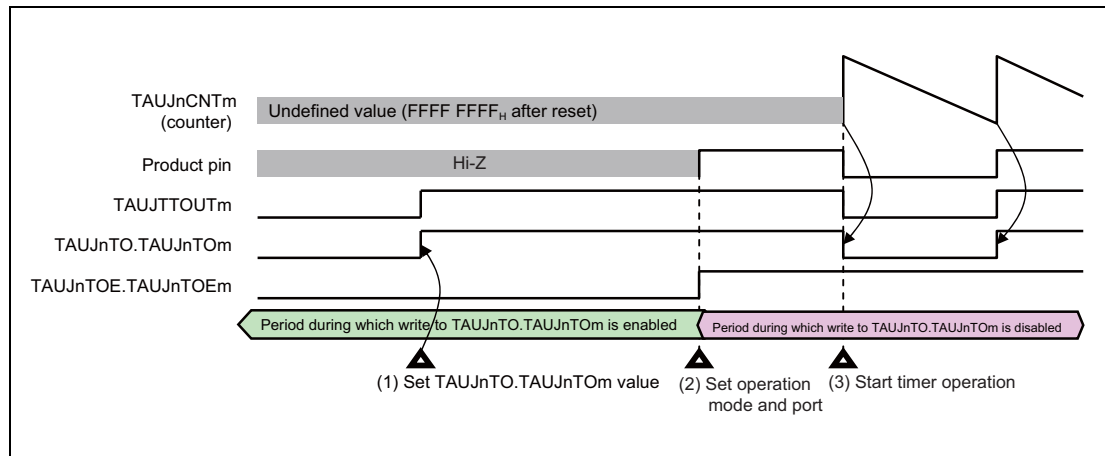
Figure 30.6 General Procedure for Specifying a TAUJTOUT m Channel Output Mode
