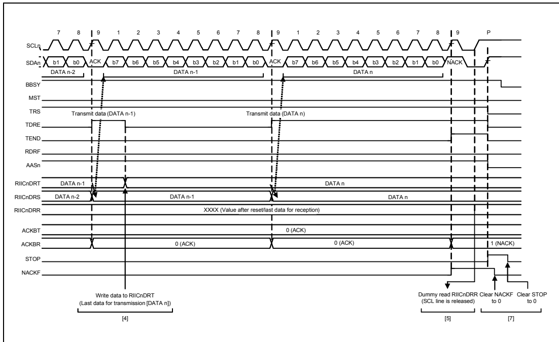
Figure 21.17 Slave Transmit Operation Timing (2)
