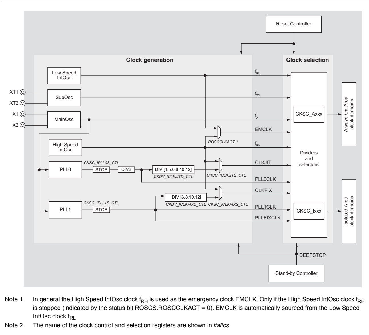
Figure 12.4 D1M1-V2 Clock Controller block diagram
