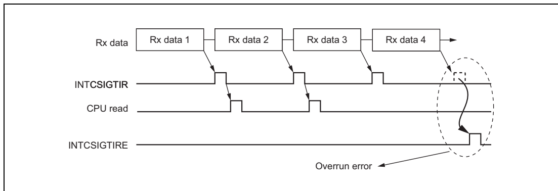
Figure 18.25 Overrun Error Detection - Example
