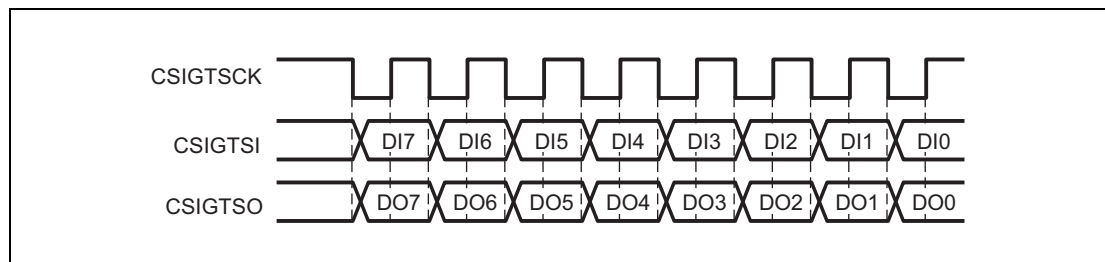
Figure 18.6 Transmission/Reception in Master Mode
