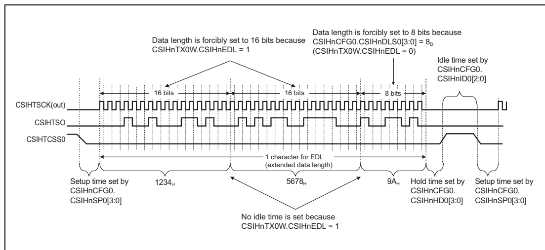
Figure 19.25 EDL Timing Diagram
