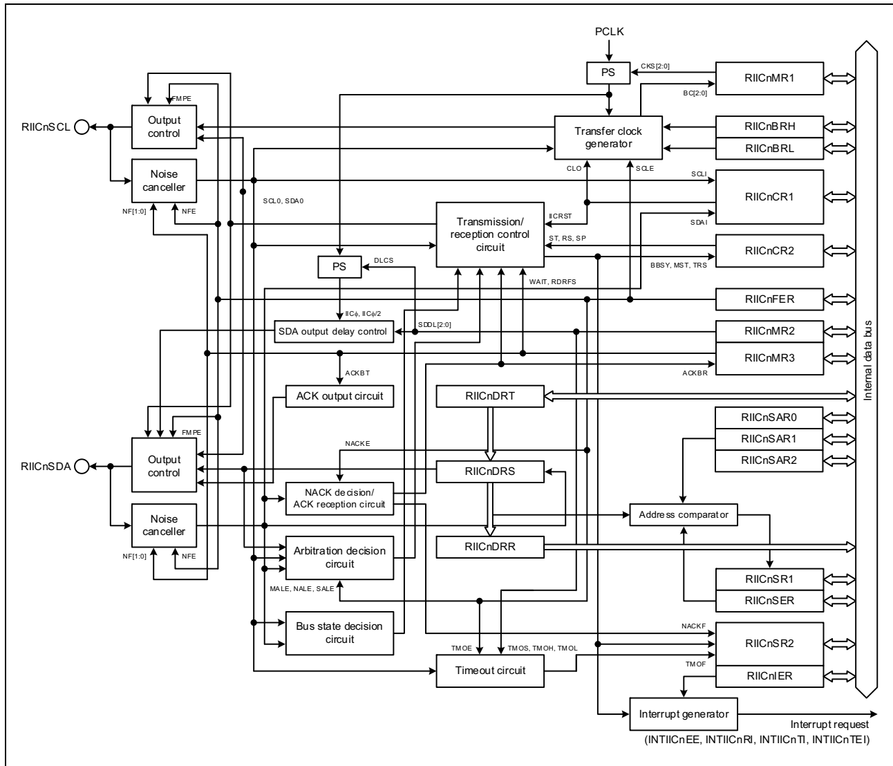
Figure 21.1 Block Diagram of RIIC
