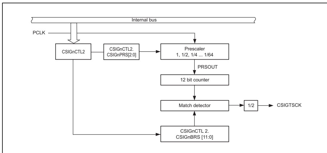
Figure 18.10 BRG Block Diagram
