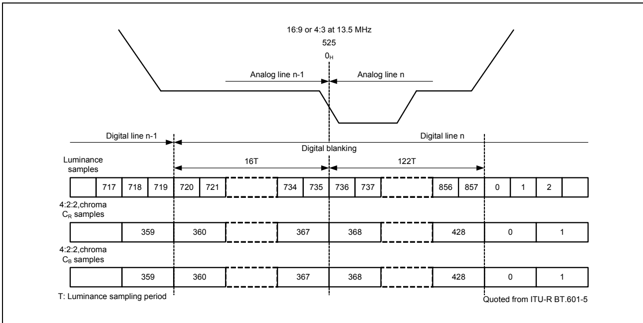
Figure 38.10 BT601 Horizontal Timing (525 Lines/59.94 Hz)
