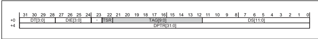
Figure 24.33 Configuration of Descriptor for a Transmitted Frame
