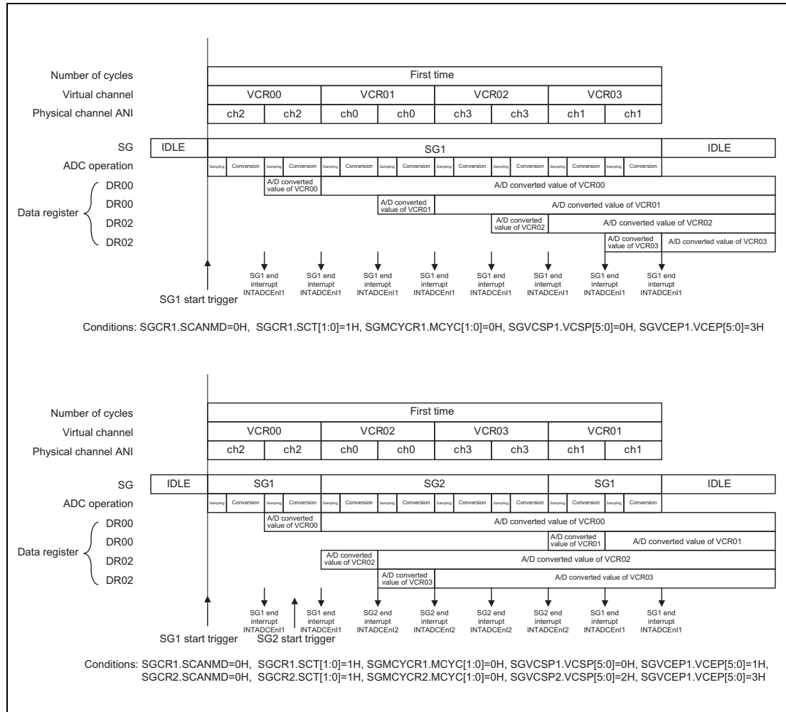
Figure 45.10 Example of Channel Repeat Operation 1
