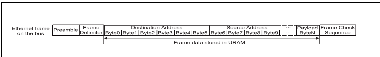
Figure 24.2 Data for Reception in an Ethernet Frame
