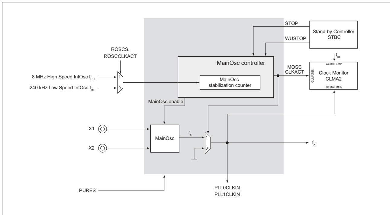
Figure 12.11 Main Oscillator (MainOsc)
