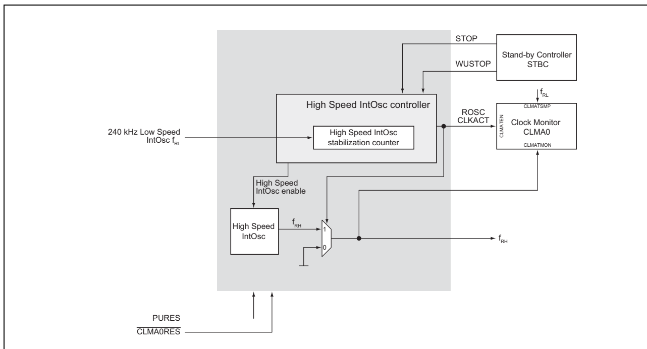
Figure 12.13 High Speed Internal Oscillator (High Speed IntOsc)
