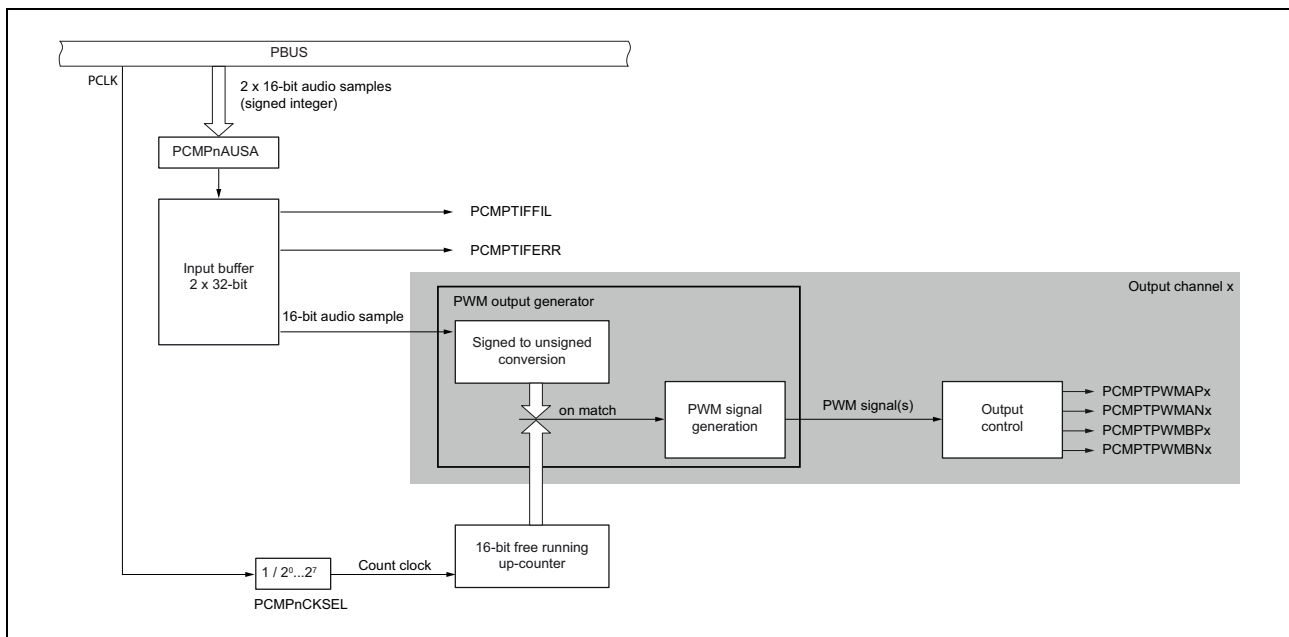
Figure 34.1 Functional blocks of the PCM-PWM module
