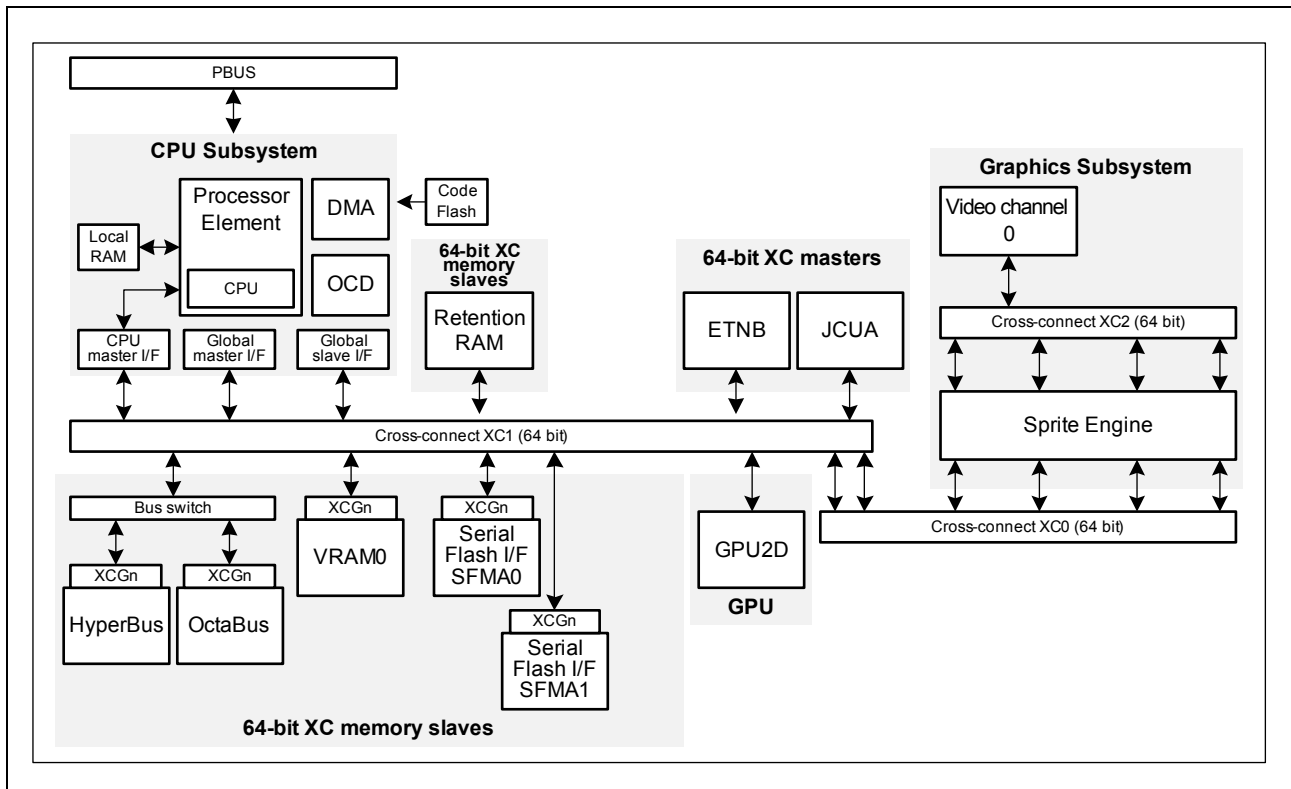
Figure 14.11 D1M1-V2 bus architecture overview
