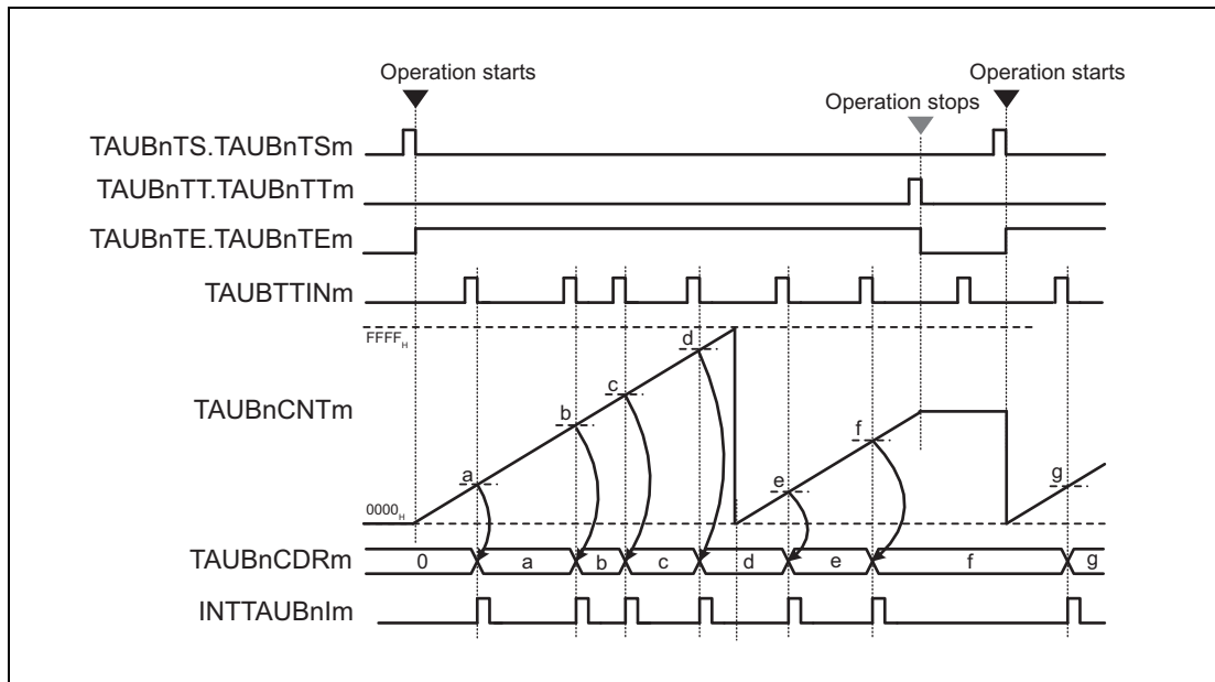
Figure 29.64 Operation Stop and Restart, (TAUBnCMORM.TAUBnMD0 = 0, TAUBnCMURm.TAUBnTIS[1:0] = 00 B )
