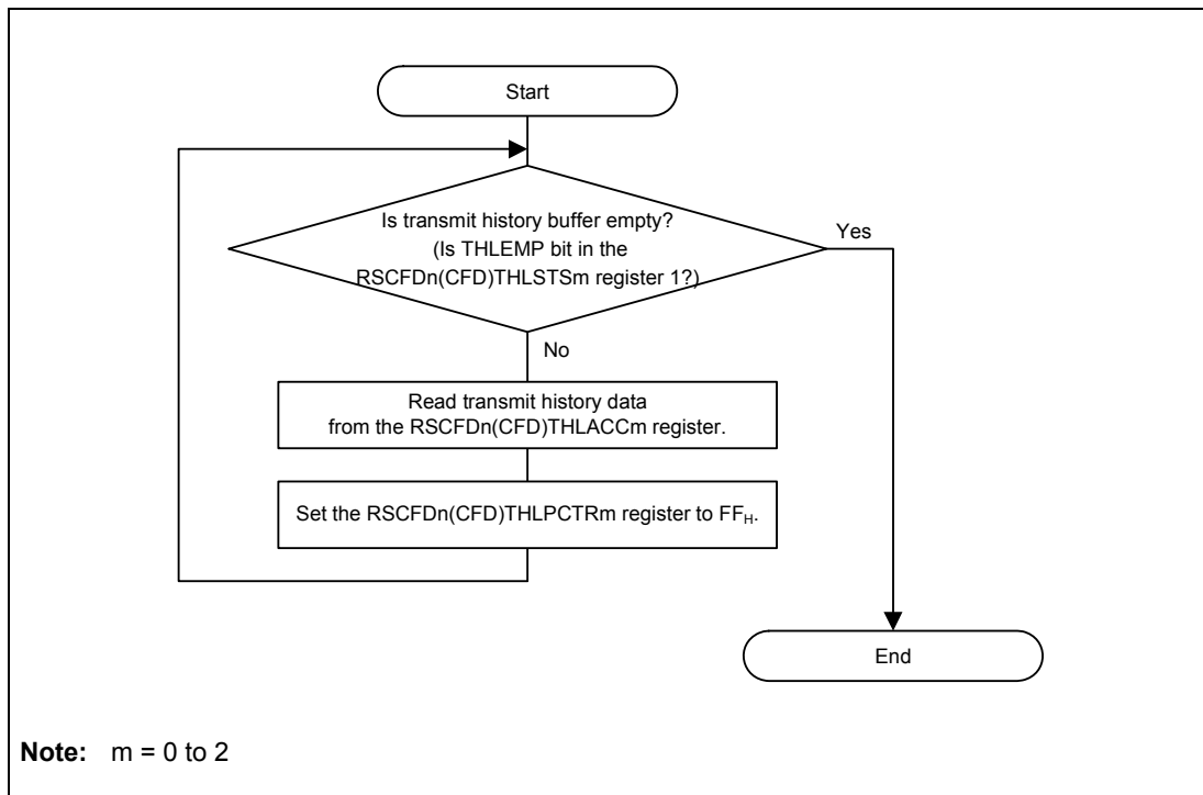
Figure 23.34 Transmit History Buffer Reading Procedure
