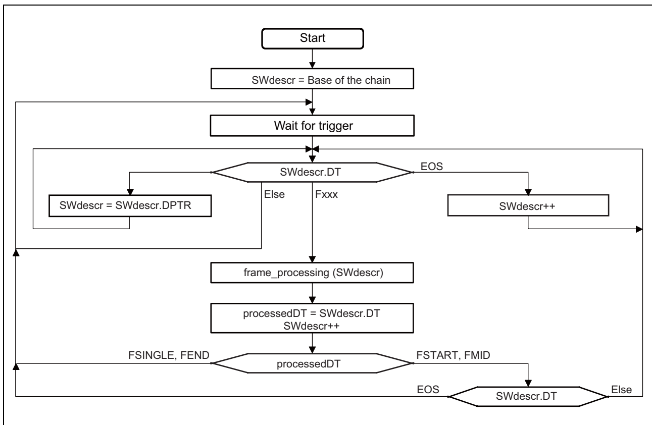
Figure 24.28 Flow of Reception Descriptor Processing (with Write-Back)
