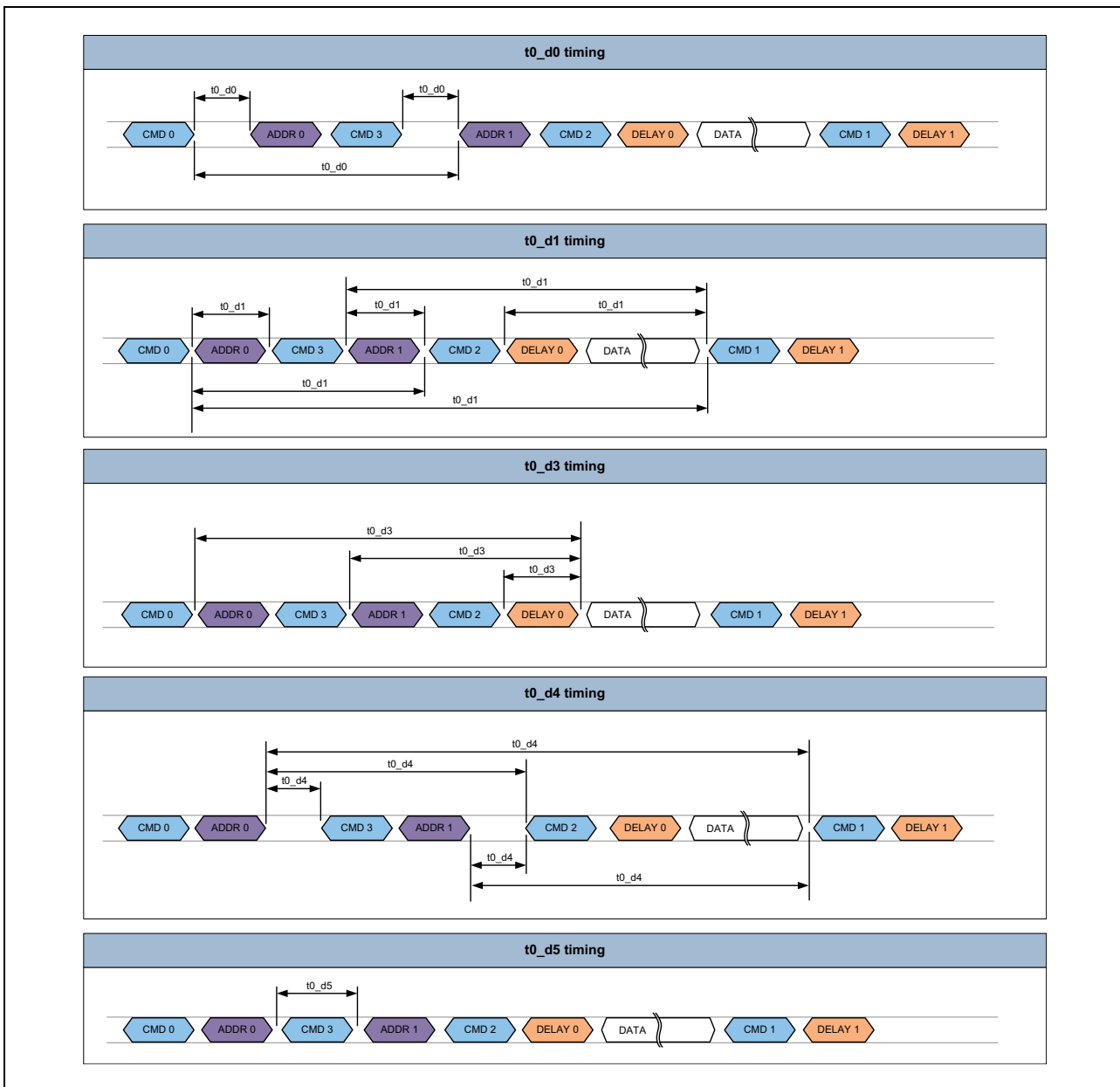
Figure 58.27 Generic Sequence Timing parameters
