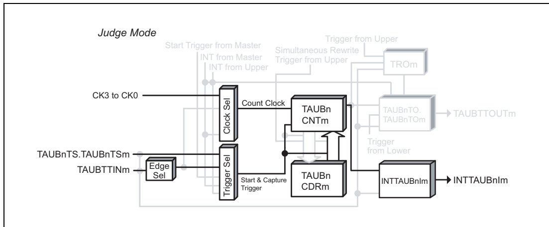
Figure 29.68 Block Diagram for TAUBTTINm Input Pulse Interval Judgment Function
