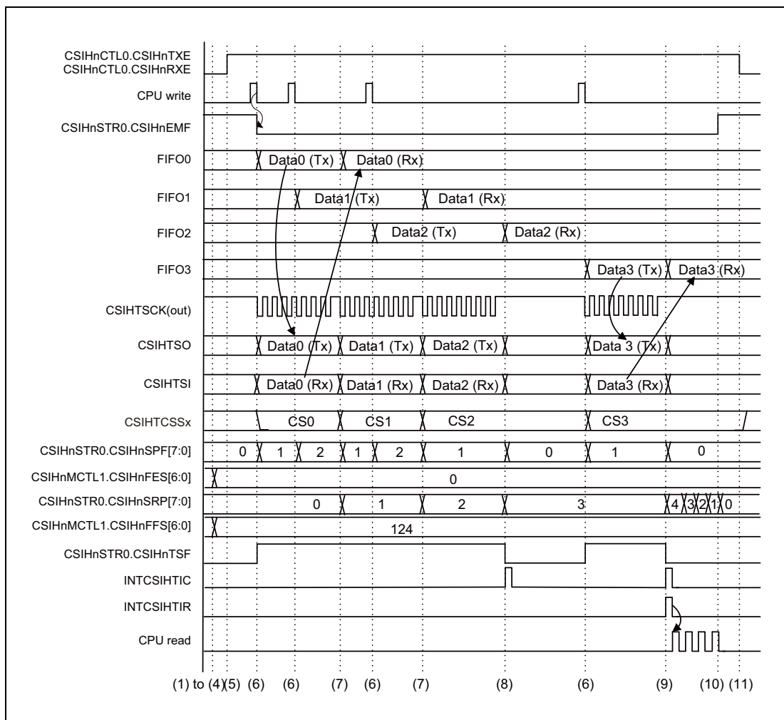
Figure 19.57 Master in FIFO Mode, CSIHnCTL1.CSIHnJE = 0
