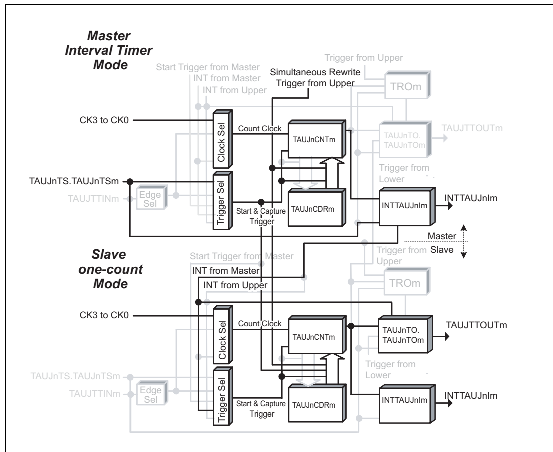
Figure 30.43 Block Diagram for PWM Output Function
