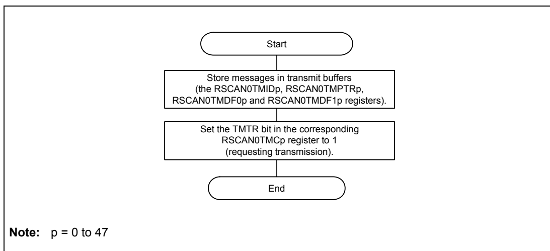
Figure 22.26 Procedure for Transmission from Transmit Buffers
