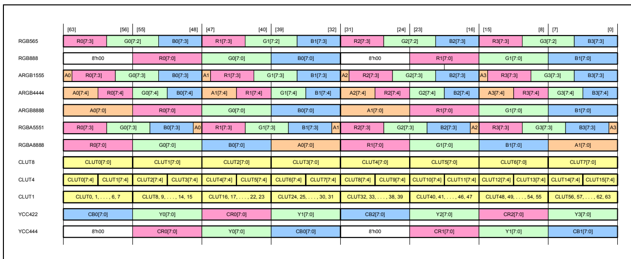
Figure 38.46 Data Arrangement with Endian Control Disabled (GR_RDSWA = 000)
