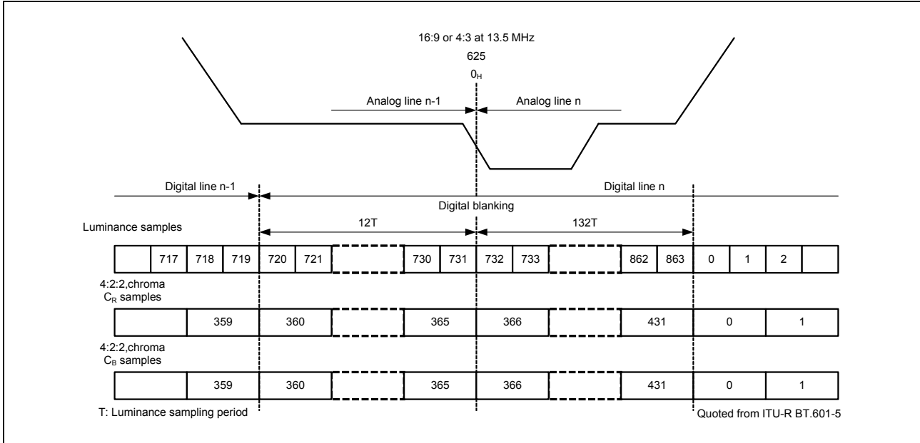
Figure 38.9 BT601 Horizontal Timing (625 Lines/50.00 Hz)
