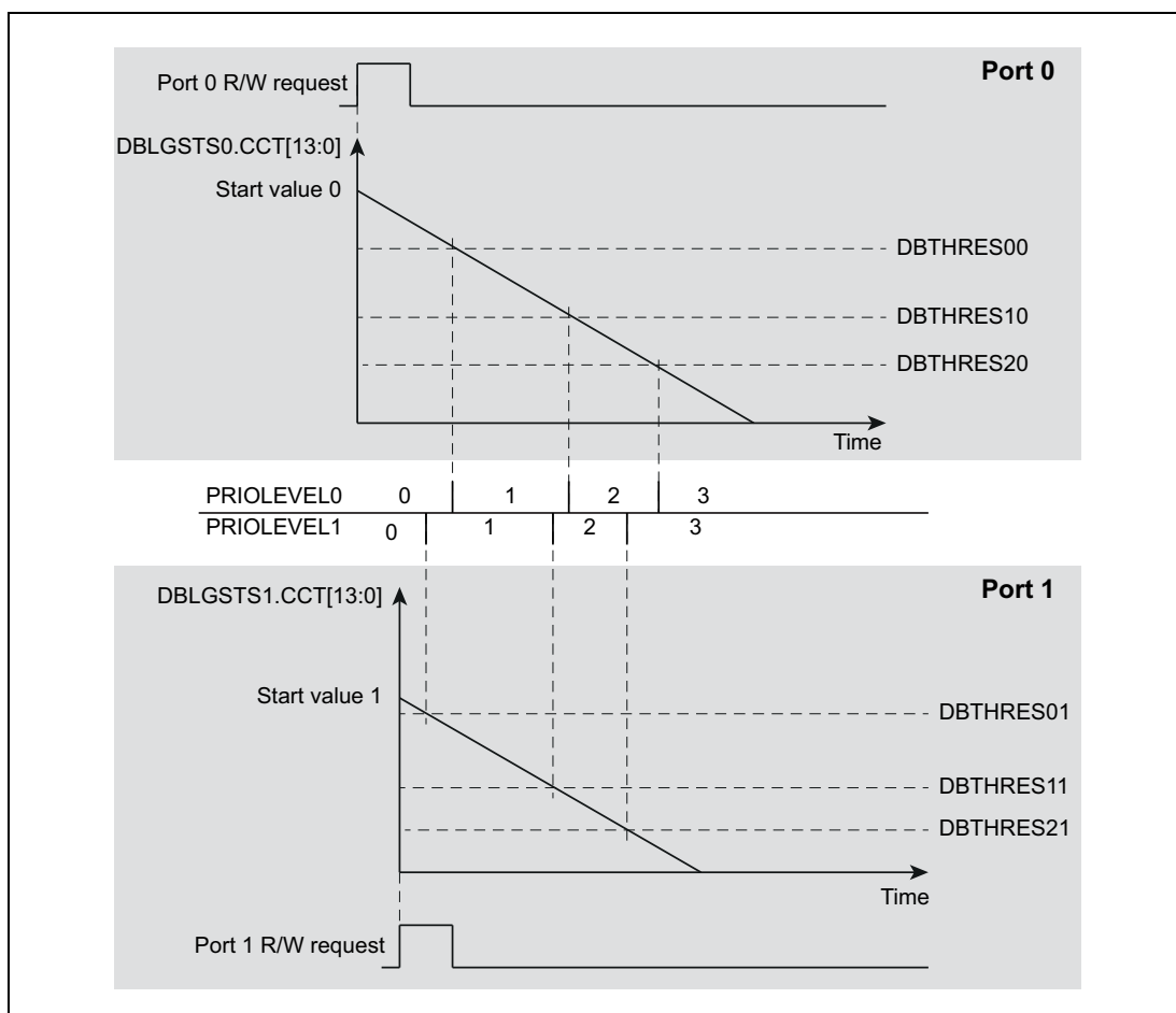
Figure 16.3 Dynamic priority control principle
