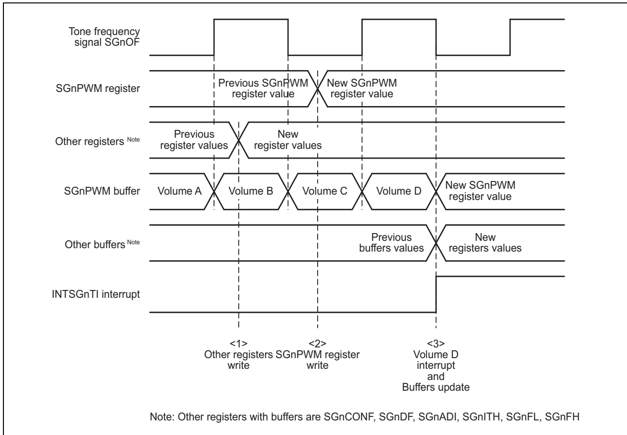
Figure 33.6 Update of buffer values by INTSGnTI (SGNCONF.SGNBE = 1)
