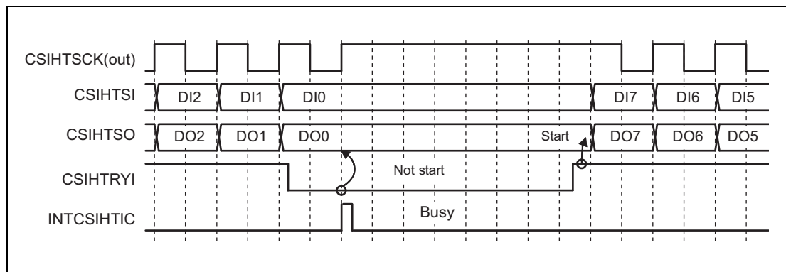
Figure 19.35 Master's Reaction on CSIHTRYI ( CSIHnCFGx.CSIHnDAPx = 1 )
