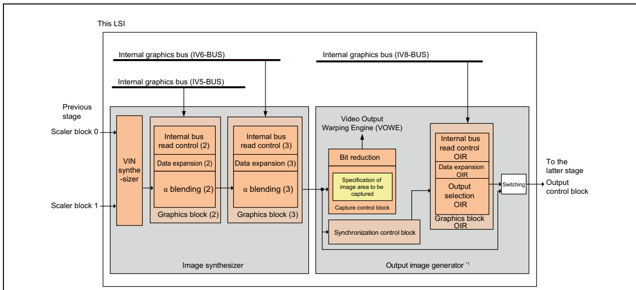
Figure 38.2 Video Display Controller Middle Stage Block Diagram
