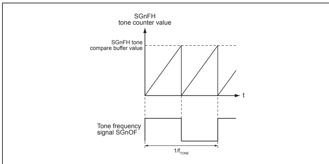
Figure 33.3 Generation of tone frequency
