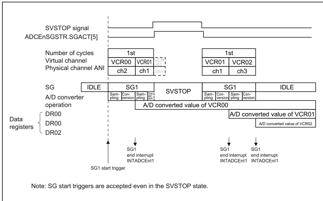
Figure 45.17 Example of SVSTOP Operation (ADCEnADCR.SUSMTD[1:0] = 10 and ADCEnEMU.SVSDIS = 0)
