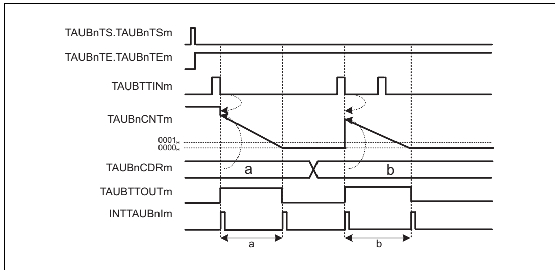
Figure 29.46 General Timing Diagram for One-Pulse Output Function
