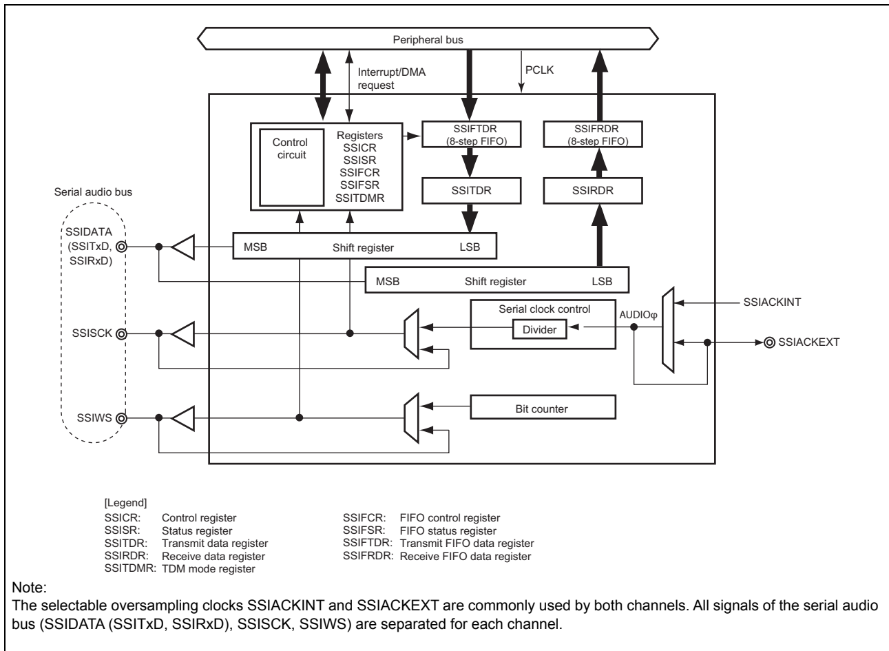
Figure 35.1 Block Diagram of the Serial Sound Interface
