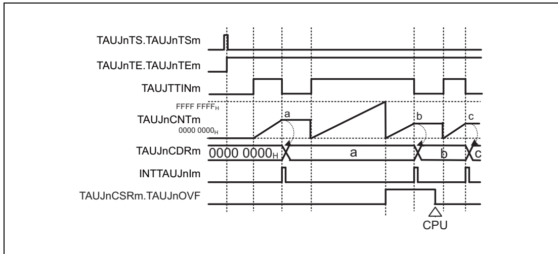
Figure 30.30 \text{TAUJnCMORm.TAUJnCOS}[1:0] = 01_{\text{B}} , \text{TAUJnCMORm.TAUJnMD0} = 0 , \text{TAUJnCMURm.TAUJnTIS}[1:0] = 11_{\text{B}}
