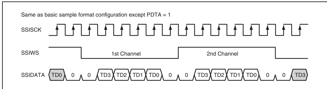
Figure 35.16 Parallel Right-Aligned with Delay
