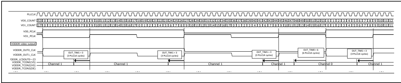
Figure 37.38 VODDR WVGA + WQVGA (50 Hz) Video Output
