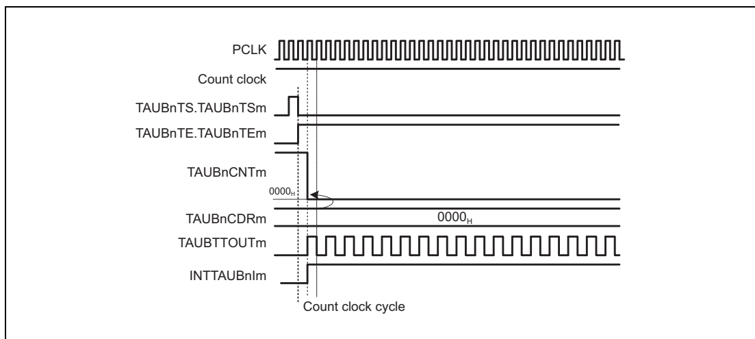
Figure 29.27 TAUBnCDRm = 0000 H , Count Clock = PCLK
