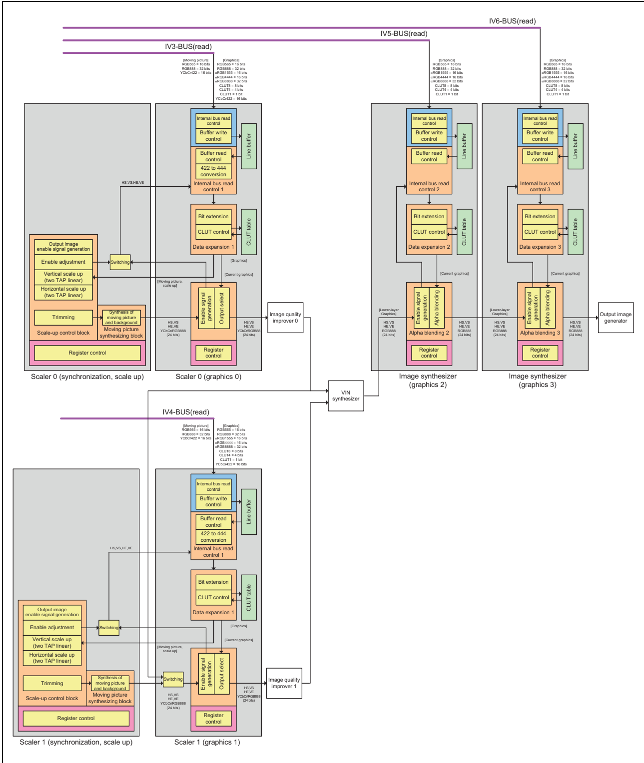
Figure 38.43 Functional Block Diagram of Image Synthesizer
