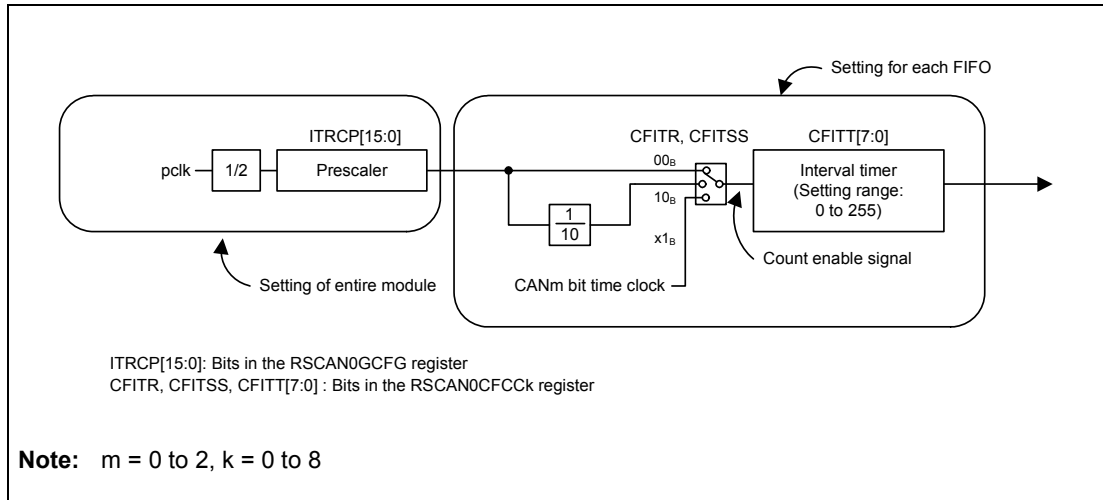
Figure 22.10 Interval Timer Block Diagram
