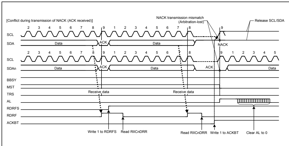
Figure 21.34 Example of Arbitration-Lost Detection during Transmission of NACK (NALE = 1)
