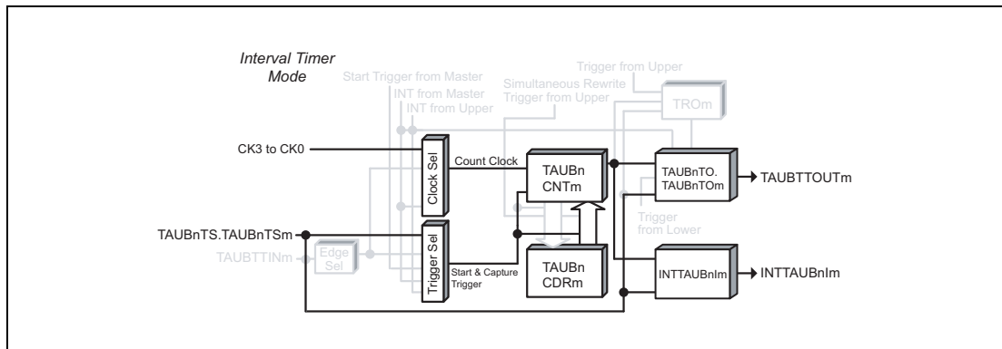
Figure 29.24 Block Diagram for Interval Timer Function
