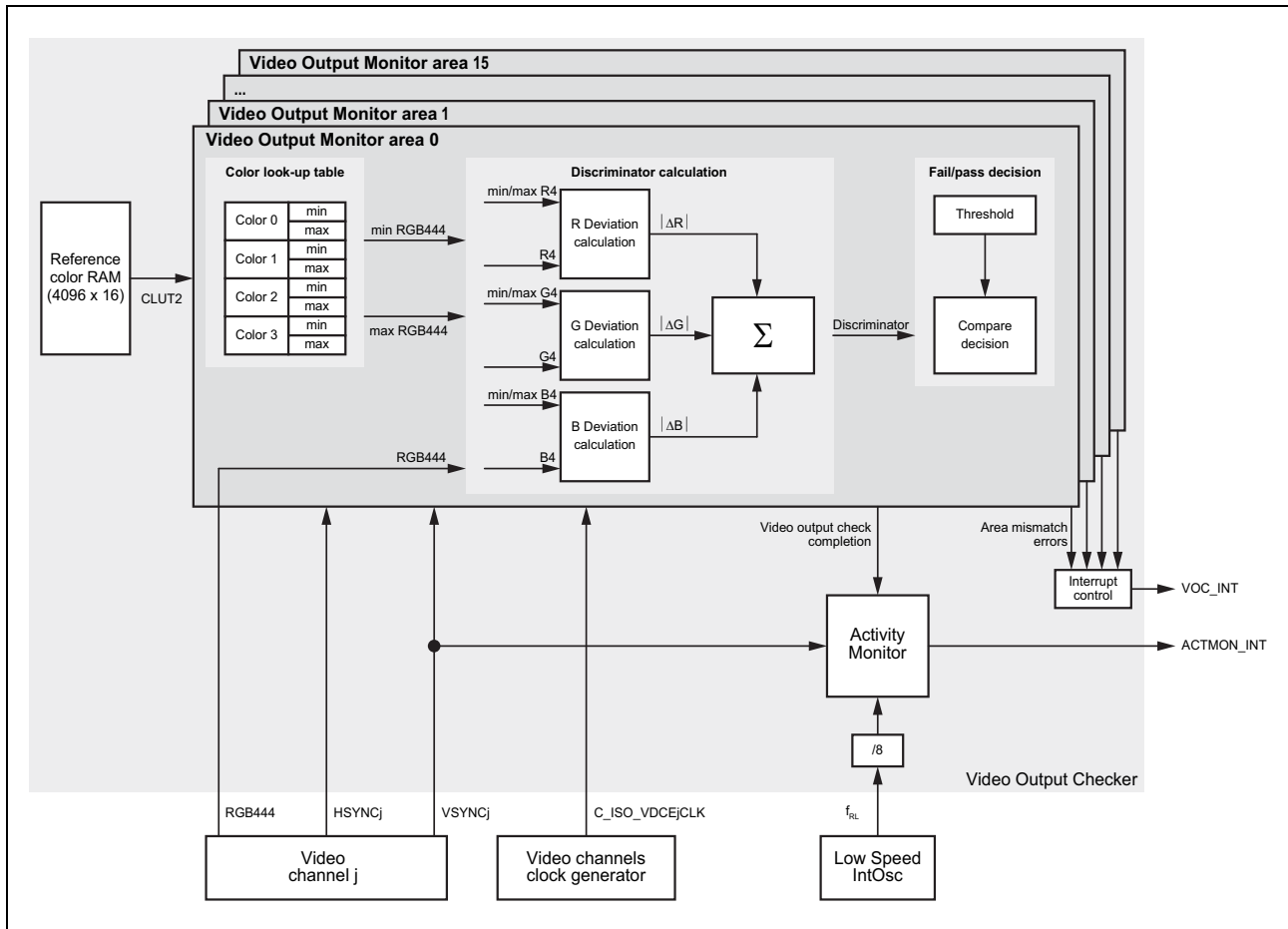
Figure 40.1 Block diagram of the Video Output Checker A
