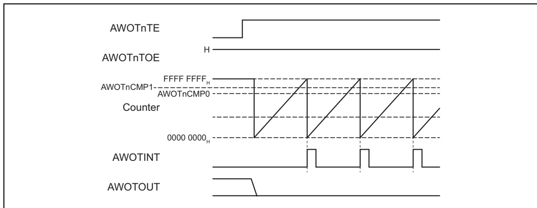
Figure 28.7 PWM mode with 0 % duty cycle
