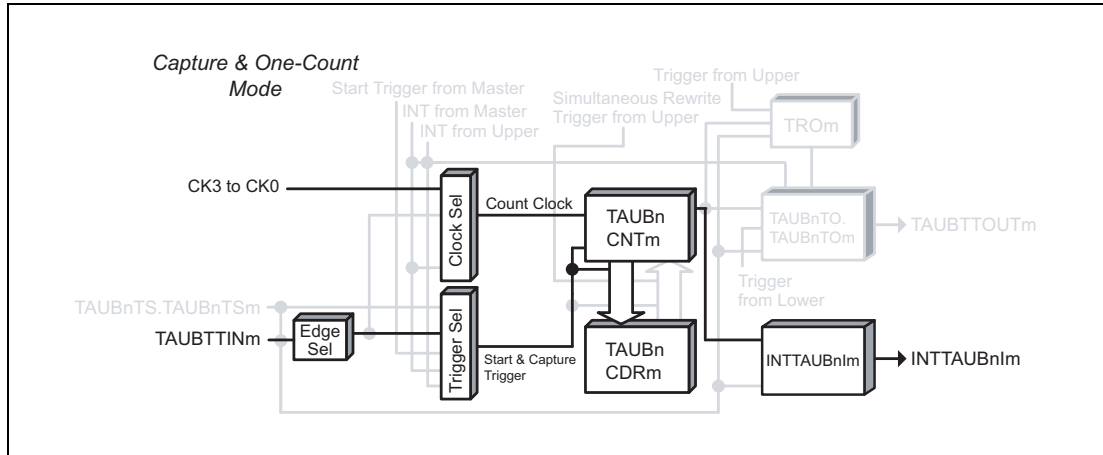
Figure 29.55 Block Diagram for TAUBTTINm Input Signal Width Measurement Function
