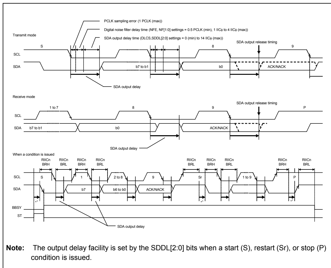
Figure 21.22 SDA Output Delay Facility
