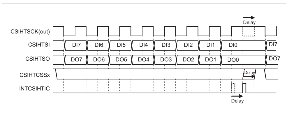
Figure 19.2 Interrupt Delay Function (CSIHnCTL1.CSIHnSIT = 1)
