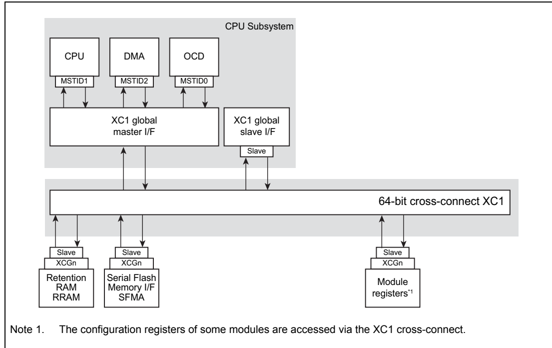
Figure 14.2 D1L1 cross-connect XC1
