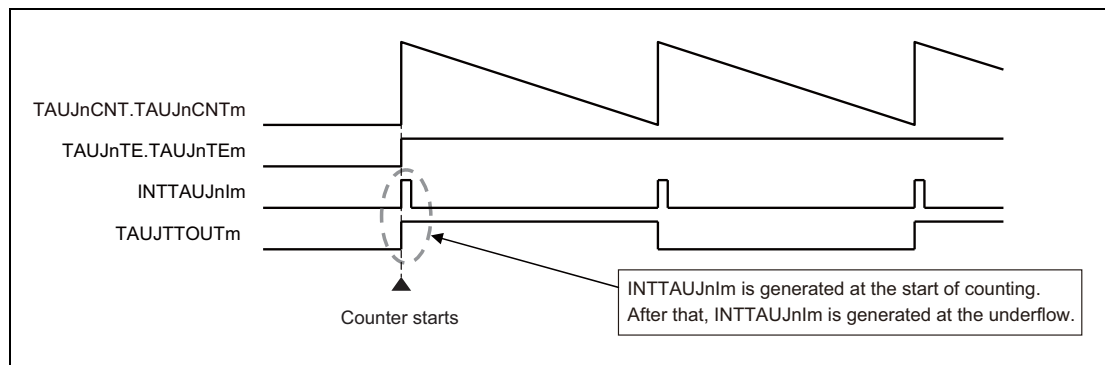
Figure 30.10 INTTAUJnIm Generation Timing (when TAUJnCMORm.TAUJnMD0 = 1)
