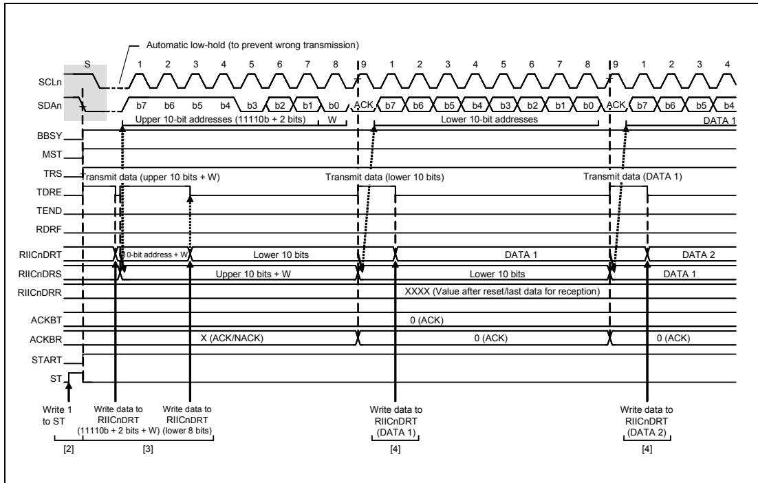
Figure 21.8 Master Transmit Operation Timing (2) (10-Bit Address Format)
