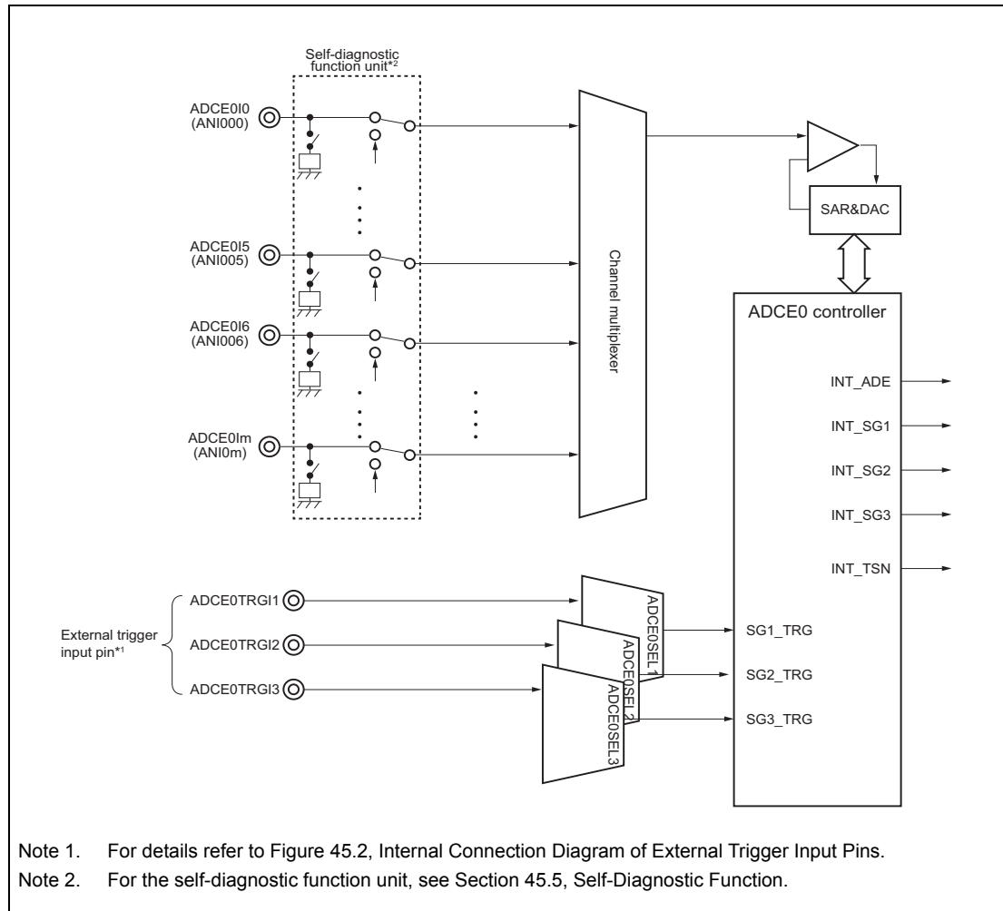
Figure 45.1 ADCE0 Block Diagram
