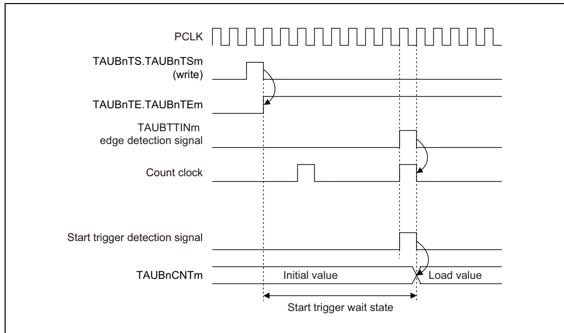
Figure 29.12 Start Timing in Other Operating Modes
