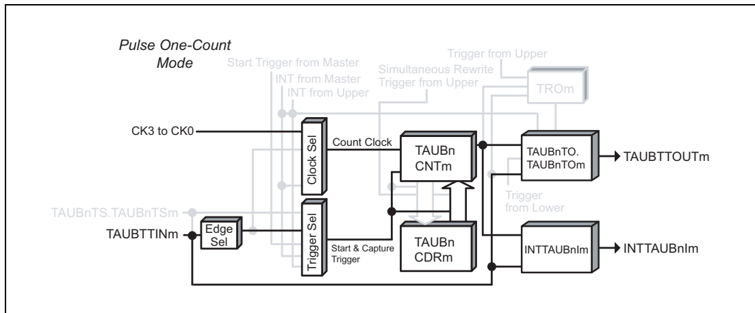
Figure 29.45 Block Diagram for One-Pulse Output Function
