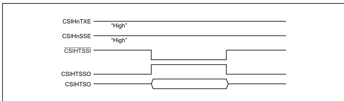
Figure 19.29 Operation of CSIHnTSSO
