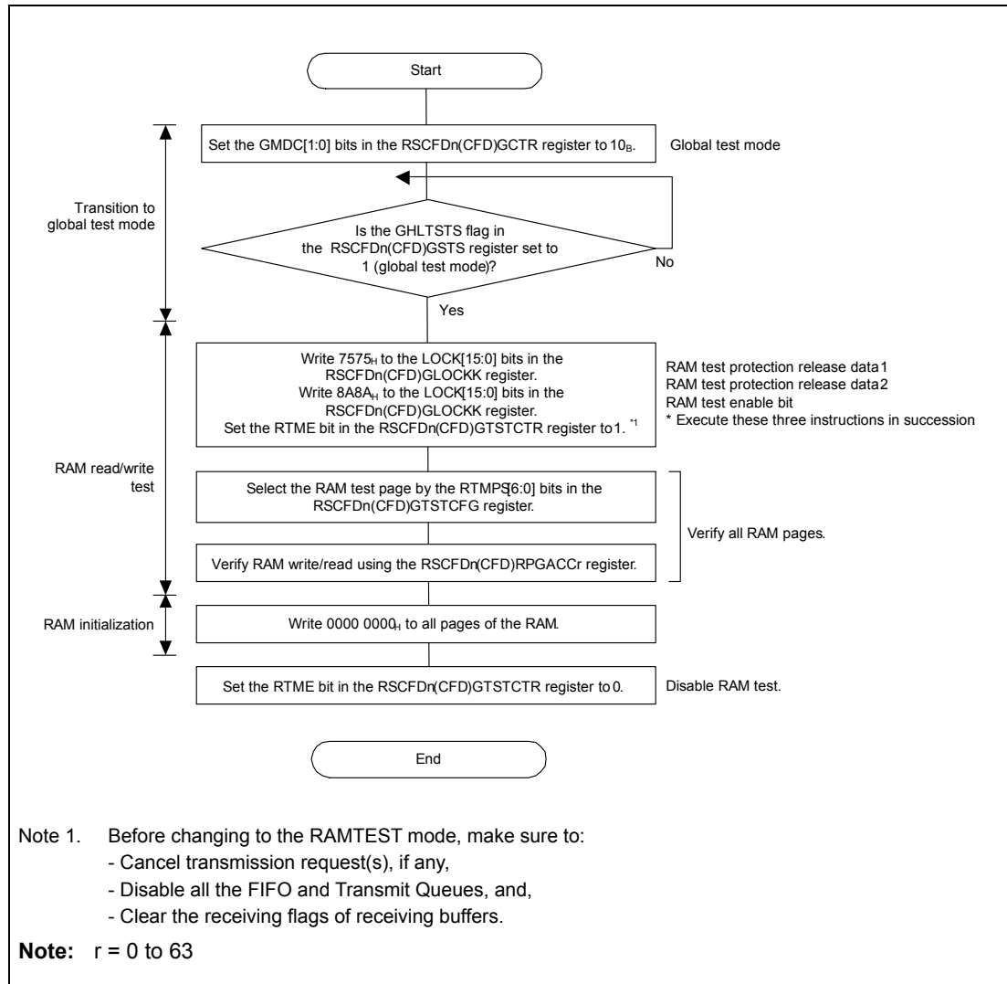
Figure 23.37 RAM Test Setting Procedure
