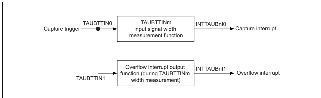
Figure 29.17 Combination of TAUBTTINm Input Signal Width Measurement Function and Overflow Interrupt Output Function (during TAUBTTINm Width Measurement)
