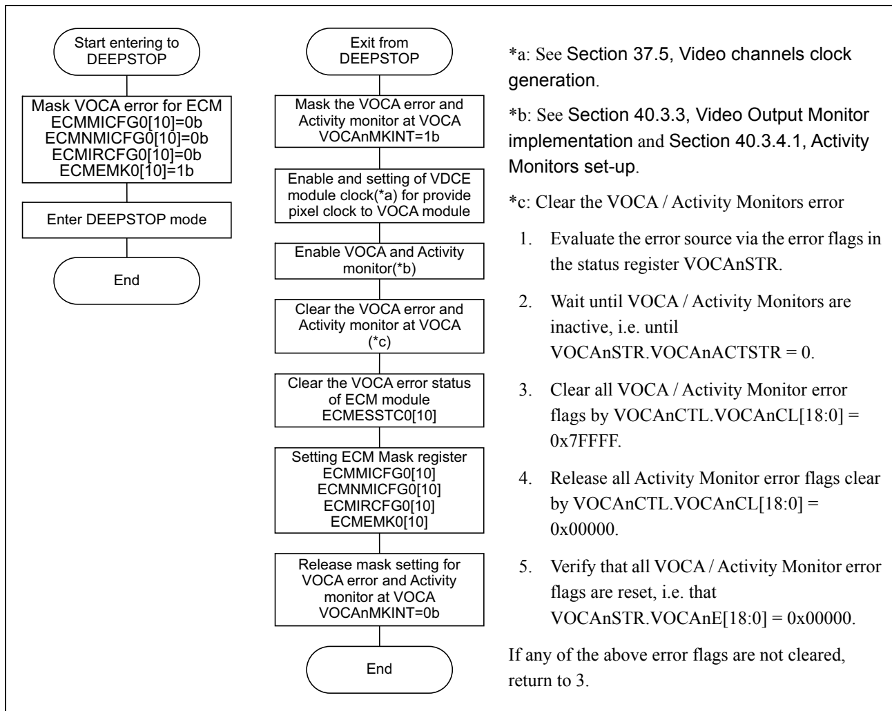
Figure 40.9 Workaround of unintended VOCA error (if VOCA is used)
