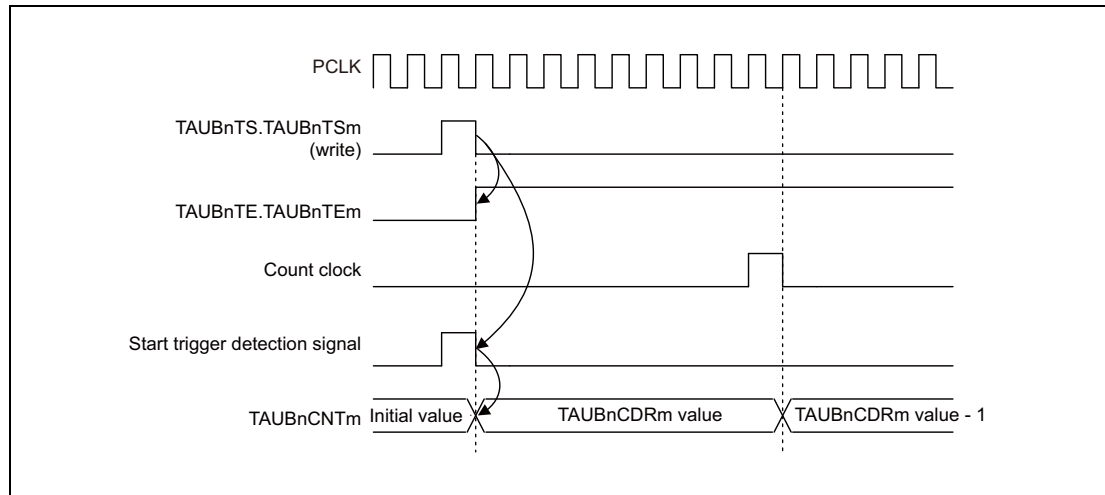
Figure 29.11 Start Timing in Event Count Mode
