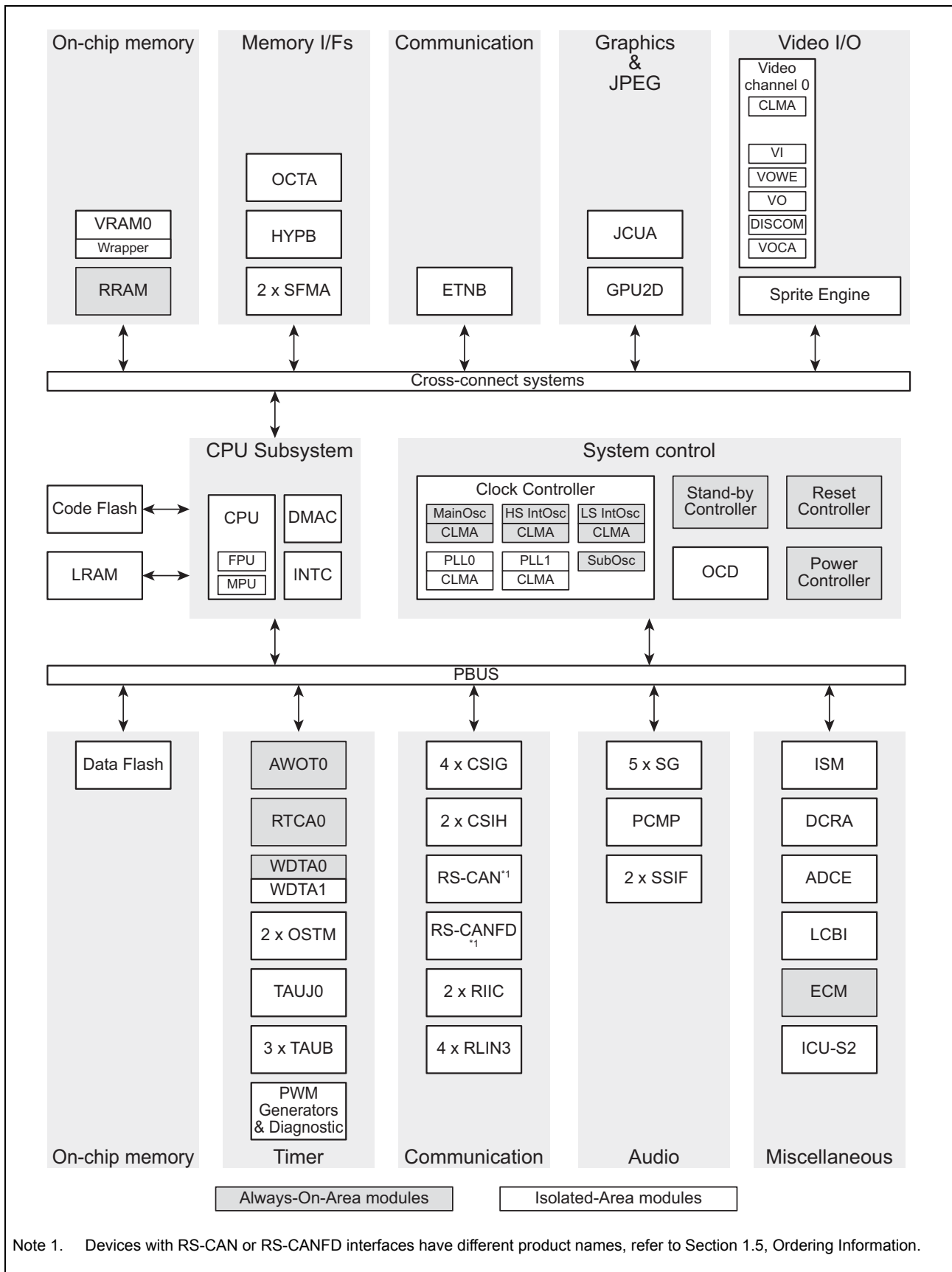
Figure 1.4 D1M1-V2 block diagram
