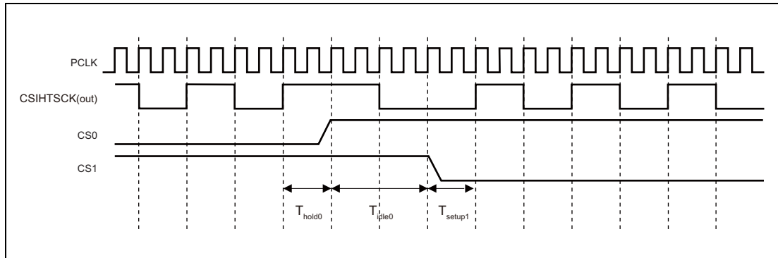
Figure 19.17 Clock Phase Timing with PCLK/4 , T_{hold0} = T_{setup1} = 0.5CSIHTSCK , T_{idle0} = 1CSIHTSCK , CSIHnCFG0.CSIHnCKP0 = 0 (CSIHTCSS0) → CSIHnCFG1.CSIHnCKP1 = 1 (CSIHTCSS1)
