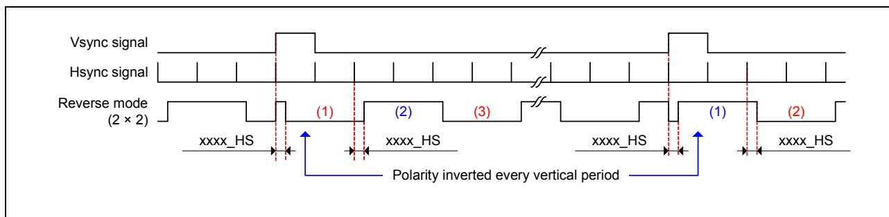
Figure 38.75 Horizontal Panel Driver Signal (in 2 × 2 Reverse Mode)
