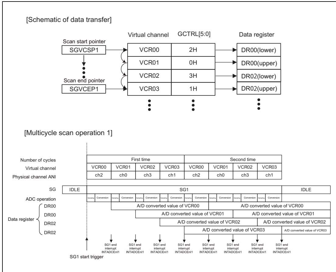
Figure 45.7 Example of Multicycle Scan Operation 1
