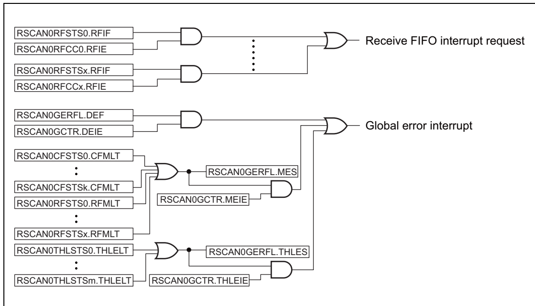
Figure 22.2 CAN Global Interrupt Block Diagram
