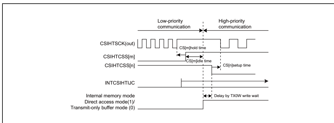
Figure 19.47 Transition from Low-Priority Mode to High-Priority Mode
