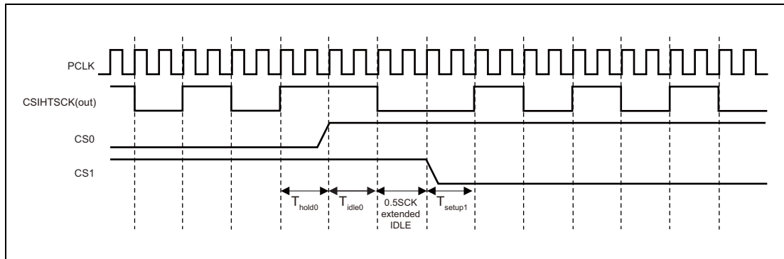
Figure 19.16 Clock Phase Timing with PCLK/4 , T_{hold0} = T_{setup1} = 0.5CSIHTSCK , T_{idle0} = 0.5CSIHTSCK , CSIHnCFG0.CSIHnCKP0 = 0 (CSIHTCSS0) → CSIHnCFG1.CSIHnCKP1 = 1 (CSIHTCSS1)
