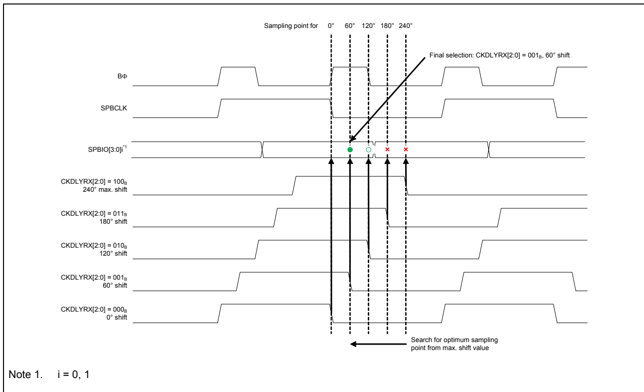
Figure 17.28 Sampling point calibration
