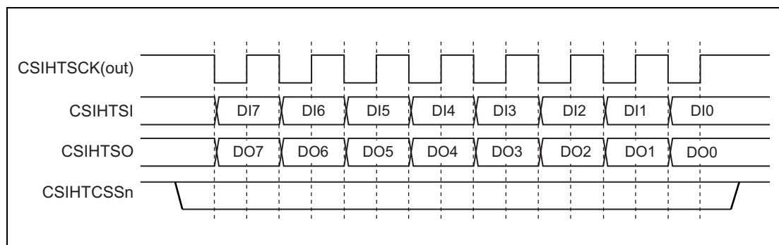
Figure 19.9 Transmit/Receive in Master Mode
