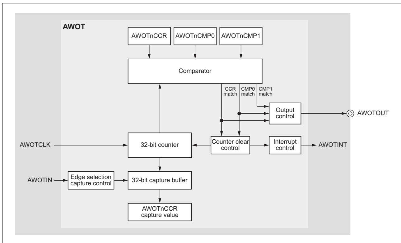
Figure 28.1 Block diagram of the AWOT
