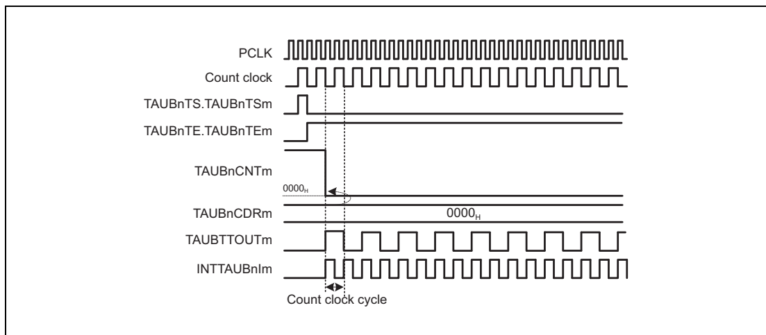
Figure 29.26 TAUBnCDRm = 0000 H , Count Clock = PCLK/2
