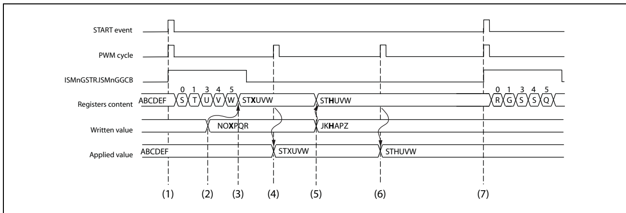
Figure 46.18 Channel data update timing
