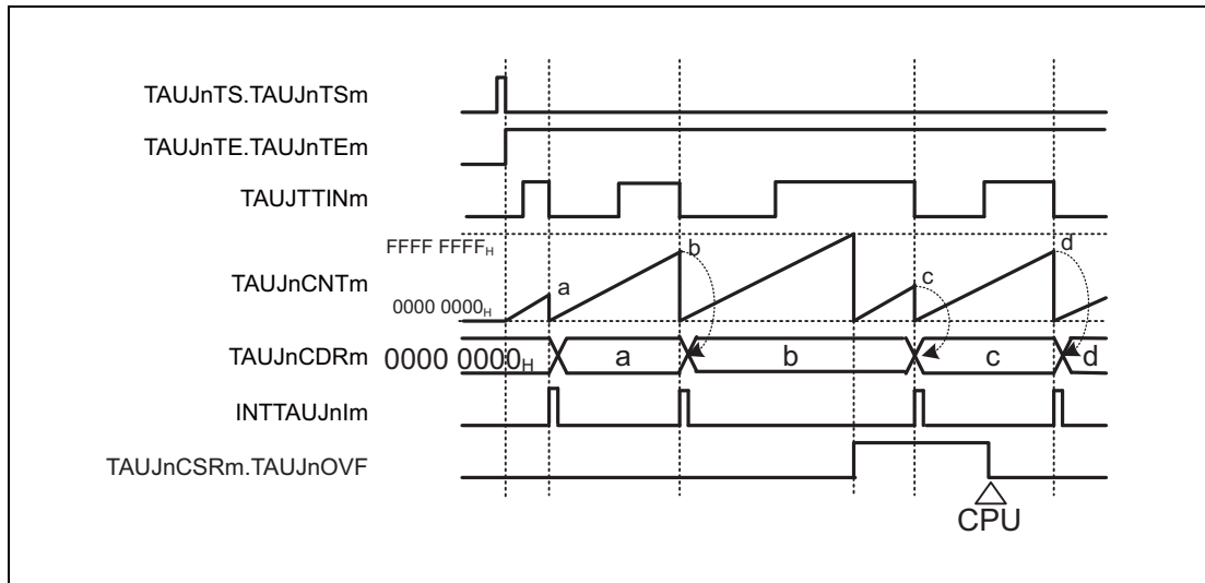
Figure 30.24 \text{TAUJnCMORm.TAUJnCOS}[1:0] = 01_B , \text{TAUJnCMORm.TAUJnMD0} = 0 , \text{TAUJnCMURm.TAUJnTIS}[1:0] = 00_B
