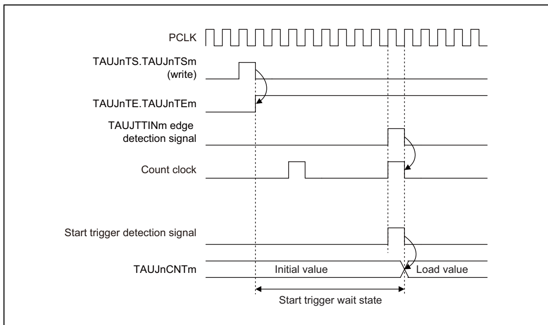
Figure 30.8 Start Timing in Other Operating Modes
