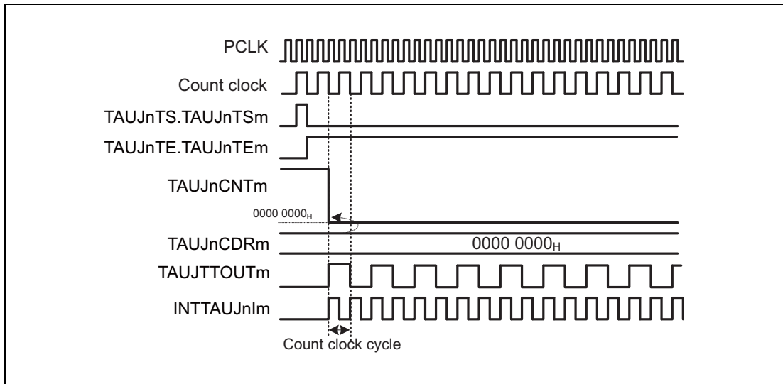
Figure 30.14 TAUJnCDRm = 0000 0000 H , Count Clock = PCLK/2
