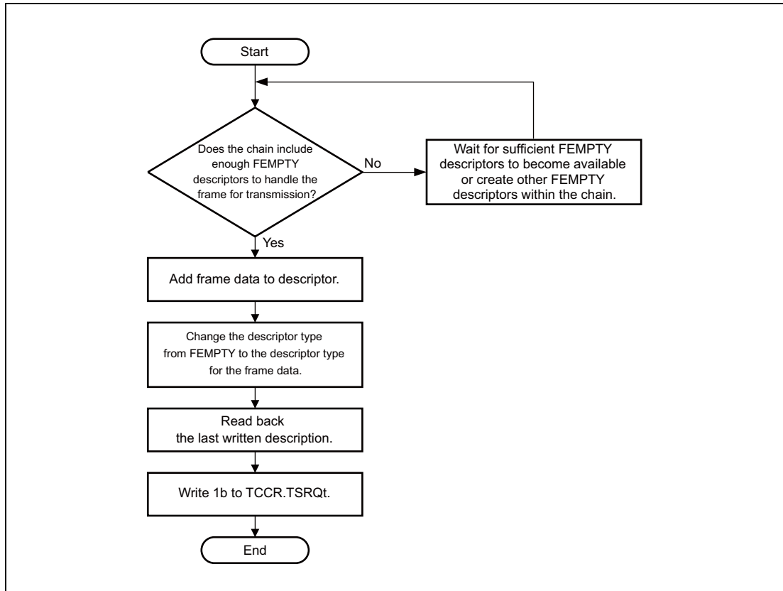
Figure 24.35 Software Flow for Immediate Frame Transmission
