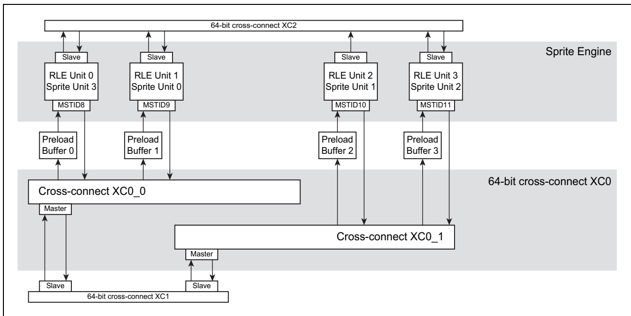
Figure 14.12 D1M1-V2 cross-connect XC0
