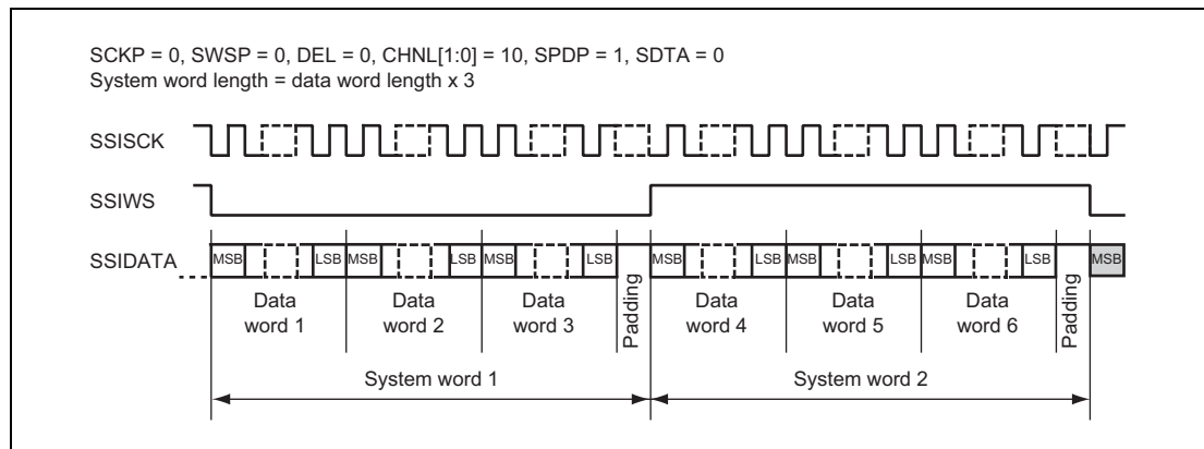
Figure 35.7 Multi-Channel Format (6 Channels with High Padding)
