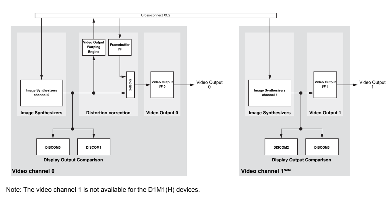
Figure 41.1 DISCOM connections to the video channels
