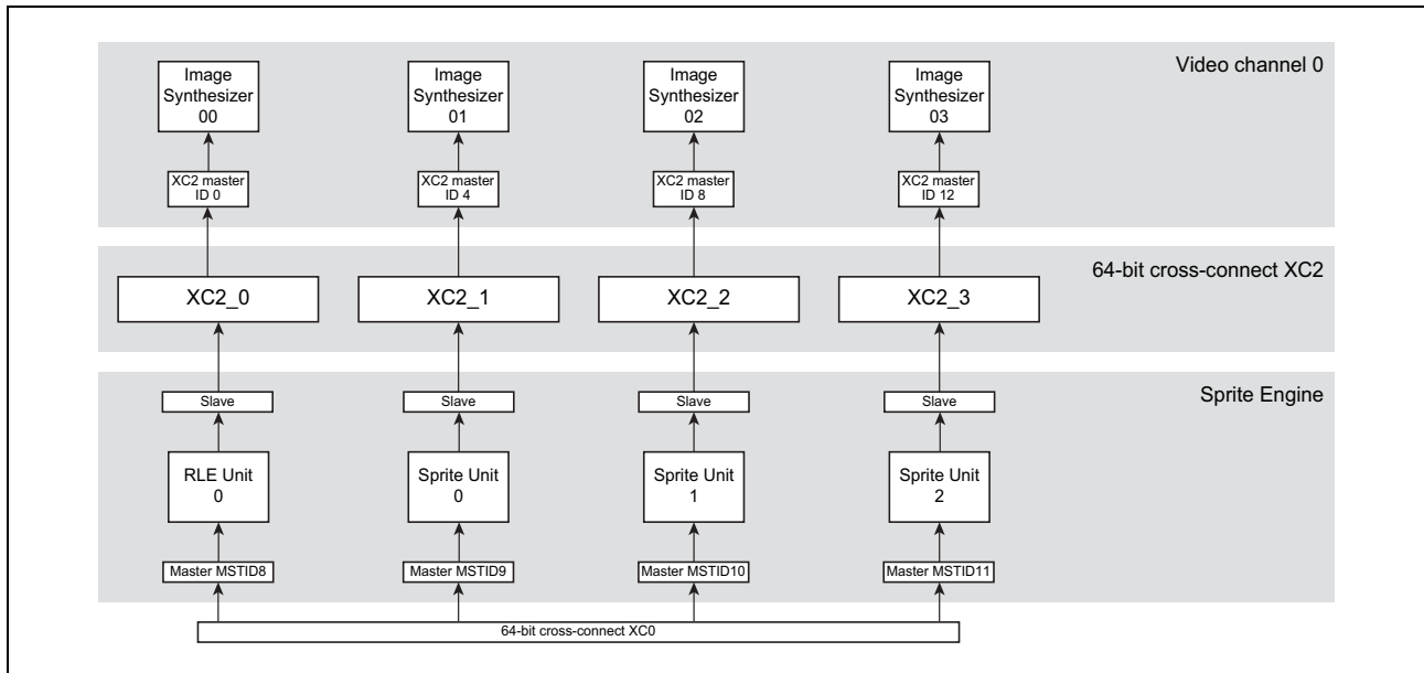
Figure 14.6 D1L2(H) cross-connect XC2
