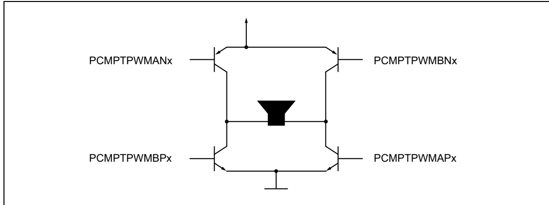
Figure 34.10 Driving a full H-bridge
