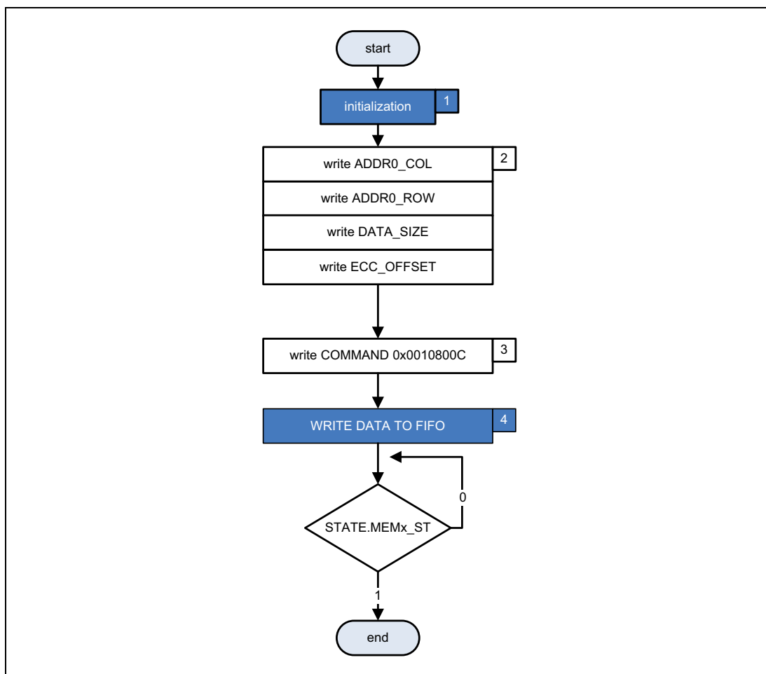
Figure 58.36 Writing Partial Pages
