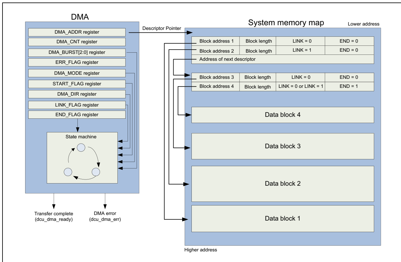
Figure 58.40 Example of Scatter-Gather DMA Data Transfer
