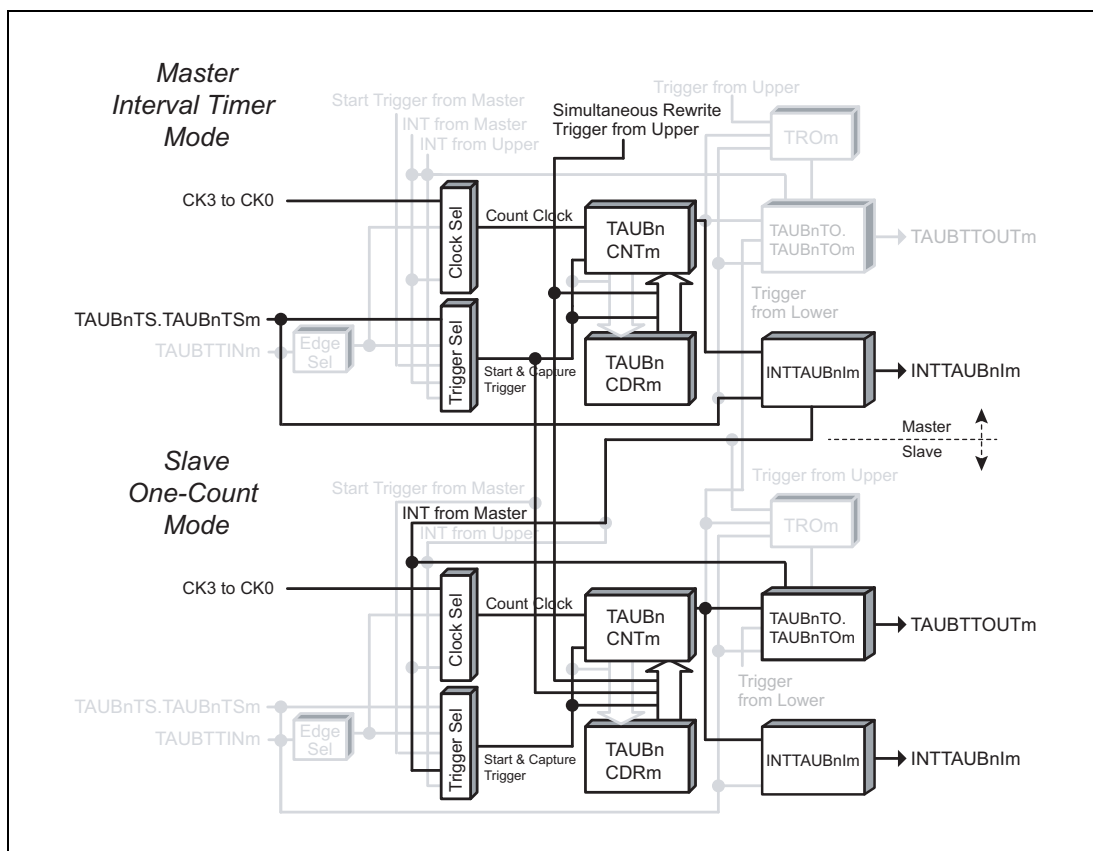
Figure 29.78 Block Diagram for PWM Output Function
