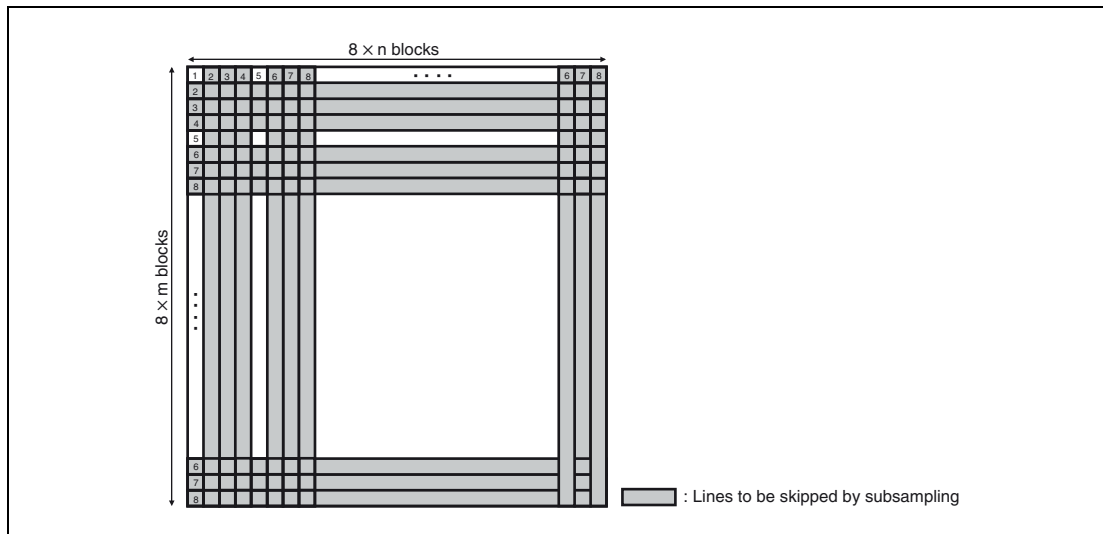
Figure 44.12 MCU when subsampling into 1/4 is selected
