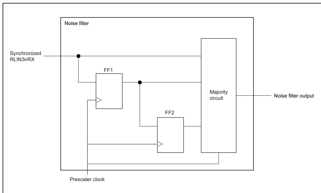
Figure 20.31 Example of Noise Filter Circuit
