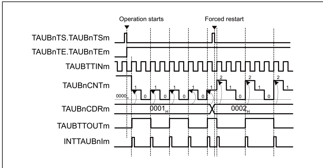
Figure 29.39 Forced Restart, (TAUBnCMORM.TAUBnMD0 = 1, TAUBnCMURm.TAUBnTIS[1:0] = 01 B )
