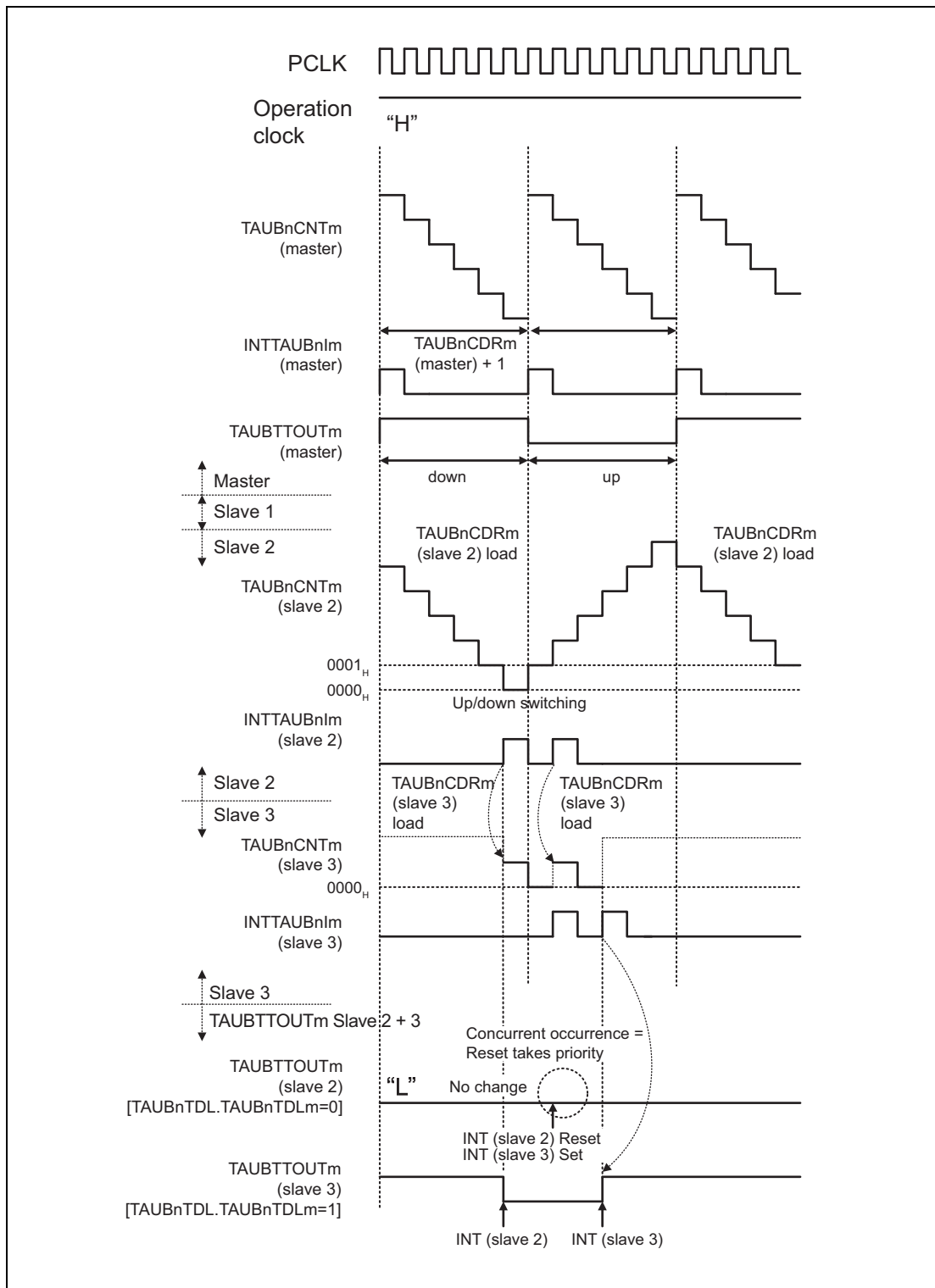
Figure 29.108 TAUBnCDRm (master) = 0005 H , TAUBnCDRm (slave 2) = 0005 H , TAUBnCDRm (slave 3) = 0001 H PWM Signal Width (positive phase) = 0
