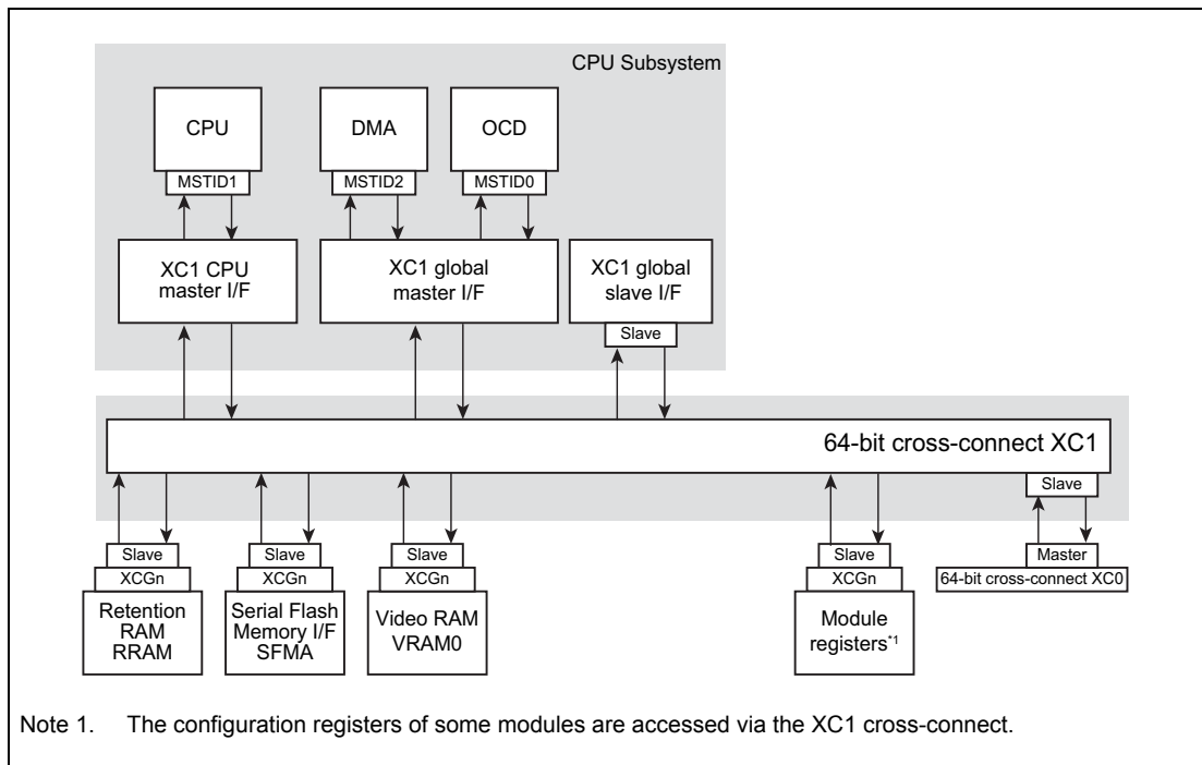
Figure 14.5 D1L2(H) cross-connect XC1
