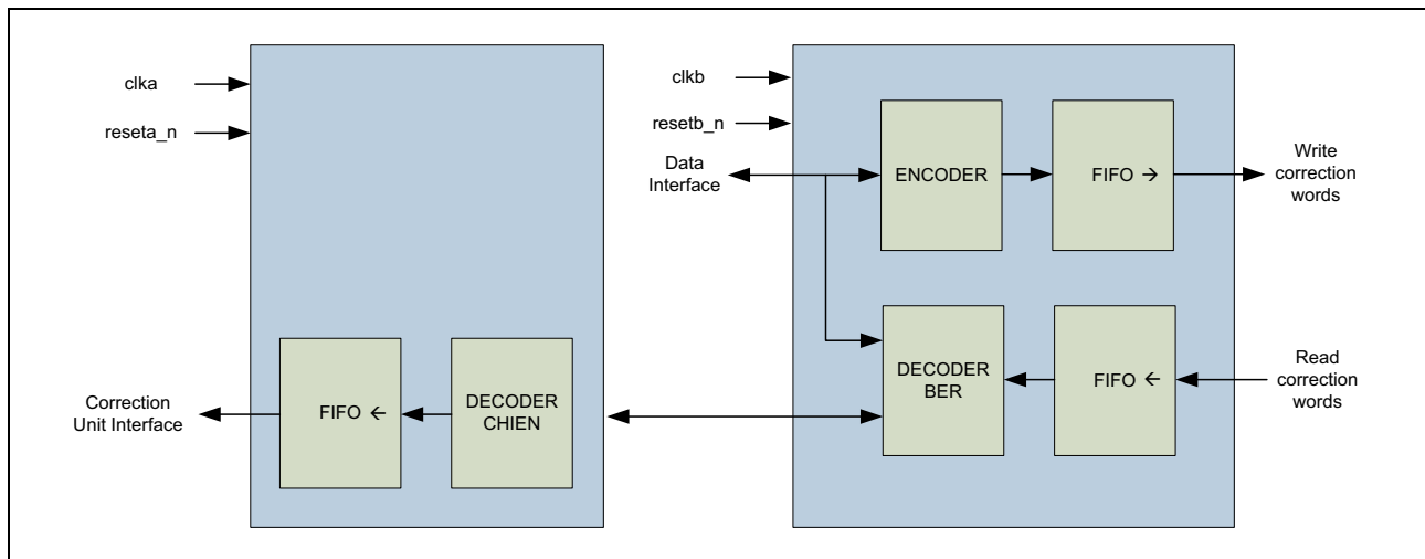
Figure 58.41 ECC Module Block Diagram
