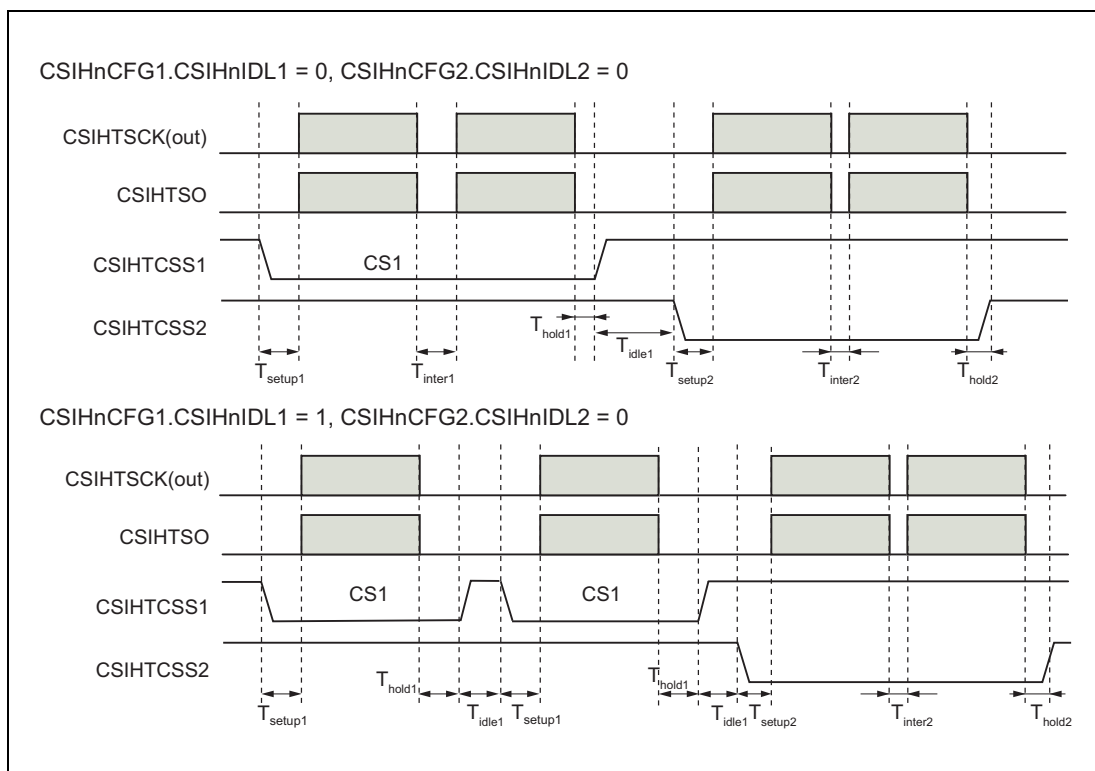
Figure 19.13 Chip Select Timings
