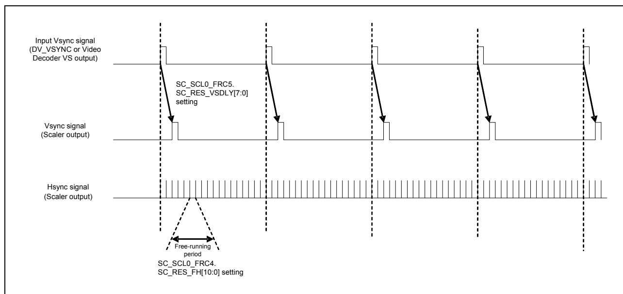
Figure 38.4 External Input Vsync Timing
