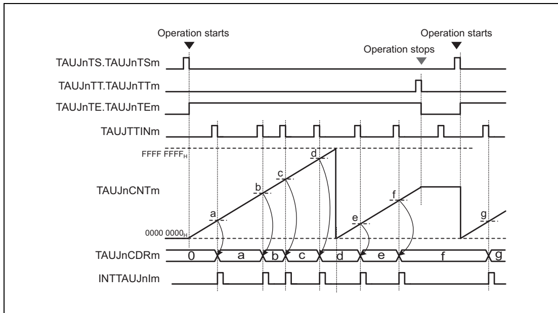
Figure 30.35 Operation Stop and Restart ( TAUJnCMORm.TAUJnMD0 = 0 , TAUJnCMURm.TAUJnTIS[1:0] = 00_B )
