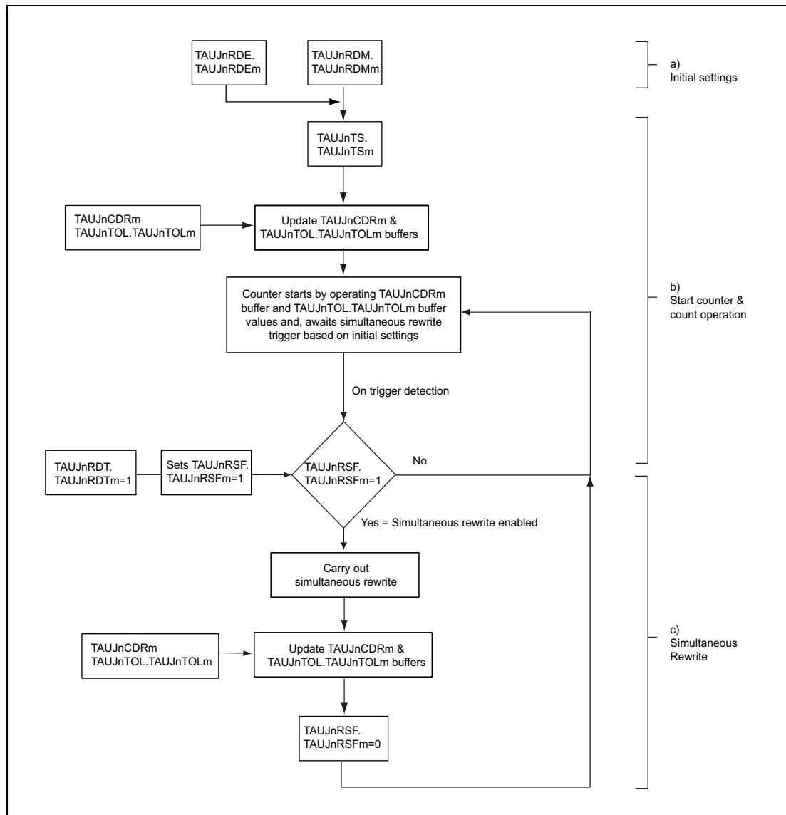
Figure 30.4 General Procedure for Simultaneous Rewrite
