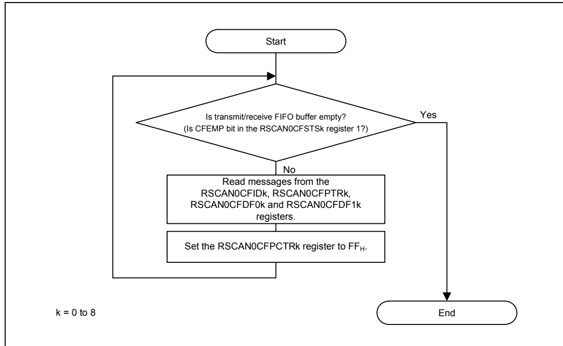
Figure 22.24 Transmit/Receive FIFO Buffer Reading Procedure
