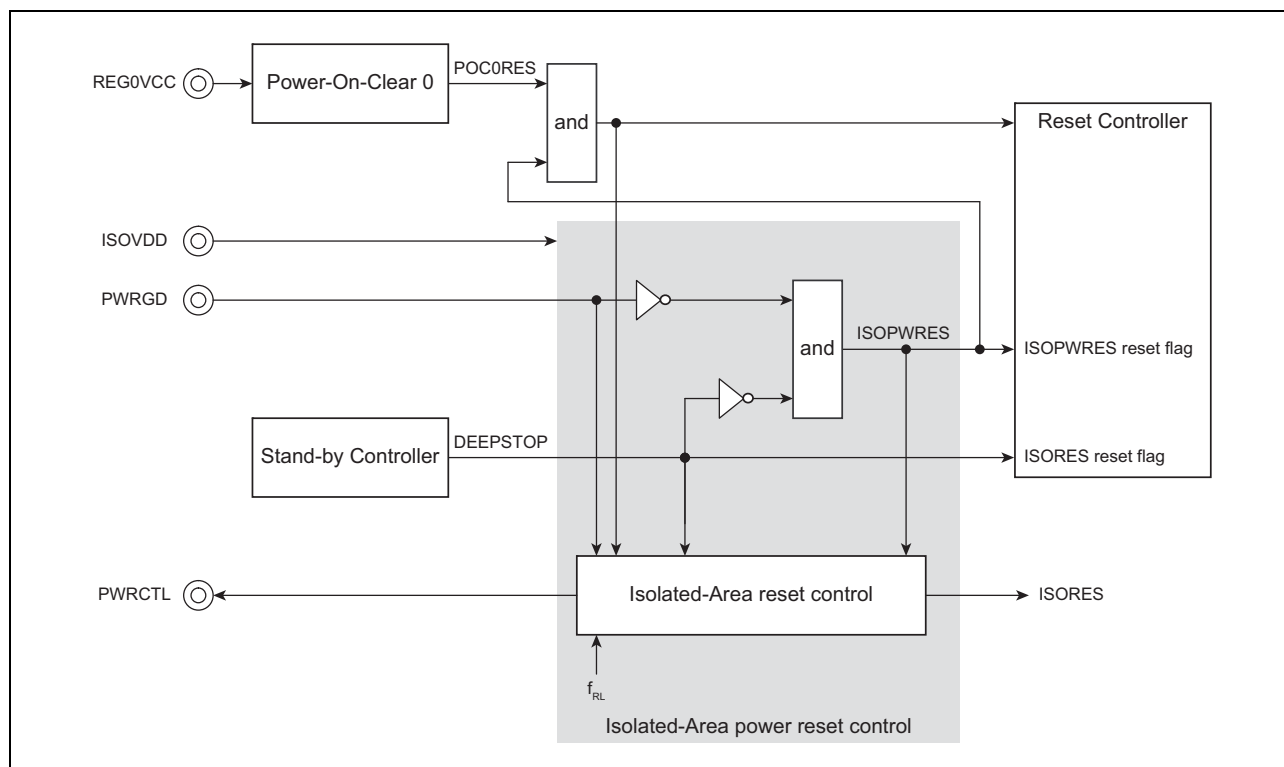
Figure 9.3 D1M2(H) Isolated-Area power reset
