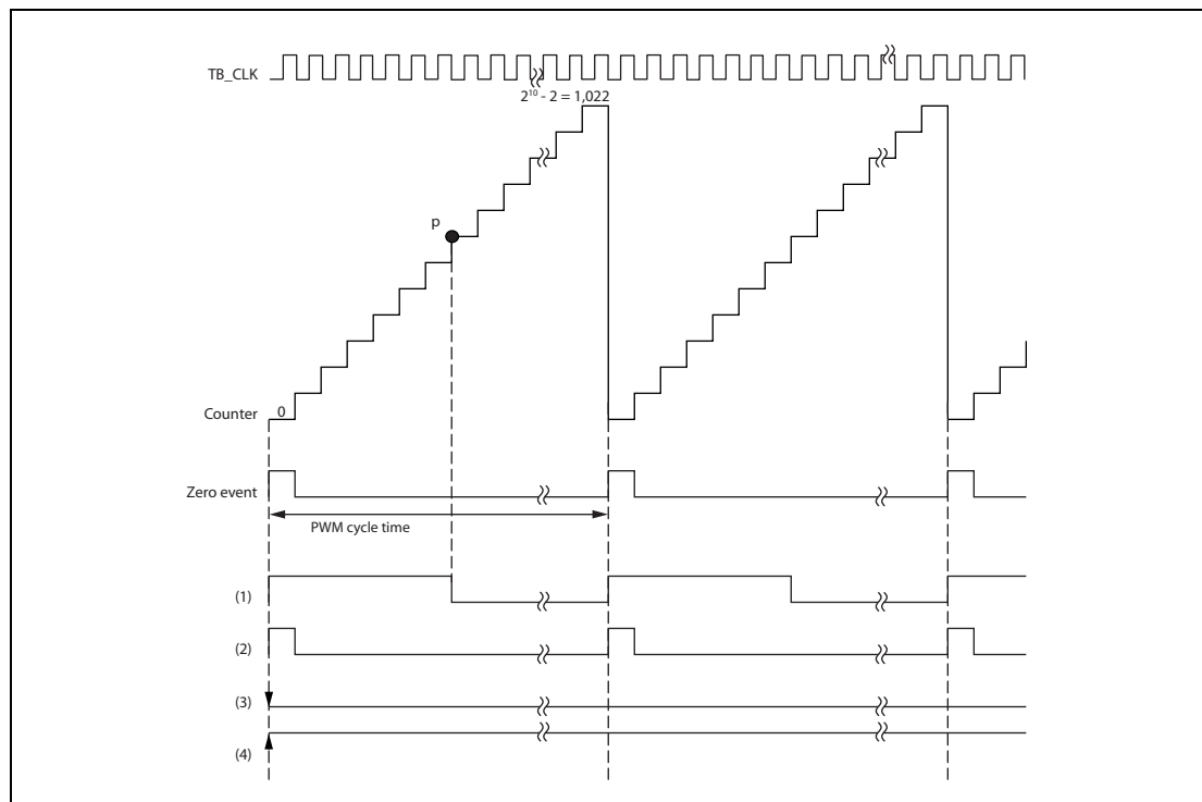
Figure 46.4 Examples of different PWM signals
