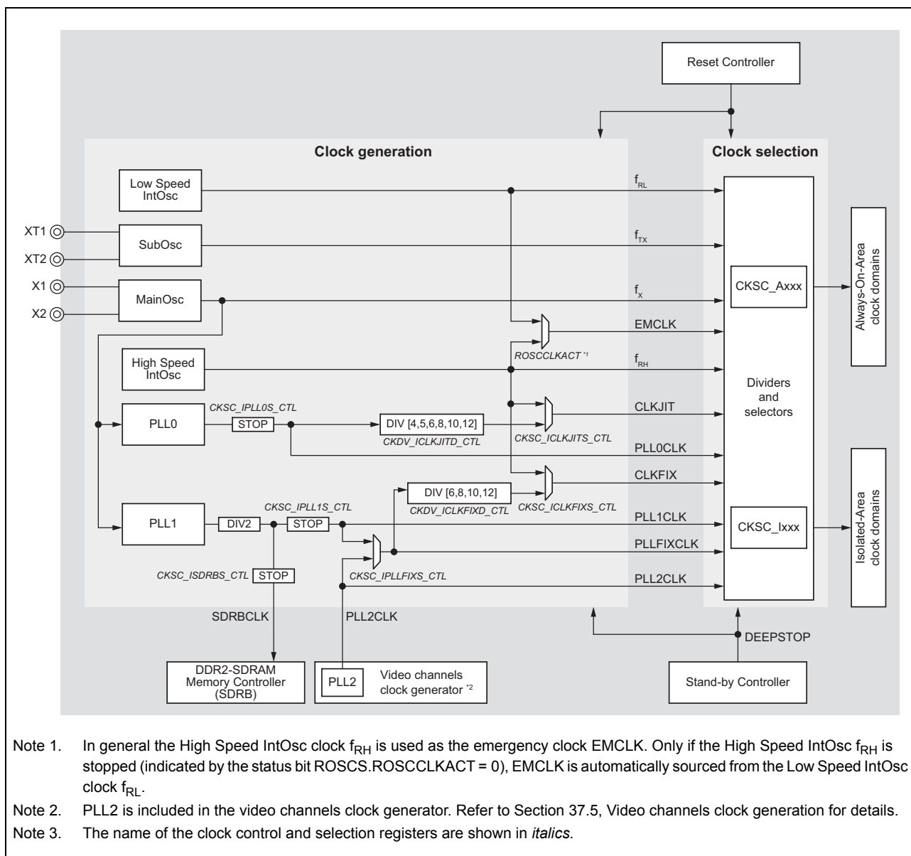
Figure 12.6 D1M2(H) Clock Controller block diagram
