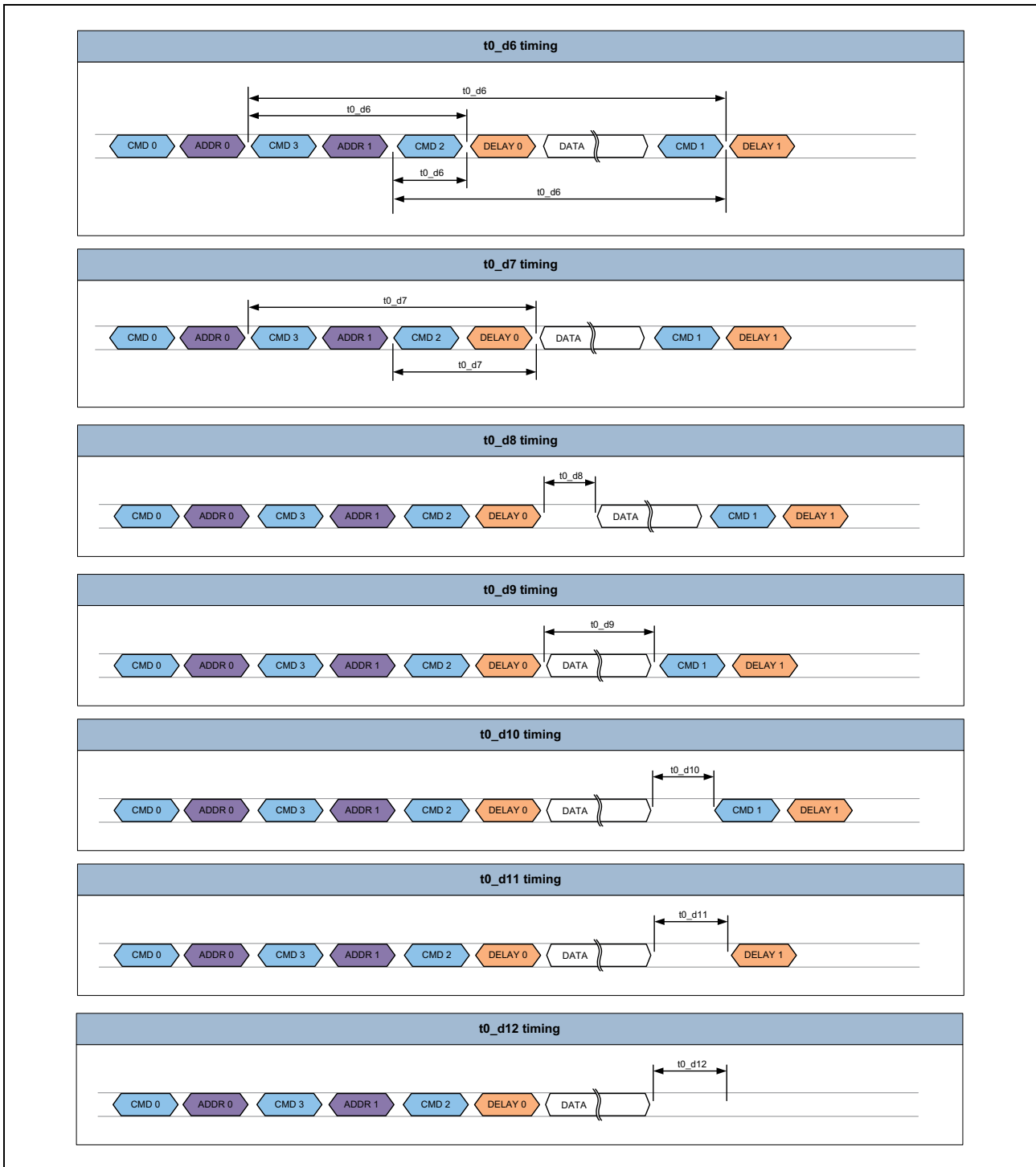
Figure 58.28 Generic Sequence Timing parameters
