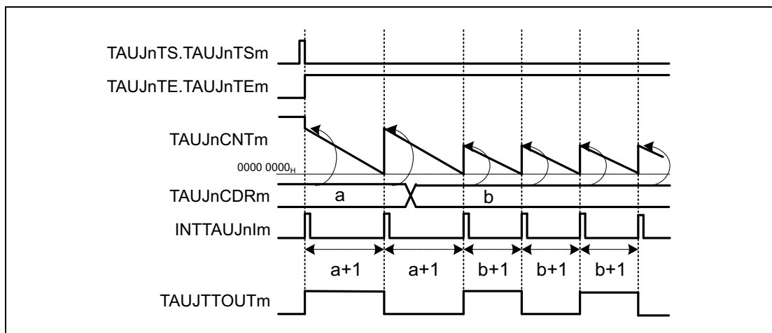
Figure 30.13 General Timing Diagram for Interval Timer Function
