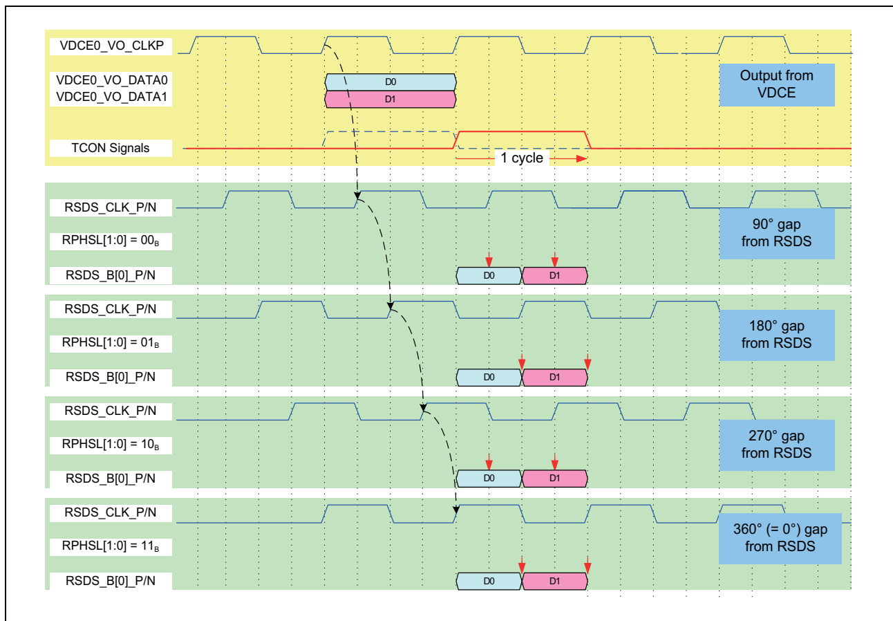
Figure 37.24 RSDS clock phase shift
