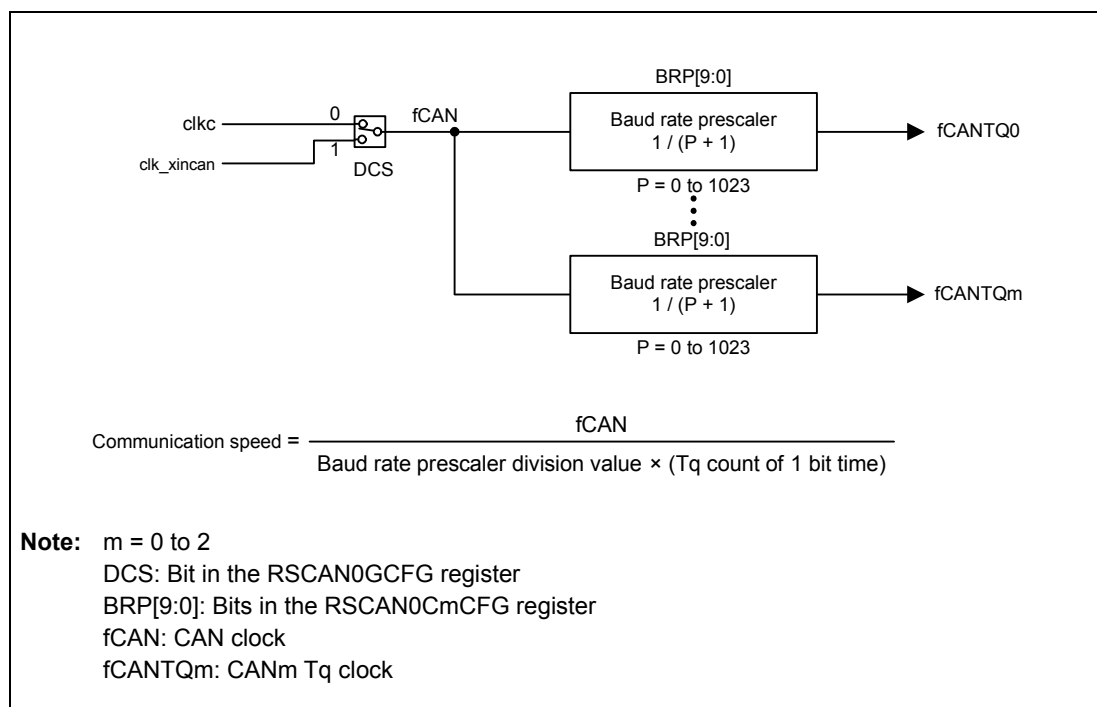
Figure 22.18 CAN Clock Control Block Diagram
