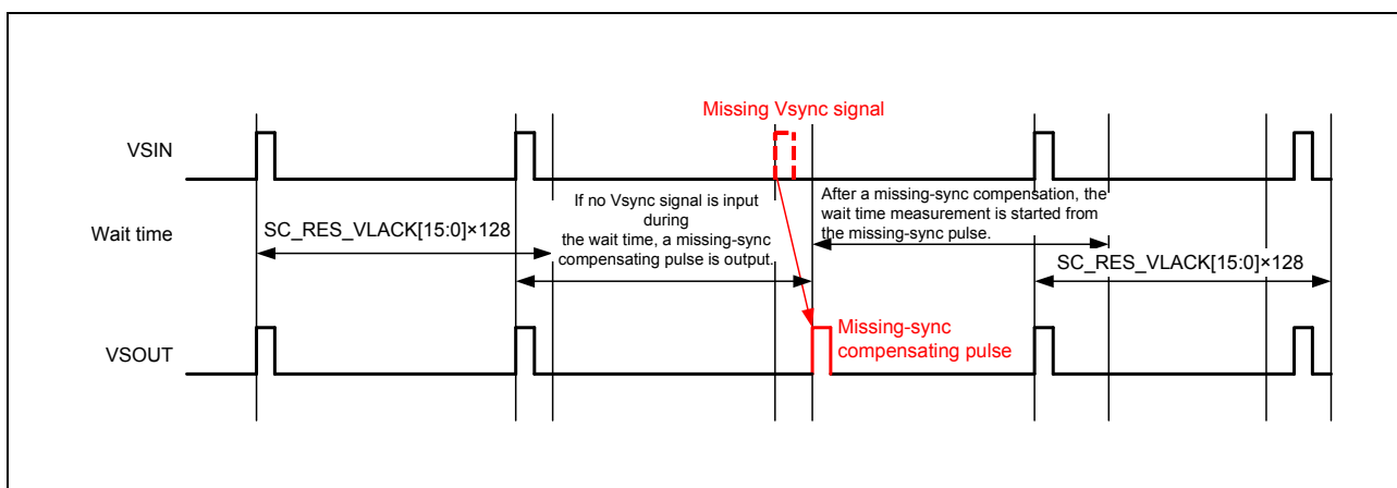
Figure 38.27 Compensation of Missing Vsync Signals
