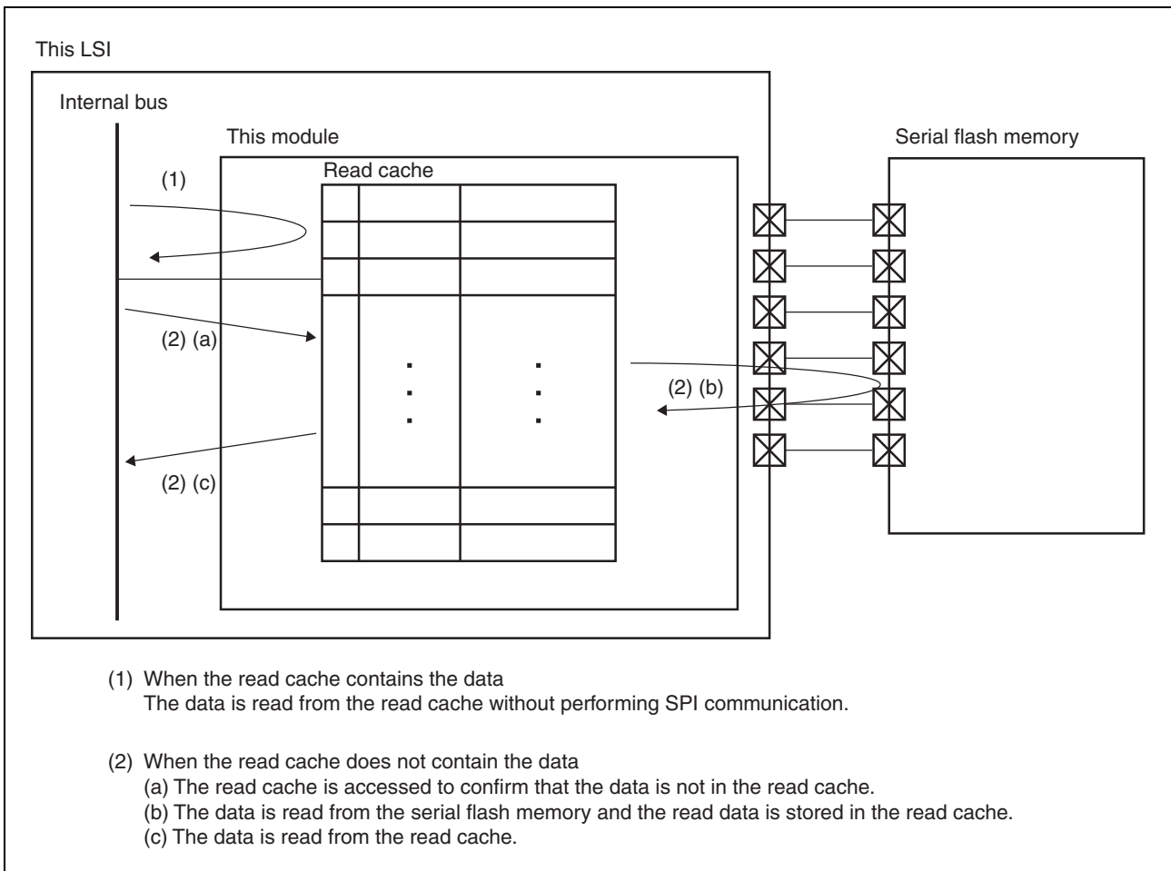
Figure 17.8 Burst Read Operation
