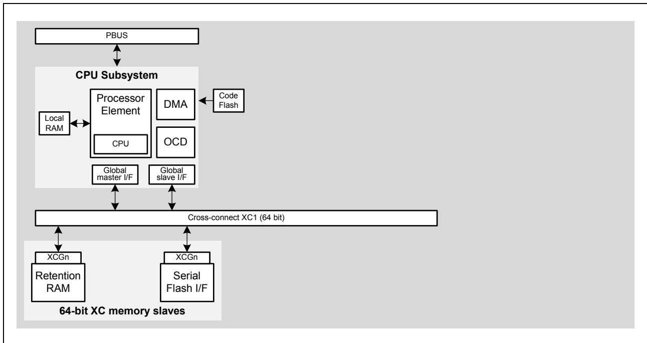
Figure 14.1 D1L1 bus architecture overview
