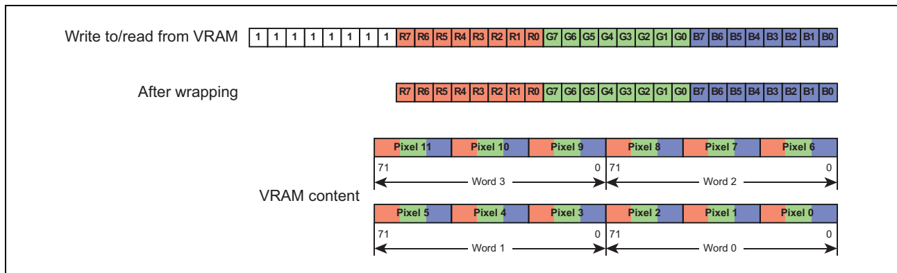
Figure 54.5 Wrapped 24 bpp RGB888
