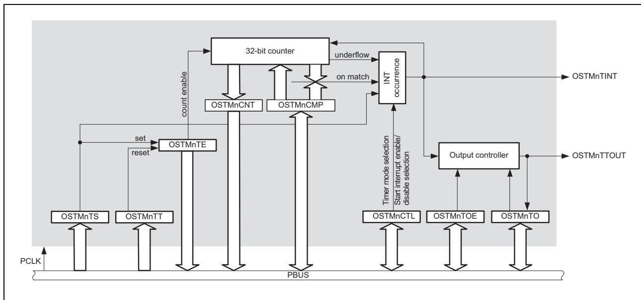
Figure 27.1 Block diagram of OSTM
