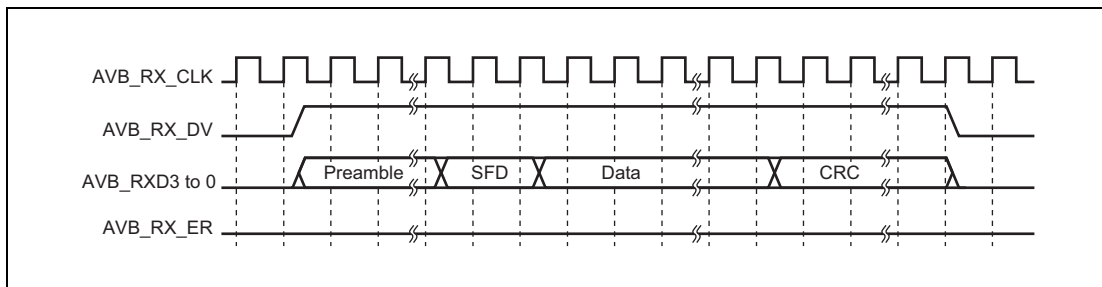
Figure 24.66 MII Frame Receive Timing (Normal Reception)
