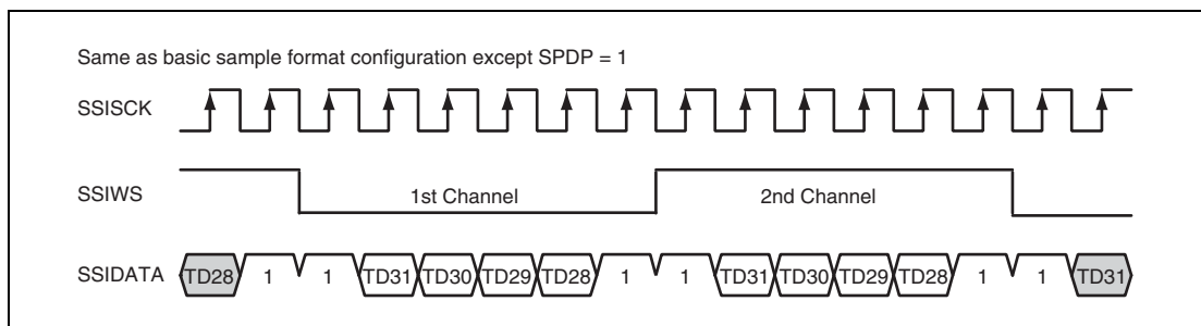
Figure 35.12 Inverted Padding Polarity
