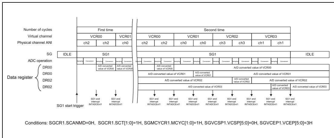
Figure 45.11 Example of Channel Repeat Operation 2
