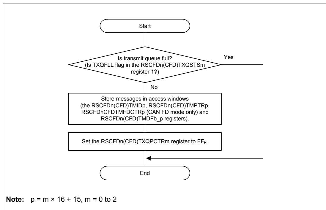
Figure 23.33 Procedure for Transmission from the Transmit Queue
