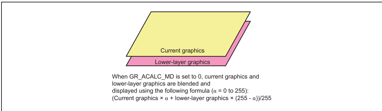
Figure 38.51 Graphics Planes with GR_DISP_SEL Set to 3
