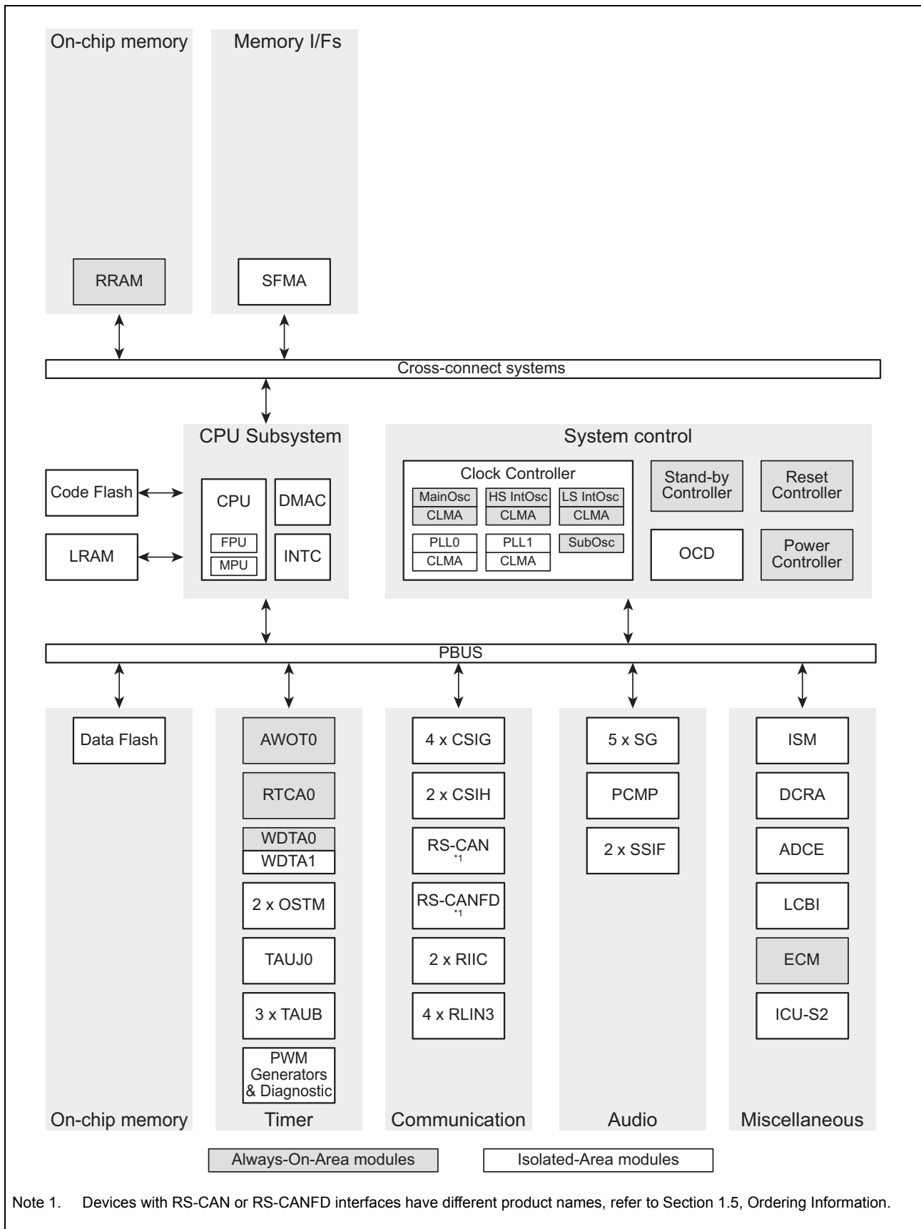
Figure 1.1 D1L1 block diagram
