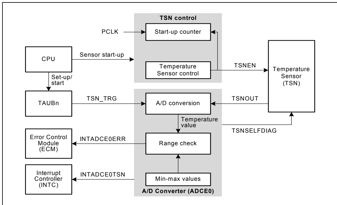
Figure 11.1 Temperature measurement set-up
