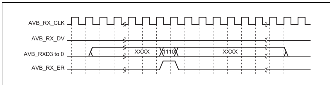
Figure 24.68 MII Frame Receive Timing (Reception Error (2))
