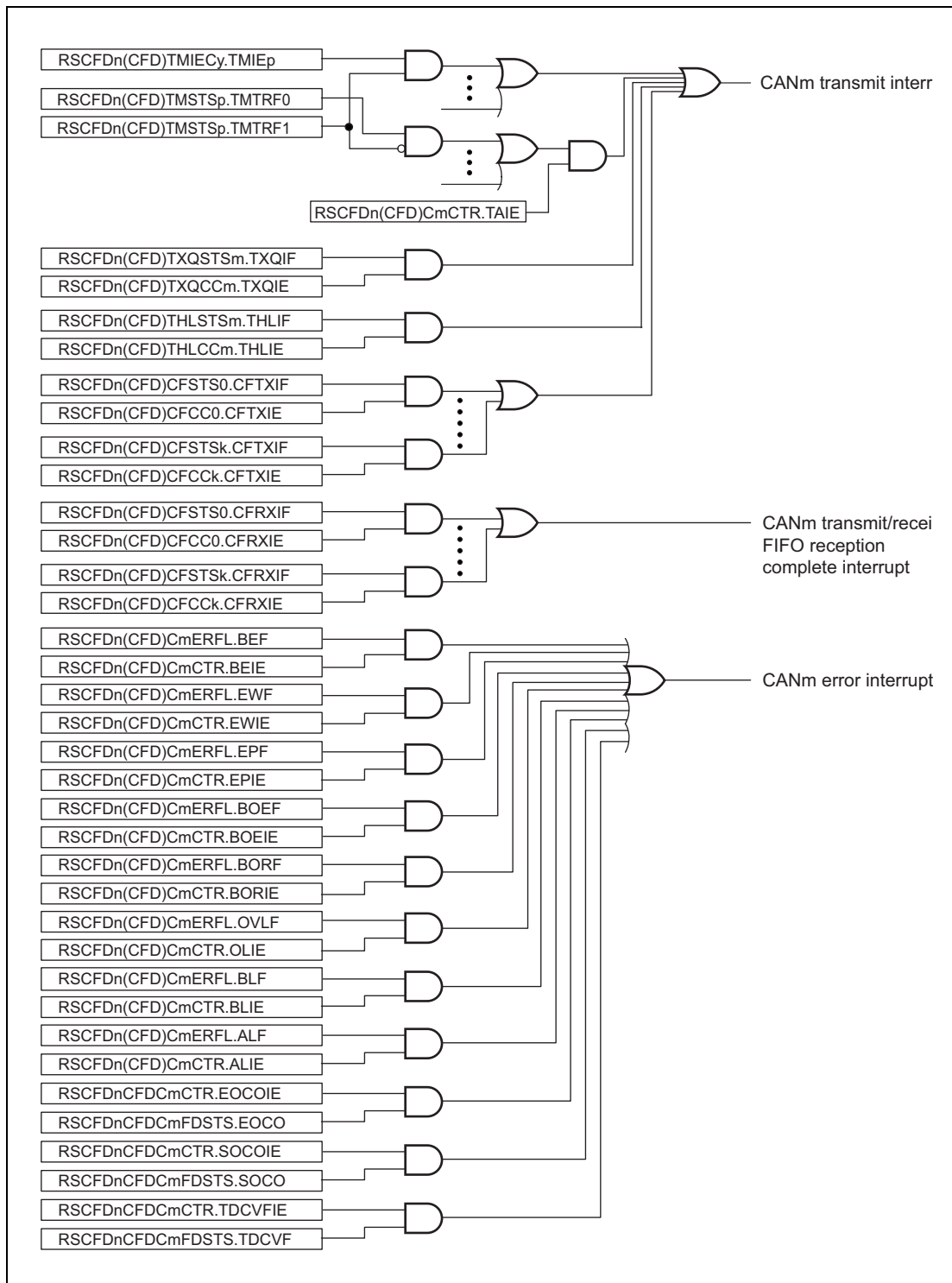
Figure 23.3 CAN Channel Interrupt Block Diagram
