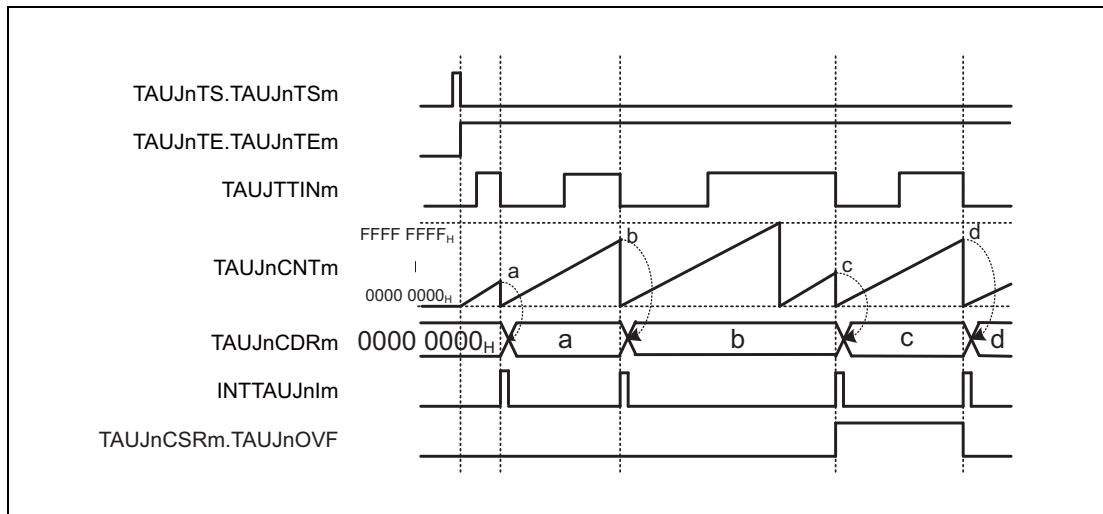
Figure 30.23 TAUJnCMORM.TAUJnCOS[1:0] = 00 B , TAUJnCMORM.TAUJnMD0 = 0, TAUJnCMURm.TAUJnTIS[1:0] = 00 B
