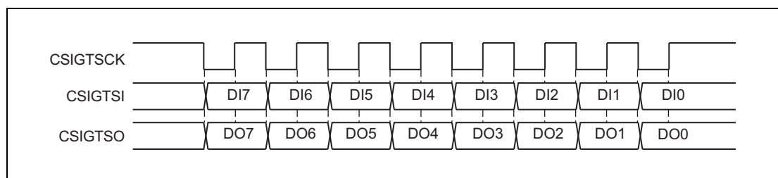
Figure 18.7 Transmission/Reception in Slave Mode
