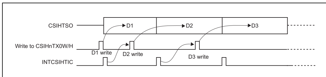
Figure 19.4 Immediate Generation of INTCSIHTIC (CSIHnCTL1.CSIHnSLIT = 1)
