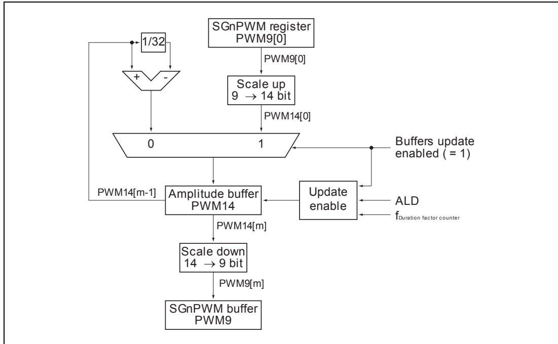
Figure 33.7 Volume calculation in ALD mode
