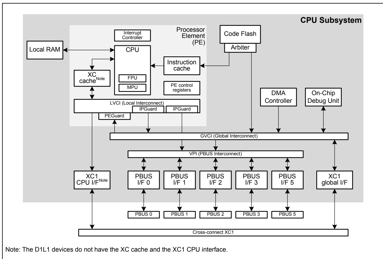
Figure 3.1 CPU Subsystem block diagram
