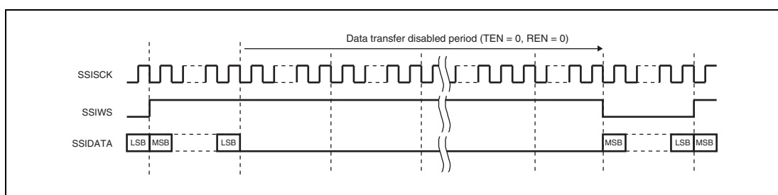
Figure 35.21 WS Continue Mode Disabled
