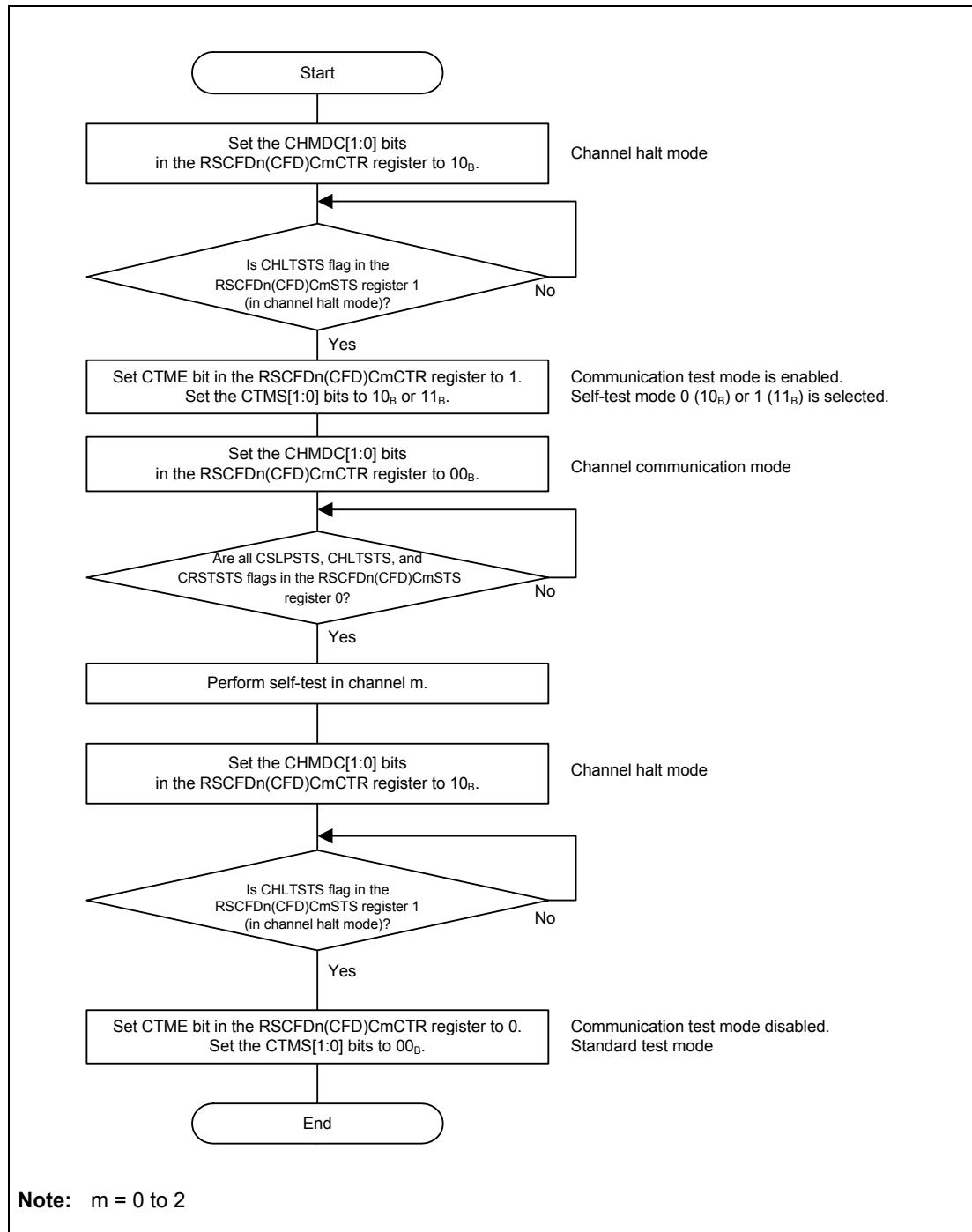
Figure 23.35 Self-Test Mode Setting Procedure
