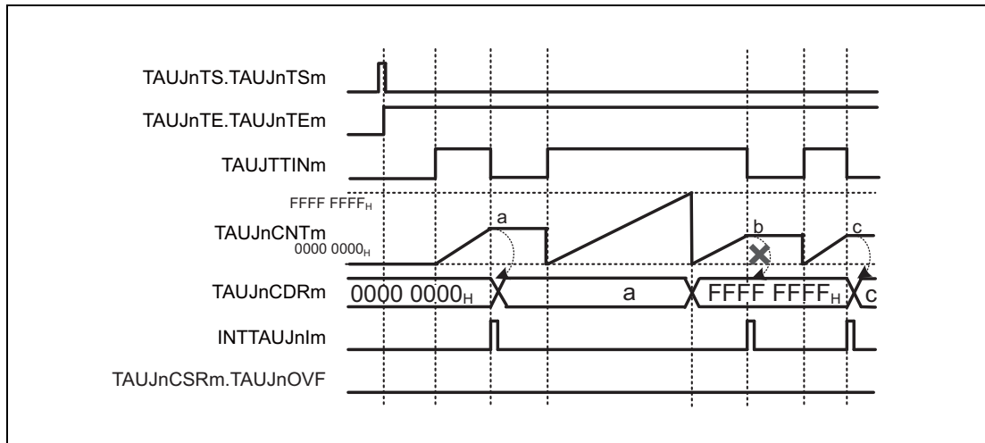
Figure 30.31 \text{TAUJnCMORm.TAUJnCOS}[1:0] = 10_{\text{B}} , \text{TAUJnCMORm.TAUJnMD0} = 0 , \text{TAUJnCMURm.TAUJnTIS}[1:0] = 11_{\text{B}}
