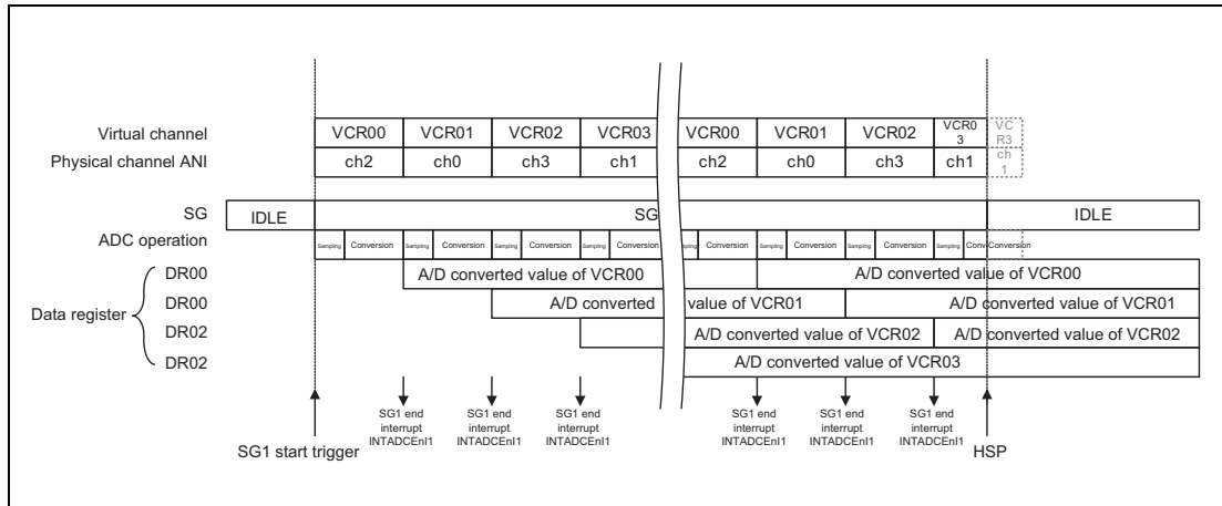
Figure 45.9 Example of Continuous Scan Operation
