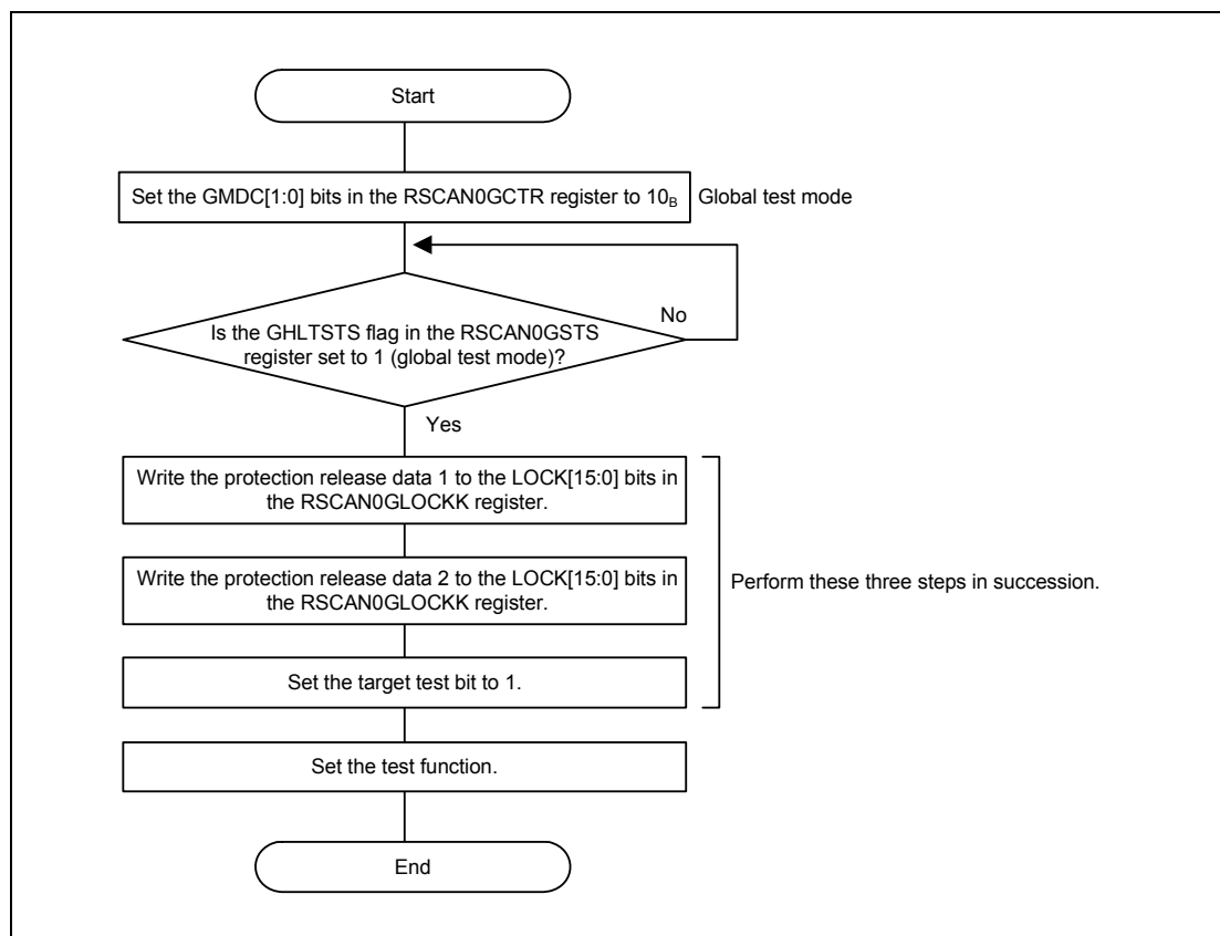
Figure 22.35 Protection Release Procedure
