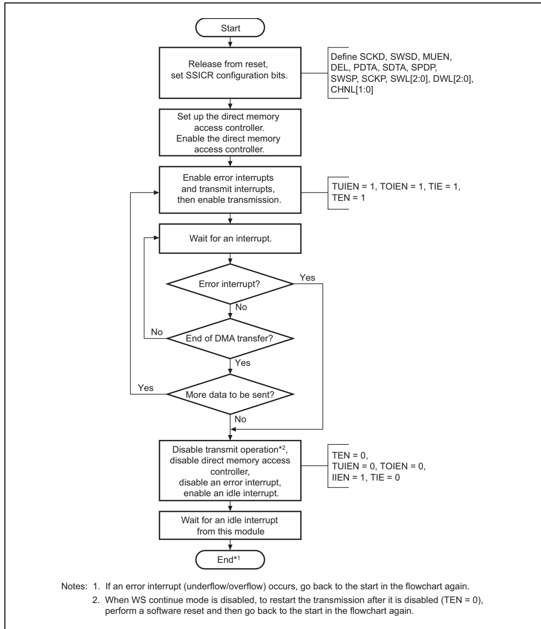
Figure 35.23 Transmission Using Direct Memory Access Controller
