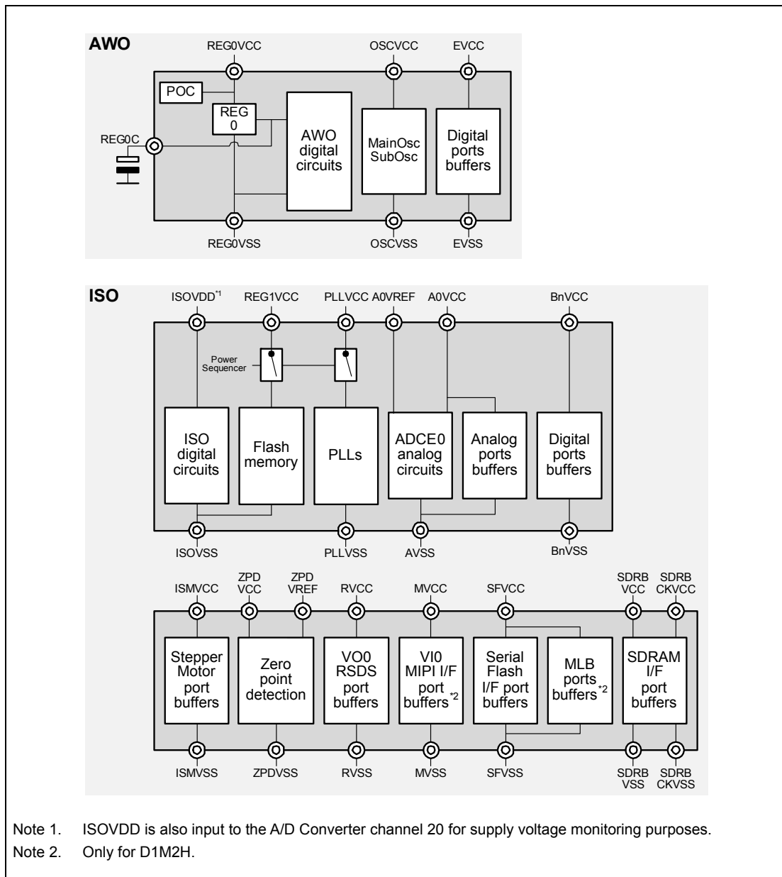
Figure 10.3 D1M2(H) power supply overview
