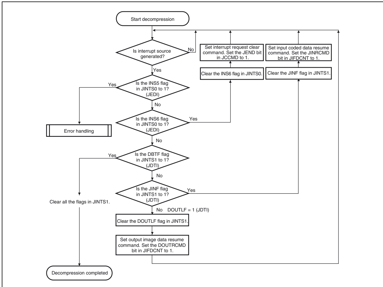
Figure 44.7 Decompression Process Flow
