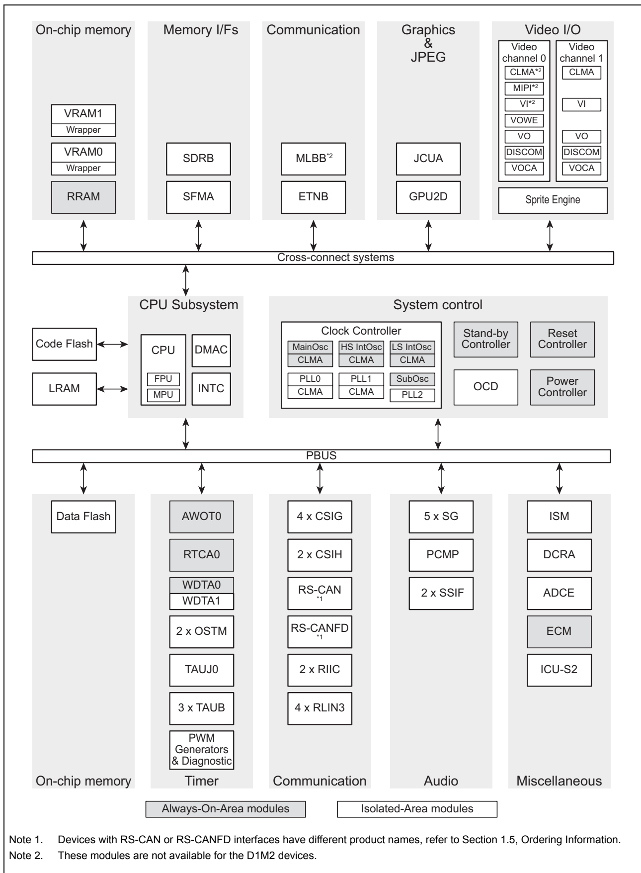
Figure 1.6 D1M2(H) block diagram
