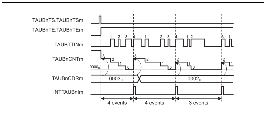
Figure 29.41 General Timing Diagram for External Event Count Function
