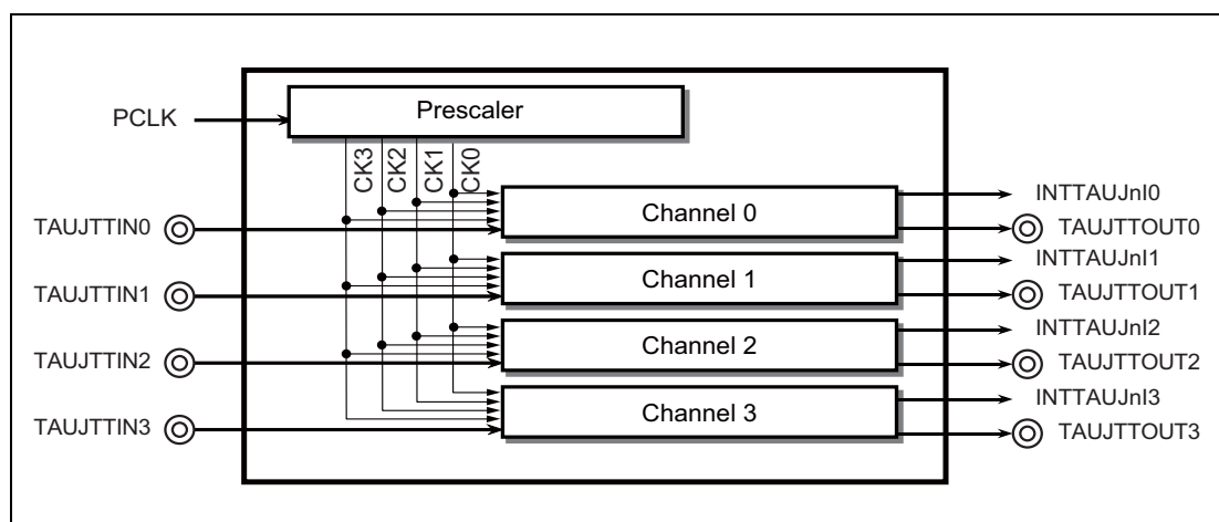
Figure 30.1 TAUJ I/O and Interrupt Request Signals
