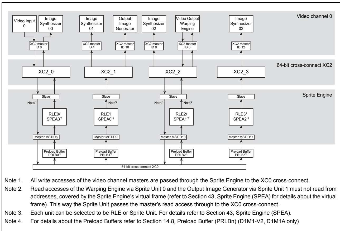
Figure 14.14 D1M1-V2 cross-connect XC2
