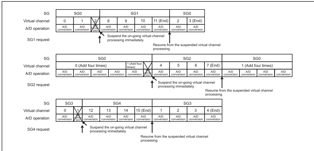
Figure 45.15 Example of Asynchronous Suspend and Resume Operation
