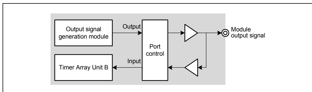
Figure 2.13 Port output check by timers
