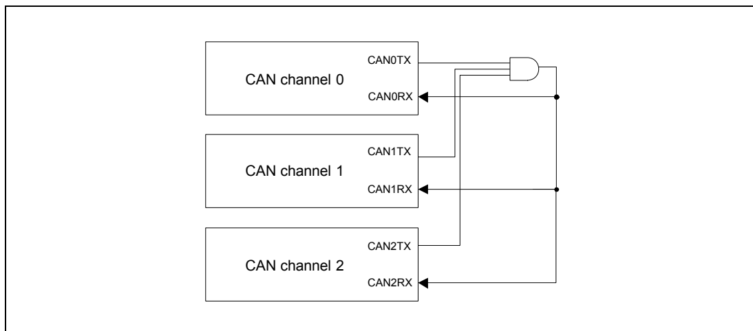
Figure 22.15 Connection for Inter-Channel Communication Test
