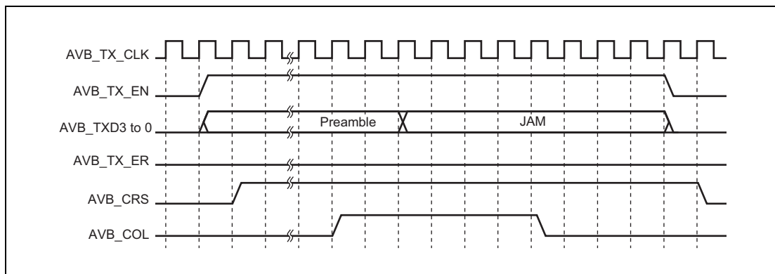
Figure 24.64 MII Frame Transmit Timing (Collision)
