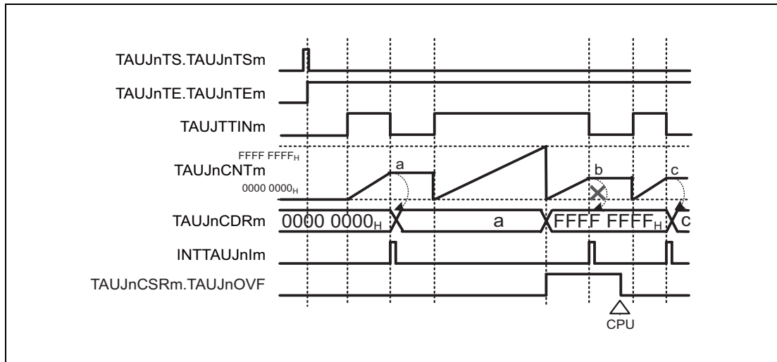
Figure 30.32 \text{TAUJnCMORm.TAUJnCOS}[1:0] = 11_{\text{B}} , \text{TAUJnCMORm.TAUJnMD0} = 0 , \text{TAUJnCMURm.TAUJnTIS}[1:0] = 11_{\text{B}}
