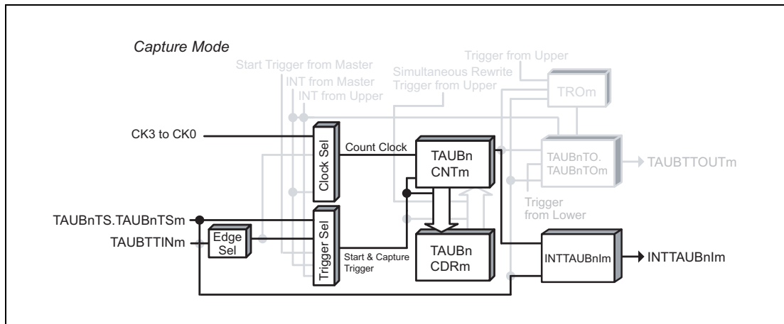
Figure 29.47 Block Diagram for TAUBTTINm Input Pulse Interval Measurement Function
