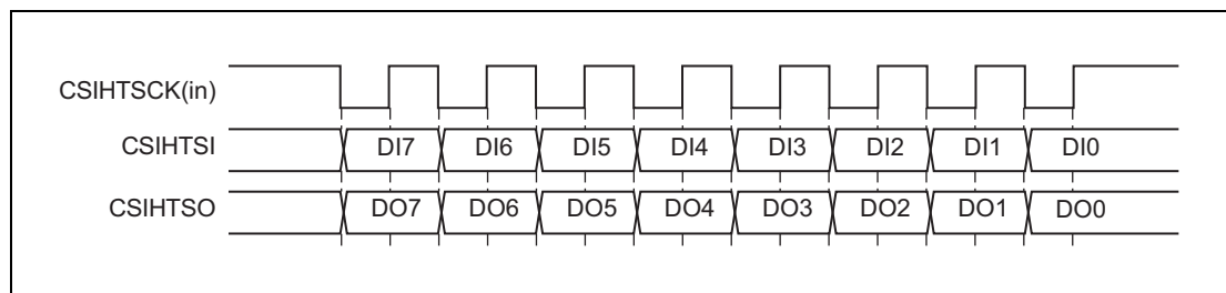
Figure 19.10 Transmit/Receive in Slave Mode
