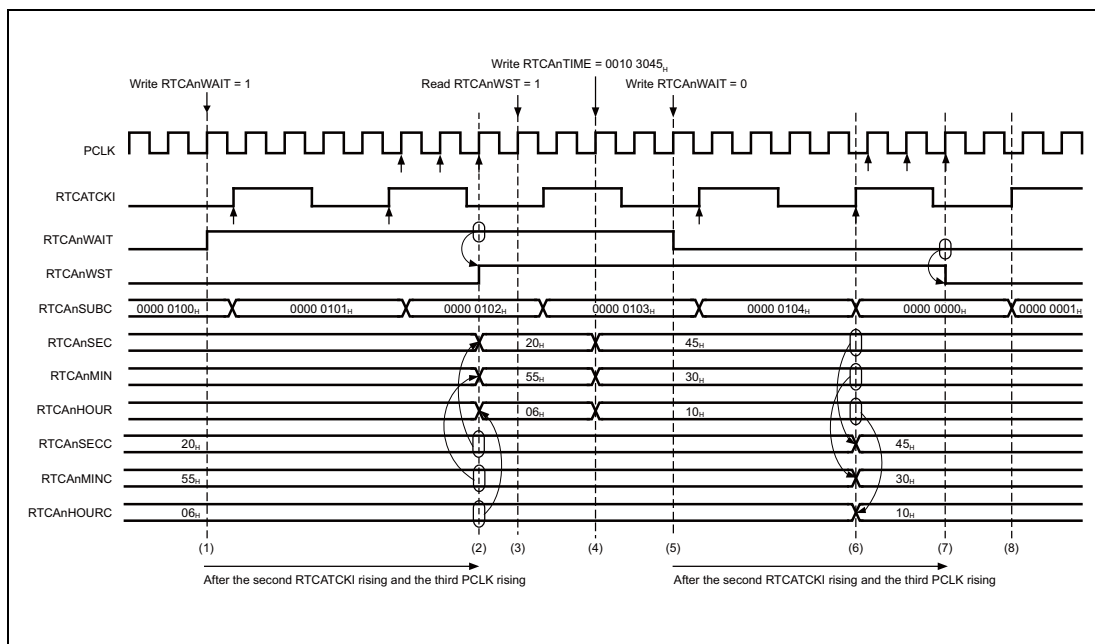
Figure 31.13 Clock Counter Update Timing
