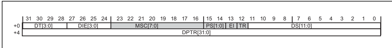
Figure 24.24 Configuration of Descriptor for a Received Frame
