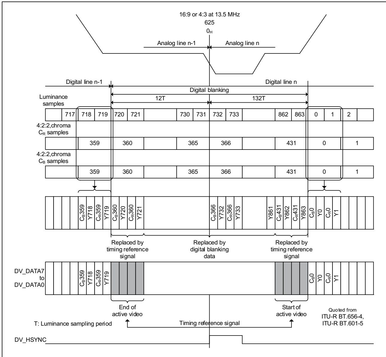
Figure 38.13 BT656 Horizontal Timing (625 Lines/50.00 Hz)
