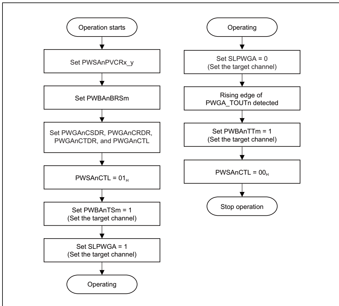
Figure 32.2 PWM-Diag Operating Procedure
