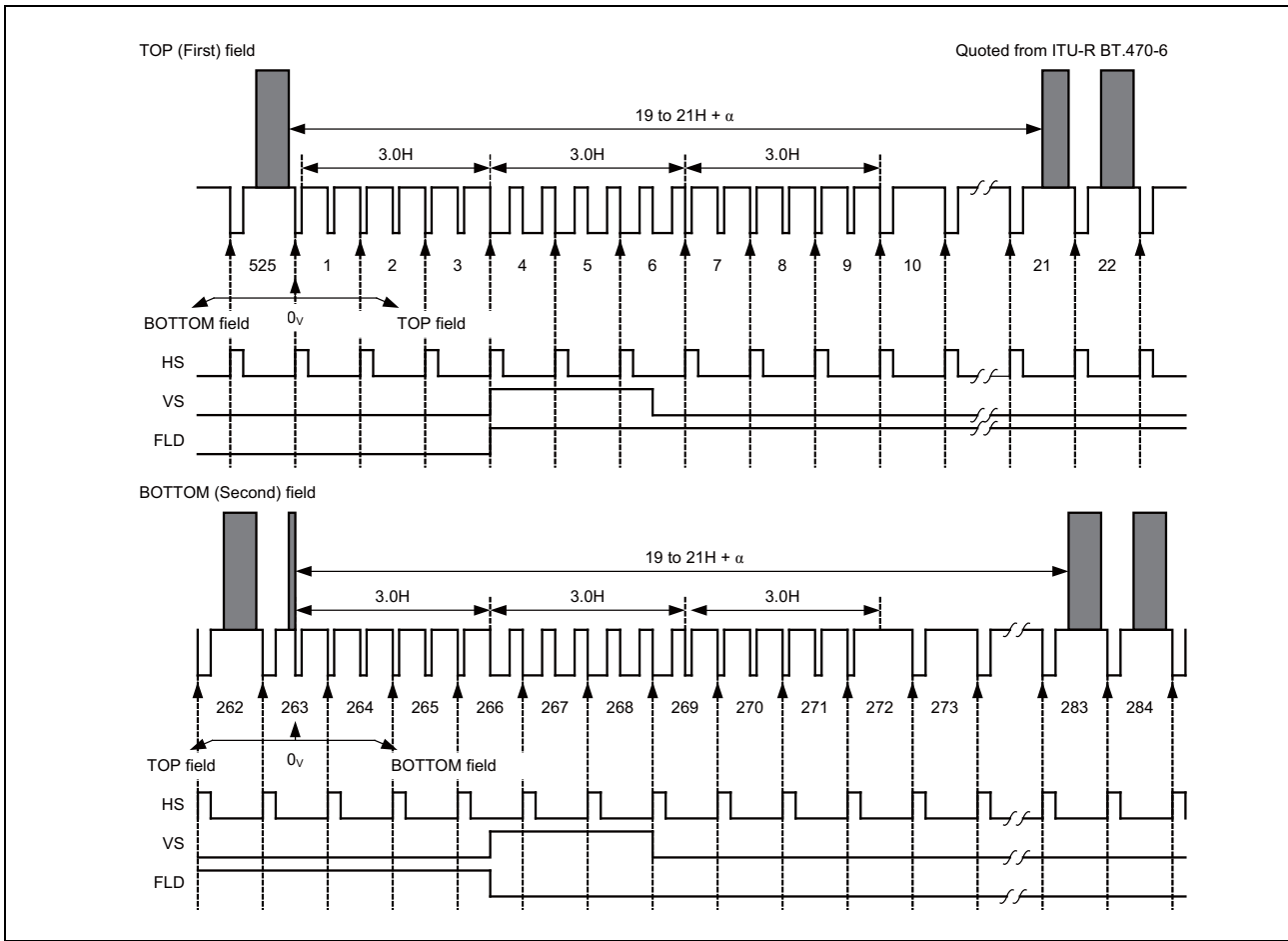
Figure 38.12 BT601 Vertical Timing (525 Lines/59.94 Hz)
