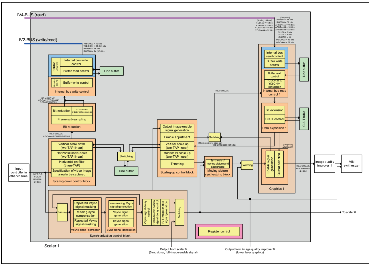
Figure 38.25 Functional Block Diagram of Scaler 1
