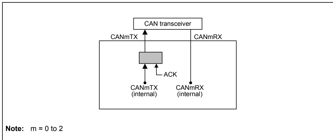
Figure 23.13 Connection when Self-Test Mode 0 is Selected
