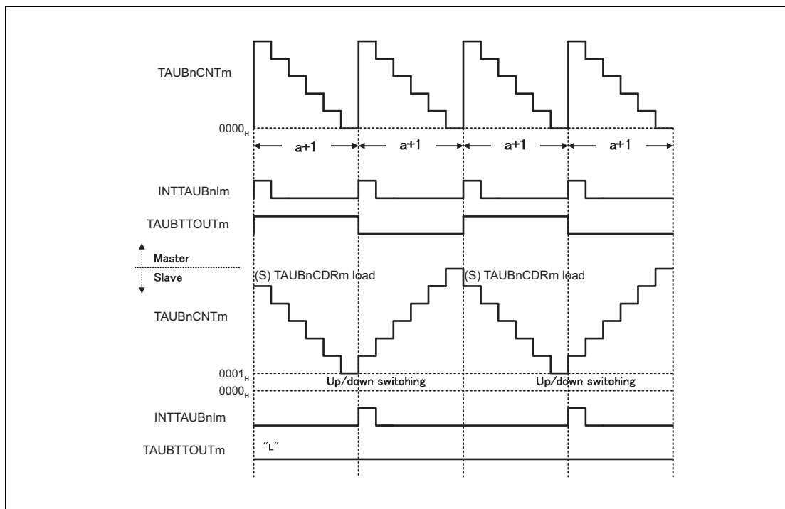
Figure 29.100 TAUBnCDRm (slave) \geq TAUBnCDRm (master) + 1
