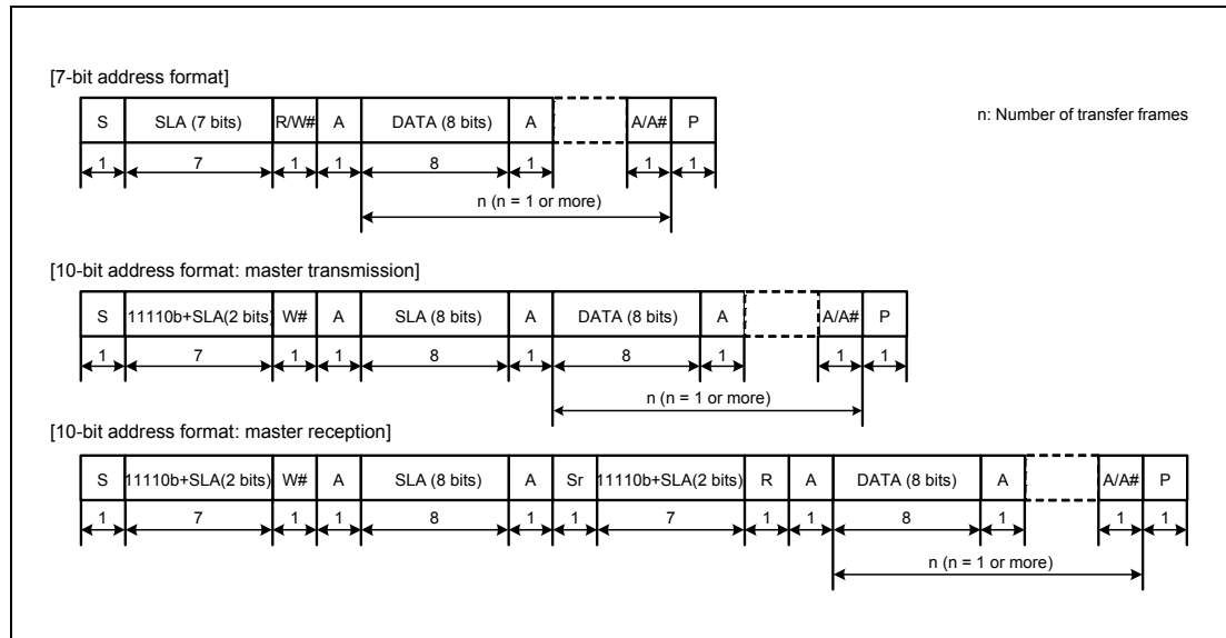
Figure 21.3 I 2 C Bus Format
