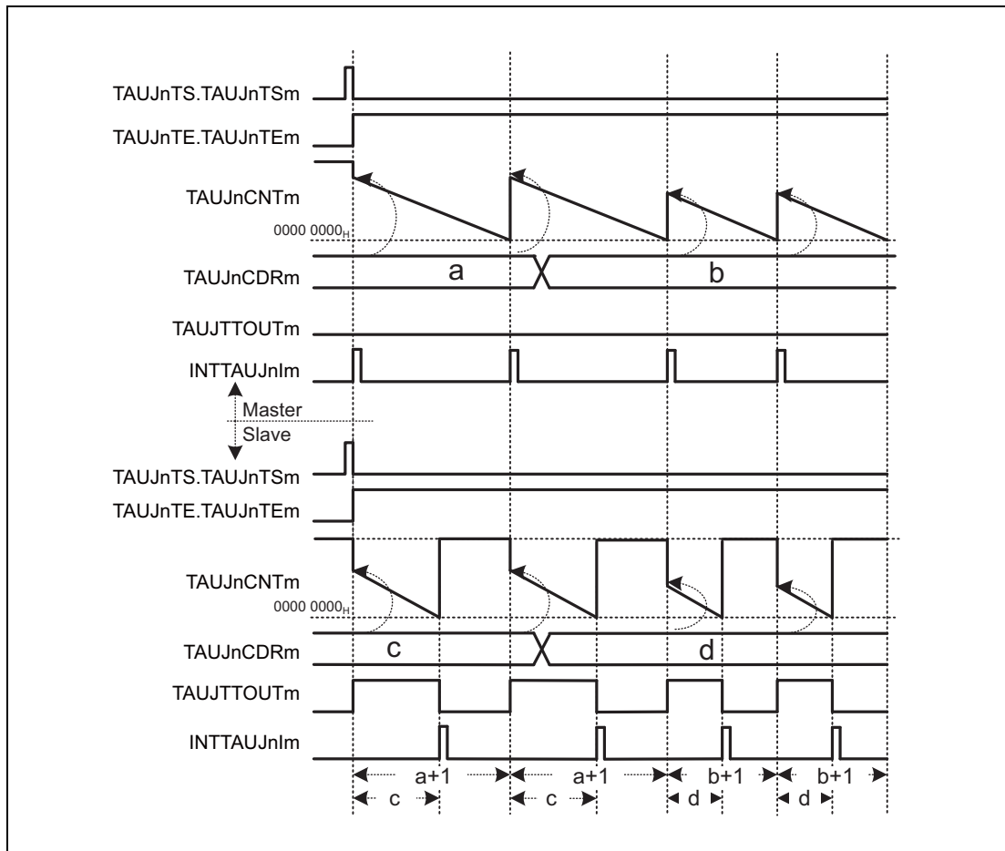
Figure 30.44 General Timing Diagram for PWM Output Function
