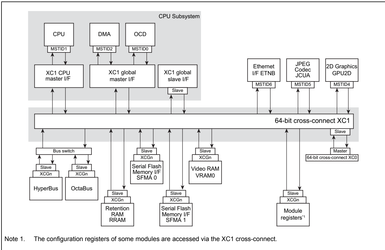
Figure 14.13 D1M1-V2 cross-connect XC1
