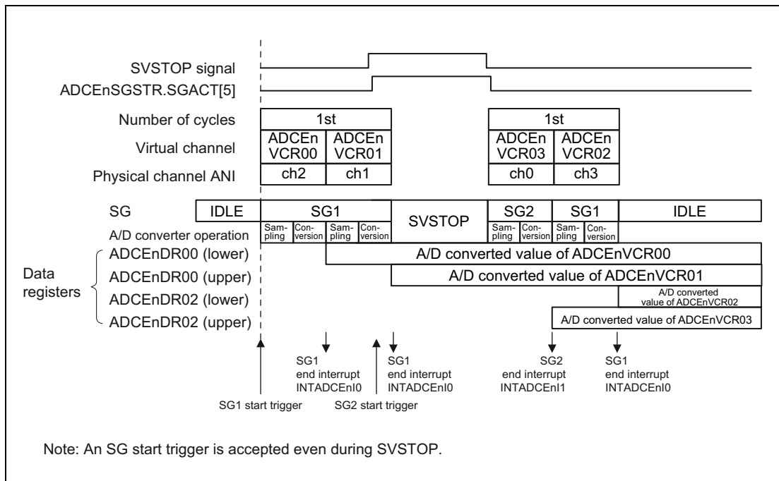
Figure 45.19 Conflict of SVSTOP Start and High-Priority SG Start Trigger (ADCEnADCR.SUSMTD[1:0] = 00, ADCEnEMU.SVSDIS = 0)
