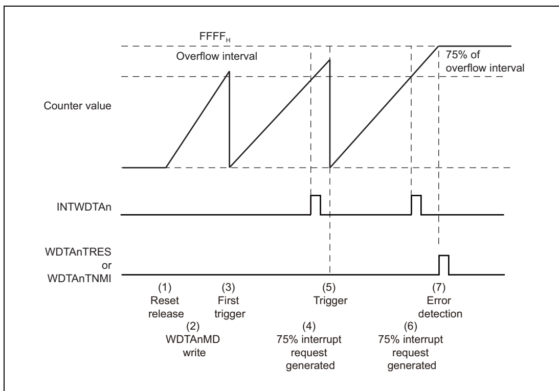
Figure 26.5 Timing Diagram of WDTA 75% Interrupt Request Signals
