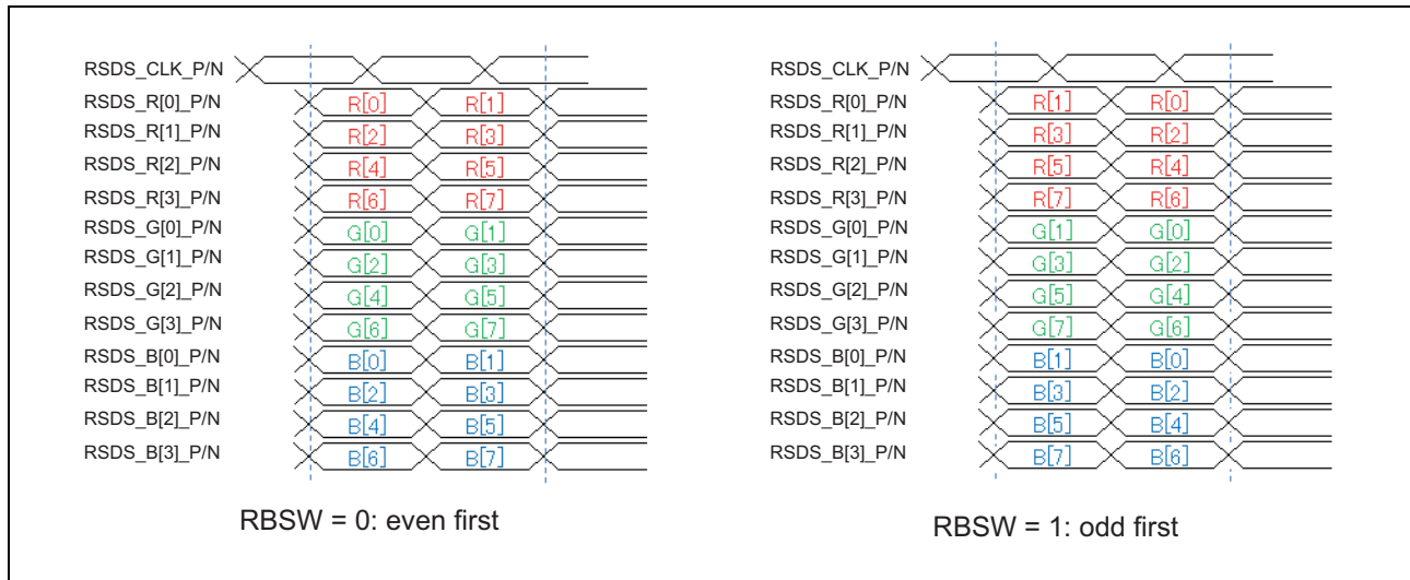
Figure 37.25 RSDS data bitswap
