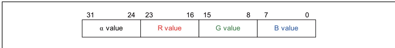
Figure 38.54 Data Arrangement in CLUT Table
