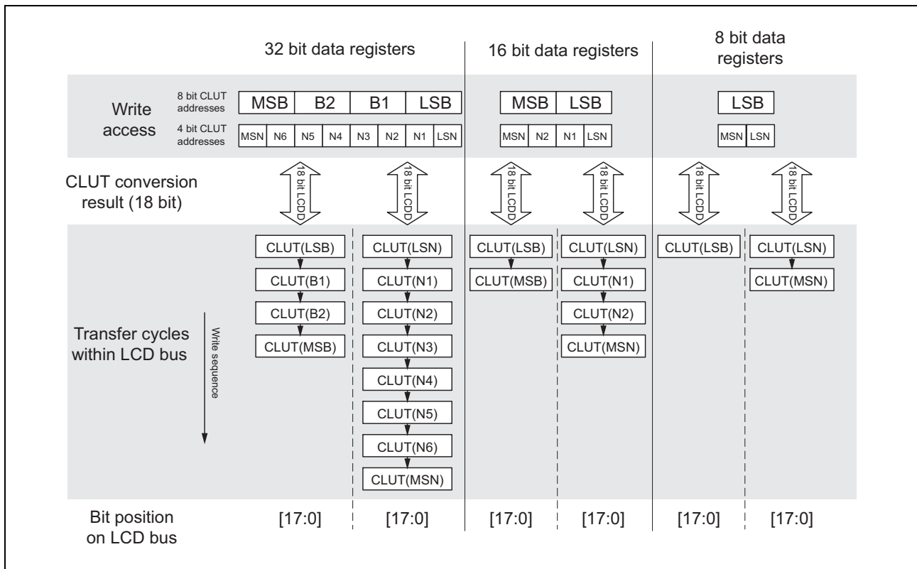
Figure 36.9 Data transfer types with CLUT usage on 18-bit LCD bus
