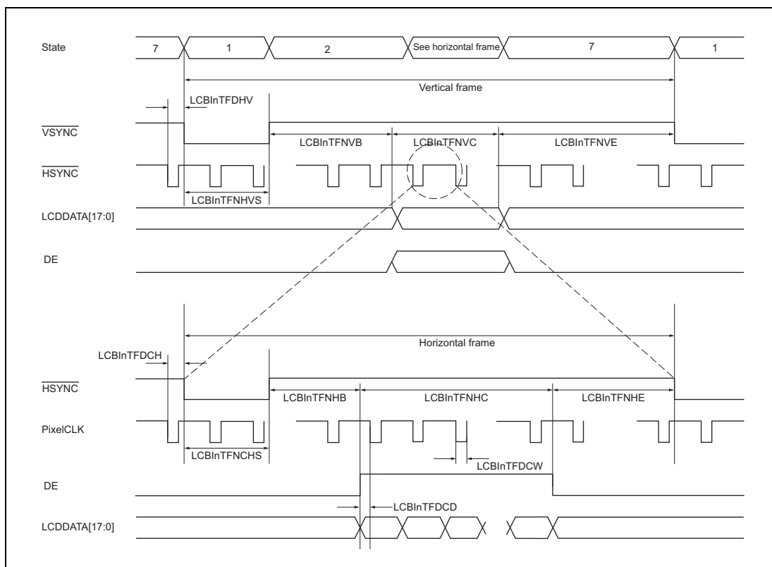
Figure 36.6 TFT operation mode general timing
