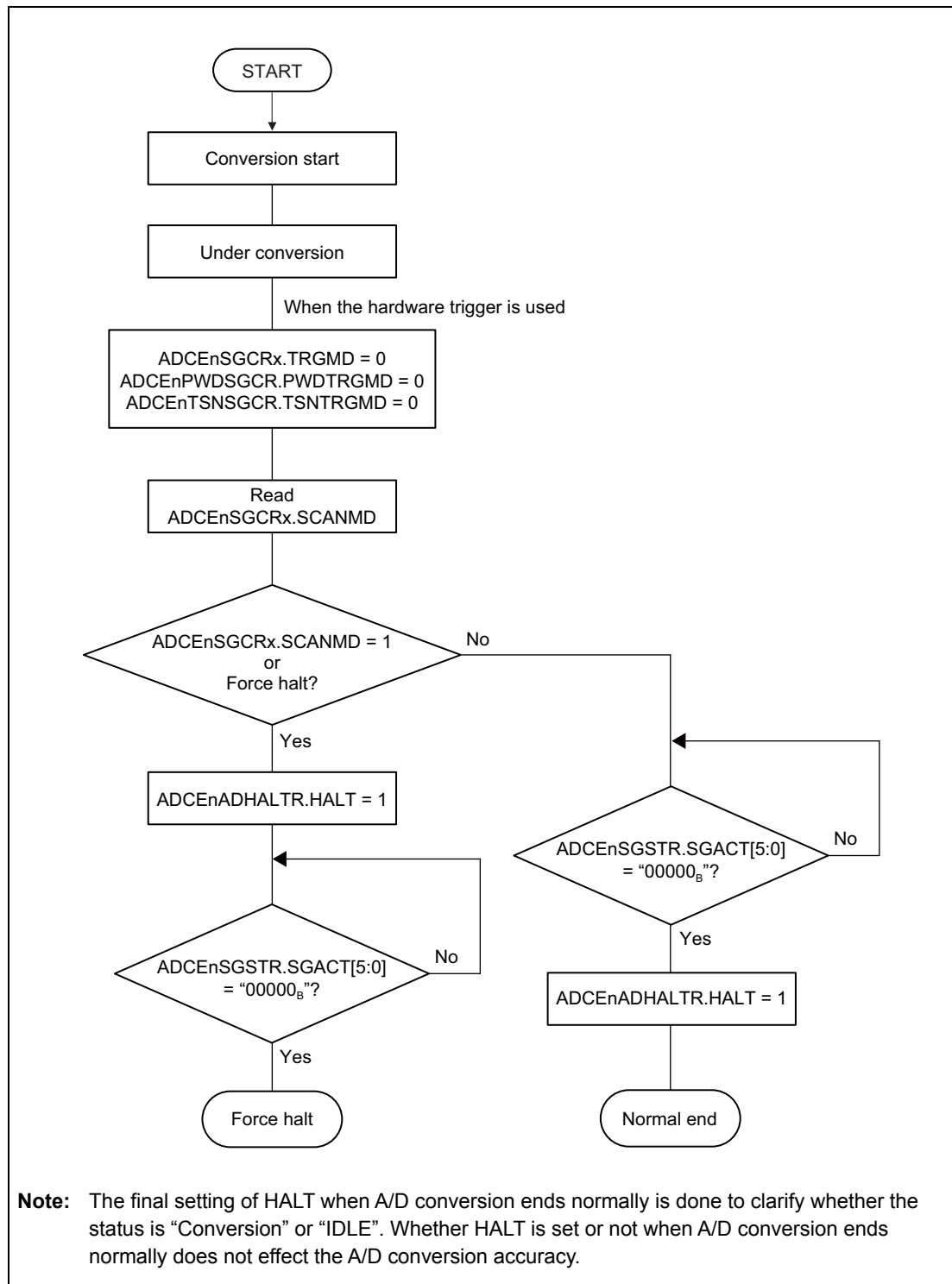
Figure 45.6 Flow at the End of A/D Conversion
