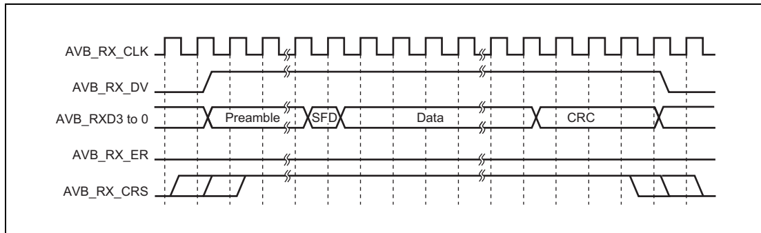
Figure 24.69 MII Fame Receive Timing (Normal Reception)
