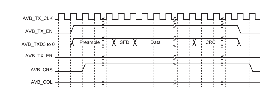
Figure 24.63 MII Frame Transmit Timing (Normal Transmission)
