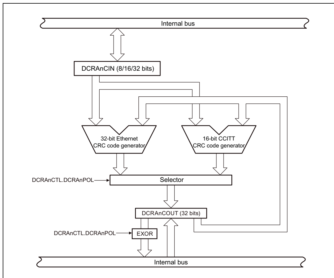
Figure 49.1 Block Diagram of Data CRC Function A
