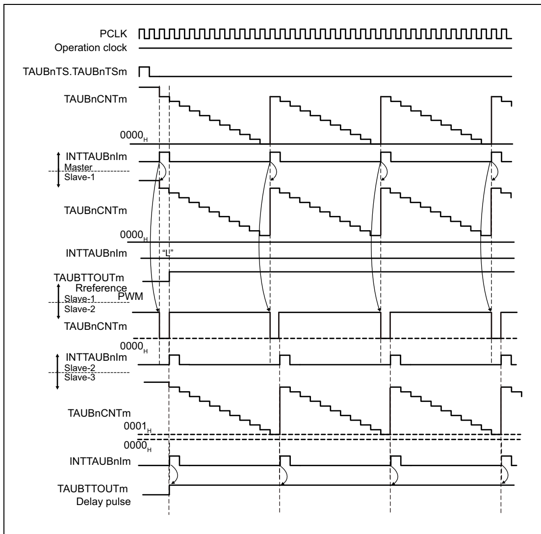
Figure 29.94 Duty Cycle (slave 3) = 100%
