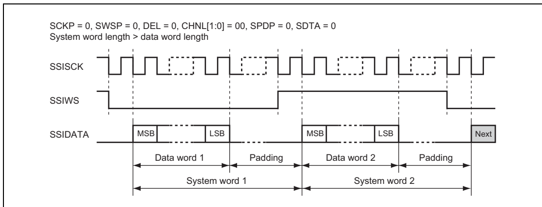
Figure 35.3 I 2 S Compatible Format (with Padding)
