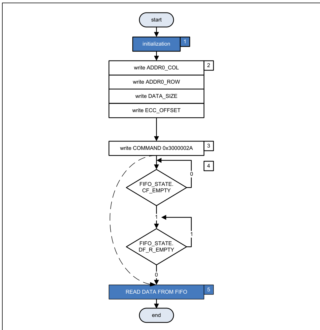
Figure 58.37 Reading Partial Pages
