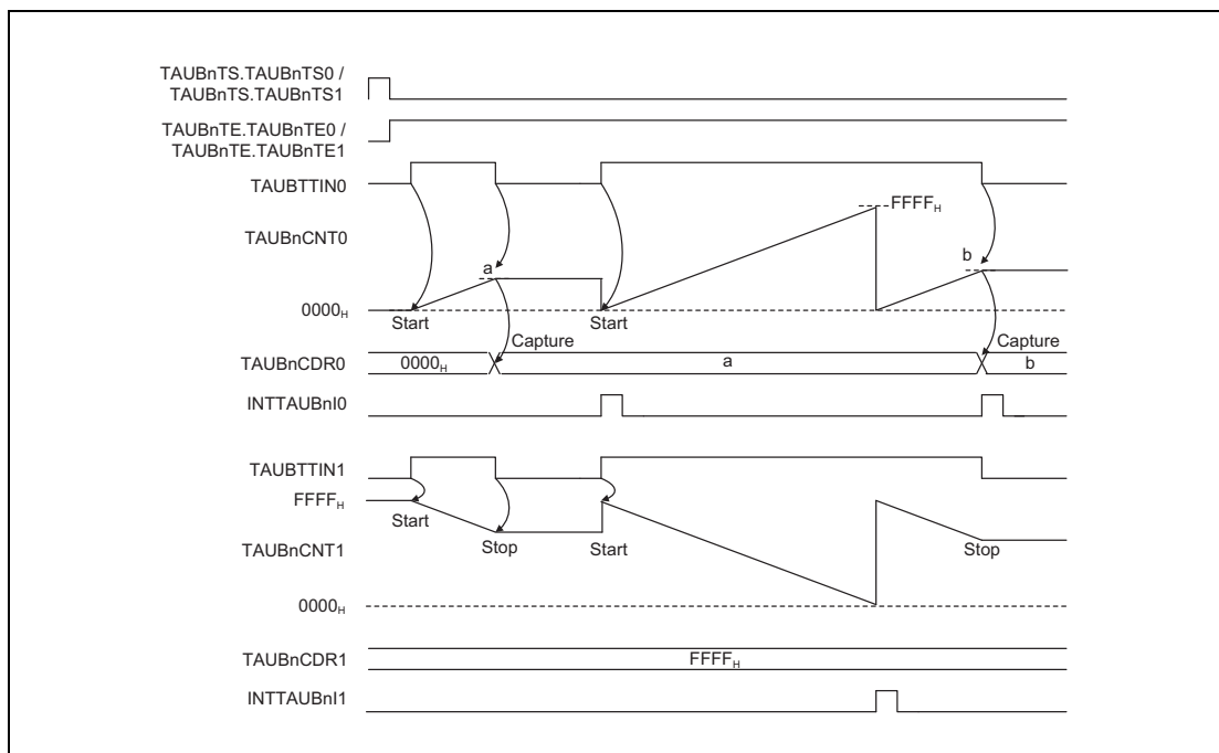
Figure 29.18 Interrupt Generation by Combination of TAUBTTINm Input Signal Width Measurement Function and Overflow Interrupt Output Function (during TAUBTTINm Width Measurement)
