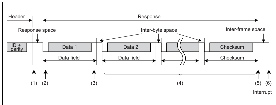
Figure 20.6 Operation in Response Reception
