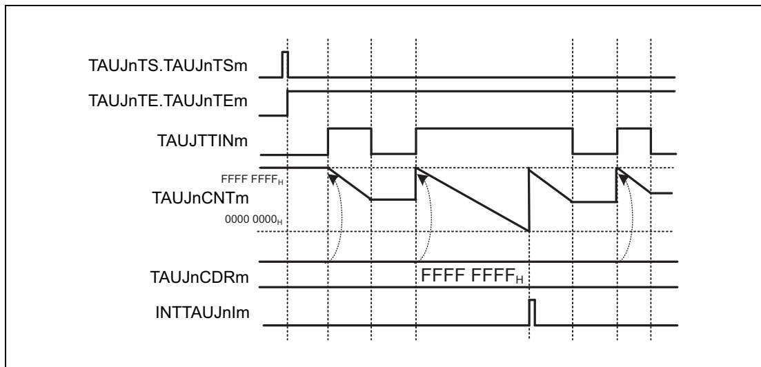
Figure 30.40 General Timing Diagram for Overflow Interrupt Output Function (during TAUJTTINm Width Measurement)
