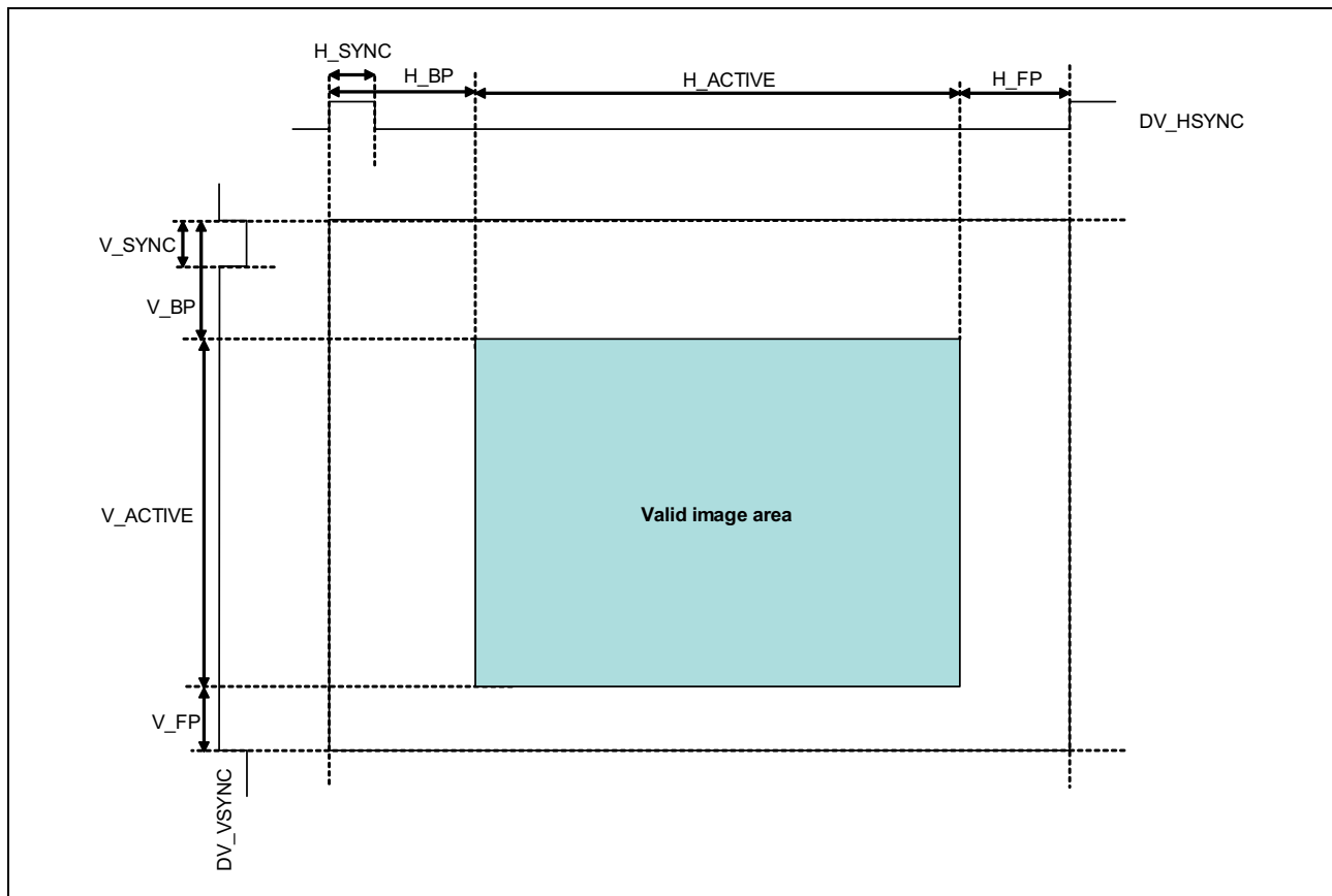
Figure 38.20 YCbCr/RGB Signal Reception Timing
