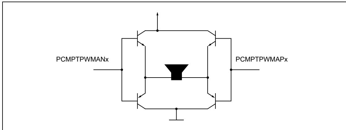
Figure 34.8 Driving a half H-bridge (here: emitter follower bridge)
