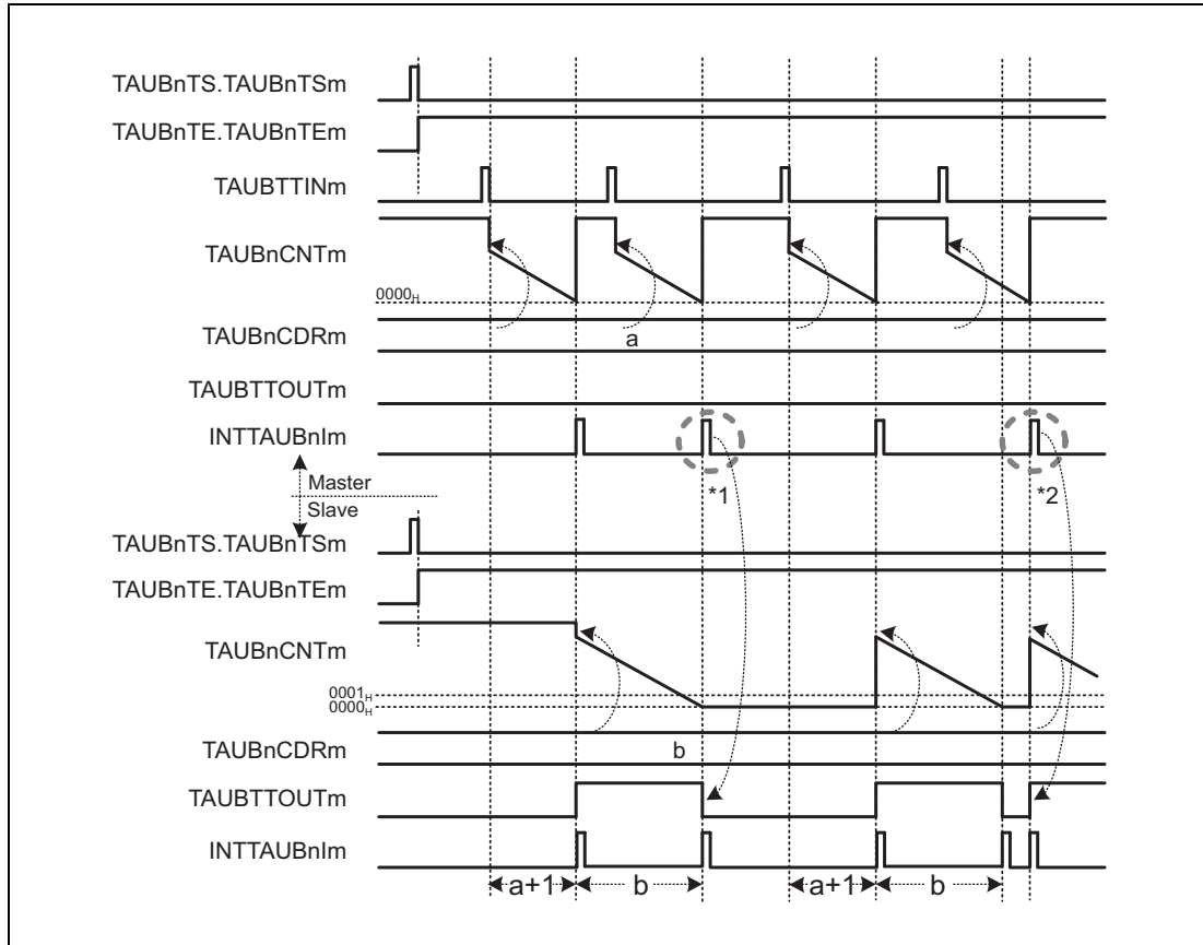
Figure 29.91 Interval of TAUBTTINm ≤ Delay Time + Pulse Width + 1
