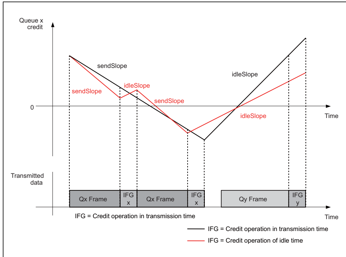
Figure 24.46 Credit Operations during IFGs
