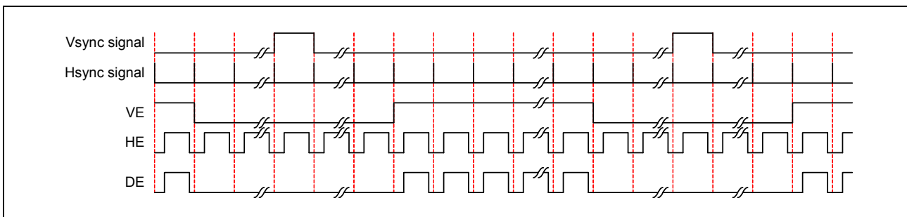
Figure 38.80 Data Enable Signal Generation
