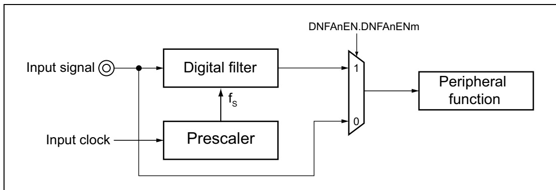
Figure 2.18 Block Diagram of Digital Filter Type C
