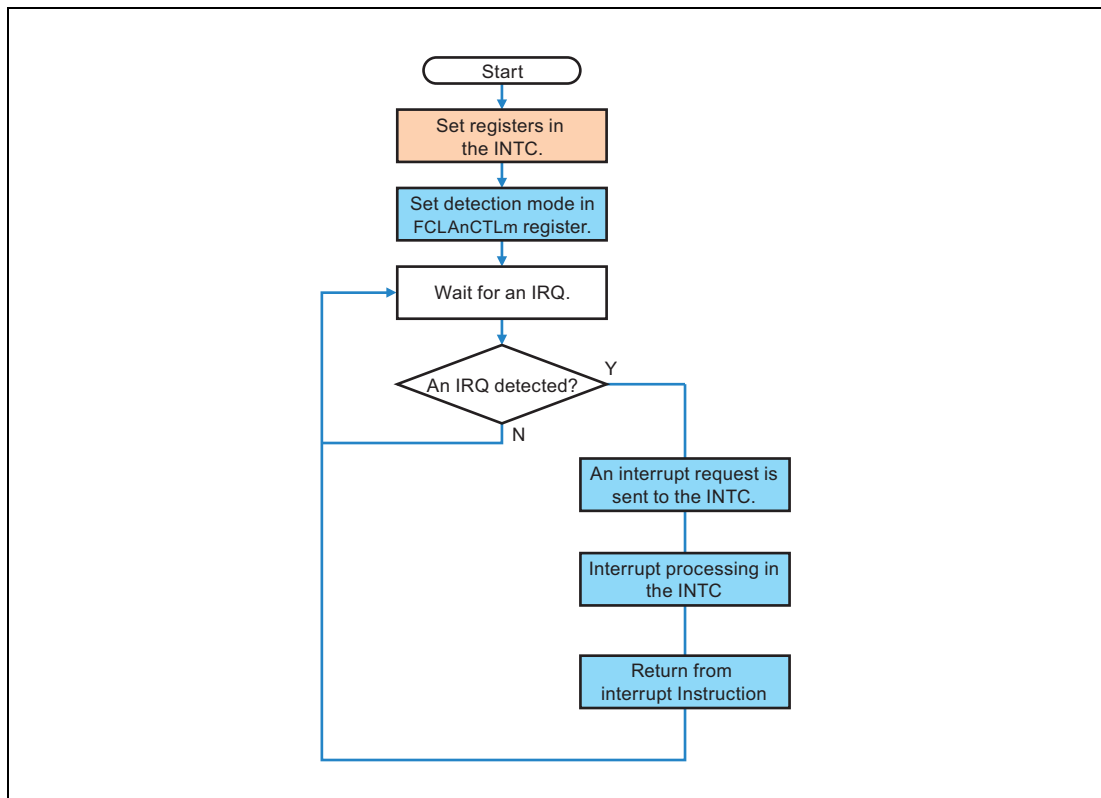
Figure 7.1 External Interrupt Processing Flow
