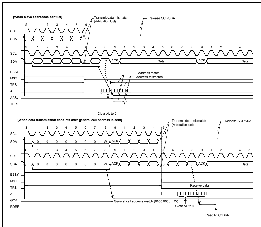
Figure 21.32 Examples of Master Arbitration-Lost Detection (MALE = 1)
