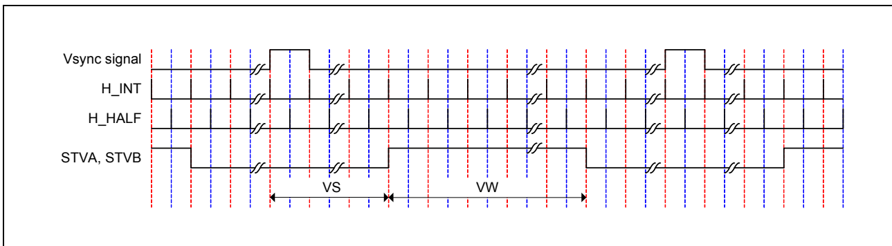
Figure 38.77 Vertical Panel Driver Signal (H_INT Reference Operation)
