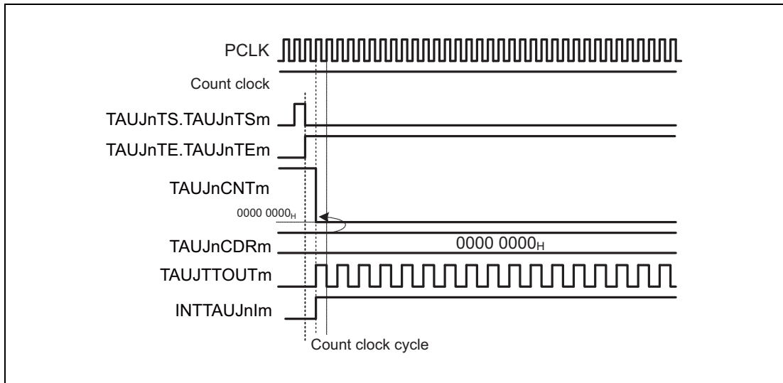
Figure 30.15 TAUJnCDRm = 0000 0000 H , Count Clock = PCLK
