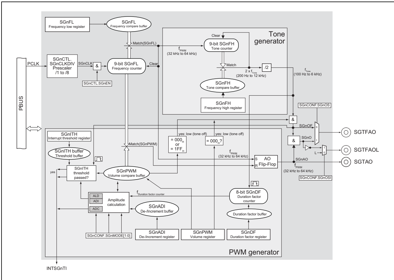
Figure 33.1 Sound Generator block diagram
