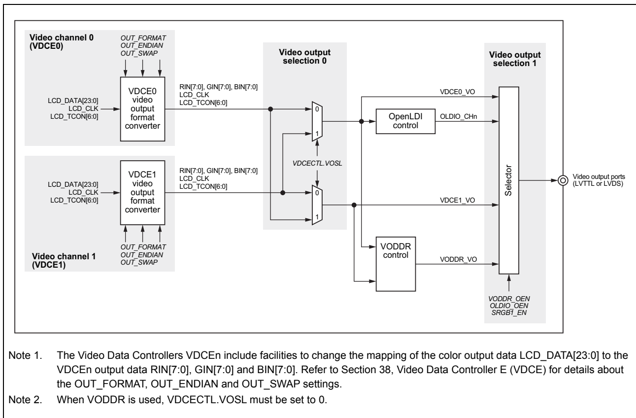
Figure 37.22 D1M1A video output selections
