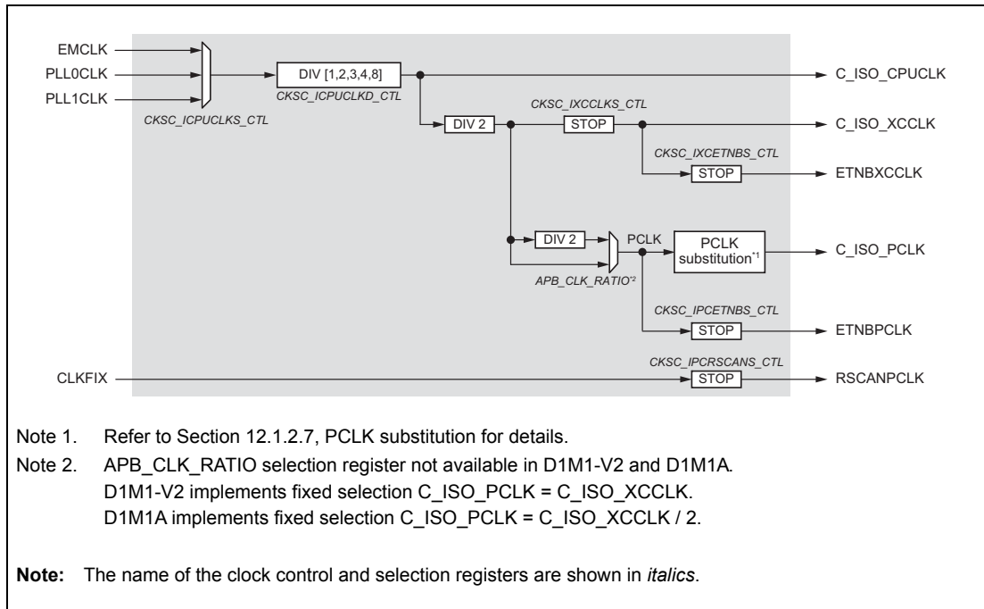
Figure 12.8 D1M1(H), D1M1-V2, D1M1A CPU and bus subsystems clock domains
