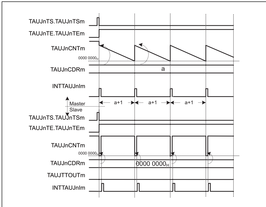
Figure 30.45 TAUJnCDRm (slave) = 0000 0000 H , Positive Logic (TAUJnTOL.TAUJnTOLm (slave) = 0)
