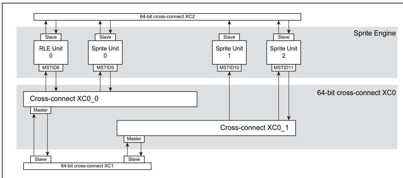
Figure 14.8 D1M1(H) cross-connect XC0
