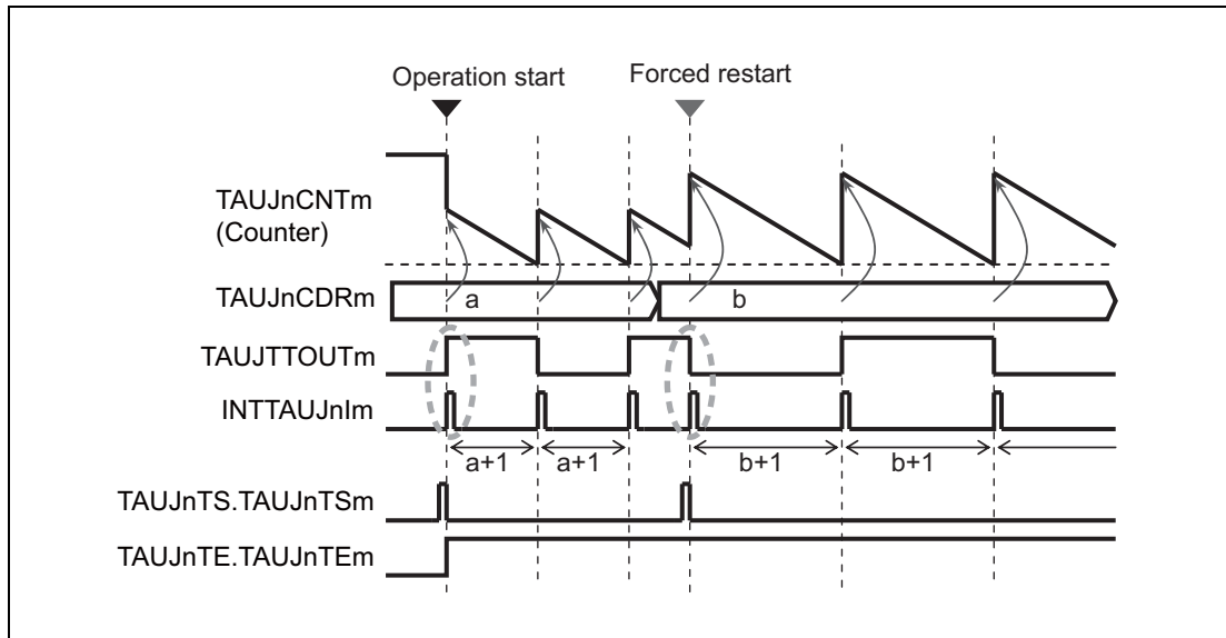
Figure 30.17 Forced Restart Operation (TAUJnCMORm.TAUJnMD0 = 1)
