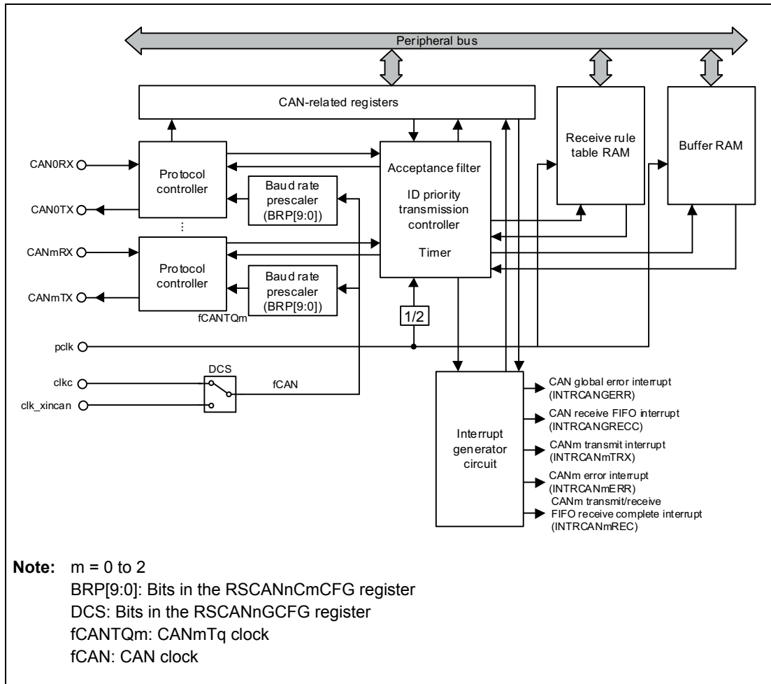
Figure 23.1 RS-CANFD module Block Diagram (Classical CAN Mode)
