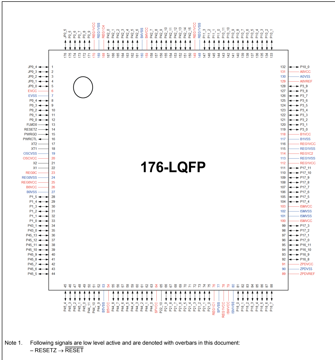
Figure 2.3 D1M1-V2 pin connection diagram (176 pins LQFP package)
