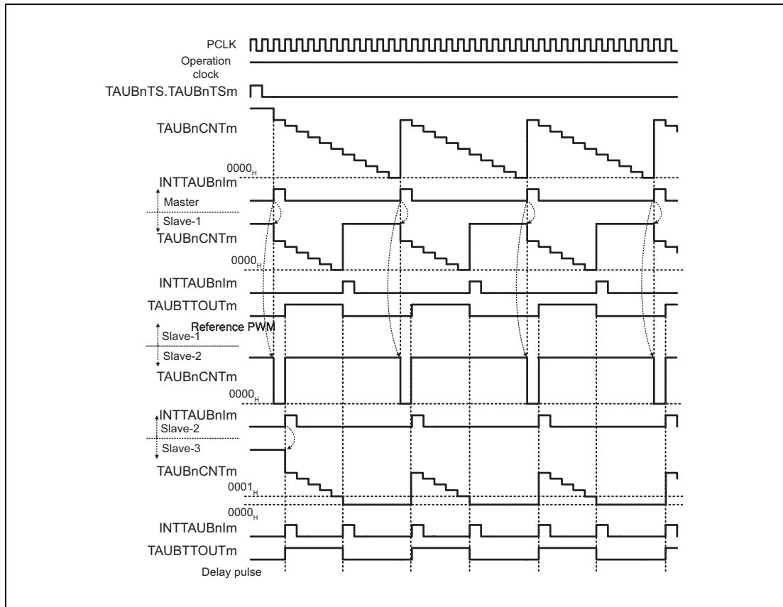
Figure 29.95 TAUBTTOUTm (slave 1) = TAUBTTOUTm (slave 3)
