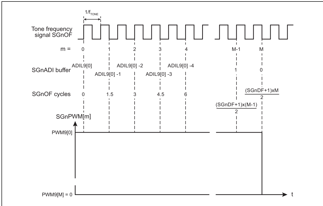
Figure 33.12 ADC mode timing
