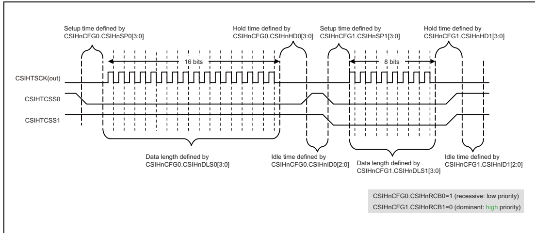
Figure 19.14 Chip Select and RCB Example
