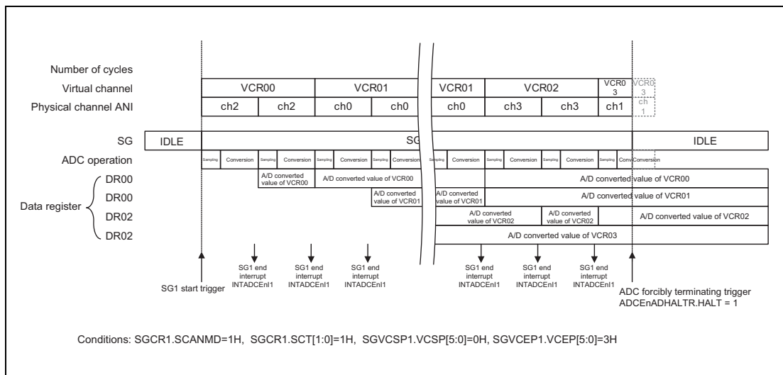
Figure 45.12 Example of Channel Repeat Operation 3
