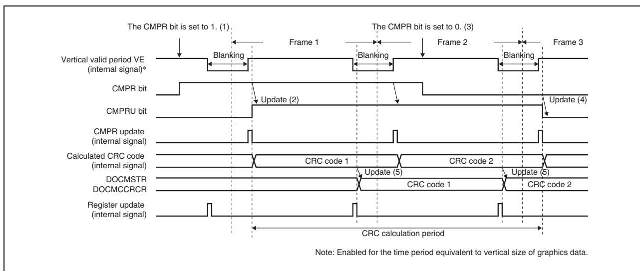
Figure 41.6 Register Update Timing
