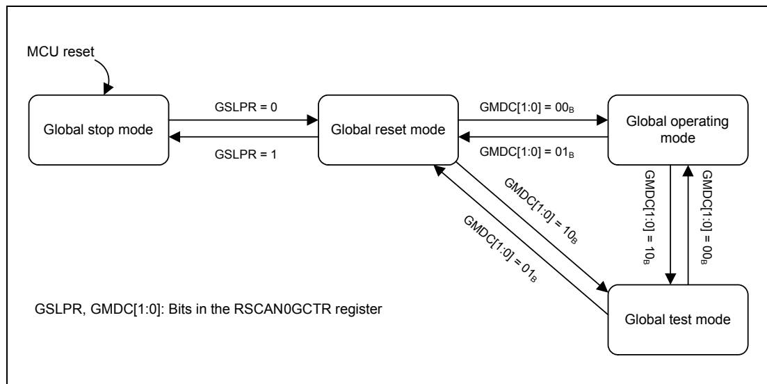
Figure 22.4 Transitions of Global Modes
