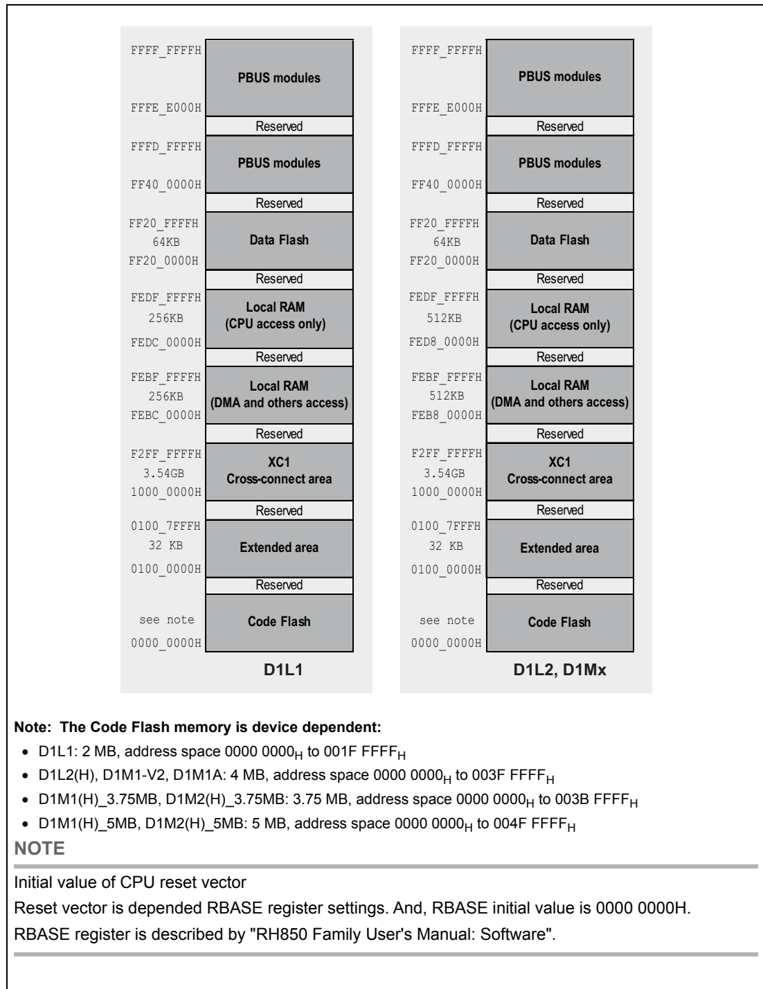
Figure 5.1 CPU address map
