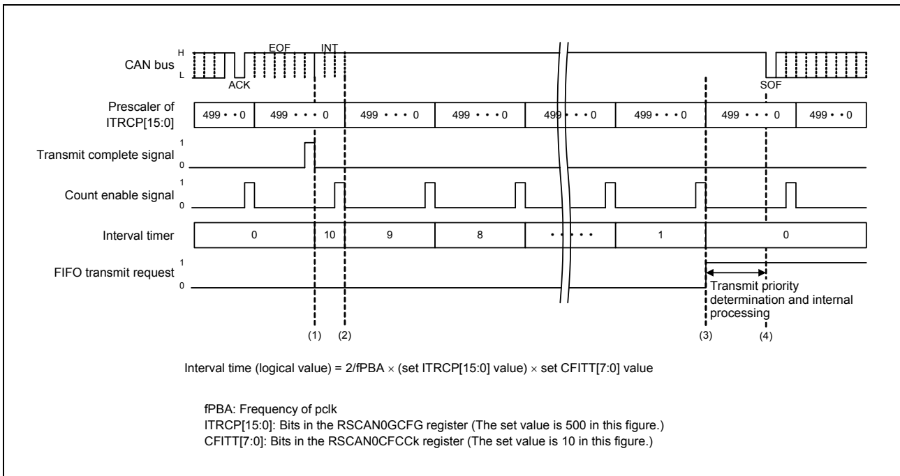
Figure 22.11 Interval Timer Timing Chart
