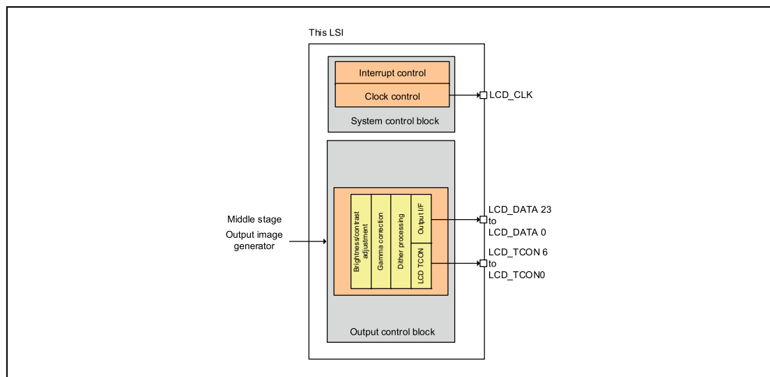
Figure 38.3 Video Display Controller Latter Stage Block Diagram
