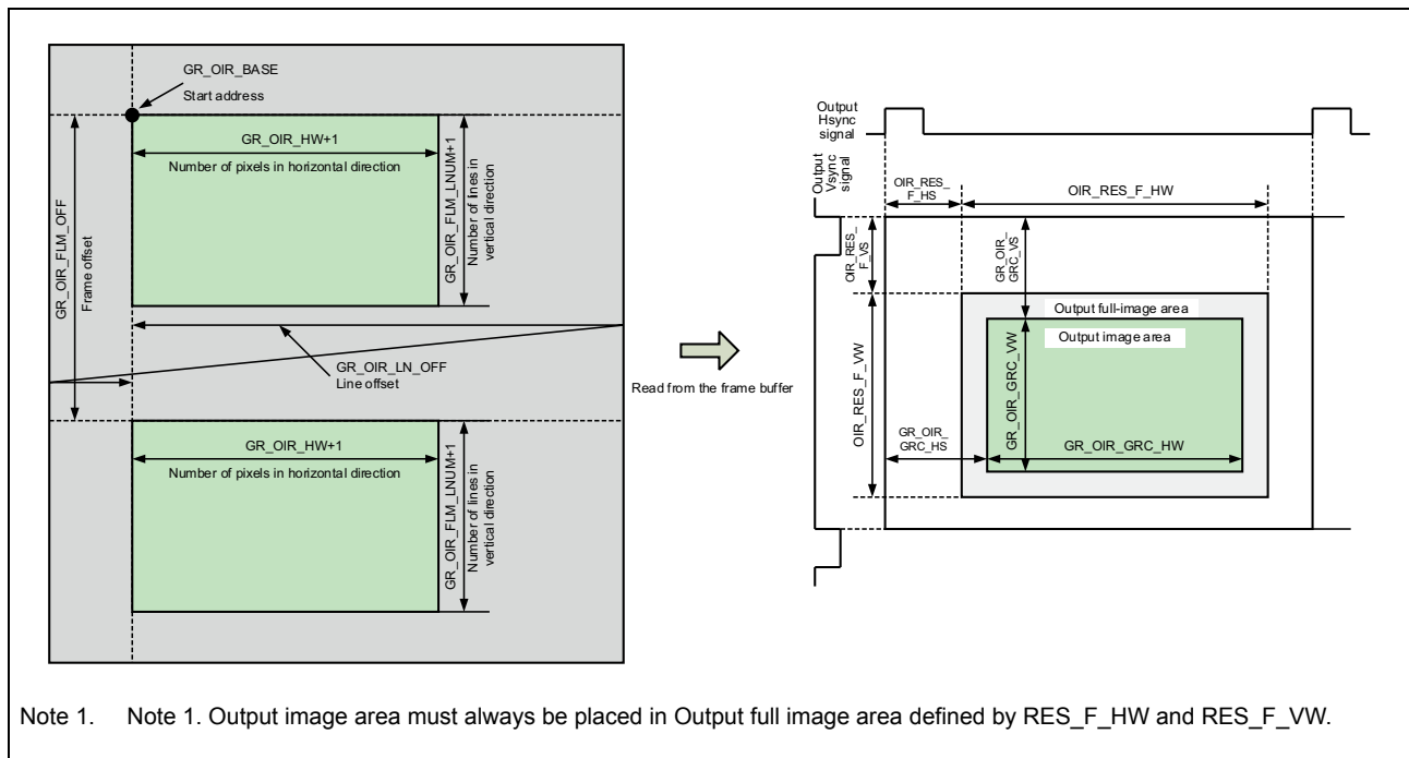
Figure 38.59 Area Setting for Graphics Display
