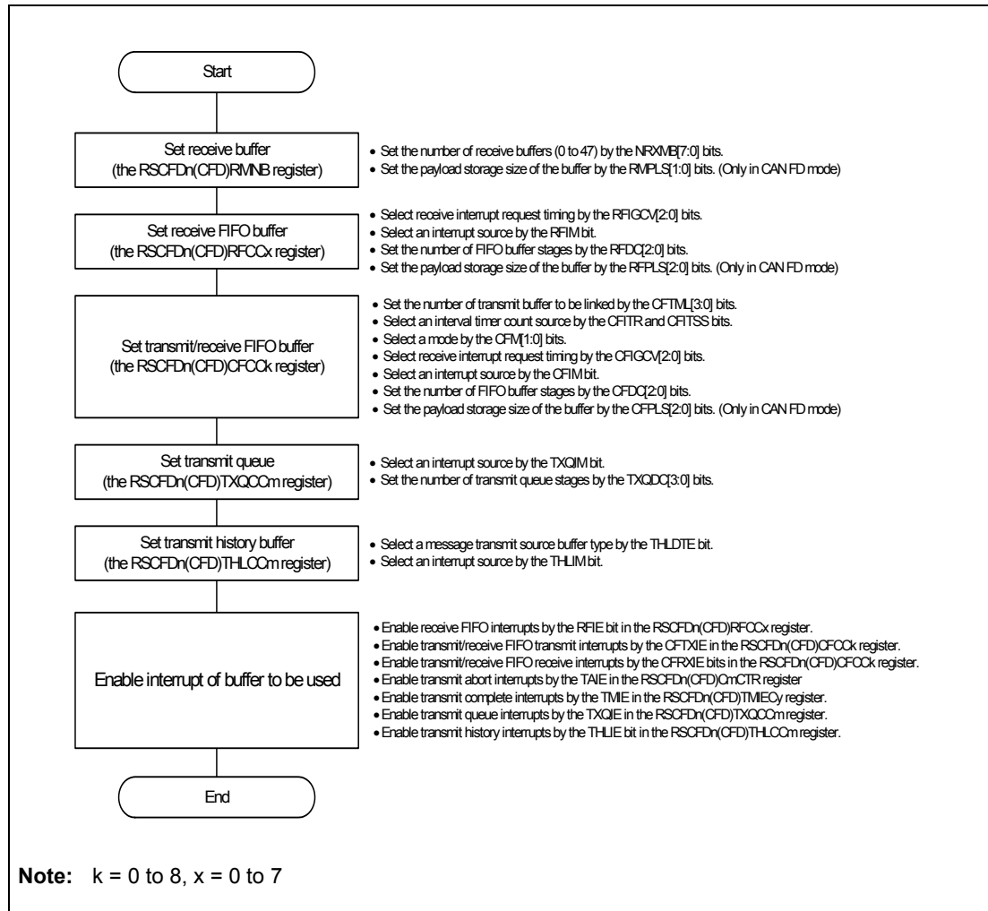
Figure 23.21 Buffer Setting Procedure
