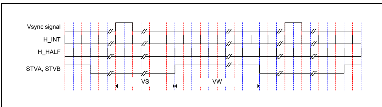
Figure 38.78 Vertical Panel Driver Signal (H_HALF Reference Operation)
