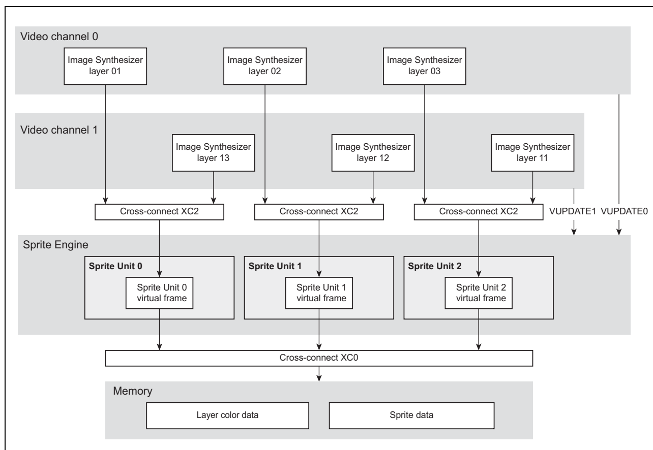
Figure 43.9 Sprite Units block diagram
