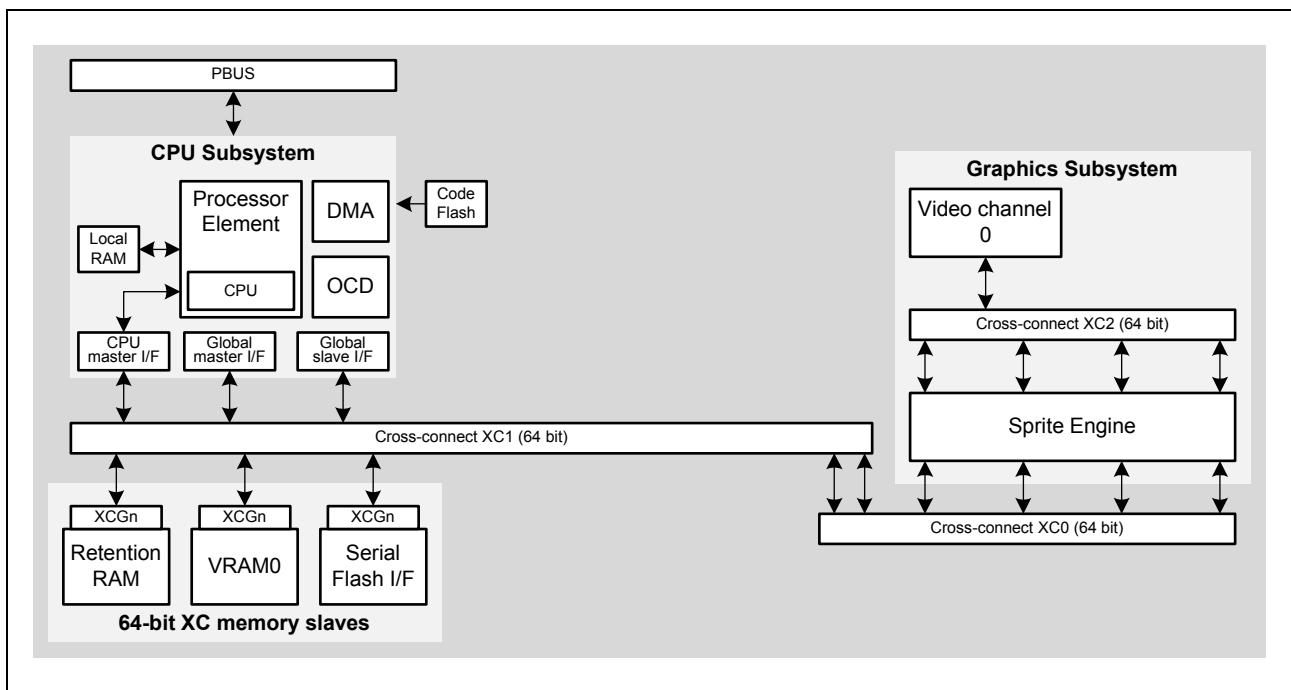
Figure 14.3 D1L2(H) bus architecture overview
