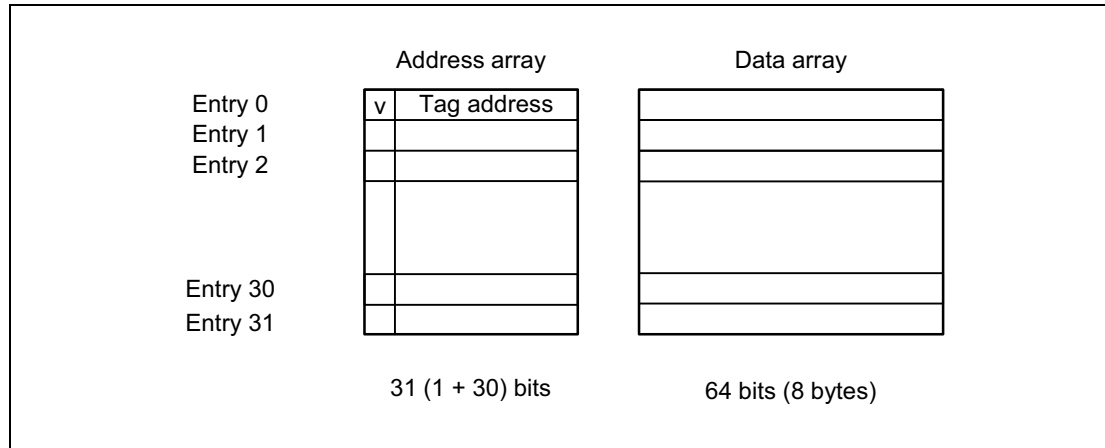
Figure 56.4 Read cache configuration
