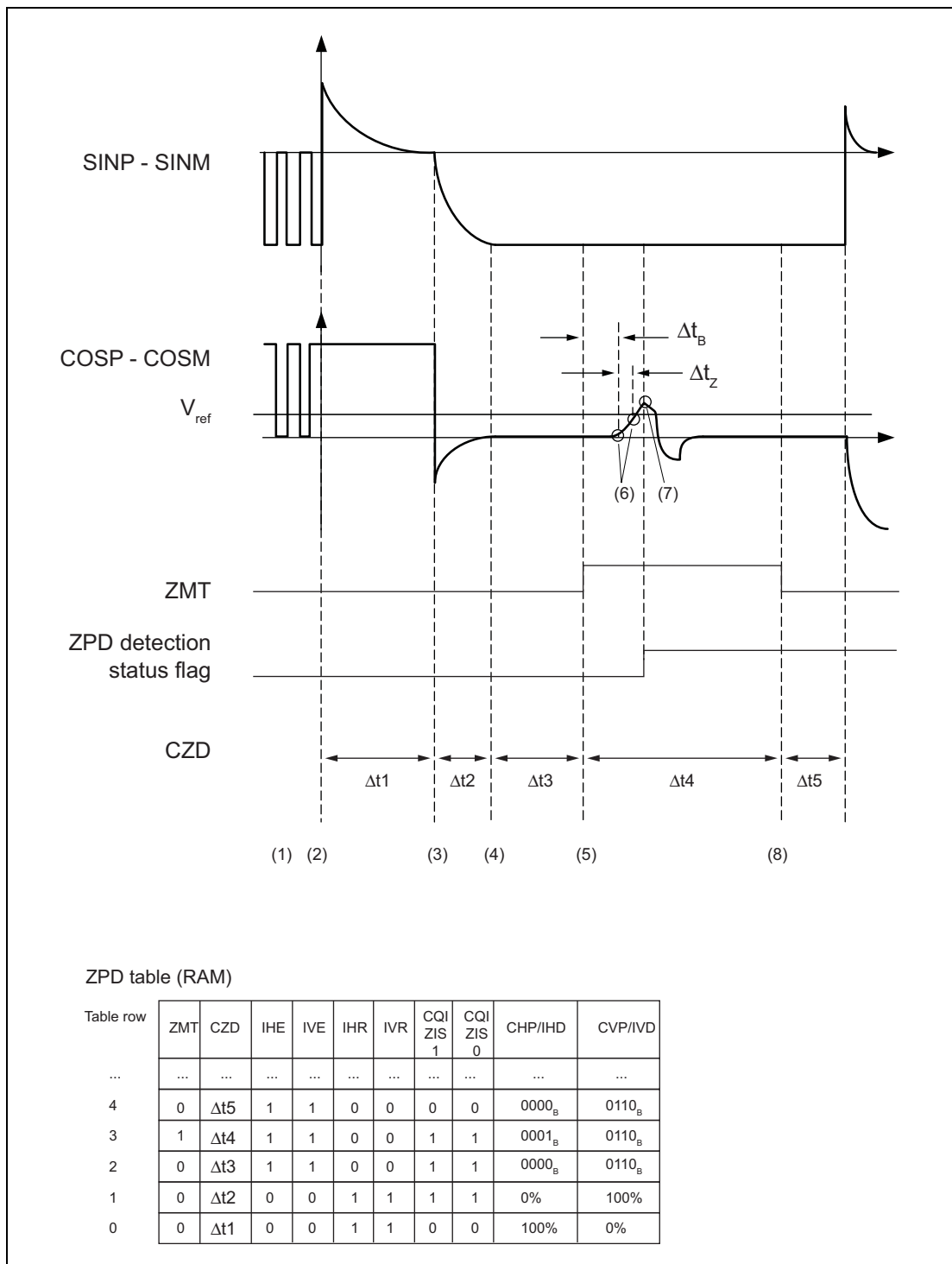
Figure 46.19 Timing of ZPD measurements with channel management
