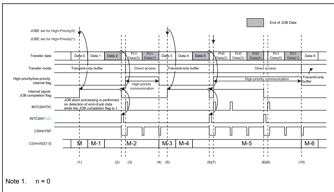
Figure 19.46 Example of CPU-Controlled High-Priority Communication
