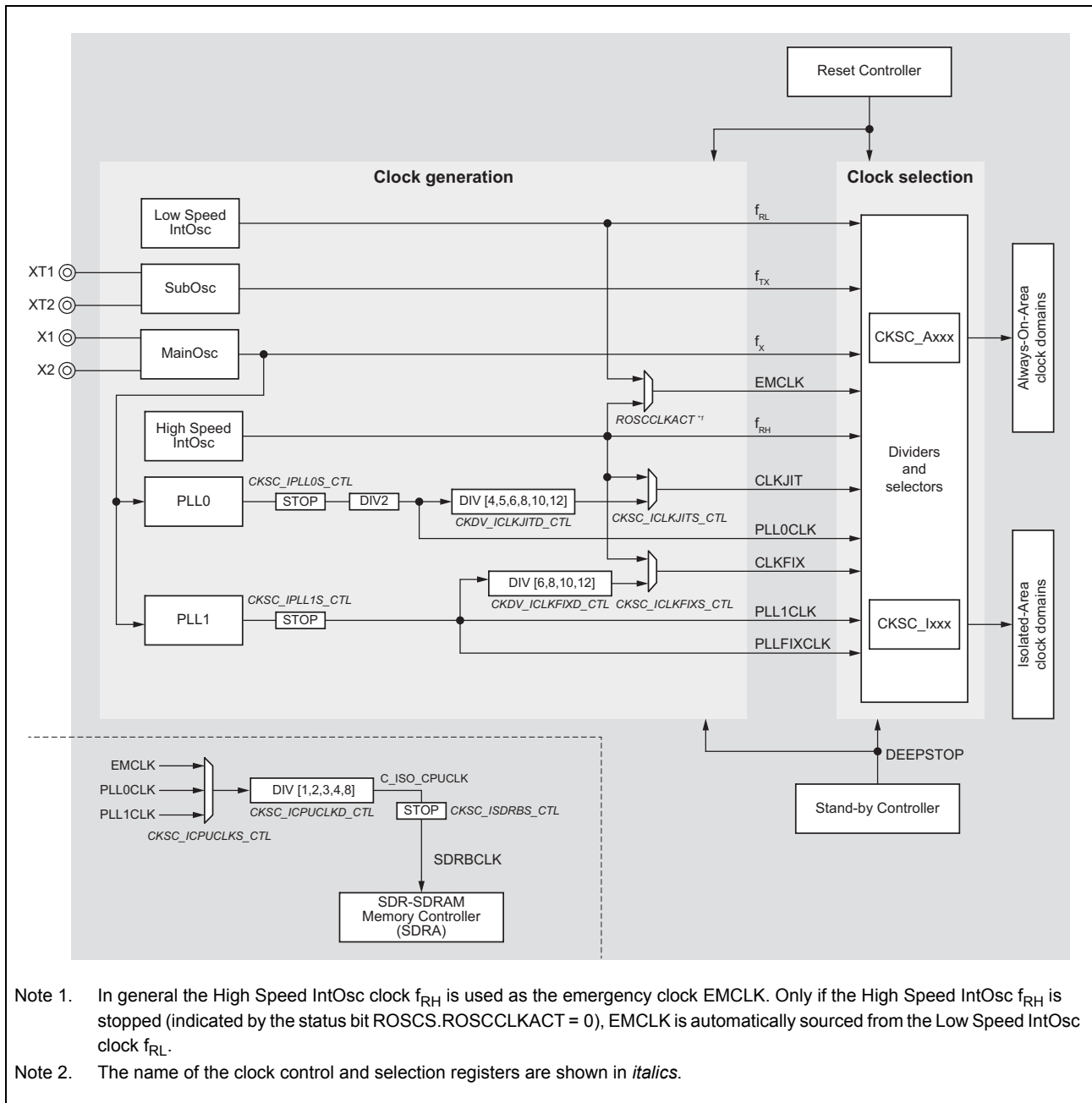
Figure 12.5 D1M1A Clock Controller block diagram
