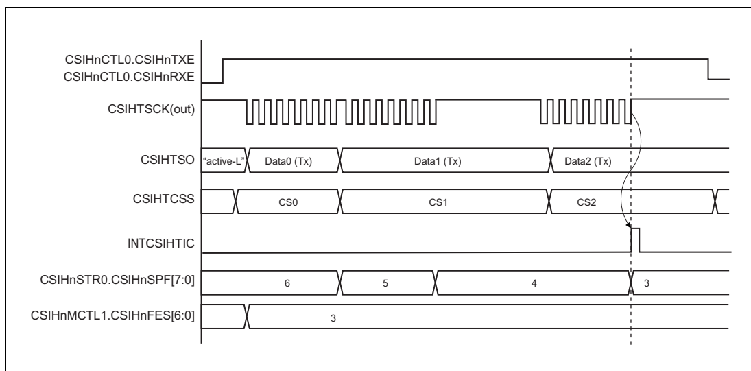
Figure 19.5 Generation of INTCSIHTIC in FIFO Memory Mode
