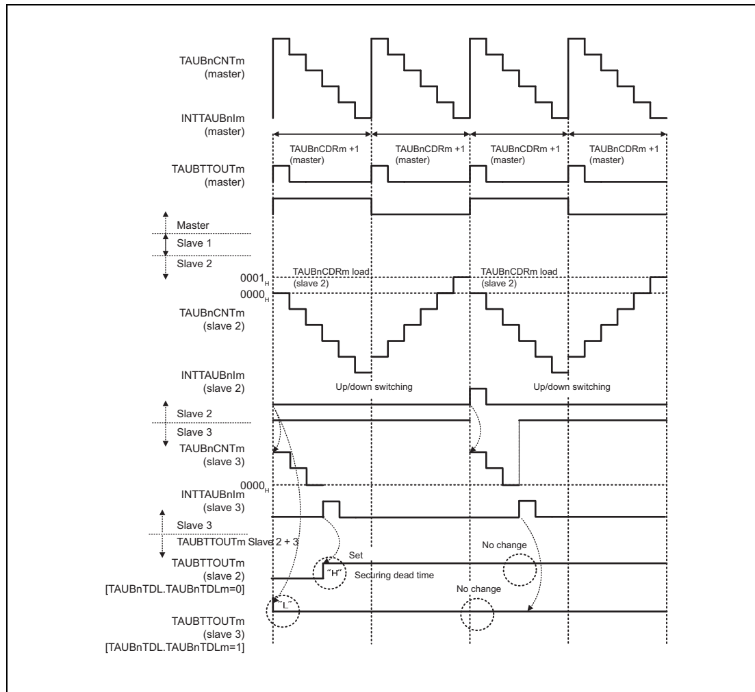
Figure 29.105 TAUBnCDRm (slave 2) = 0000 H
