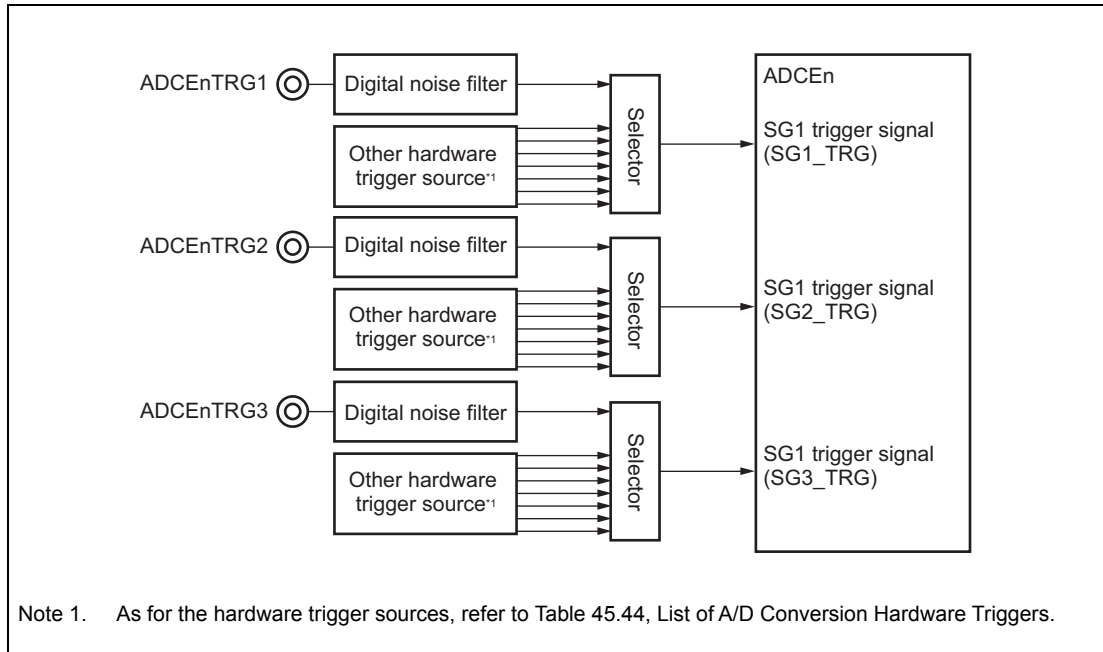
Figure 45.2 Internal Connection Diagram of External Trigger Input Pins
