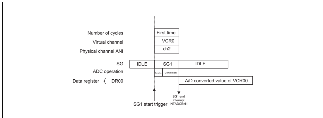
Figure 45.8 Example of Multicycle Scan Operation 2
