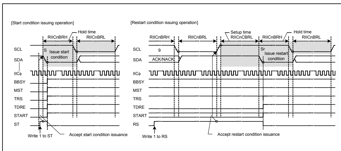
Figure 21.36 Start Condition/Restart Condition Issue Timing (ST and RS Bits)
