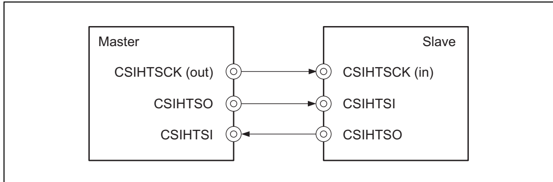
Figure 19.11 Direct Master/Slave Connection
