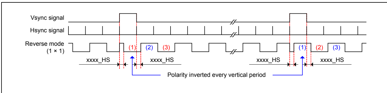
Figure 38.73 Horizontal Panel Driver Signal (in 1 × 1 Reverse Mode)
