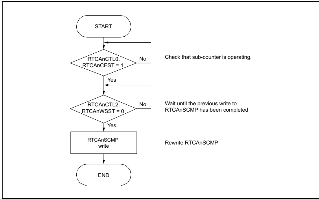
Figure 31.11 Writing the RTCAnSCMP Register
