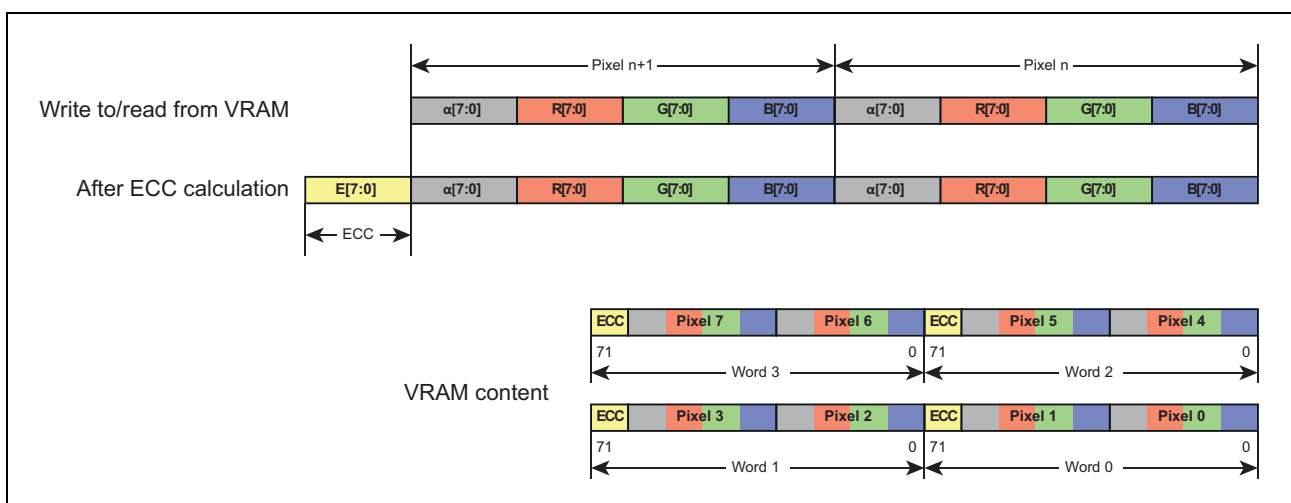
Figure 54.4 Direct 32-bit mode with ECC
