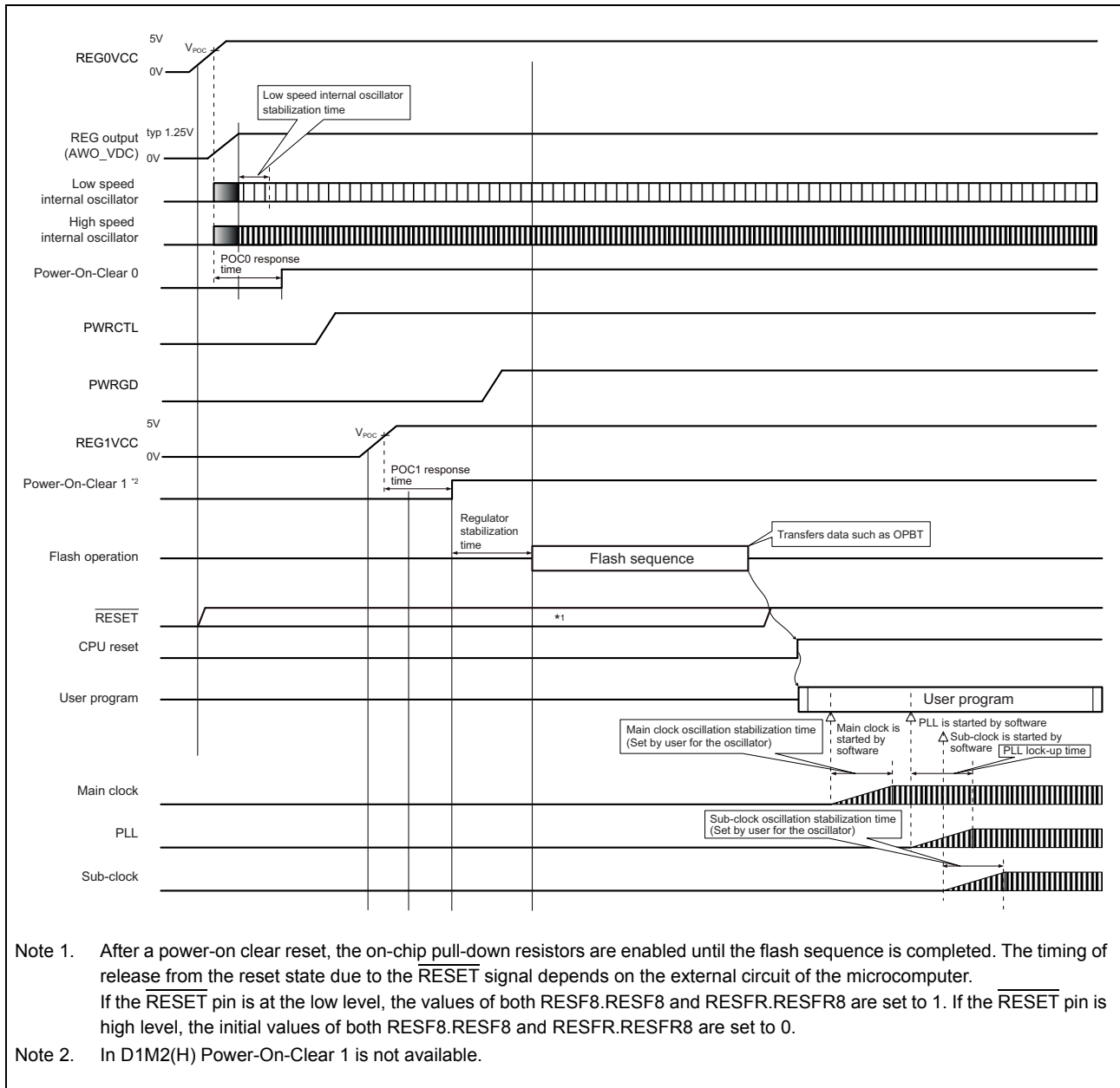
Figure 9.7 When \overline{\text{RESET}} is Released before the Flash Sequence is Completed
