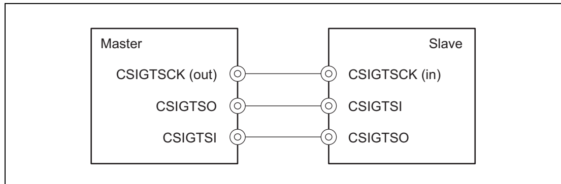
Figure 18.8 Direct Master/Slave Connection
