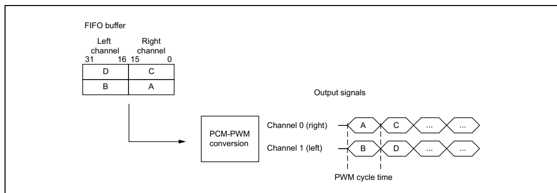
Figure 34.6 PCM-PWM in stereo mode
