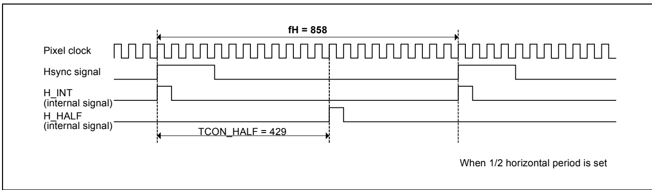
Figure 38.76 1/2 Pulse (H_HALF) Signal Generation
