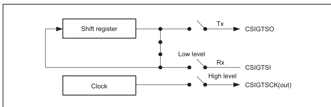
Figure 18.21 Operation in Loop-Back Mode
