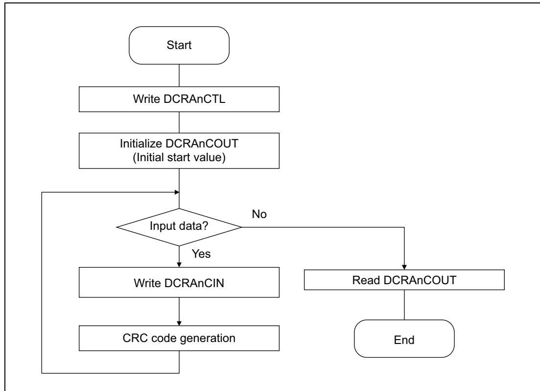
Figure 49.2 Flowchart of Data CRC Function A
