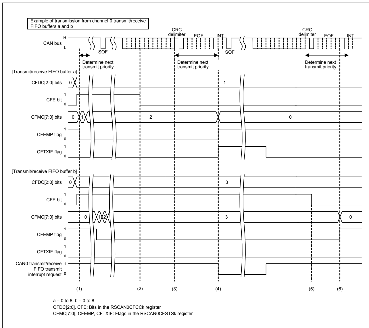
Figure 22.31 Transmit/Receive FIFO Buffer Transmission Timing Chart (Transmit Abort Completed)
