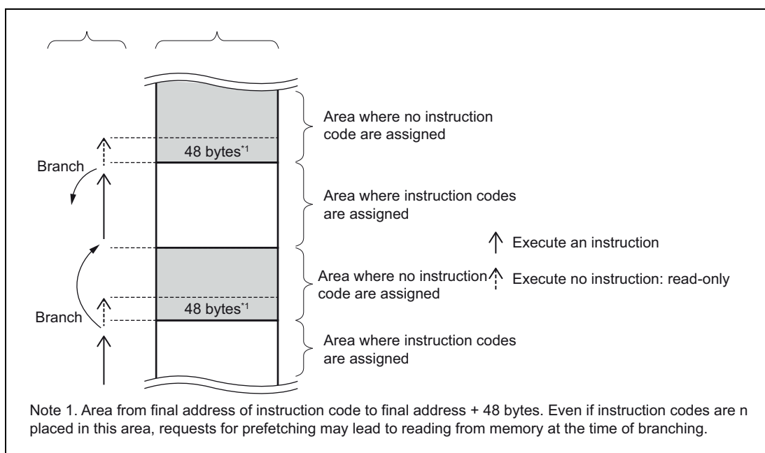
Figure 3.2 Area that Requires Attention Regarding Prefetching
