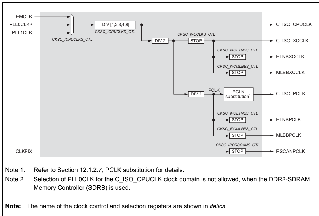
Figure 12.9 D1M2(H) CPU and bus subsystems clock domains
