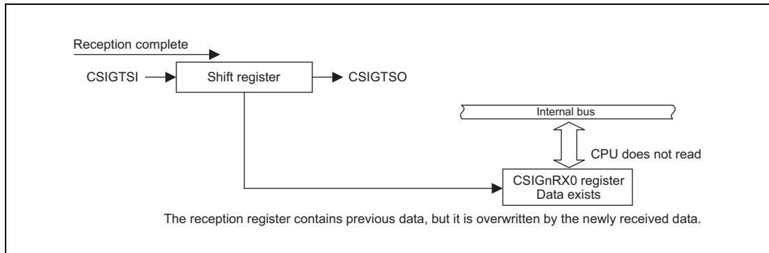
Figure 18.24 Overrun Error Detection
