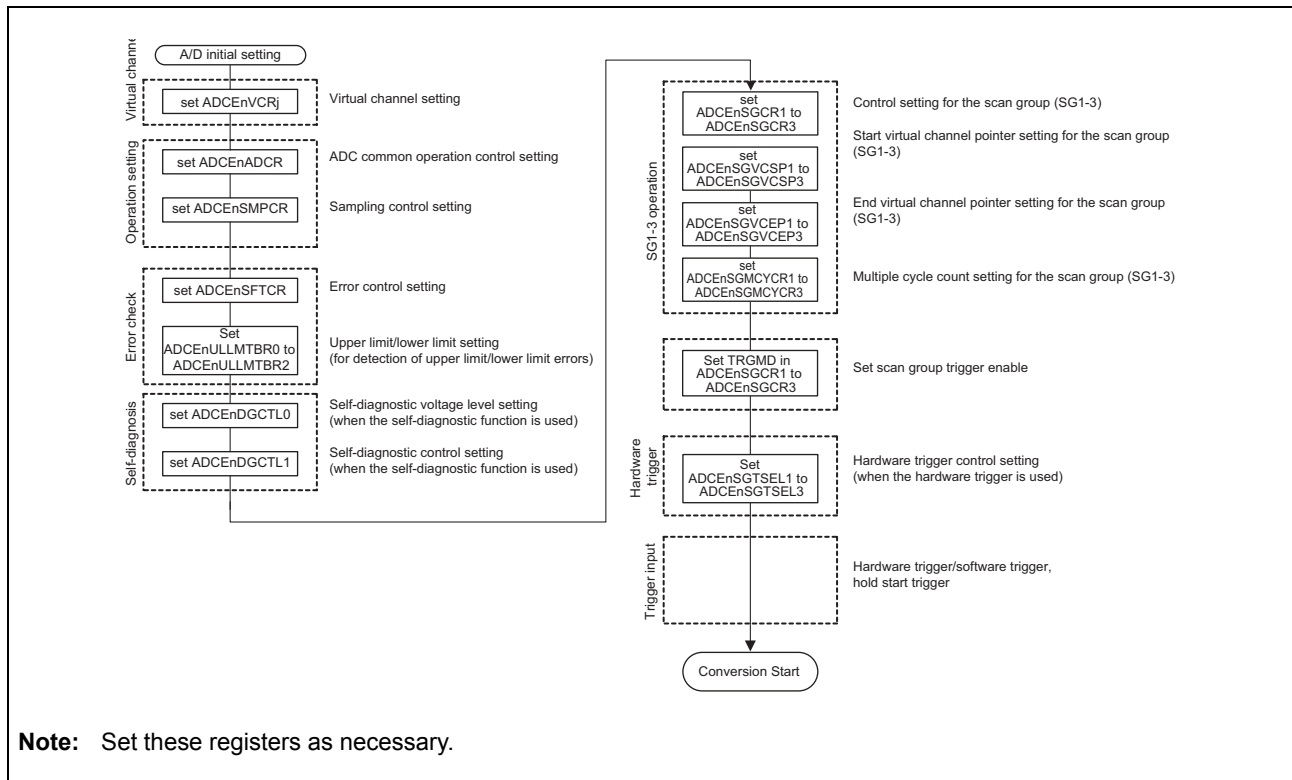
Figure 45.4 Flowchart for Initial Setting
