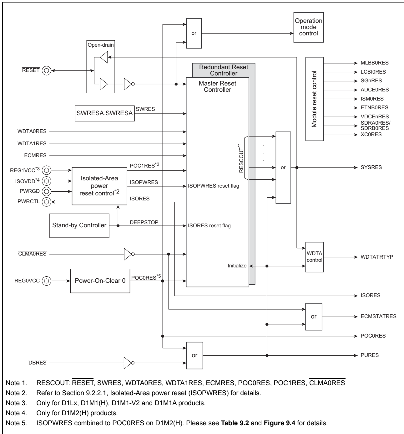
Figure 9.1 Block diagram of the Reset Controller
