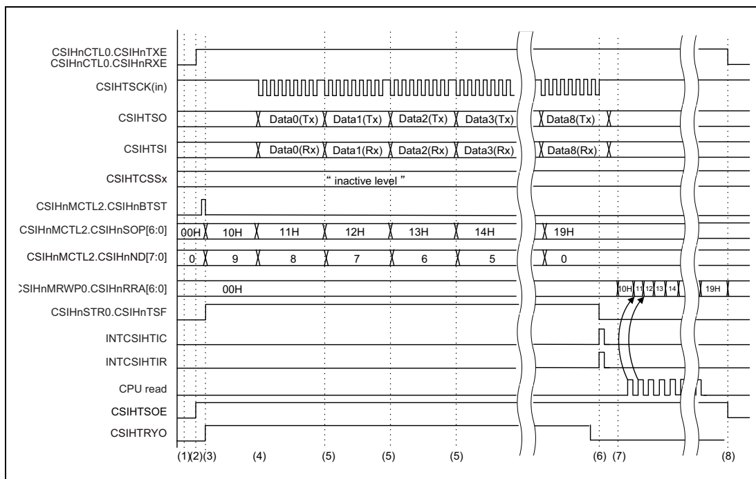
Figure 19.56 Slave in Dual Buffer Mode, CSIHnCTL1.CSIHnJE = 0
