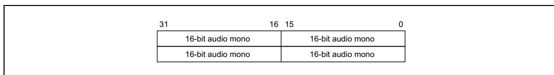
Figure 34.4 FIFO buffer in mono mode
