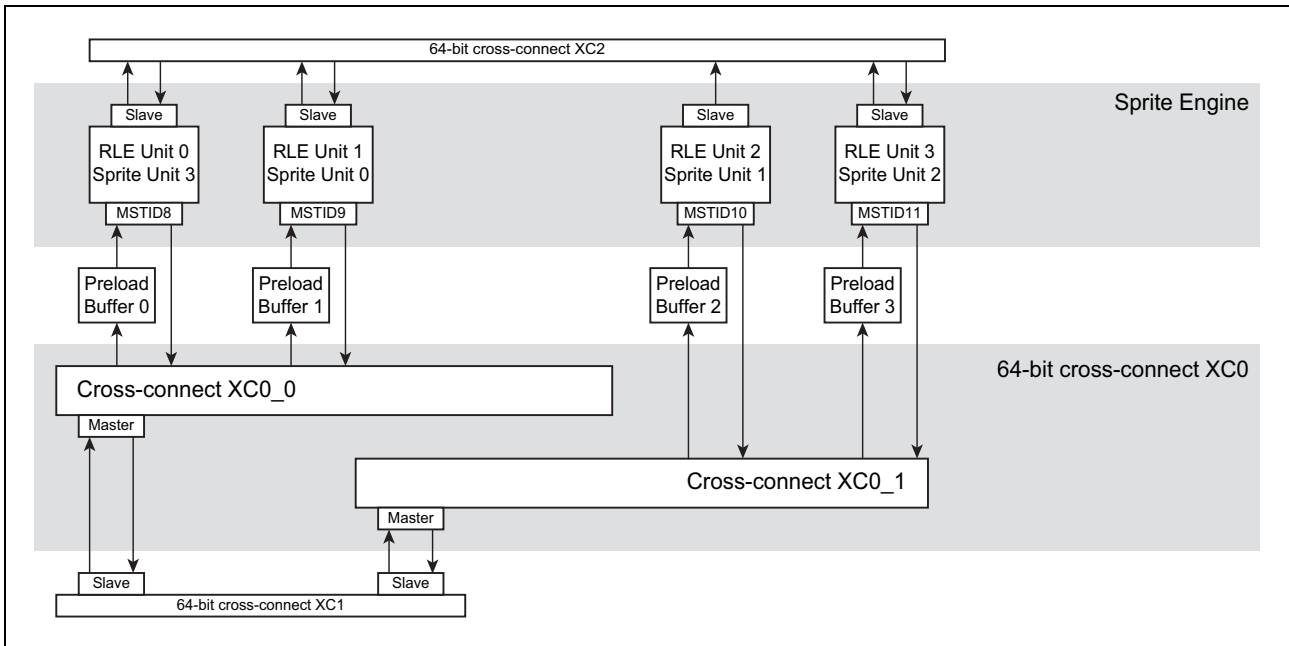
Figure 14.16 D1M1A cross-connect XC0
