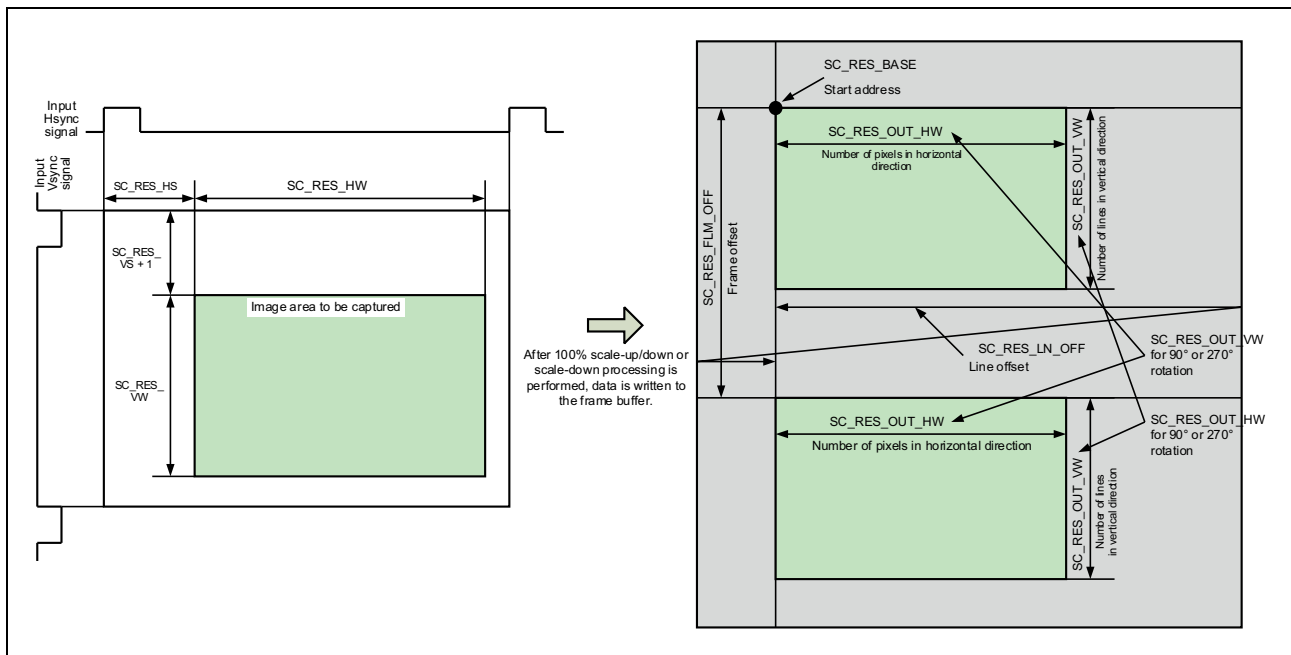
Figure 38.36 Data Arrangement in Frame Buffer
