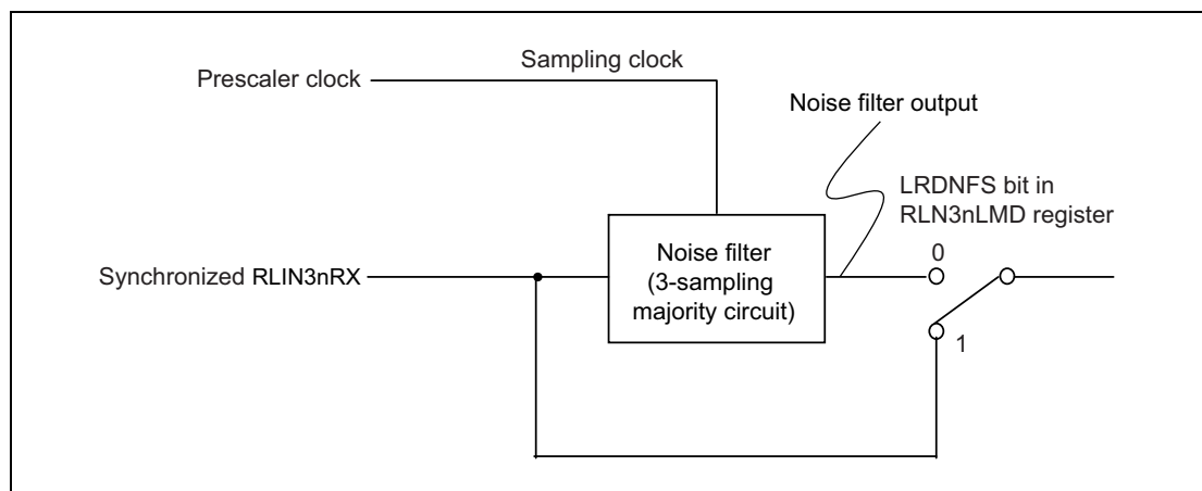
Figure 20.30 Configuration of Noise Filter
