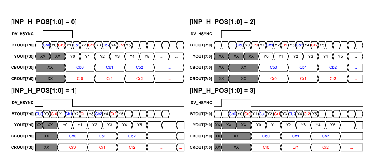
Figure 38.18 YCbCr Data Expansion for BT656/BT601 Input
