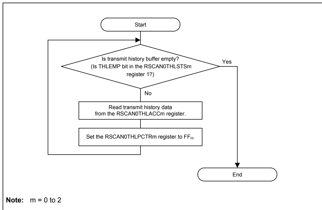
Figure 22.33 Transmit History Buffer Reading Procedure
