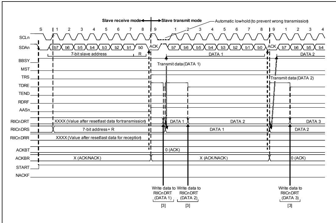
Figure 21.16 Slave Transmit Operation Timing (1) (7-Bit Address Format)
