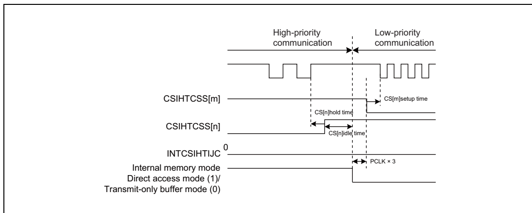
Figure 19.48 Transition from High-Priority Mode to Low-Priority Mode
