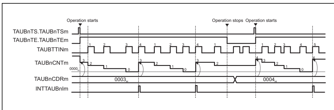
Figure 29.43 Operation Stop and Restart, (TAUBnCMURm.TAUBnTIS[1:0] = 01 B )
