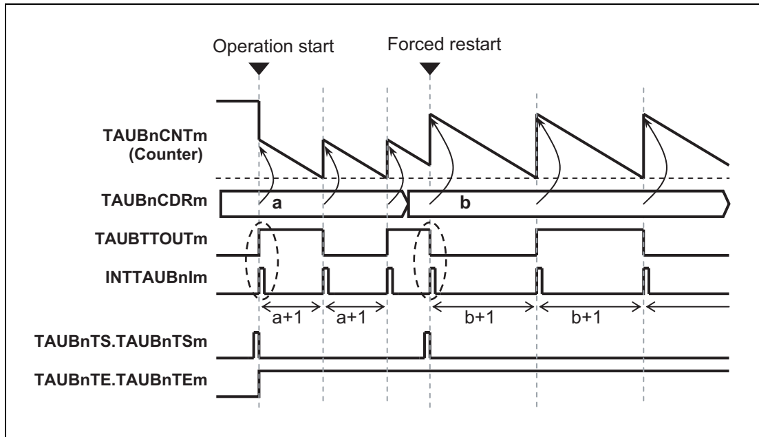
Figure 29.30 Forced Restart Operation, \text{TAUBnCMORm.TAUBnMD0} = 1
