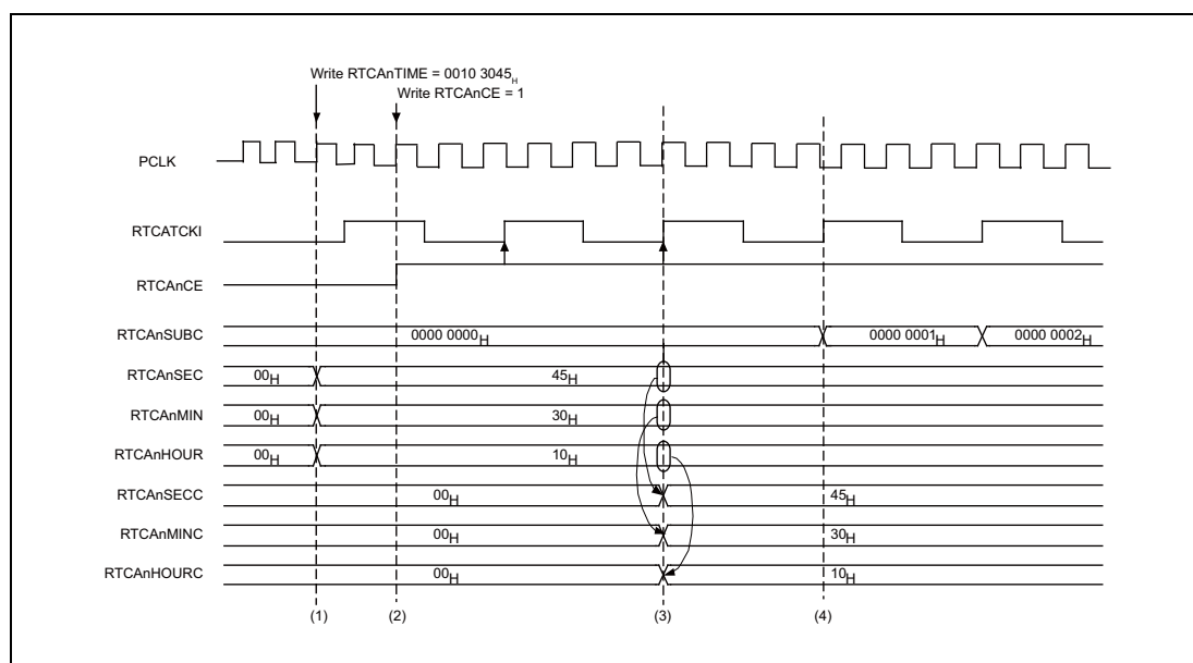
Figure 31.12 Counter Start Timing
