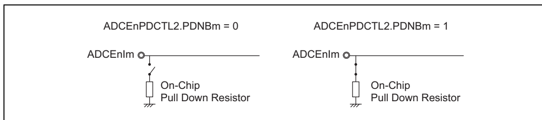
Figure 45.25 Setting of On-chip Pull Down Resistor
