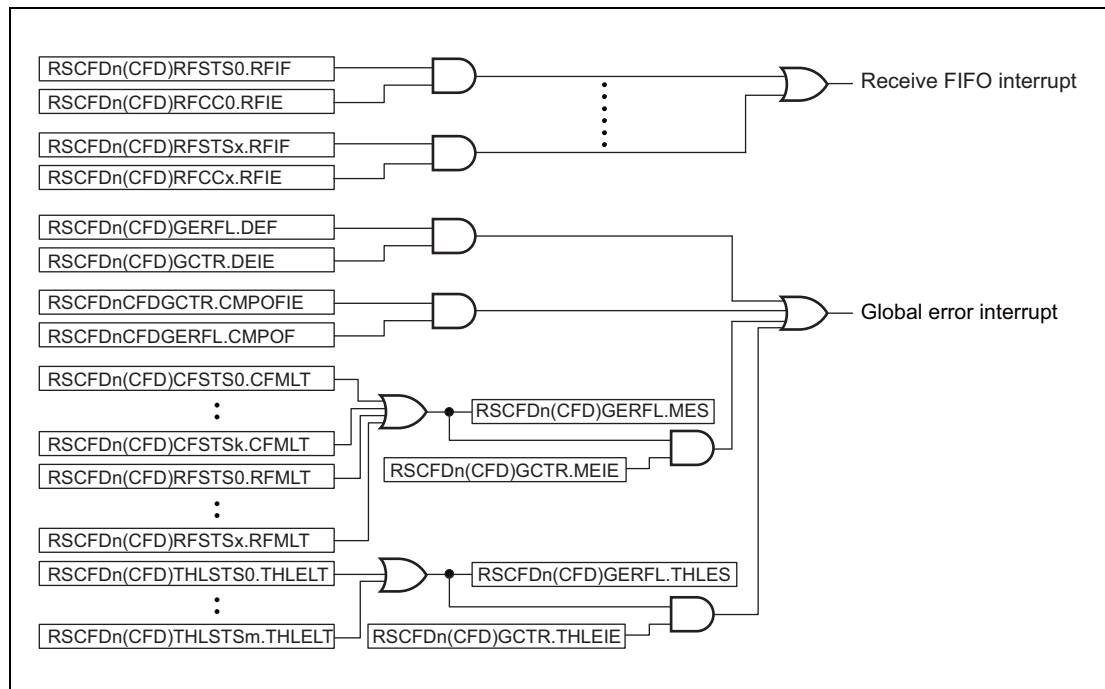
Figure 23.2 CAN Global Interrupt Block Diagram
