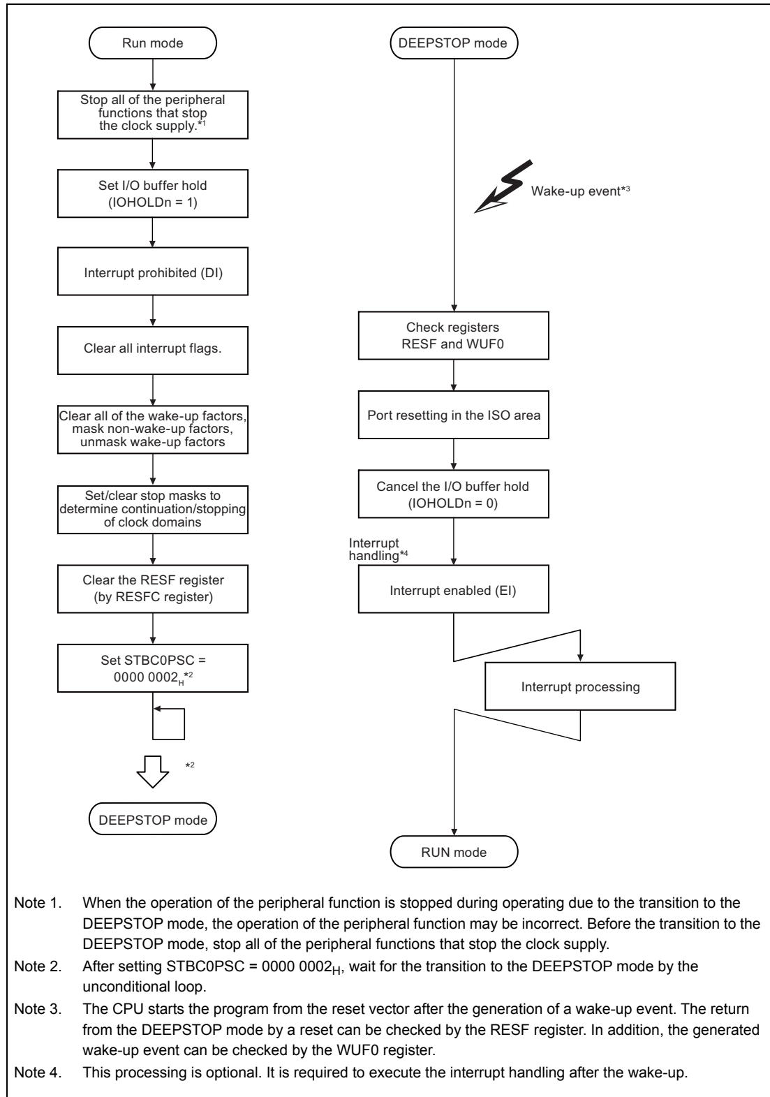
Figure 13.2 Example of DEEPSTOP mode transition (D1M1A, D1M1-V2)
