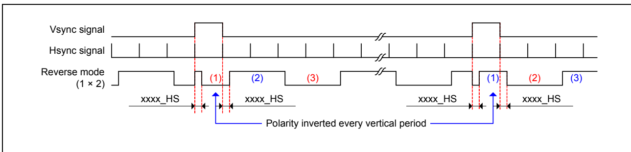
Figure 38.74 Horizontal Panel Driver Signal (in 1 × 2 Reverse Mode)
