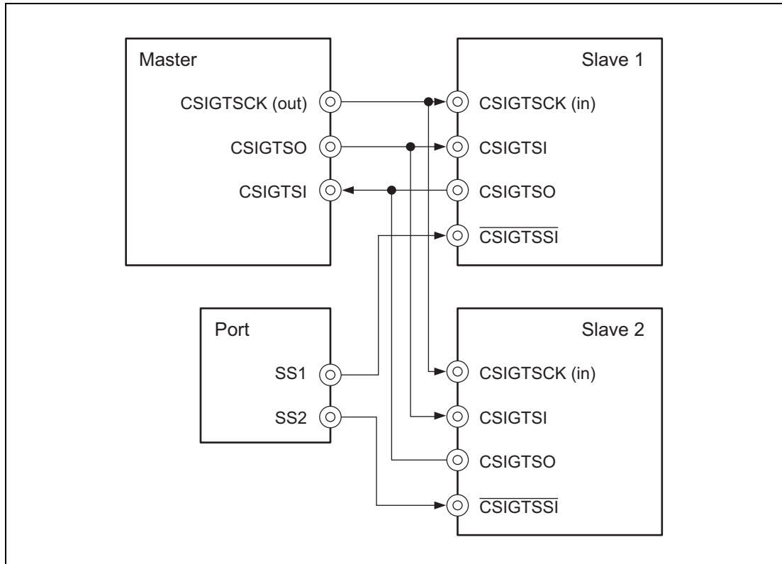
Figure 18.9 Master to Multiple Slaves Connection
