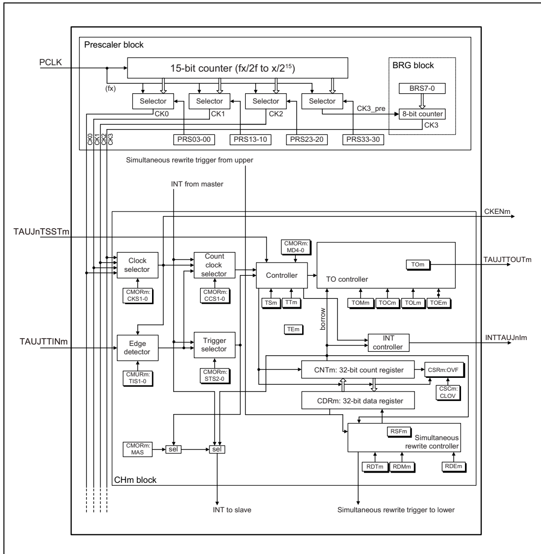
Figure 30.2 Block Diagram of the TAUJ
