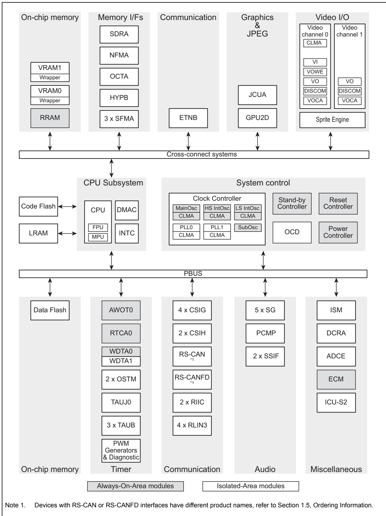
Figure 1.5 D1M1A block diagram
