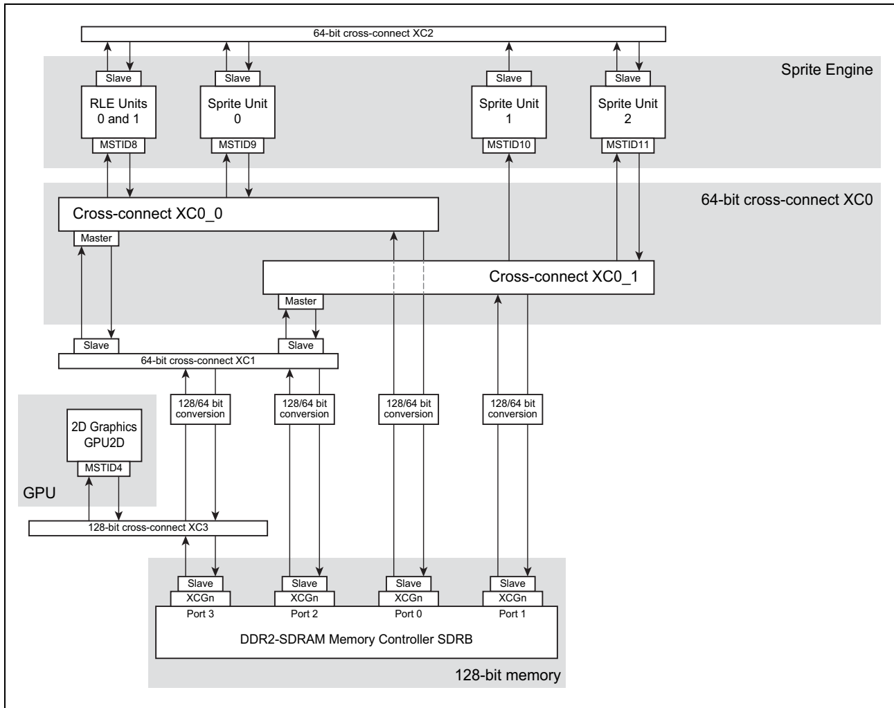
Figure 14.20 D1M2(H) cross-connect XC0
