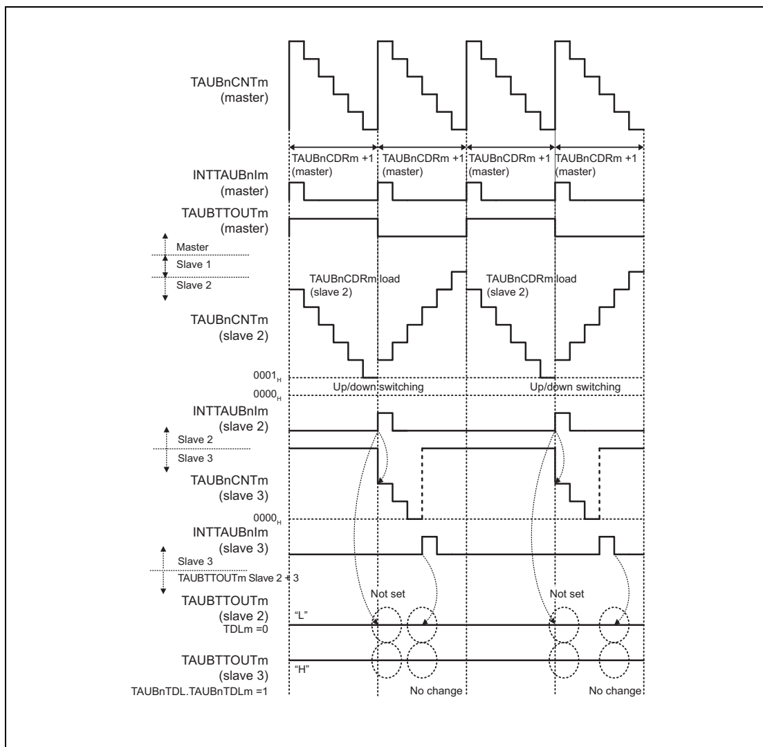
Figure 29.104 TAUBnCDRm (slave 2) ≥ TAUBnCDRm (master) + 1
