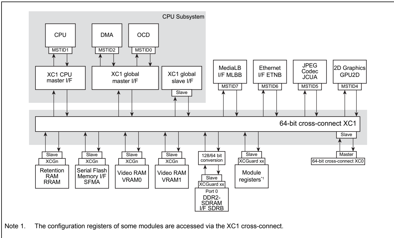
Figure 14.21 D1M2(H) cross-connect XC1
