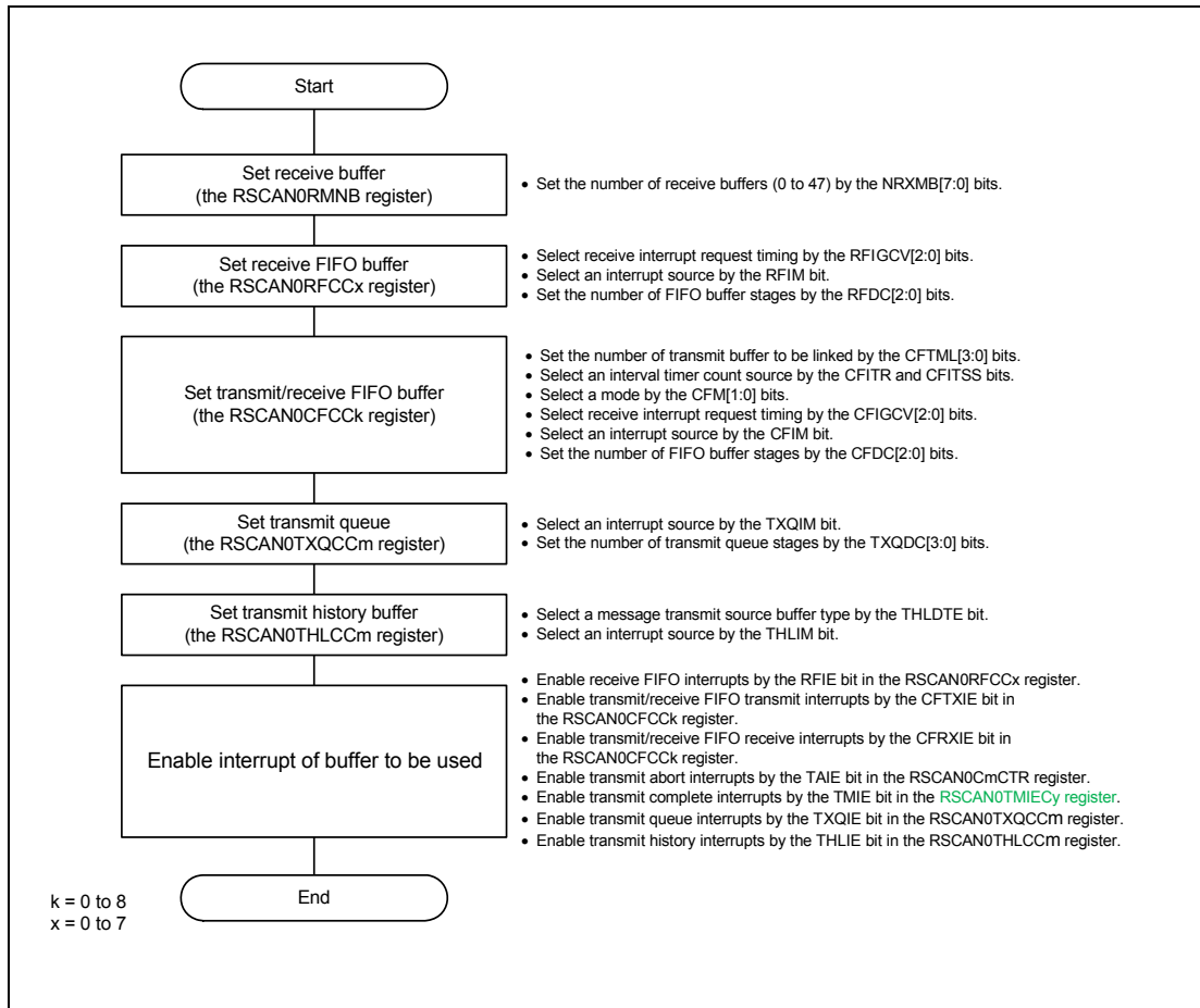
Figure 22.21 Buffer Setting Procedure
