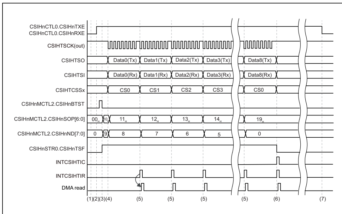
Figure 19.52 Master in Transmit-Only Buffer Mode, CSIHnCTL1.CSIHnJE = 0
