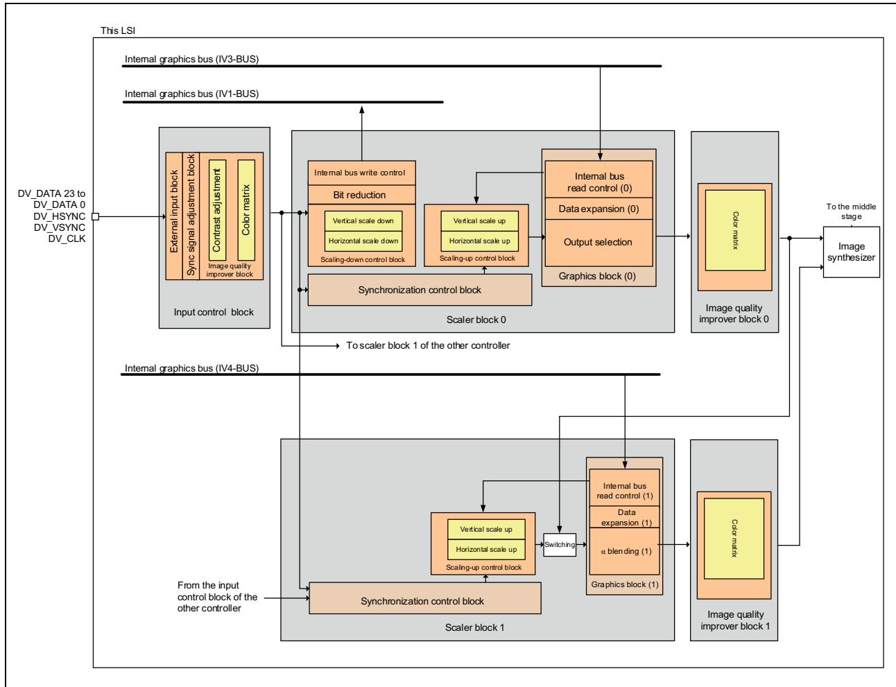
Figure 38.1 Video Display Controller Former Stage Block Diagram
