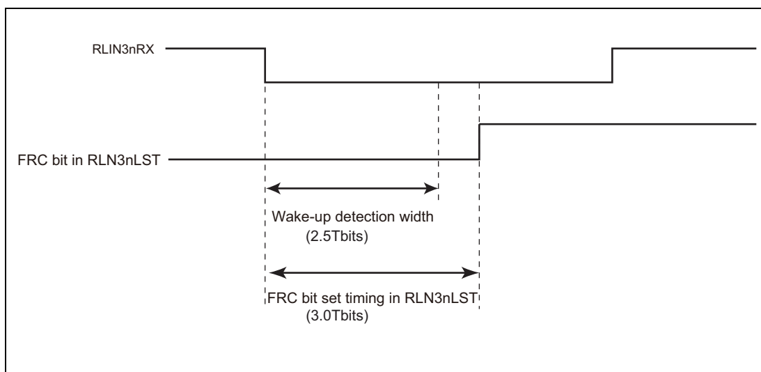
Figure 20.12 Input Signal Low level Count Function
