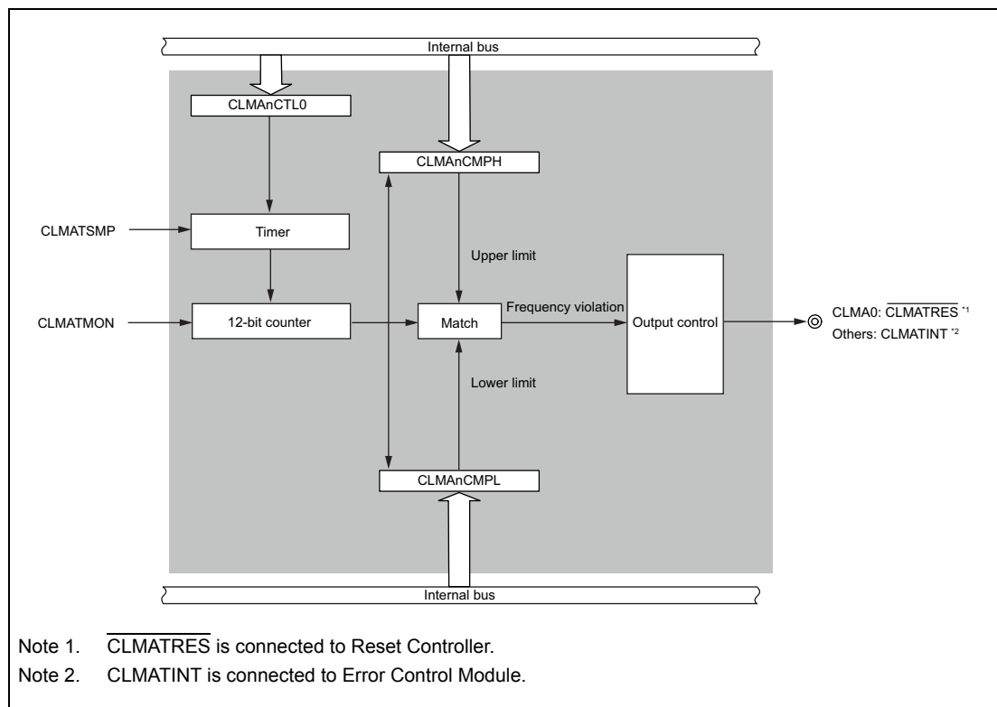
Figure 12.18 Block diagram of the Clock Monitor A
