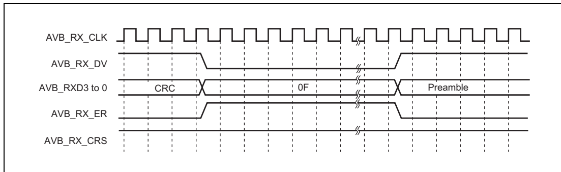
Figure 24.71 MII Fame Receive Timing (Burst Reception)
