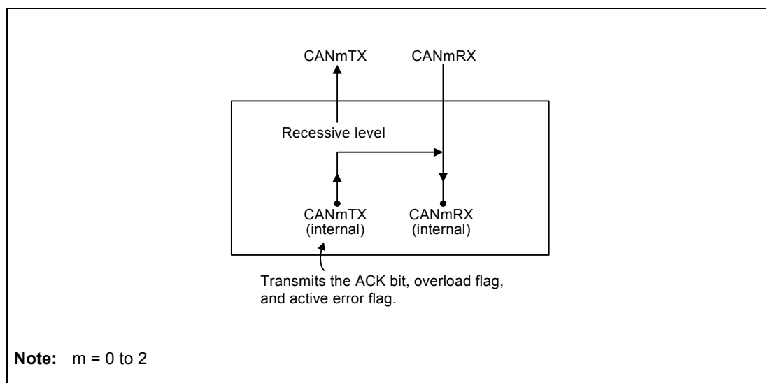
Figure 23.12 Connection when Listen-Only Mode is Selected
