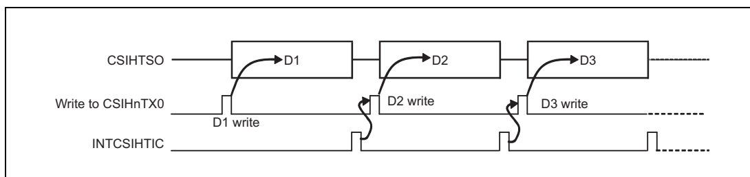
Figure 19.3 Generation of INTCSIHTIC after Transfer (CSIHnCTL1.CSIHnSLIT = 0)
