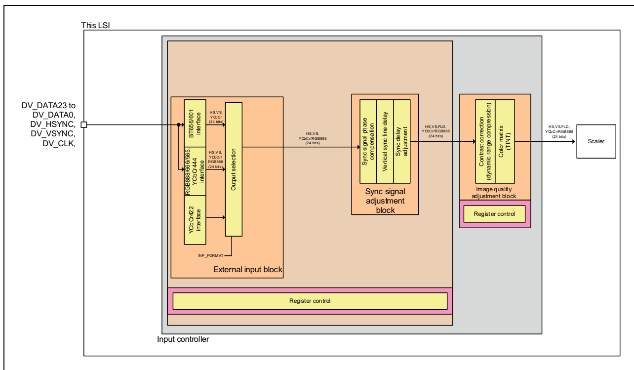
Figure 38.7 Functional Block Diagram of Input Controller
