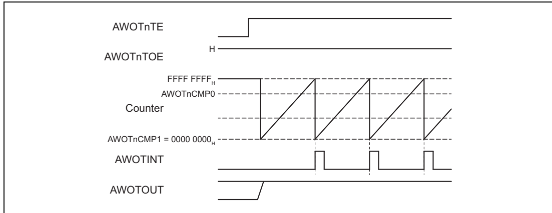
Figure 28.6 PWM mode with 100 % duty cycle
