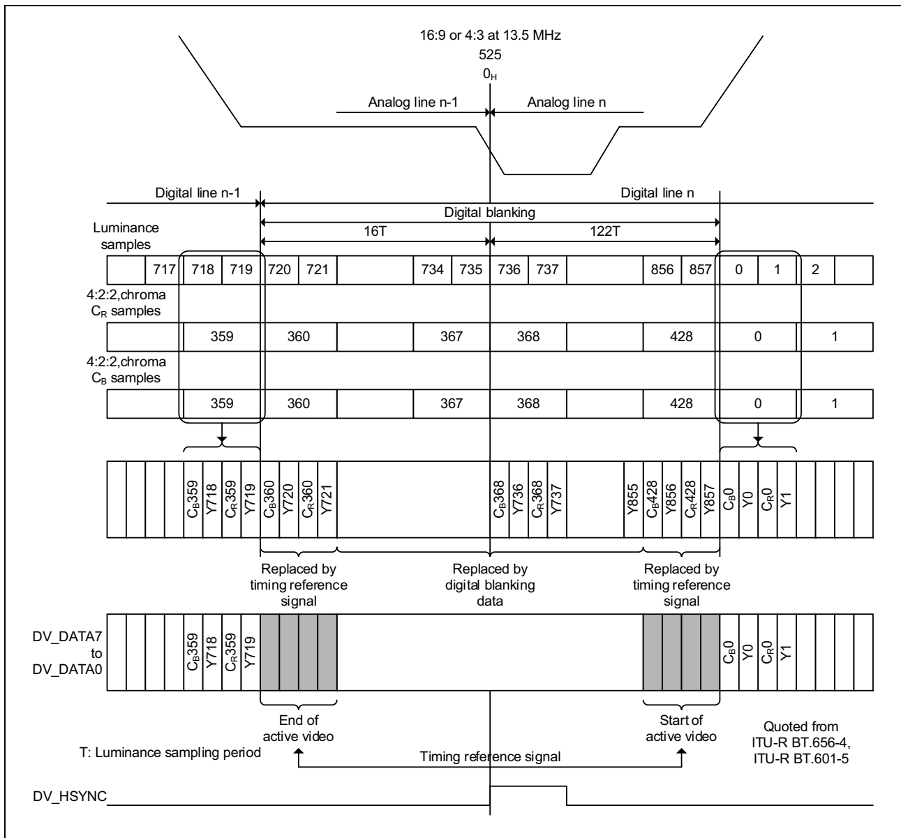
Figure 38.14 BT656 Horizontal Timing (525 Lines/59.94 Hz)
