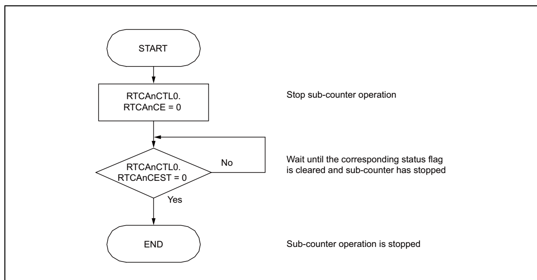
Figure 31.4 RTCA Stop Procedure
