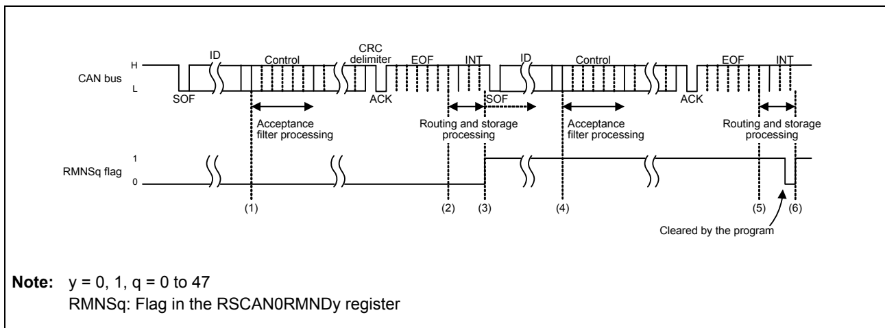
Figure 22.23 Receive Buffer Reception Timing Chart
