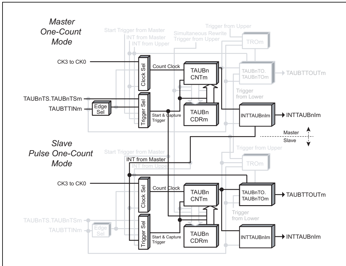
Figure 29.84 Block Diagram for One-Shot Pulse Output Function
