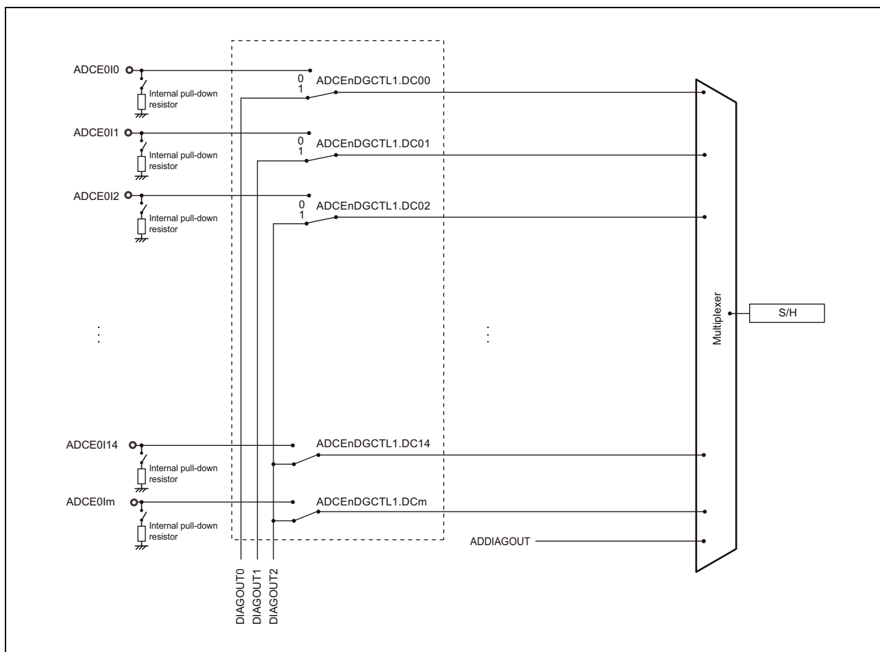
Figure 45.24 Overview of Self-Diagnostic Functions
