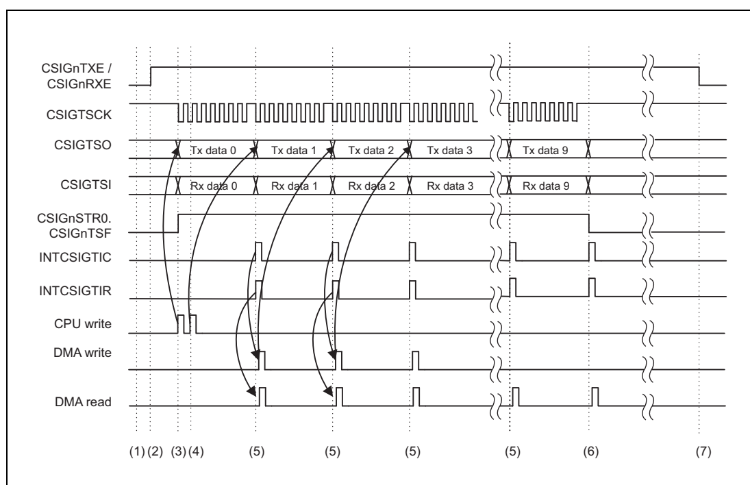
Figure 18.26 Communication in Master Mode
