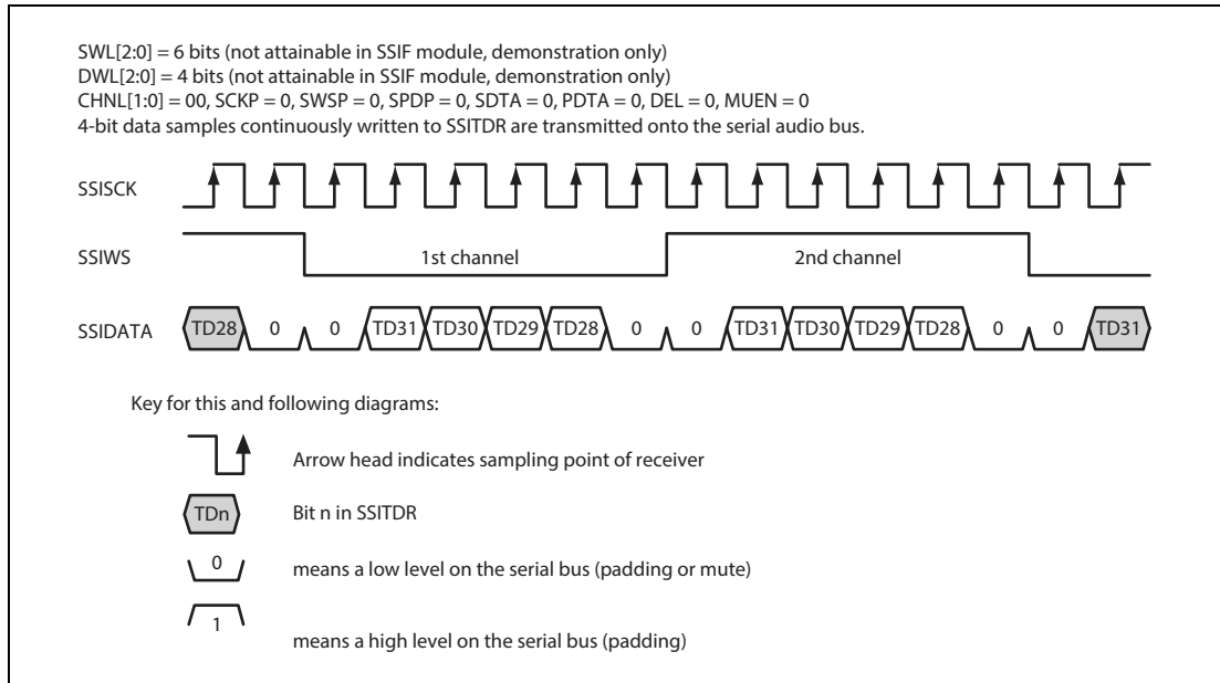
Figure 35.9 Basic Sample Format (Transmit Mode with Example System/Data Word Length)
