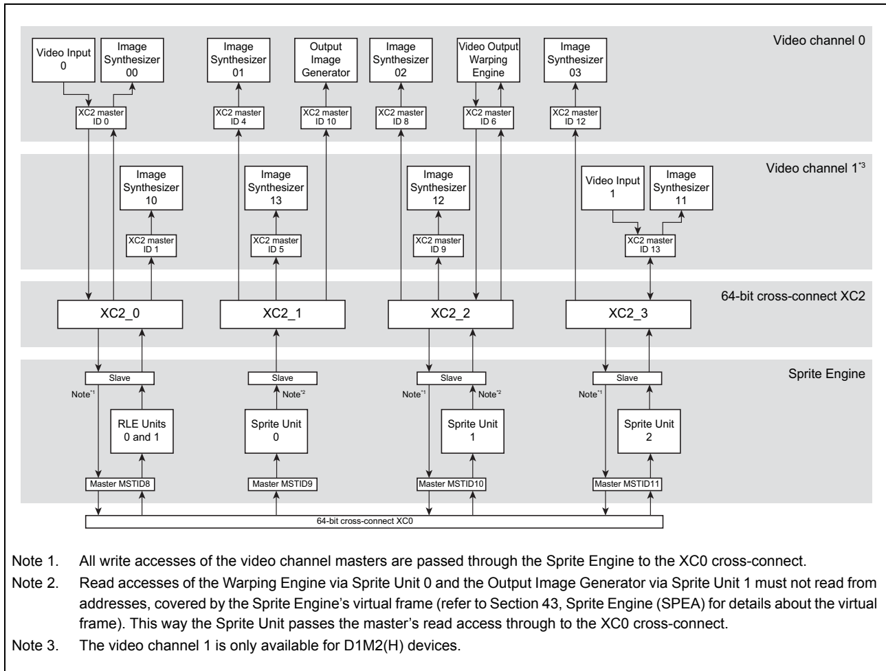
Figure 14.22 D1M2(H) cross-connect XC2
