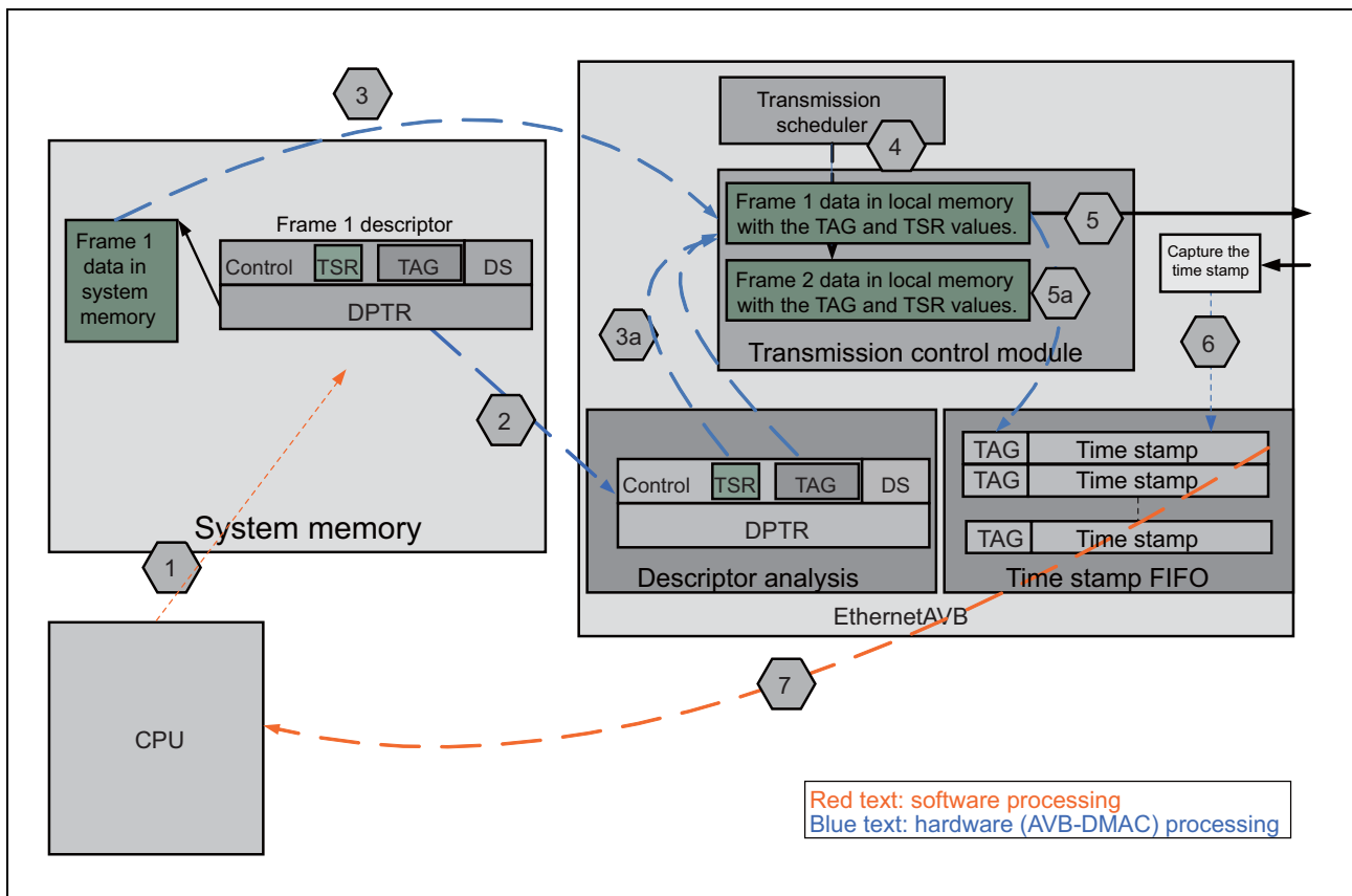
Figure 24.41 Mechanism to Support Transmission Time Stamps
