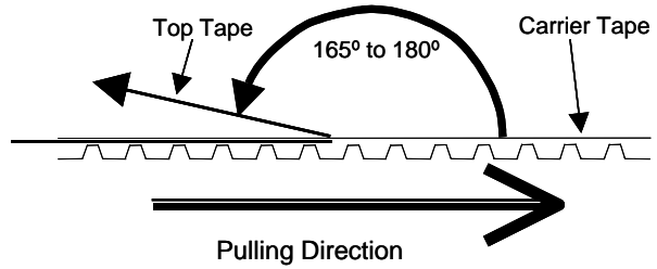
Fig.9 Peeling Strength
