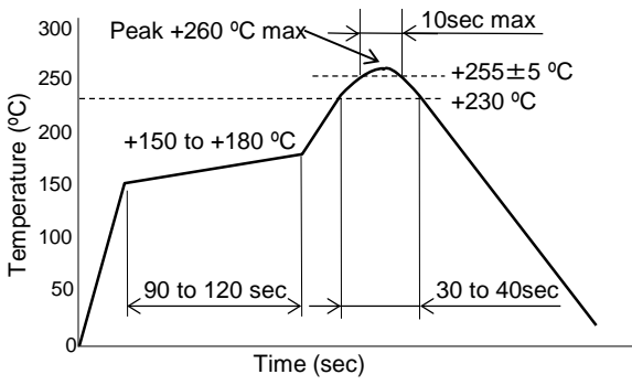
Fig.5 Reflow profile (Lead Free Available)
