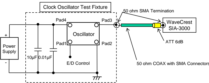
Fig.1 Test Circuits
