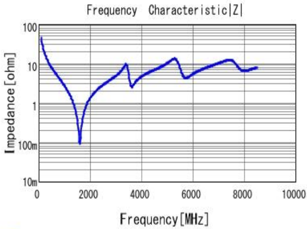
GQM1555C2A360JB01 |Z| DCOV, 25degC
