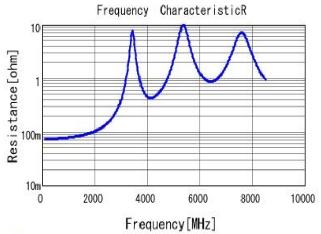
GQM1555C2A360JB01 R DCOV, 25degC
