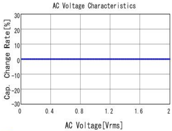
GQM1555C2A360JB01 C-AC Voltage capchange, DCOV, 25.0d
