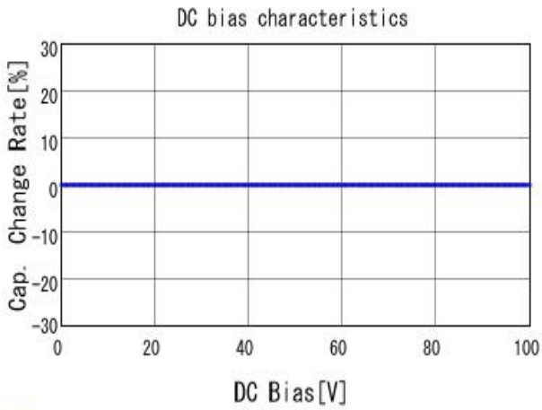
GQM1555C2A360JB01 C-DC bias capchange, 25.0degC, AC1V
