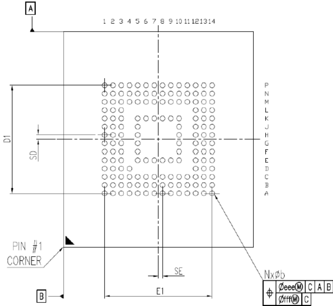
Bottom view
