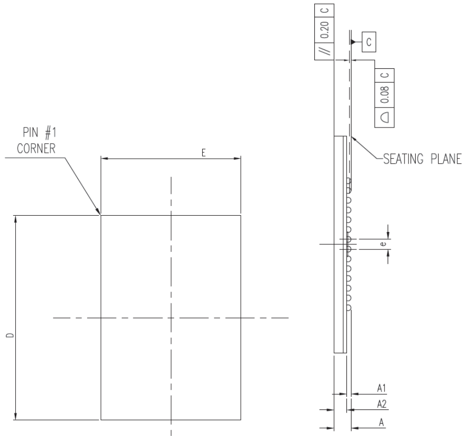
Figure 2 – Package Dimensions
