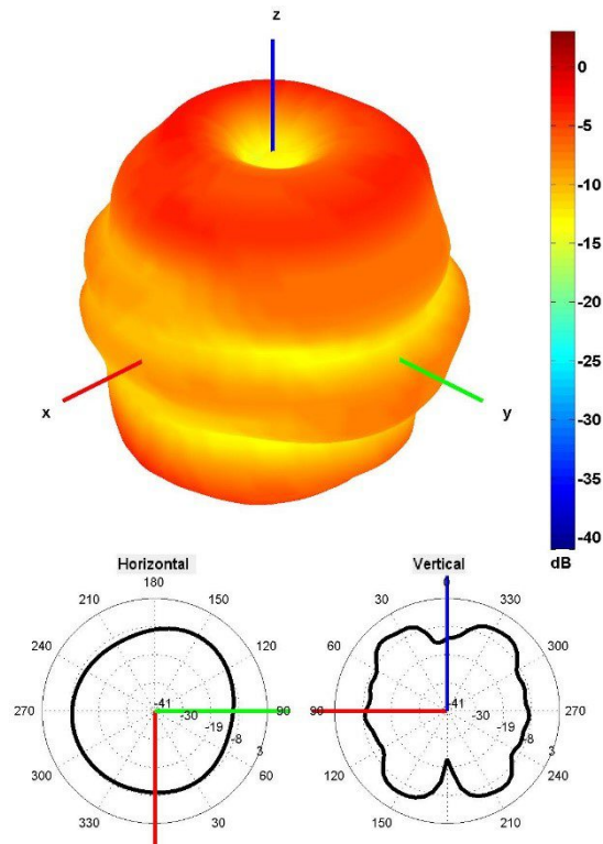
3600 MHz Radiation pattern
