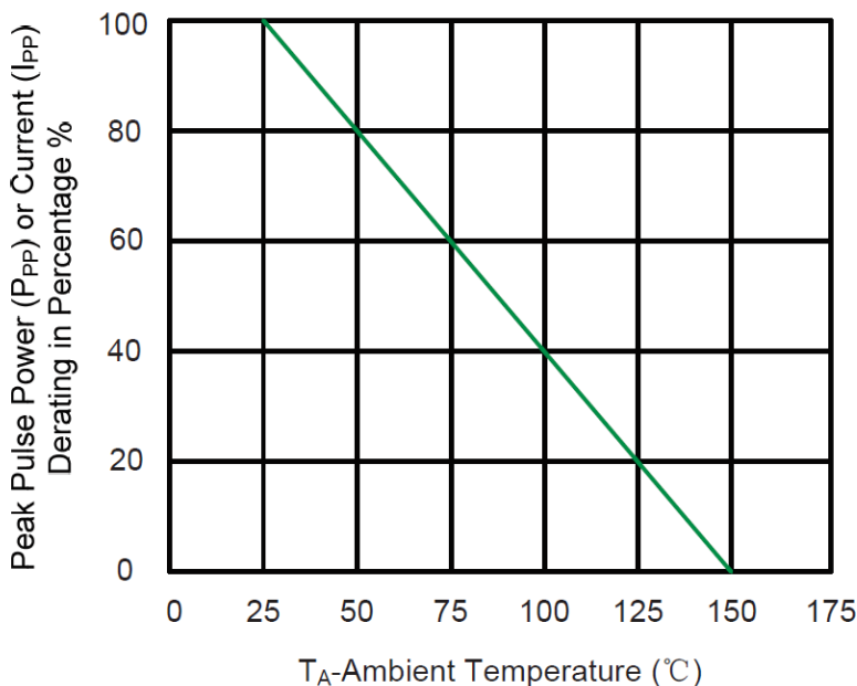
Figure 2. Pulse Derating Curve
