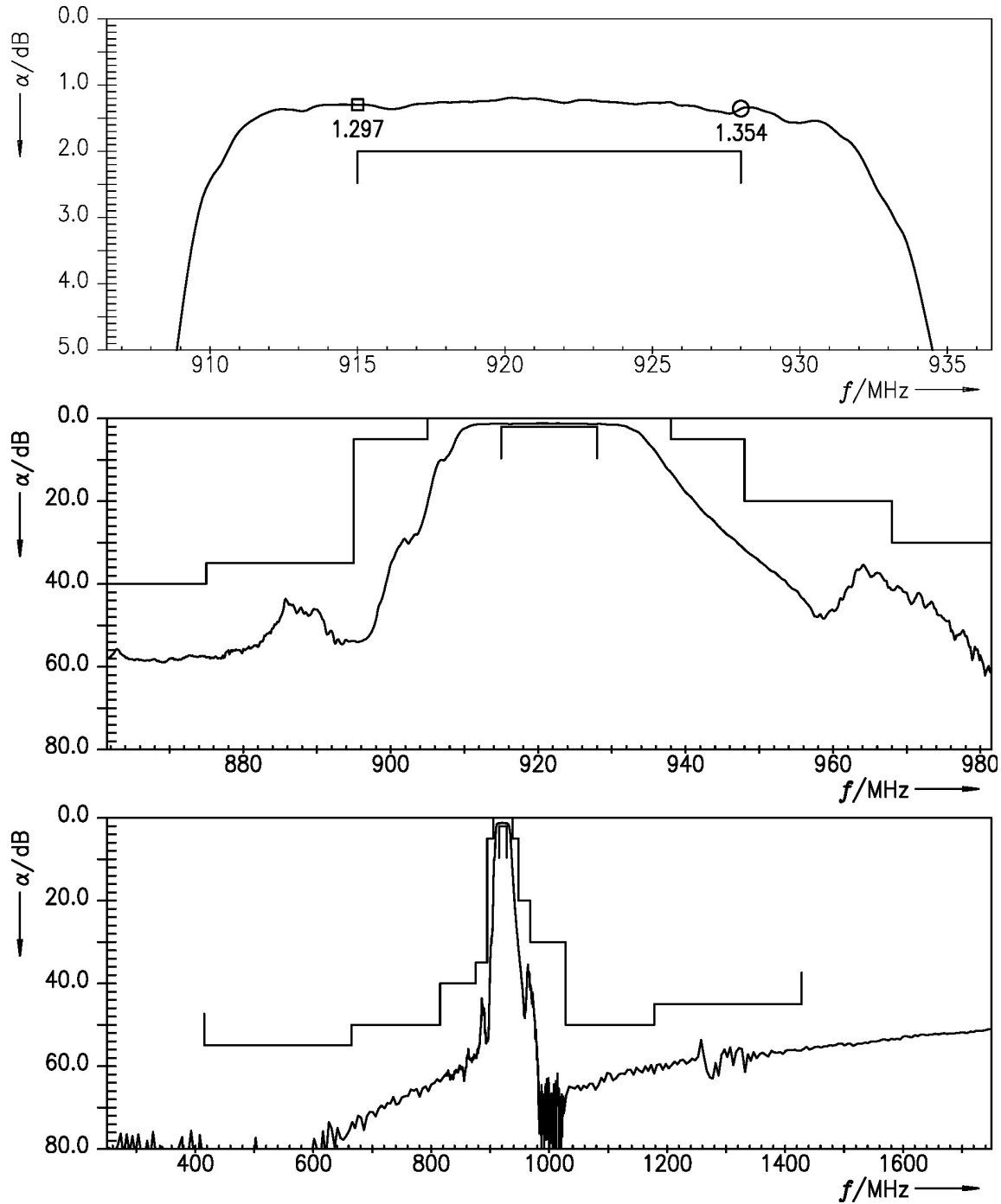
Figure 4: Attenuation .
