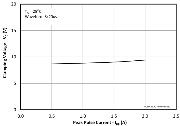
Clamping Voltage vs. Peak Pulse Current (tp=8/20us)
