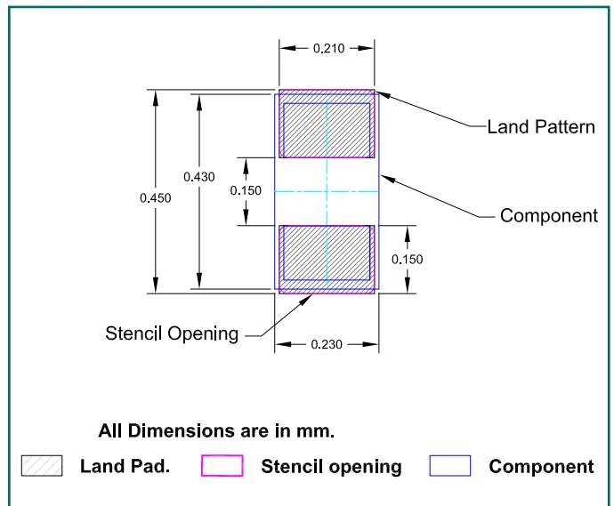
Figure 1 - Mounting Pattern - 0.075mm Stencil
