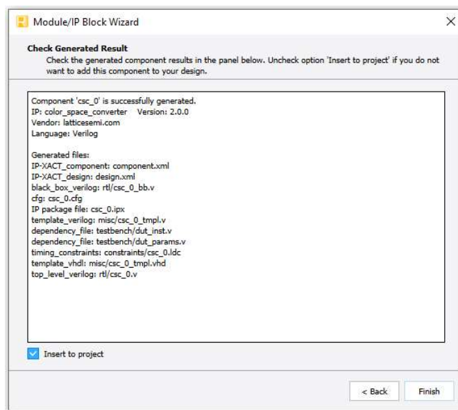
Figure 3.3. Check Generating Result
