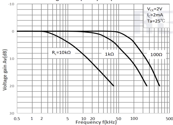
Fig.11 Frequency Response
