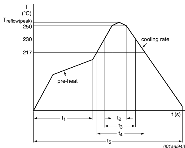
Fig 8. Pb-free solder reflow profile
