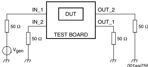
Fig 5. Crosstalk measurement configuration
