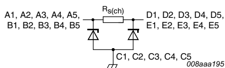
Fig 2. Schematic diagram IP4041CX25
