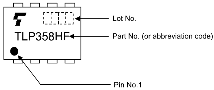
Fig. 14.1 Marking
