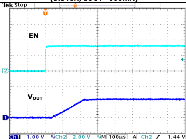
FIGURE 8 TURN-ON (3.3VIN, IOUT=600mA)
