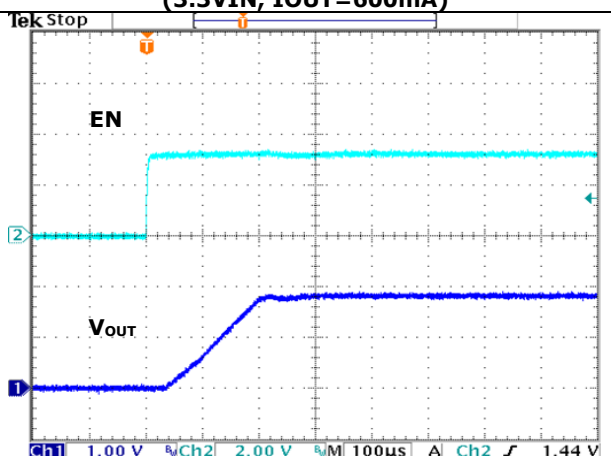
FIGURE 14 TURN-ON (3.3VIN, IOUT=600mA)
