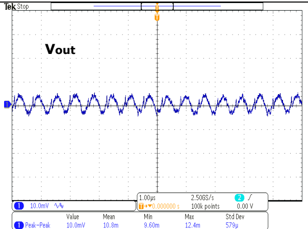
FIGURE 6 OUTPUT RIPPLE (3.3VIN, IOUT=600mA)
