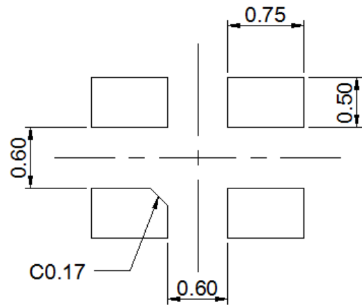
RECOMMENDED STENCIL PATTERN BASED ON 100μm THICKNESS STENCIL
