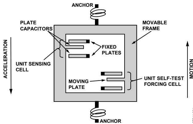
Figure 4. Simplified View of ADXL180 Sensor Under Acceleration
