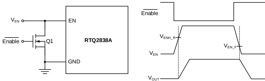
Figure 9. Logic Control for the EN Pin
