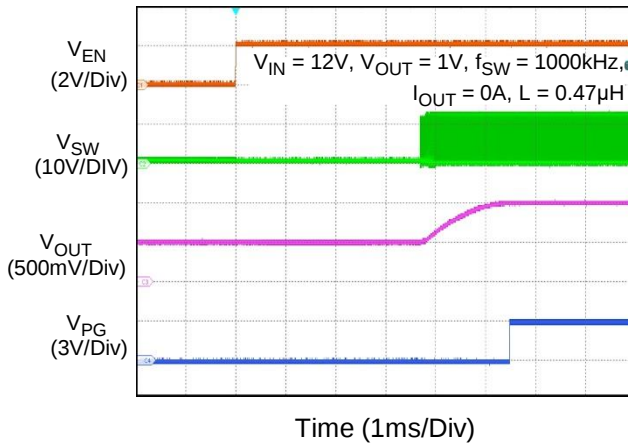
Pre-bias Start-up
