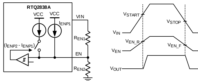
Figure 10. Adjustable VIN UVLO
