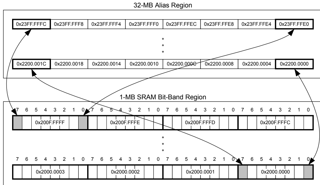
Figure 2-4. Bit-Band Mapping
