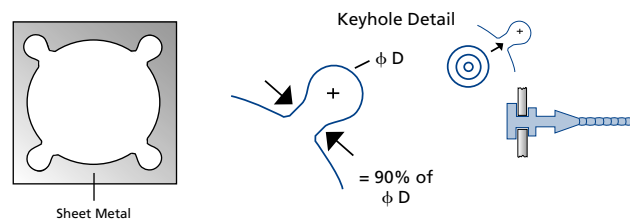
Figure 9: Rotational Keyhole
