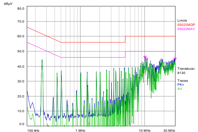
Figure 11, DIM3R3400 EMI(work with Delta power module Q48SQ12033NRFH).
