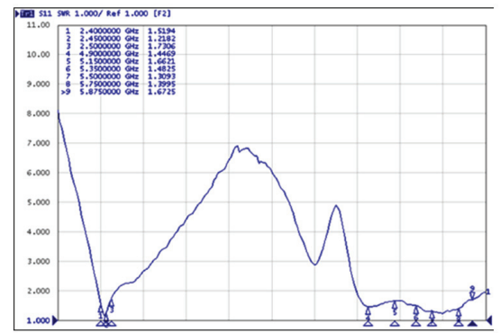
WTL2449C Return Loss Plot
