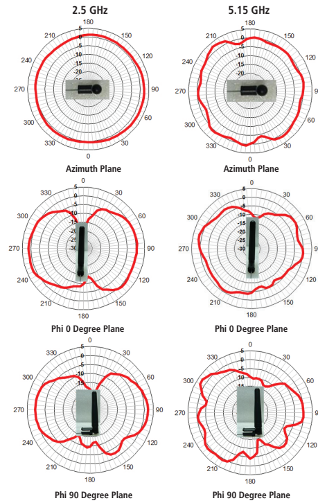
WTL2449S Typical Radiation Patterns
