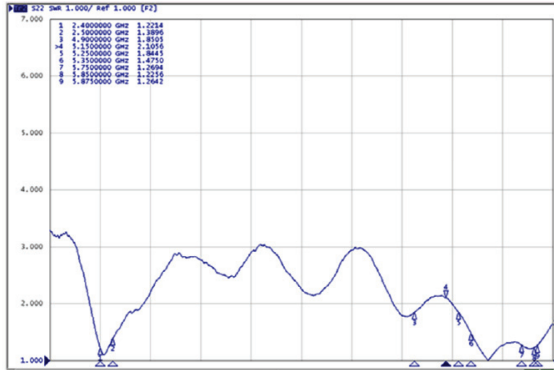
WTL2449S Return Loss Plot
