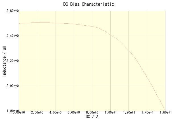
VLM1055T-2R5M8R0-2(Amb. Temp. = 20degc)
