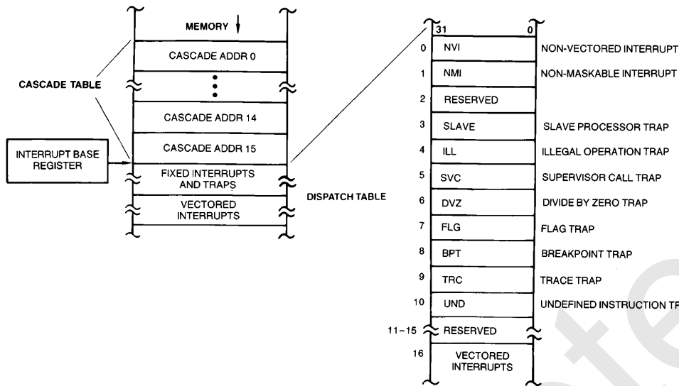
FIGURE 3-4. Interrupt Dispatch and Cascade Tables
