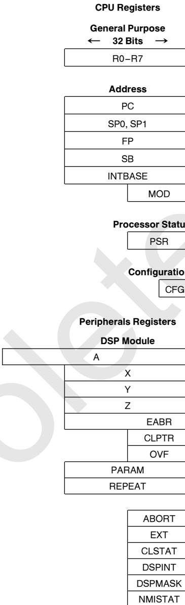
FIGURE 2-1. NS32FX164 Internal Registers
