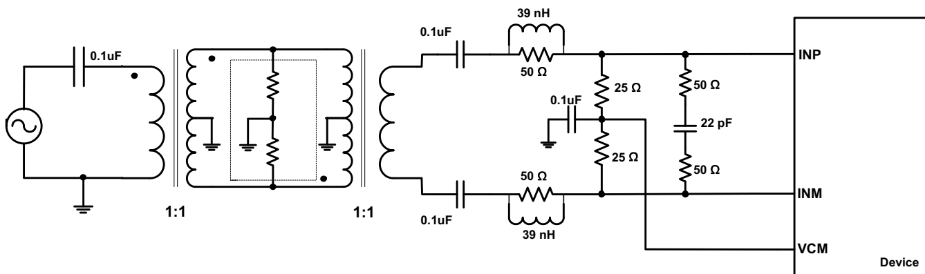
Figure 202. Driving Circuit for Low Input Frequencies
