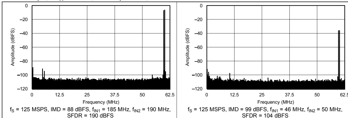
Figure 46. FFT for Two-Tone Input Signal (-7 dBFS at 185 MHz and 190 MHz)
