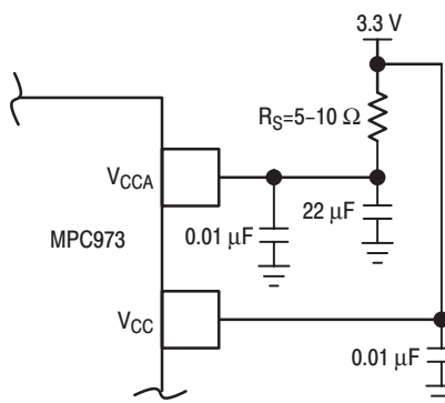
Figure 13. Power Supply Filter
