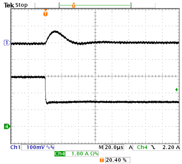
Fig-1.0V-7: Output voltage response for V_{out}=1.0V to negative load current step change from 3A to 1.5A with slew rate of -5A/us at V_{in}=12V . C_o=47\mu F \times 2 ceramic. Top trace: output voltage (100mV/div.) Bottom trace: load current (1A/div.) Time scale: 20us/div.
