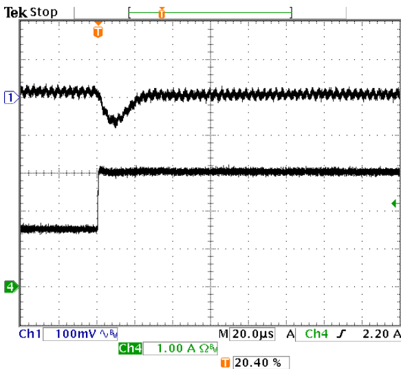
Fig-5.0V-6: Output voltage response for Vout=5.0V to positive load current step change from 1.5A to 3A with slew rate of 5A/us at Vin=12V. Co=47uFx2 ceramic. Top trace: output voltage (100mV/div.) Bottom trace: load current (1A/div.) Time scale: 20us/div.
