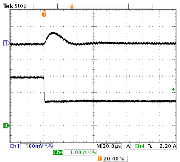
Fig-1.2V-7: Output voltage response for V_{out}=1.2V to negative load current step change from 3A to 1.5A with slew rate of -5A/\mu s at V_{in}=12V . C_o=47\mu F \times 2 ceramic. Top trace: output voltage (100mV/div.) Bottom trace: load current (1A/div.) Time scale: 20us/div.
