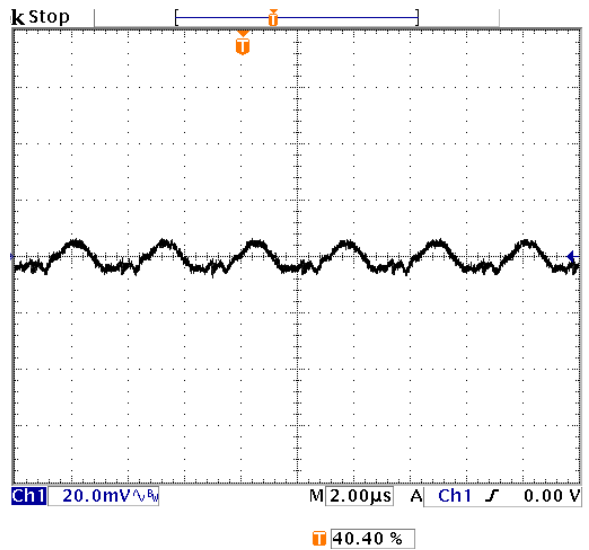
Fig-3.3V-5: Output voltage ripple (20mV/div.) for V_{out}=3.3V at full rated load current into a resistive load with external capacitance 47\mu F \times 2 ceramic + 1\mu F ceramic at V_{in}=12V . Time scale: 2 us/div.
