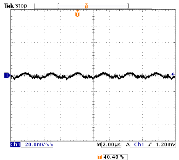
Fig-1.5V-5: Output voltage ripple (20mV/div.) for V_{out}=1.5V at full rated load current into a resistive load with external capacitance 47\mu F \times 2 ceramic + 1\mu F ceramic at V_{in}=12V . Time scale: 2 us/div
