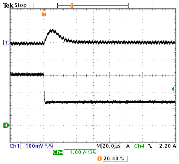
Fig-3.3V-7: Output voltage response for V_{out}=3.3V to negative load current step change from 3A to 1.5A with slew rate of -5A/\mu s at V_{in}=12V . C_o=47\mu F \times 2 ceramic. Top trace: output voltage (100mV/div.) Bottom trace: load current (1A/div.) Time scale: 20us/div.
