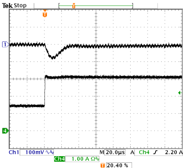
Fig-3.3V-6: Output voltage response for V_{out}=3.3V to positive load current step change from 1.5A to 3A with slew rate of 5A/\mu s at V_{in}=12V . C_o=47\mu F \times 2 ceramic. Top trace: output voltage (100mV/div.) Bottom trace: load current (1A/div.) Time scale: 20us/div.
