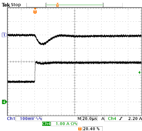
Fig-1.2V-6: Output voltage response for V_{out}=1.2V to positive load current step change from 1.5A to 3A with slew rate of 5A/\mu s at V_{in}=12V . C_o=47\mu F \times 2 ceramic. Top trace: output voltage (100mV/div.) Bottom trace: load current (1A/div.) Time scale: 20us/div.
