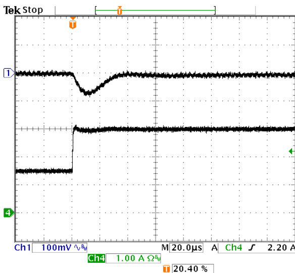
Fig-1.5V-6: Output voltage response for V_{out}=1.5V to positive load current step change from 1.5A to 3A with slew rate of 5A/\mu s at V_{in}=12V . C_o=47\mu F \times 2 ceramic. Top trace: output voltage (100mV/div.) Bottom trace: load current (1A/div.) Time scale: 20us/div.
