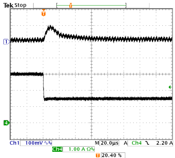
Fig-5.0V-7: Output voltage response for Vout=5.0V to negative load current step change from 3A to 1.5A with slew rate of -5A/us at Vin=12V. Co=47uFx2 ceramic. Top trace: output voltage (100mV/div.) Bottom trace: load current (1A/div.) Time scale: 20us/div.
