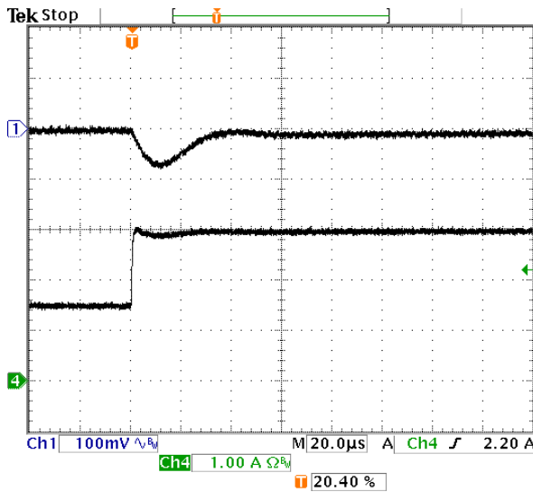
Fig-1.0V-6: Output voltage response for V_{out}=1.0V to positive load current step change from 1.5A to 3A with slew rate of 5A/us at V_{in}=12V . C_o=47\mu F \times 2 ceramic. Top trace: output voltage (100mV/div.) Bottom trace: load current (1A/div.) Time scale: 20us/div.
