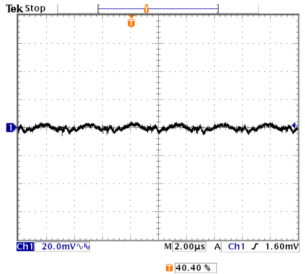
Fig-1.0V-5: Output voltage ripple (20mV/div.) for V_{out}=1.0V at full rated load current into a resistive load with external capacitance 47\mu F \times 2 ceramic + 1uF ceramic at V_{in}=12V . Time scale: 2 us/div
