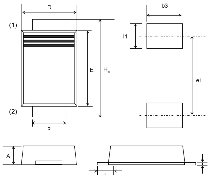
SOD-128, (PMDTM)
