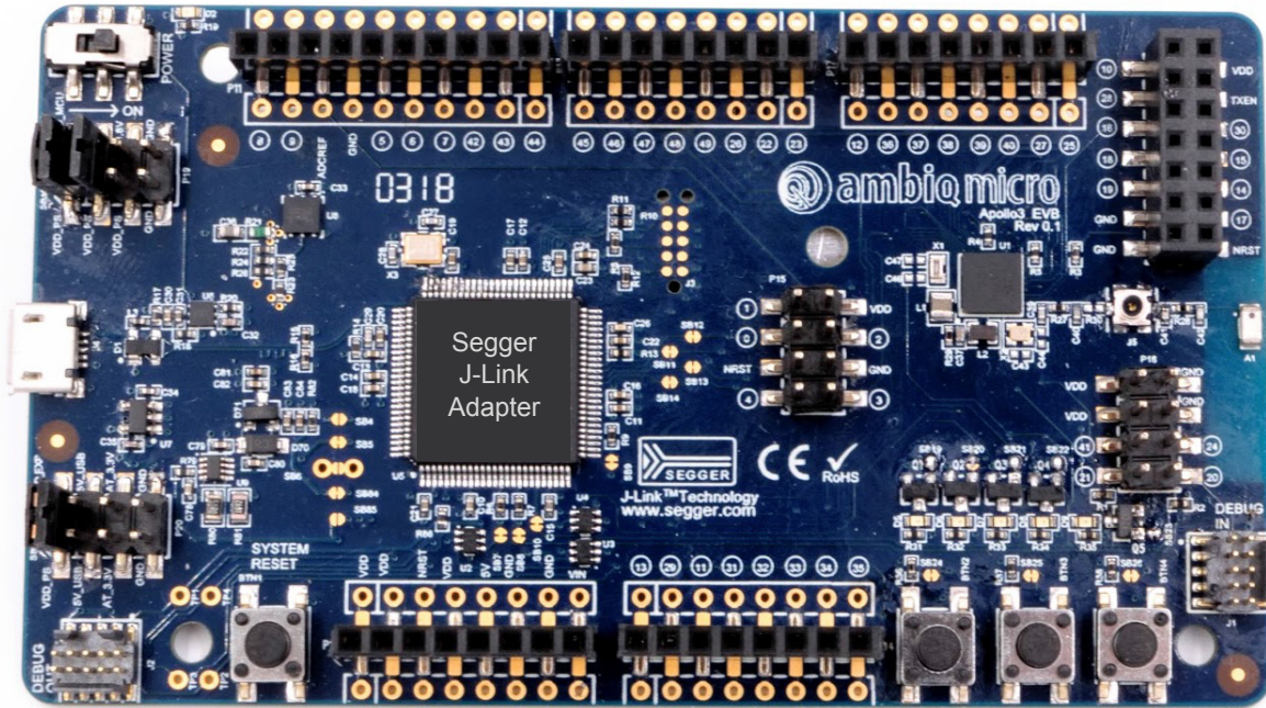
Figure 1. Apollo3 Blue EVB, Revision 1.0
