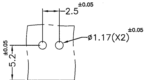
MOUNTING HOLE
