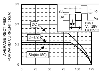
AMBIENT TEMPERATURE : T_a(^{\circ}C) Derating Curve*( I_o - T_a )
